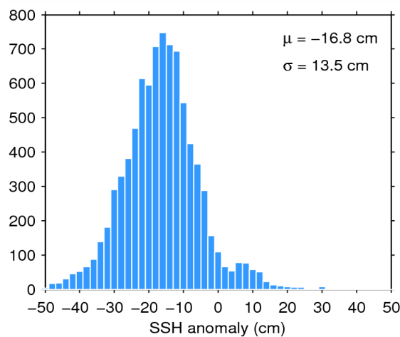
Figure 7. Histogram of flag-valid SSH anomaly over oceans and lakes for 01/11/2014. The mean ( \mu ) and standard deviation ( \sigma ) are also shown. Note that values outside [-50\ 50] cm are excluded from the histogram for the sake of readability but not from the computation of \mu and \sigma .
