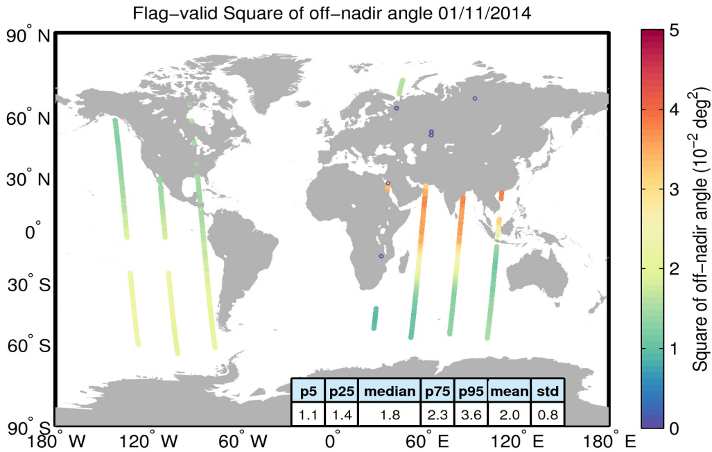
Figure 37. Geographical distribution of flag-valid mispointing data over oceans and lakes for 01/11/2014. The statistical values shown in the table refer to the mispointing in 10^{-2} \text{ deg}^2 and are calculated over all measurements shown in the figure.
