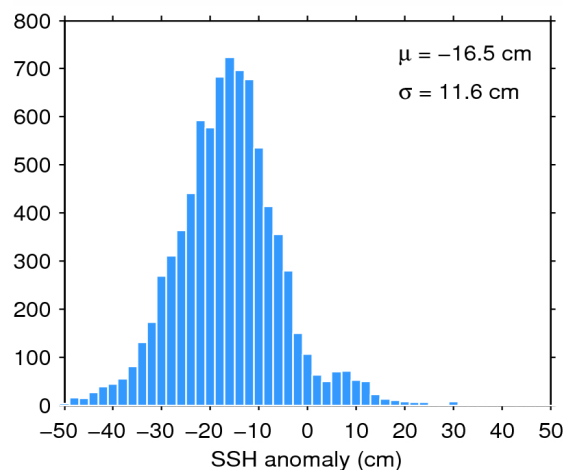
Figure 11. Histogram of science-valid SSH anomaly over oceans and lakes for 01/11/2014. The mean ( \mu ) and standard deviation ( \sigma ) are also shown. Note that values outside [-50 50] cm are excluded from the histogram for the sake of readability but not from the computation of \mu and \sigma .
