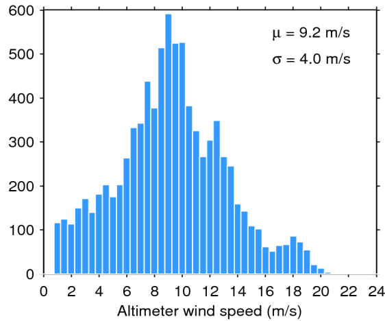
Figure 33. Histogram of flag-valid wind over oceans and lakes for 01/11/2014. The mean ( \mu ) and standard deviation ( \sigma ) are also shown. Note that values larger than 24 m/s are excluded from the histogram for the sake of readability but not from the computation of \mu and \sigma .
