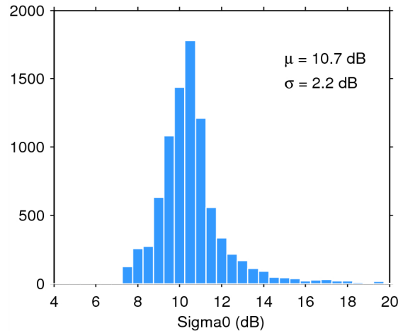
Figure 25. Histogram of flag-valid sigma0 over oceans and lakes for 01/11/2014. The mean ( \mu ) and standard deviation ( \sigma ) are also shown. Note that values outside [4 20] dB are excluded from the histogram for the sake of readability but not from the computation of \mu and \sigma .
