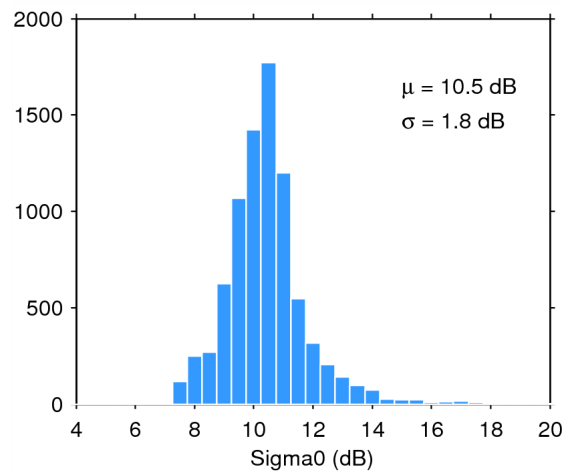
Figure 28. Histogram of science-valid sigma0 over oceans and lakes for 01/11/2014. The mean ( \mu ) and standard deviation ( \sigma ) are also shown. Note that values outside [4 20] dB are excluded from the histogram for the sake of readability but not from the computation of \mu and \sigma .
