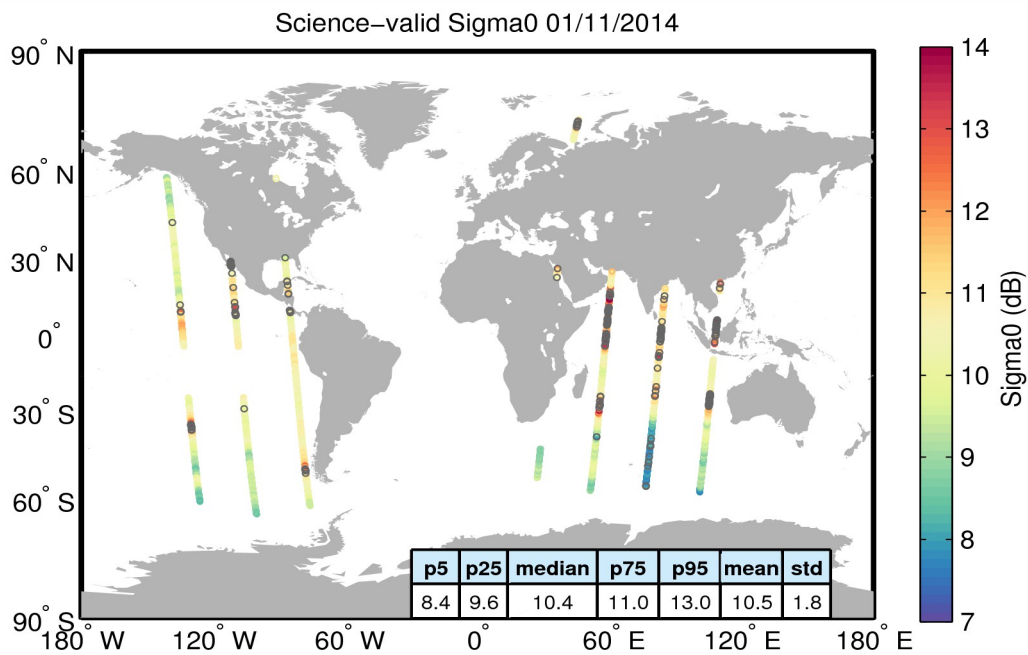
Figure 27. Geographical distribution of science-valid sigma0 data over oceans and lakes for 01/11/2014. The statistical values shown in the table refer to the sigma0 in dB and are calculated over all measurements shown in the figure. Gray circles denote records that have been rejected based on the editing criteria described in Table 4.
