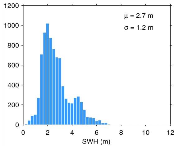
Figure 17. Histogram of flag-valid SWH over oceans and lakes for 01/11/2014. The mean ( \mu ) and standard deviation ( \sigma ) are also shown. Note that values larger than 12 m are excluded from the histogram for the sake of readability but not from the computation of \mu and \sigma .
