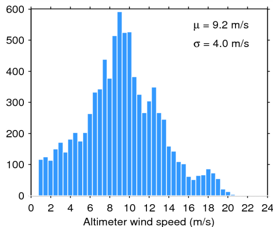
Figure 35. Histogram of science-valid wind over oceans and lakes for 01/11/2014. The mean ( \mu ) and standard deviation ( \sigma ) are also shown. Note that values larger than 24 m/s are excluded from the histogram for the sake of readability but not from the computation of \mu and \sigma .
