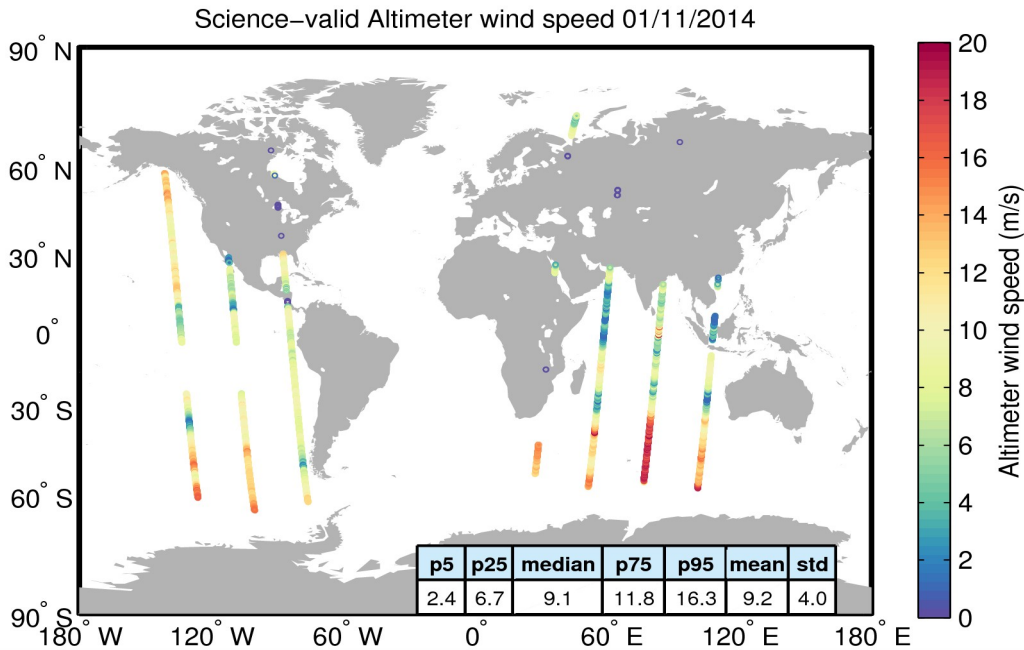
Figure 34. Geographical distribution of science-valid wind data over oceans and lakes for 01/11/2014. The statistical values shown in the table refer to the wind in m/s and are calculated over all measurements shown in the figure. Gray circles denote records that have been rejected based on the editing criteria described in Table 5.
