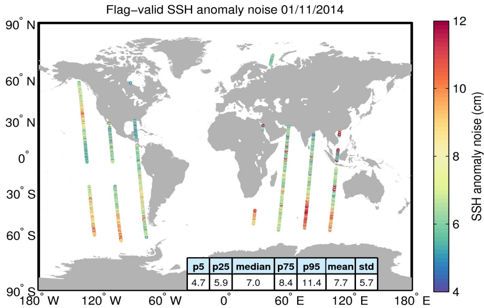
Figure 8. Geographical distribution of flag-valid 20-Hz SSH anomaly measurement noise over oceans and lakes for 01/11/2014. The statistical values shown in the table refer to the SSH anomaly noise and are calculated over all measurements shown in the figure.
