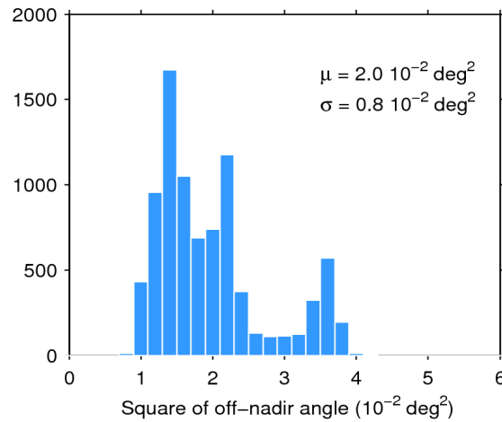
Figure 39. Histogram of flag-valid mispointing over oceans and lakes for 01/11/2014. The mean ( \mu ) and standard deviation ( \sigma ) are also shown. Note that values than 6 \cdot 10^{-2} \text{ deg}^2 are excluded from the histogram for the sake of readability but not from the computation of \mu and \sigma .
