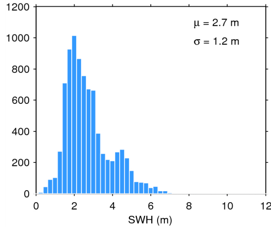
Figure 20. Histogram of science-valid SWH over oceans and lakes for 01/11/2014. The mean ( \mu ) and standard deviation ( \sigma ) are also shown. Note that values larger than 12 m are excluded from the histogram for the sake of readability but not from the computation of \mu and \sigma .
