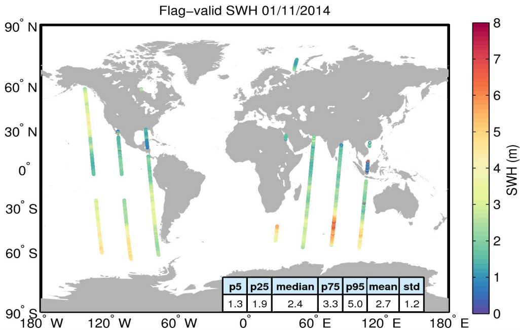
Figure 15. Geographical distribution of flag-valid SWH data over oceans and lakes for 01/11/2014. The statistical values shown in the figure refer to the SWH in m and are calculated over all measurements shown in the figure.
