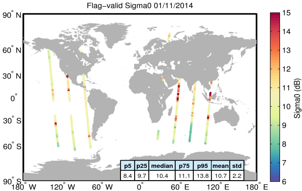
Figure 23. Geographical distribution of flag-valid sigma0 data over oceans and lakes for 01/11/2014. The statistical values shown in the table refer to the sigma0 in dB and are calculated over all measurements shown in the figure.
