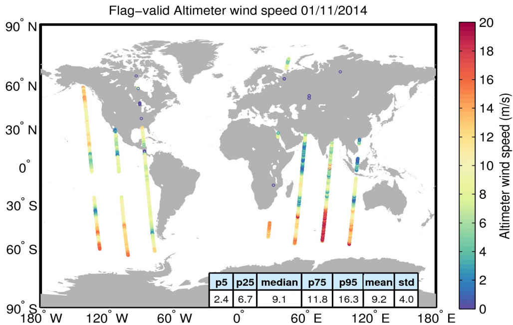
Figure 31. Geographical distribution of flag-valid wind data over oceans and lakes for 01/11/2014. The statistical values shown in the table refer to the wind in m/s and are calculated over all measurements shown in the figure.
