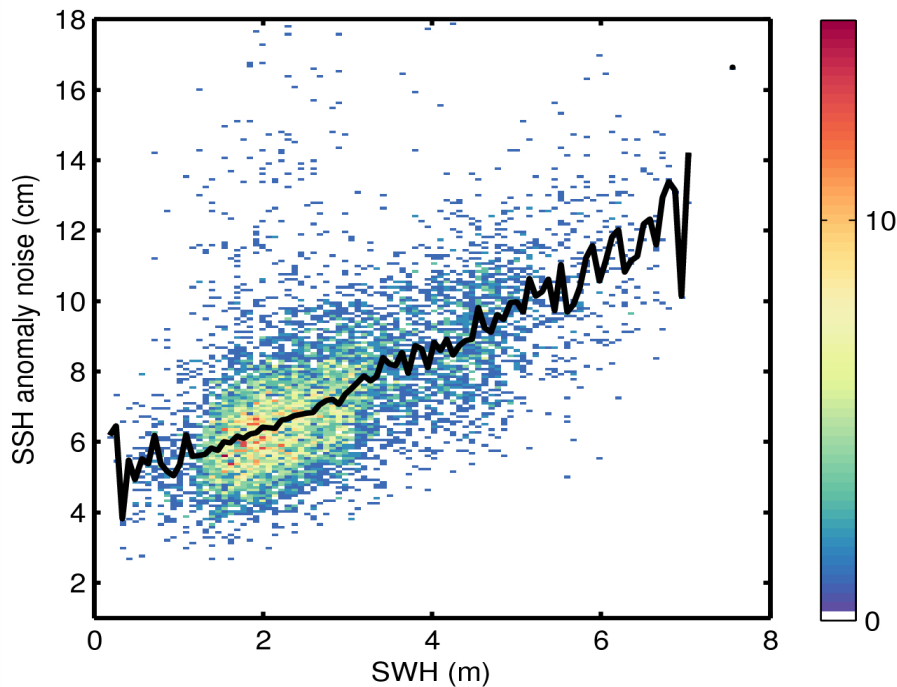
Figure 9. 2D histogram showing flag-valid SSH anomaly noise as a function of SWH for 01/11/2014. The black line denotes the median SSH anomaly as a function of SWH.
