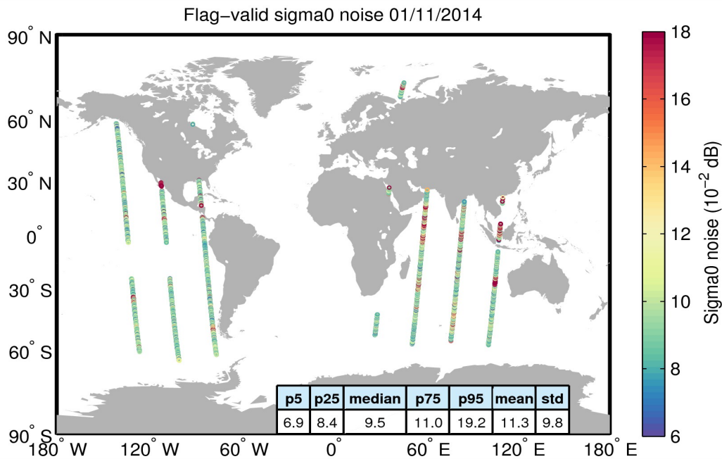
Figure 26. Geographical distribution of flag-valid 20-Hz sigma0 measurement noise over oceans and lakes for 01/11/2014. The statistical values shown in the table refer to the sigma0 noise and are calculated over all measurements shown in the figure.
