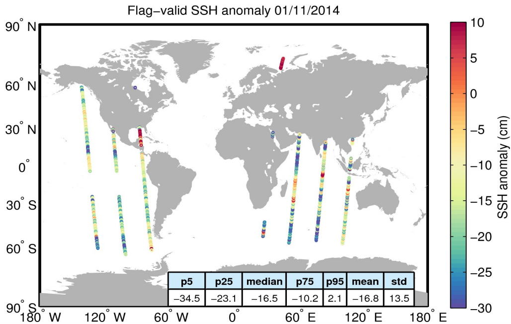
Figure 5. Geographical distribution of flag-valid 1-Hz SSH anomaly data over oceans and lakes for 01/11/2014. The statistical values shown in the table refer to the SSH anomaly in cm and are calculated over all measurements shown in the figure.
