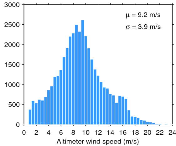
Figure 33. Histogram of flag-valid wind over oceans and lakes for 30/10/2014. The mean ( \mu ) and standard deviation ( \sigma ) are also shown. Note that values larger than 24 m/s are excluded from the histogram for the sake of readability but not from the computation of \mu and \sigma .
