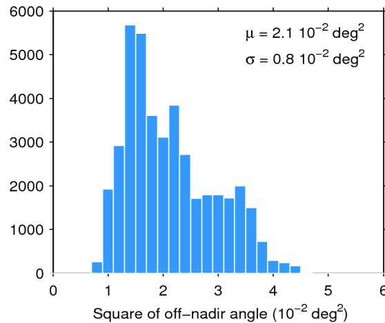
Figure 39. Histogram of flag-valid mispointing over oceans and lakes for 30/10/2014. The mean ( \mu ) and standard deviation ( \sigma ) are also shown. Note that values than 6 \cdot 10^{-2} \text{ deg}^2 are excluded from the histogram for the sake of readability but not from the computation of \mu and \sigma .
