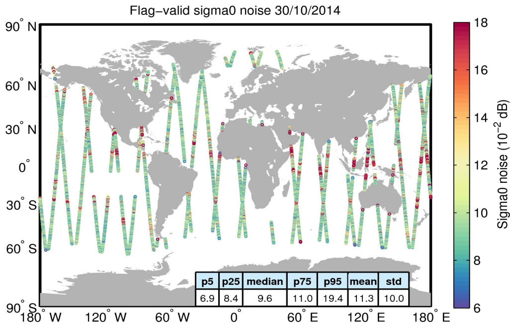
Figure 26. Geographical distribution of flag-valid 20-Hz sigma0 measurement noise over oceans and lakes for 30/10/2014. The statistical values shown in the table refer to the sigma0 noise and are calculated over all measurements shown in the figure.
