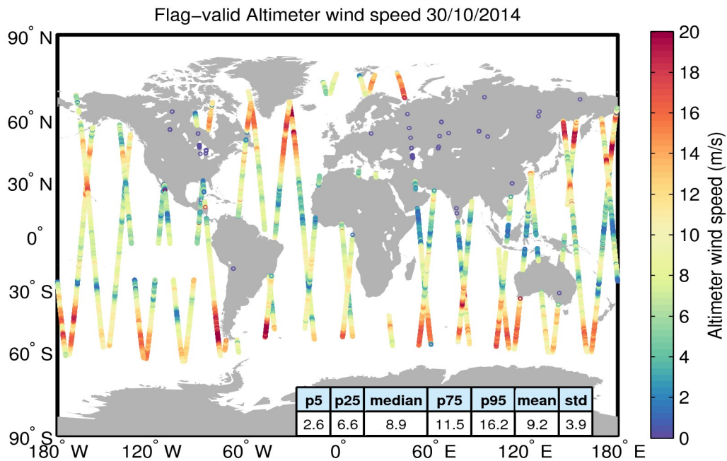
Figure 31. Geographical distribution of flag-valid wind data over oceans and lakes for 30/10/2014. The statistical values shown in the table refer to the wind in m/s and are calculated over all measurements shown in the figure.
