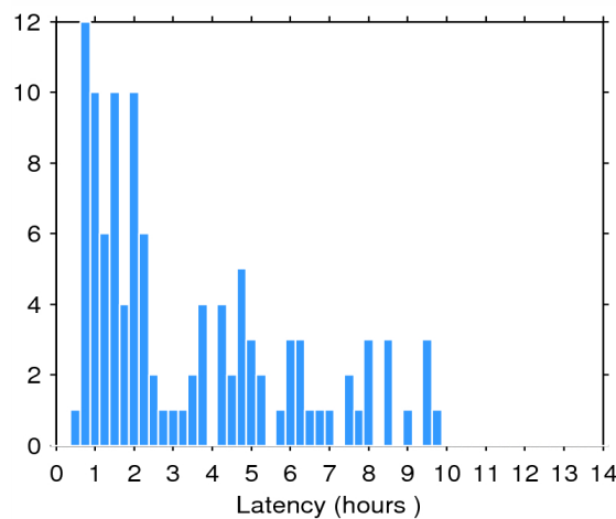
Figure 2. Histogram of the data latency for 30/10/2014. The y-axis denotes the number of files that are made available with a delay of x-hours with respect to the mean time of the records stored in the file.
