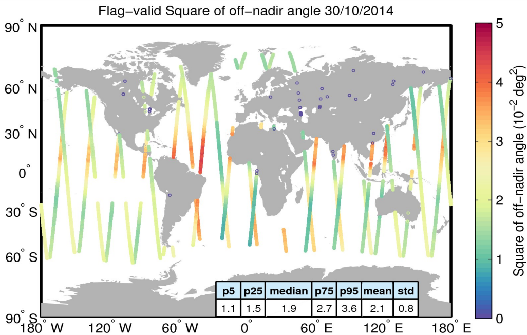
Figure 37. Geographical distribution of flag-valid mispointing data over oceans and lakes for 30/10/2014. The statistical values shown in the table refer to the mispointing in 10^{-2} deg 2 and are calculated over all measurements shown in the figure.
