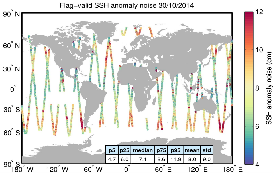
Figure 8. Geographical distribution of flag-valid 20-Hz SSH anomaly measurement noise over oceans and lakes for 30/10/2014. The statistical values shown in the table refer to the SSH anomaly noise and are calculated over all measurements shown in the figure.
