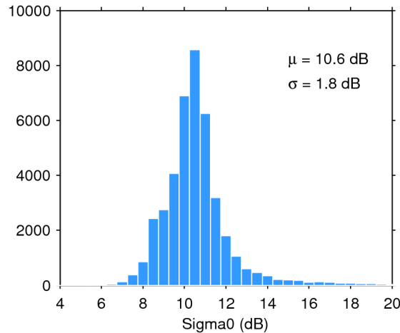
Figure 25. Histogram of flag-valid sigma0 over oceans and lakes for 30/10/2014. The mean ( \mu ) and standard deviation ( \sigma ) are also shown. Note that values outside [4 20] dB are excluded from the histogram for the sake of readability but not from the computation of \mu and \sigma .
