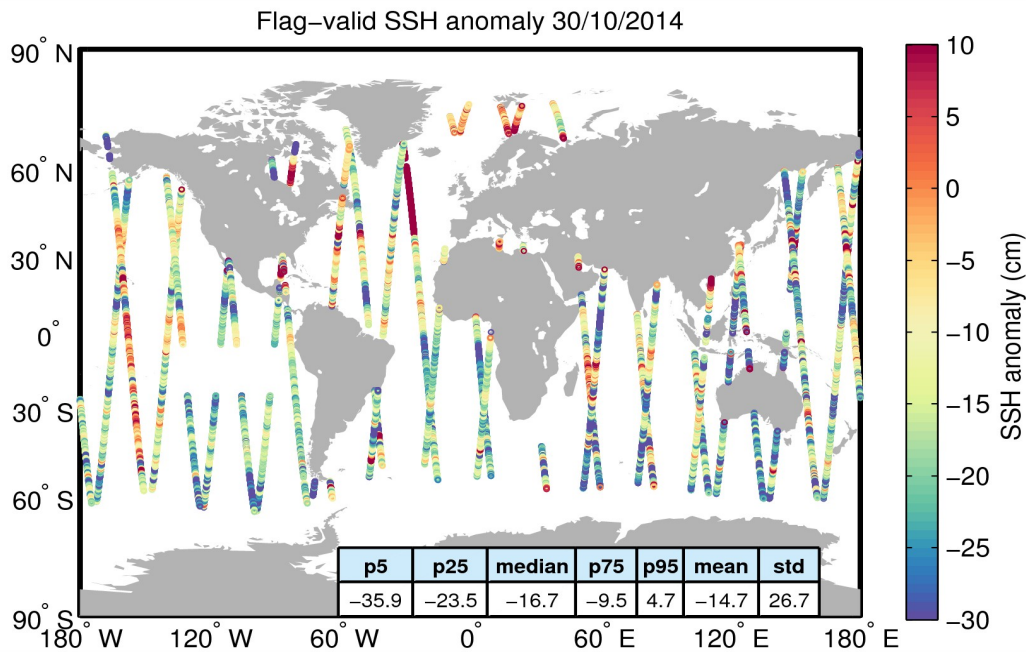
Figure 5. Geographical distribution of flag-valid 1-Hz SSH anomaly data over oceans and lakes for 30/10/2014. The statistical values shown in the table refer to the SSH anomaly in cm and are calculated over all measurements shown in the figure.
