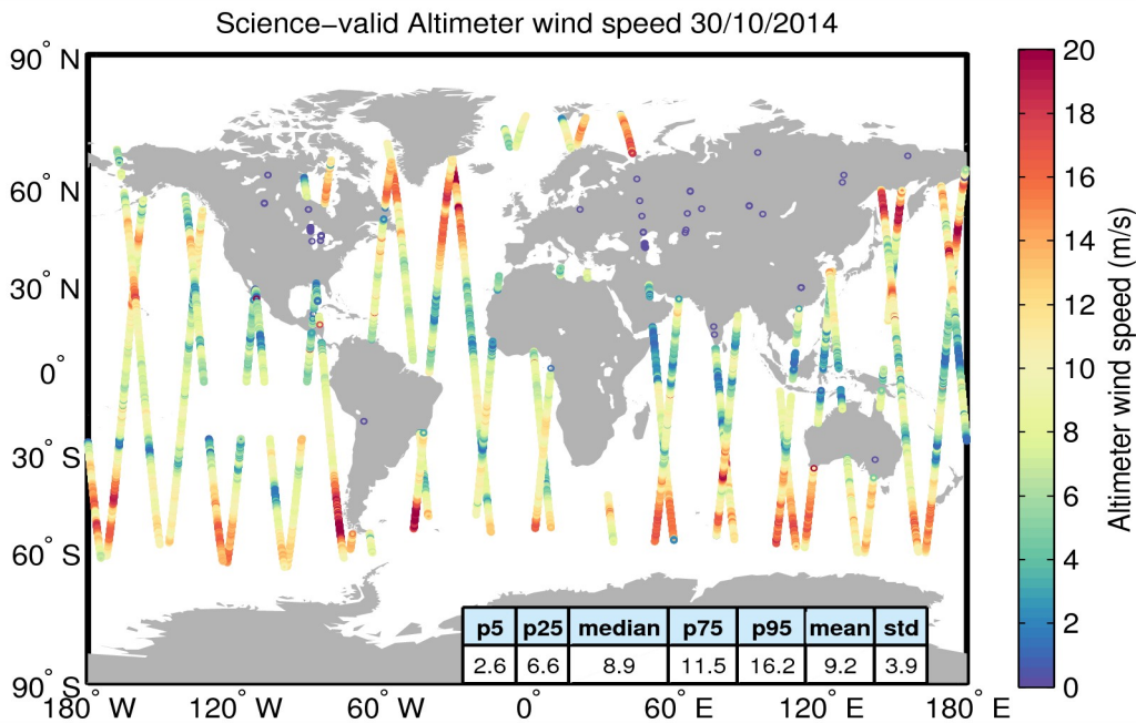
Figure 34. Geographical distribution of science-valid wind data over oceans and lakes for 30/10/2014. The statistical values shown in the table refer to the wind in m/s and are calculated over all measurements shown in the figure. Gray circles denote records that have been rejected based on the editing criteria described in Table 5.
