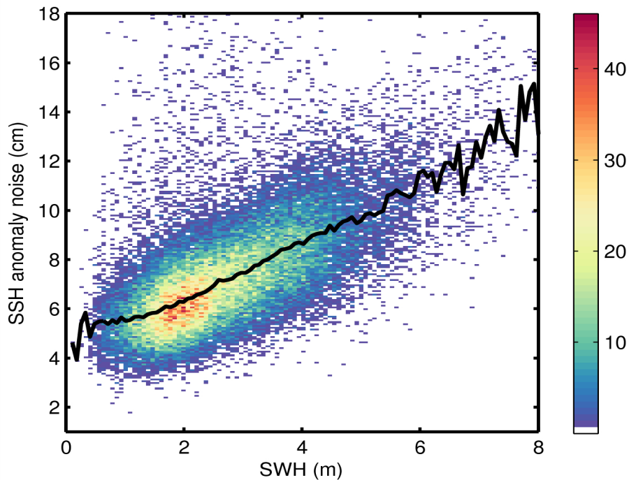
Figure 9. 2D histogram showing flag-valid SSH anomaly noise as a function of SWH for 30/10/2014. The black line denotes the median SSH anomaly as a function of SWH.
