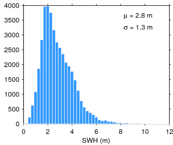
Figure 17. Histogram of flag-valid SWH over oceans and lakes for 30/10/2014. The mean ( \mu ) and standard deviation ( \sigma ) are also shown. Note that values larger than 12 m are excluded from the histogram for the sake of readability but not from the computation of \mu and \sigma .
