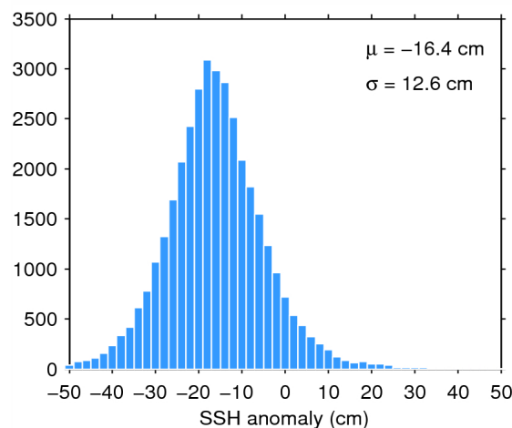
Figure 11. Histogram of science-valid SSH anomaly over oceans and lakes for 30/10/2014. The mean ( \mu ) and standard deviation ( \sigma ) are also shown. Note that values outside [-50 50] cm are excluded from the histogram for the sake of readability but not from the computation of \mu and \sigma .
