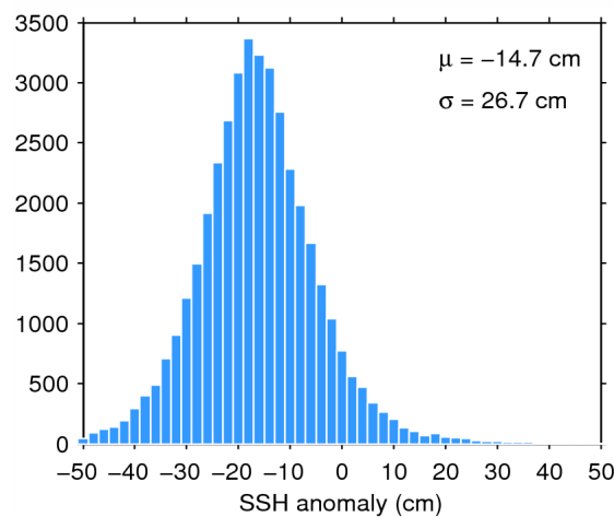
Figure 7. Histogram of flag-valid SSH anomaly over oceans and lakes for 30/10/2014. The mean ( \mu ) and standard deviation ( \sigma ) are also shown. Note that values outside [-50 50] cm are excluded from the histogram for the sake of readability but not from the computation of \mu and \sigma .
