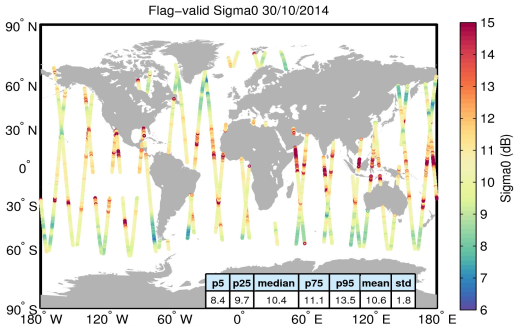
Figure 23. Geographical distribution of flag-valid sigma0 data over oceans and lakes for 30/10/2014. The statistical values shown in the table refer to the sigma0 in dB and are calculated over all measurements shown in the figure.
