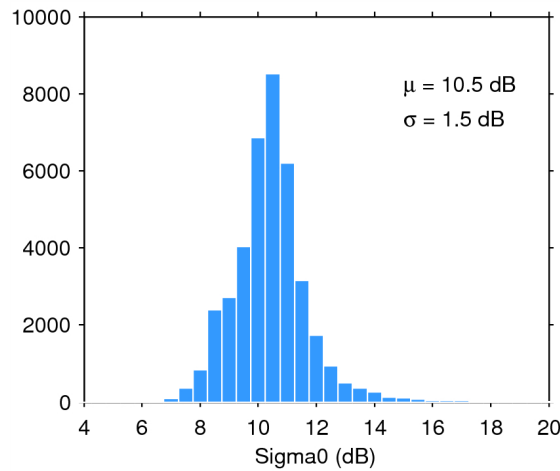
Figure 28. Histogram of science-valid sigma0 over oceans and lakes for 30/10/2014. The mean ( \mu ) and standard deviation ( \sigma ) are also shown. Note that values outside [4 20] dB are excluded from the histogram for the sake of readability but not from the computation of \mu and \sigma .
