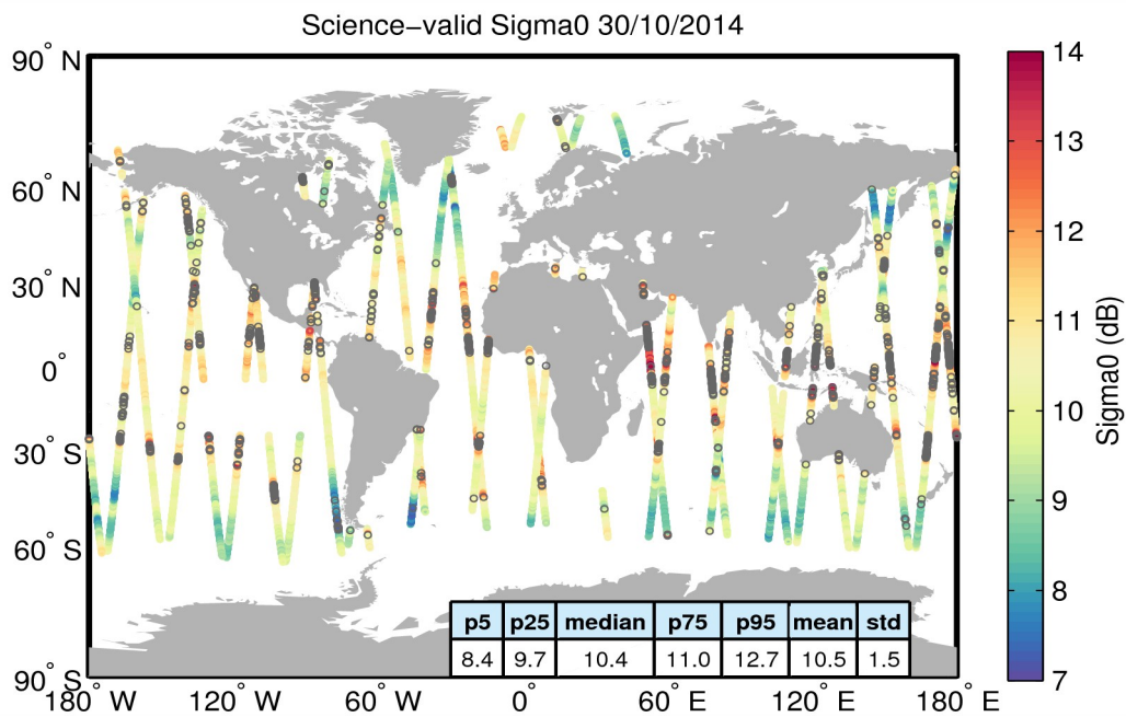
Figure 27. Geographical distribution of science-valid sigma0 data over oceans and lakes for 30/10/2014. The statistical values shown in the table refer to the sigma0 in dB and are calculated over all measurements shown in the figure. Gray circles denote records that have been rejected based on the editing criteria described in Table 4.
