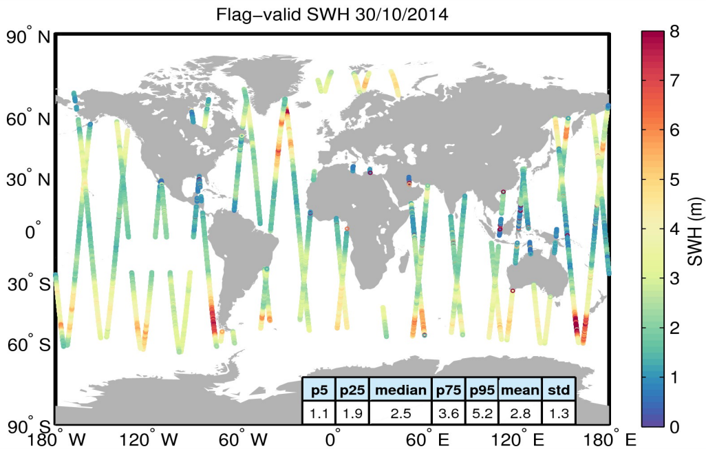
Figure 15. Geographical distribution of flag-valid SWH data over oceans and lakes for 30/10/2014. The statistical values shown in the table refer to the SWH in m and are calculated over all measurements shown in the figure.
