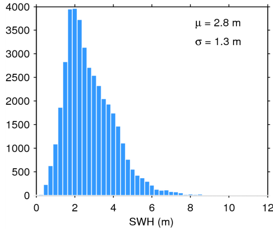
Figure 20. Histogram of science-valid SWH over oceans and lakes for 30/10/2014. The mean ( \mu ) and standard deviation ( \sigma ) are also shown. Note that values larger than 12 m are excluded from the histogram for the sake of readability but not from the computation of \mu and \sigma .
