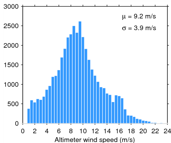
Figure 35. Histogram of science-valid wind over oceans and lakes for 30/10/2014. The mean ( \mu ) and standard deviation ( \sigma ) are also shown. Note that values larger than 24 m/s are excluded from the histogram for the sake of readability but not from the computation of \mu and \sigma .
