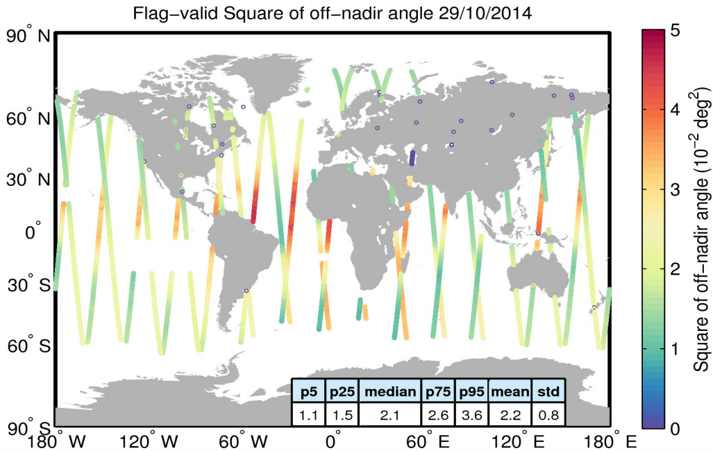
Figure 37. Geographical distribution of flag-valid mispointing data over oceans and lakes for 29/10/2014. The statistical values shown in the table refer to the mispointing in 10^{-2} \text{ deg}^2 and are calculated over all measurements shown in the figure.
