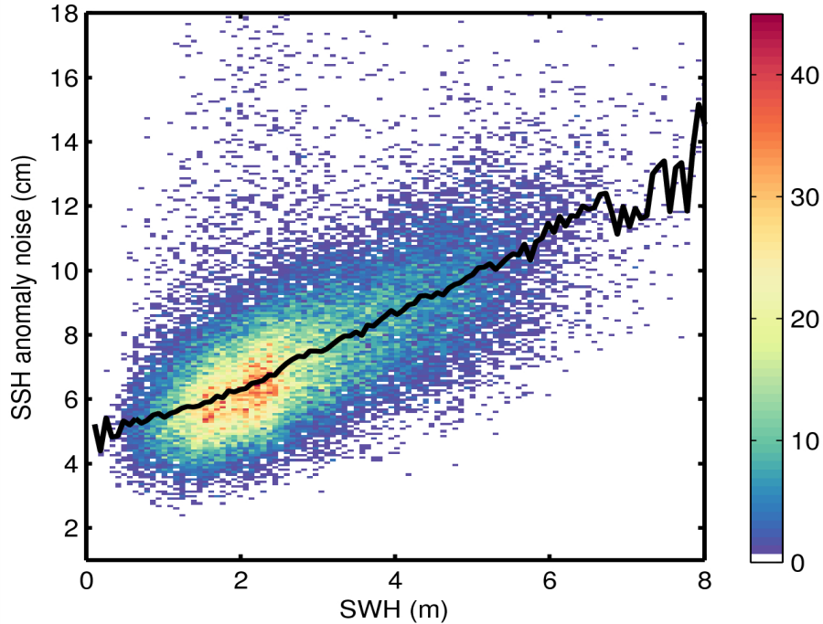
Figure 9. 2D histogram showing flag-valid SSH anomaly noise as a function of SWH for 29/10/2014. The black line denotes the median SSH anomaly as a function of SWH.
