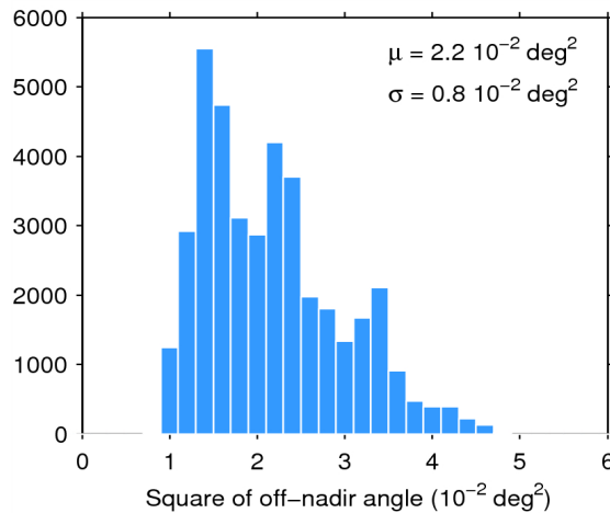
Figure 39. Histogram of flag-valid mispointing over oceans and lakes for 29/10/2014. The mean ( \mu ) and standard deviation ( \sigma ) are also shown. Note that values than 6 \cdot 10^{-2} \text{ deg}^2 are excluded from the histogram for the sake of readability but not from the computation of \mu and \sigma .
