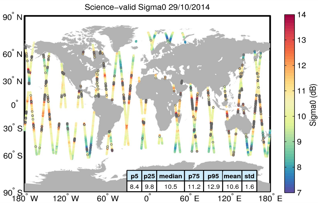
Figure 27. Geographical distribution of science-valid sigma0 data over oceans and lakes for 29/10/2014. The statistical values shown in the table refer to the sigma0 in dB and are calculated over all measurements shown in the figure. Gray circles denote records that have been rejected based on the editing criteria described in Table 4.
