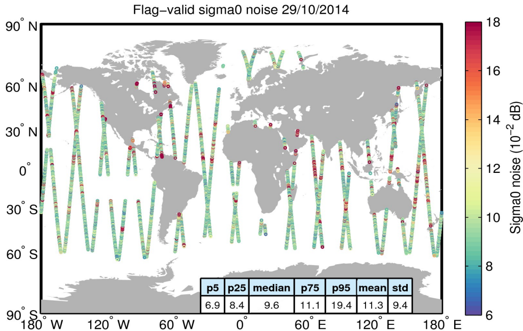
Figure 26. Geographical distribution of flag-valid 20-Hz sigma0 measurement noise over oceans and lakes for 29/10/2014. The statistical values shown in the table refer to the sigma0 noise and are calculated over all measurements shown in the figure.
