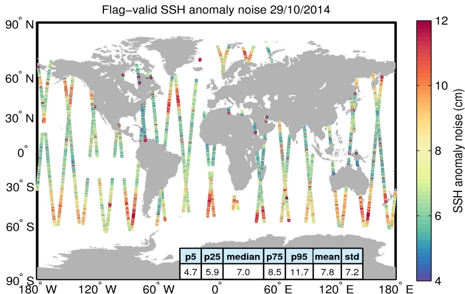
Figure 8. Geographical distribution of flag-valid 20-Hz SSH anomaly measurement noise over oceans and lakes for 29/10/2014. The statistical values shown in the table refer to the SSH anomaly noise and are calculated over all measurements shown in the figure.
