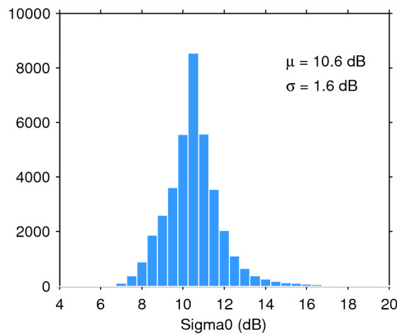
Figure 28. Histogram of science-valid sigma0 over oceans and lakes for 29/10/2014. The mean ( \mu ) and standard deviation ( \sigma ) are also shown. Note that values outside [4 20] dB are excluded from the histogram for the sake of readability but not from the computation of \mu and \sigma .
