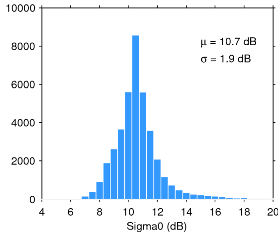
Figure 25. Histogram of flag-valid sigma0 over oceans and lakes for 29/10/2014. The mean ( \mu ) and standard deviation ( \sigma ) are also shown. Note that values outside [4 20] dB are excluded from the histogram for the sake of readability but not from the computation of \mu and \sigma .
