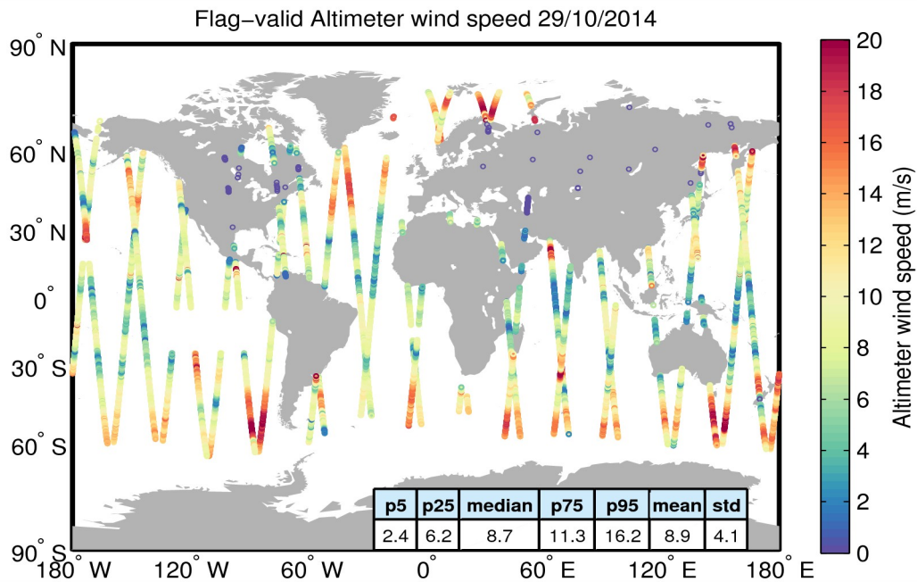
Figure 31. Geographical distribution of flag-valid wind data over oceans and lakes for 29/10/2014. The statistical values shown in the table refer to the wind in m/s and are calculated over all measurements shown in the figure.
