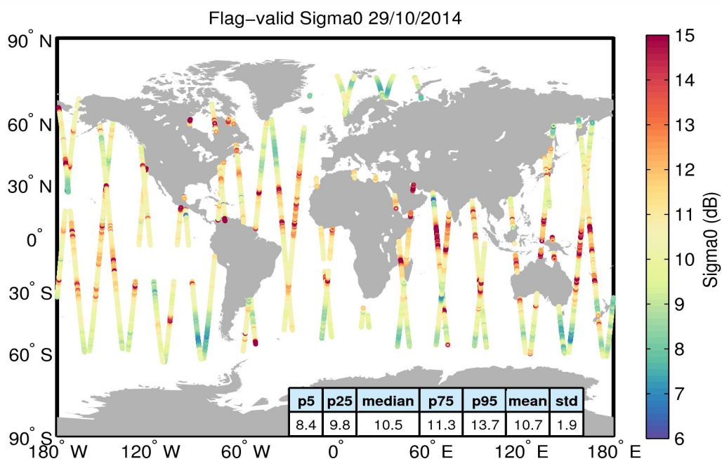
Figure 23. Geographical distribution of flag-valid sigma0 data over oceans and lakes for 29/10/2014. The statistical values shown in the table refer to the sigma0 in dB and are calculated over all measurements shown in the figure.
