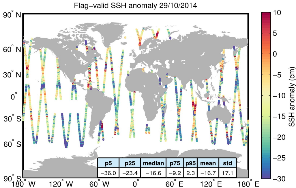
Figure 5. Geographical distribution of flag-valid 1-Hz SSH anomaly data over oceans and lakes for 29/10/2014. The statistical values shown in the table refer to the SSH anomaly in cm and are calculated over all measurements shown in the figure.
