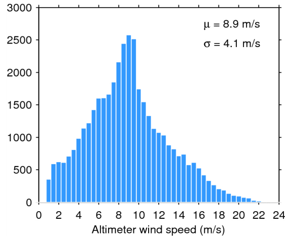
Figure 33. Histogram of flag-valid wind over oceans and lakes for 29/10/2014. The mean ( \mu ) and standard deviation ( \sigma ) are also shown. Note that values larger than 24 m/s are excluded from the histogram for the sake of readability but not from the computation of \mu and \sigma .
