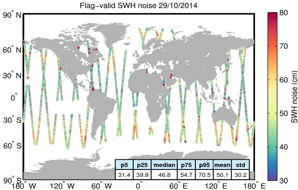
Figure 18. Geographical distribution of flag-valid 20-Hz SWH measurement noise over oceans and lakes for 29/10/2014. The statistical values shown in the figure refer to the SWH noise and are calculated over all measurements shown in the figure.
