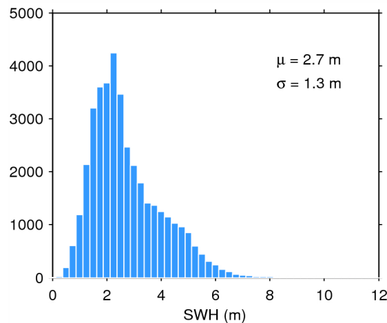
Figure 20. Histogram of science-valid SWH over oceans and lakes for 29/10/2014. The mean ( \mu ) and standard deviation ( \sigma ) are also shown. Note that values larger than 12 m are excluded from the histogram for the sake of readability but not from the computation of \mu and \sigma .
