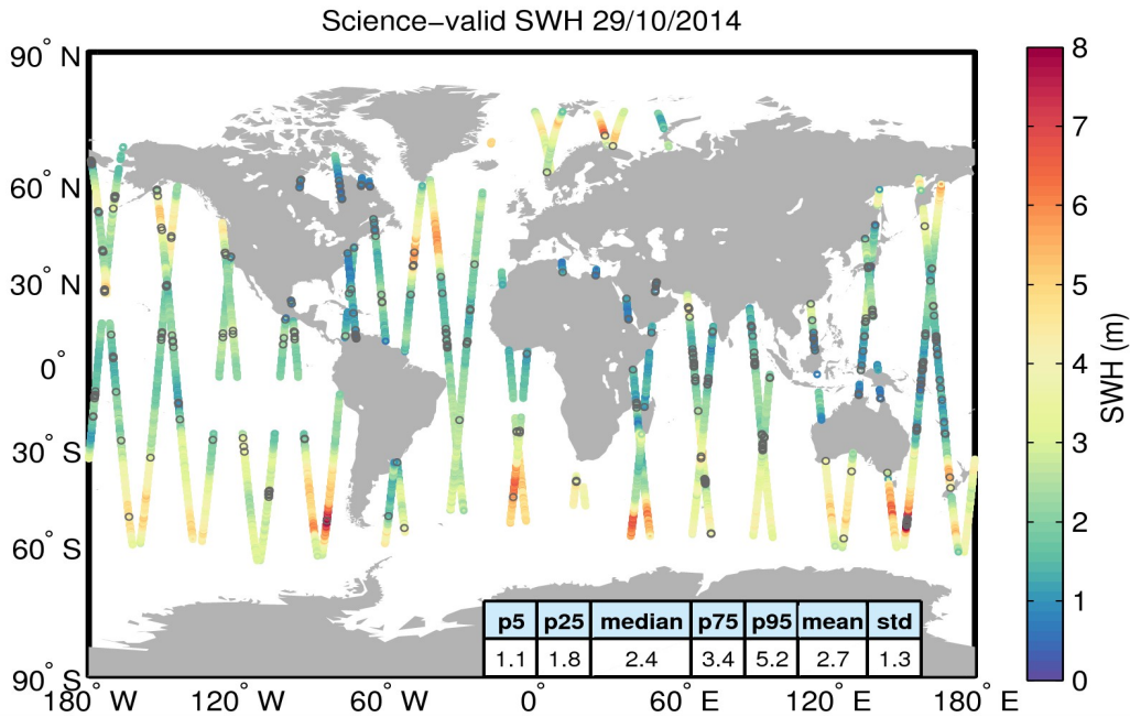
Figure 19. Geographical distribution of science-valid SWH data over oceans and lakes for 29/10/2014. The statistical values shown in the table refer to the SWH in m and are calculated over all measurements shown in the figure. Gray circles denote records that have been rejected based on the editing criteria described in Table 3.
