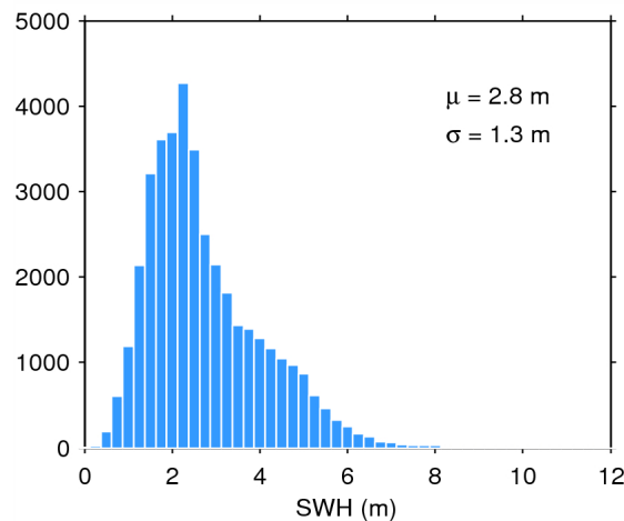
Figure 17. Histogram of flag-valid SWH over oceans and lakes for 29/10/2014. The mean ( \mu ) and standard deviation ( \sigma ) are also shown. Note that values larger than 12 m are excluded from the histogram for the sake of readability but not from the computation of \mu and \sigma .
