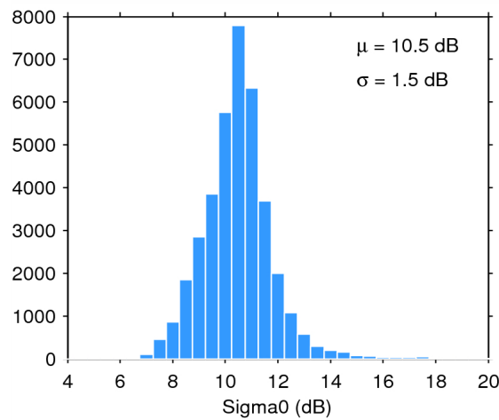
Figure 28. Histogram of science-valid sigma0 over oceans and lakes for 28/10/2014. The mean ( \mu ) and standard deviation ( \sigma ) are also shown. Note that values outside [4 20] dB are excluded from the histogram for the sake of readability but not from the computation of \mu and \sigma .
