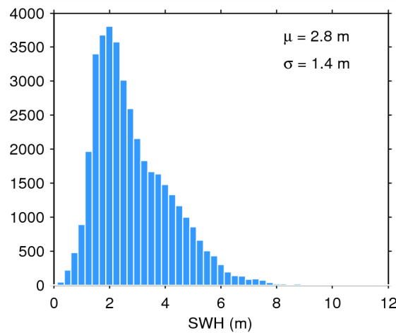
Figure 17. Histogram of flag-valid SWH over oceans and lakes for 28/10/2014. The mean ( \mu ) and standard deviation ( \sigma ) are also shown. Note that values larger than 12 m are excluded from the histogram for the sake of readability but not from the computation of \mu and \sigma .
