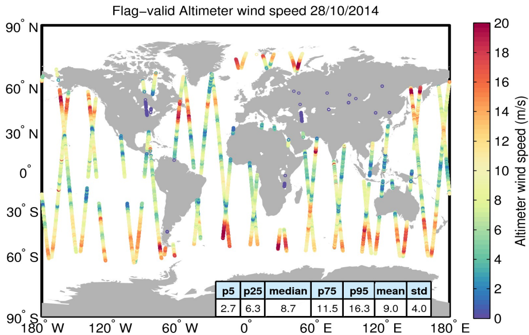
Figure 31. Geographical distribution of flag-valid wind data over oceans and lakes for 28/10/2014. The statistical values shown in the table refer to the wind in m/s and are calculated over all measurements shown in the figure.
