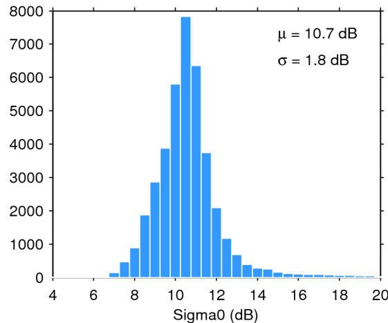
Figure 25. Histogram of flag-valid sigma0 over oceans and lakes for 28/10/2014. The mean ( \mu ) and standard deviation ( \sigma ) are also shown. Note that values outside [4 20] dB are excluded from the histogram for the sake of readability but not from the computation of \mu and \sigma .
