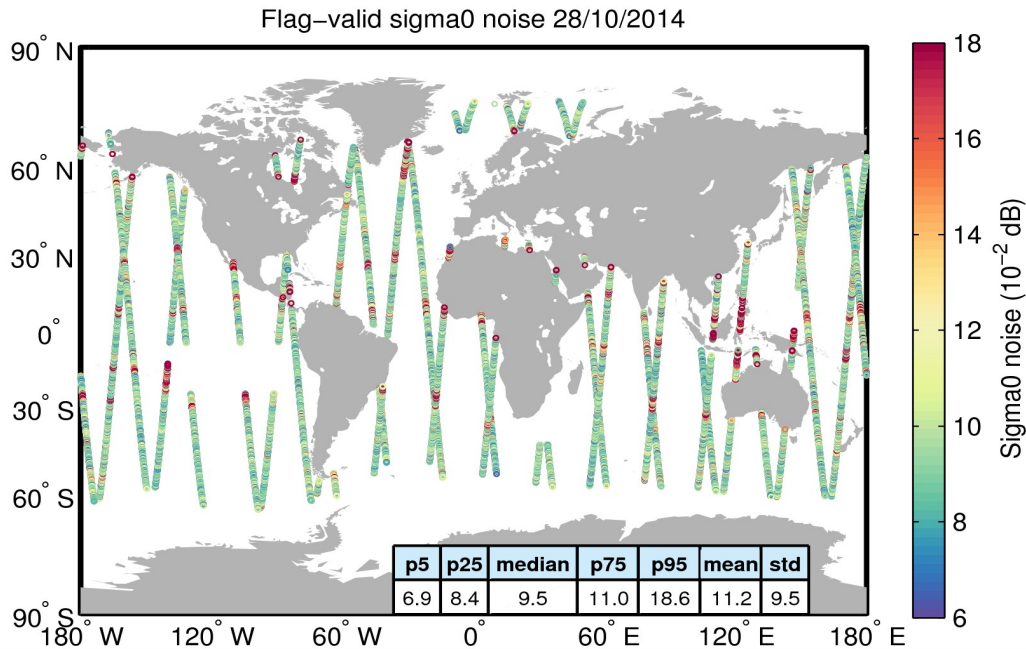
Figure 26. Geographical distribution of flag-valid 20-Hz sigma0 measurement noise over oceans and lakes for 28/10/2014. The statistical values shown in the table refer to the sigma0 noise and are calculated over all measurements shown in the figure.
