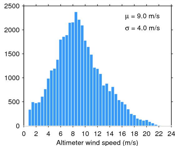
Figure 35. Histogram of science-valid wind over oceans and lakes for 28/10/2014. The mean ( \mu ) and standard deviation ( \sigma ) are also shown. Note that values larger than 24 m/s are excluded from the histogram for the sake of readability but not from the computation of \mu and \sigma .
