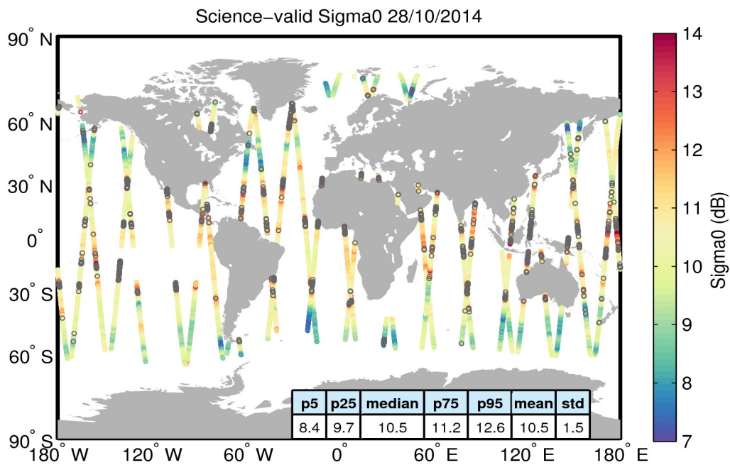
Figure 27. Geographical distribution of science-valid sigma0 data over oceans and lakes for 28/10/2014. The statistical values shown in the table refer to the sigma0 in dB and are calculated over all measurements shown in the figure. Gray circles denote records that have been rejected based on the editing criteria described in Table 4.
