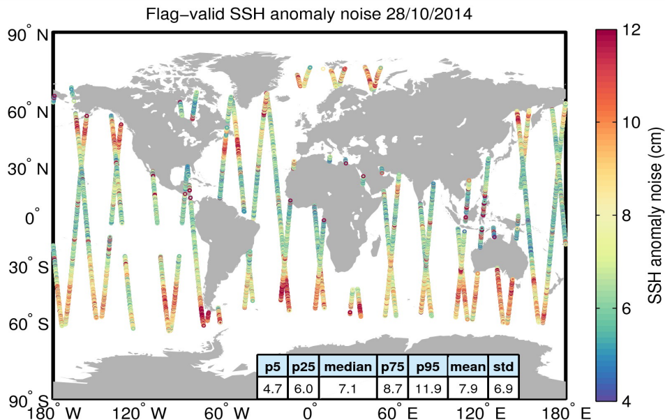
Figure 8. Geographical distribution of flag-valid 20-Hz SSH anomaly measurement noise over oceans and lakes for 28/10/2014. The statistical values shown in the table refer to the SSH anomaly noise and are calculated over all measurements shown in the figure.
