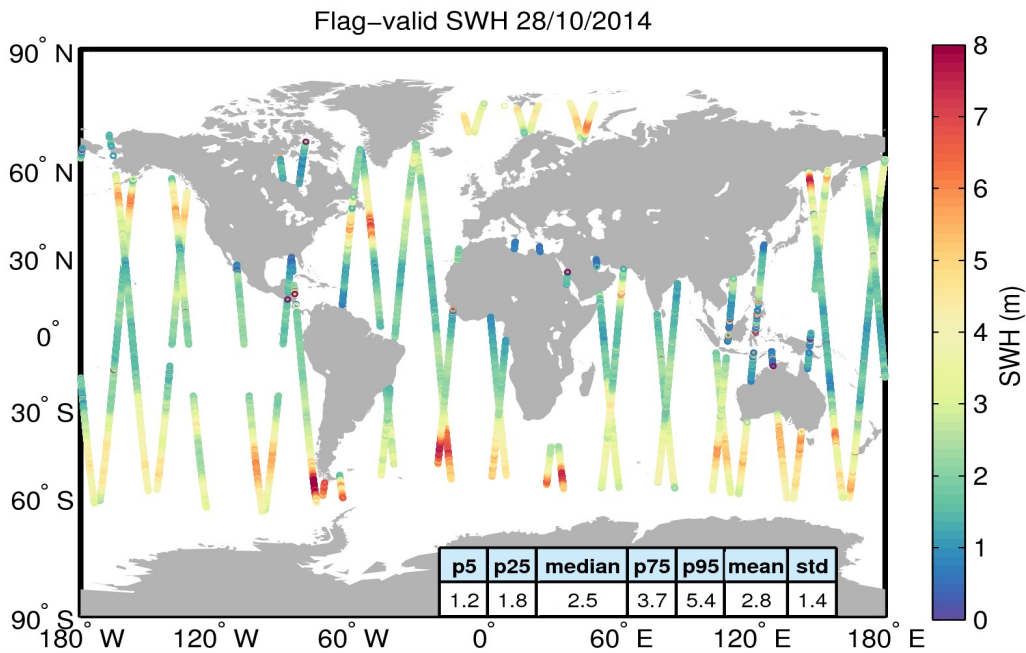
Figure 15. Geographical distribution of flag-valid SWH data over oceans and lakes for 28/10/2014. The statistical values shown in the table refer to the SWH in m and are calculated over all measurements shown in the figure.
