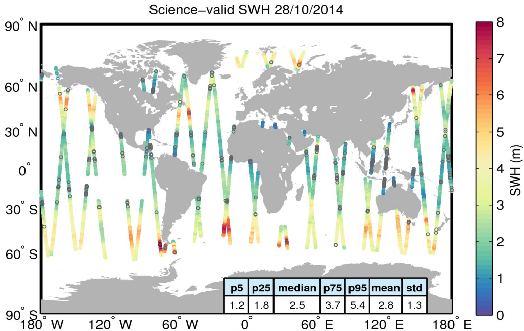
Figure 19. Geographical distribution of science-valid SWH data over oceans and lakes for 28/10/2014. The statistical values shown in the table refer to the SWH in m and are calculated over all measurements shown in the figure. Gray circles denote records that have been rejected based on the editing criteria described in Table 3.
