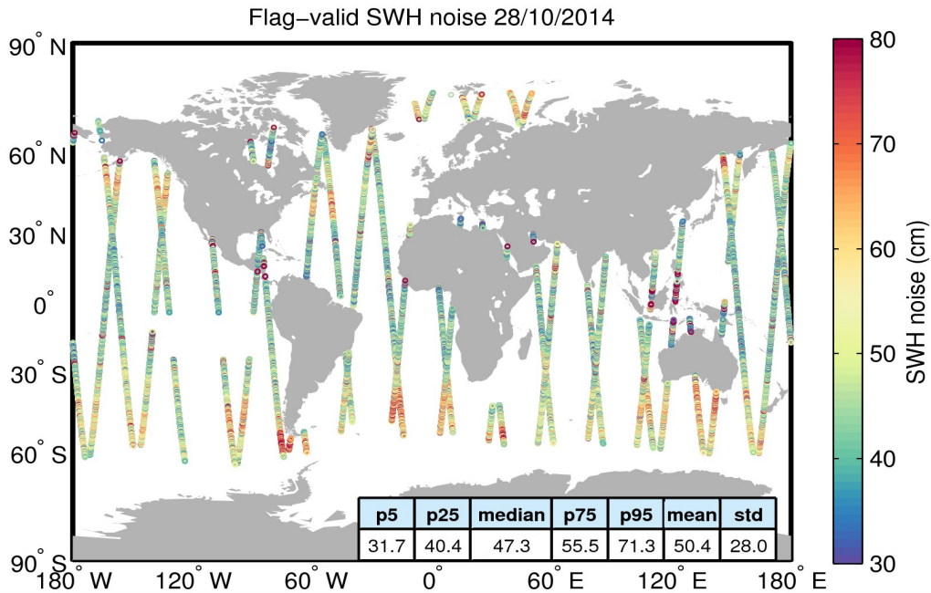
Figure 18. Geographical distribution of flag-valid 20-Hz SWH measurement noise over oceans and lakes for 28/10/2014. The statistical values shown in the figure refer to the SWH noise and are calculated over all measurements shown in the figure.
