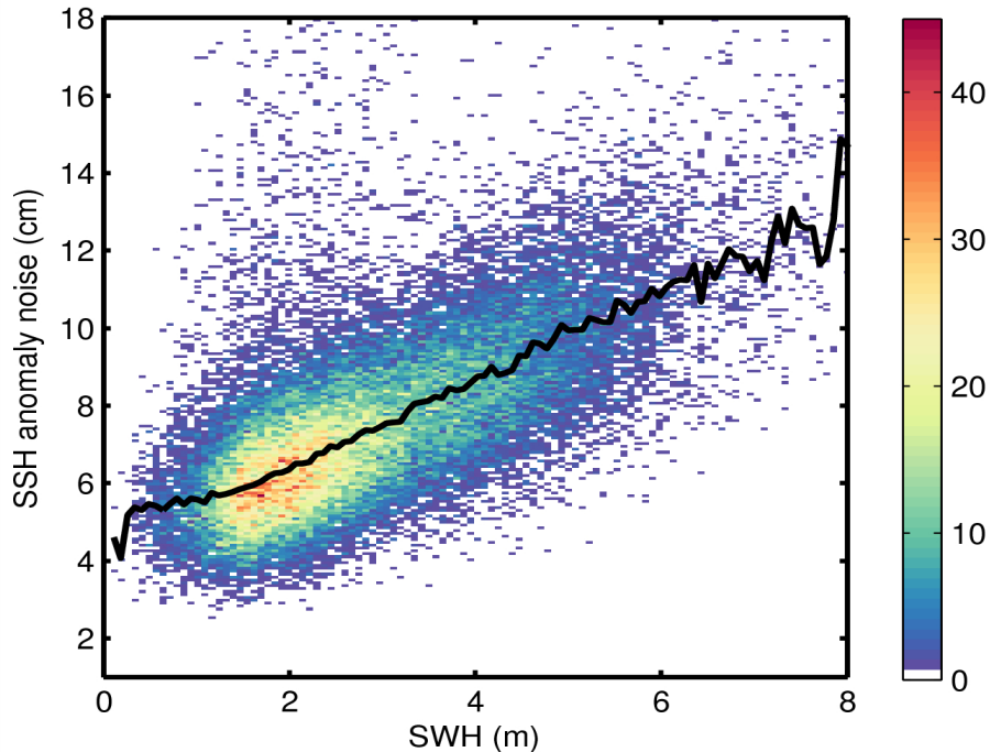
Figure 9. 2D histogram showing flag-valid SSH anomaly noise as a function of SWH for 28/10/2014. The black line denotes the median SSH anomaly as a function of SWH.
