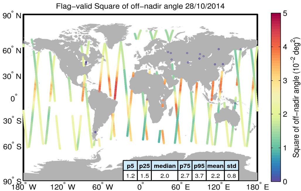
Figure 37. Geographical distribution of flag-valid mispointing data over oceans and lakes for 28/10/2014. The statistical values shown in the table refer to the mispointing in 10^{-2} \text{ deg}^2 and are calculated over all measurements shown in the figure.
