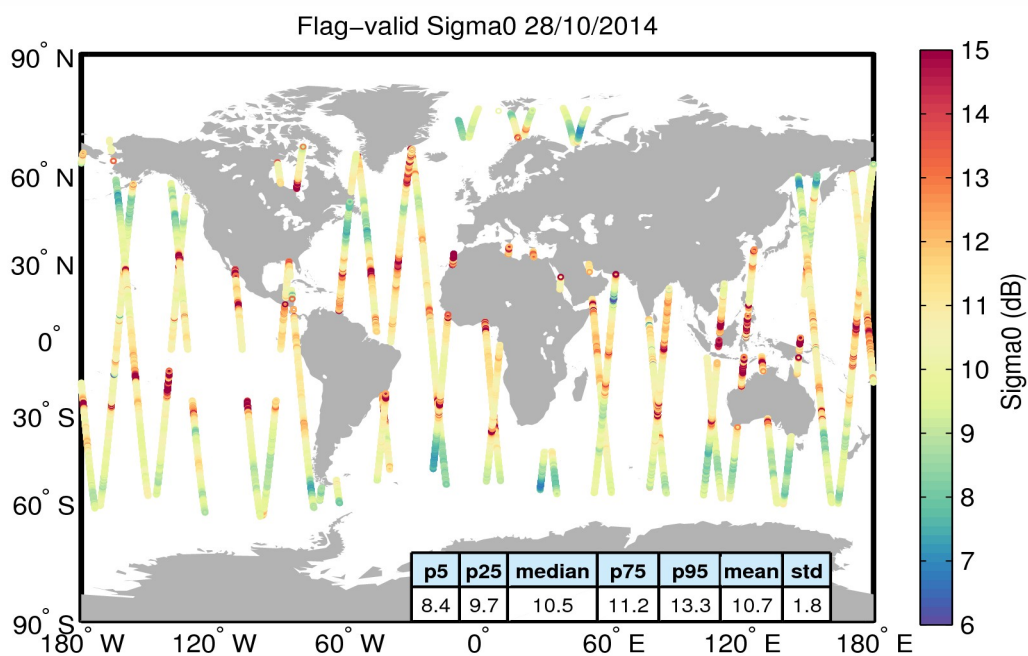
Figure 23. Geographical distribution of flag-valid sigma0 data over oceans and lakes for 28/10/2014. The statistical values shown in the table refer to the sigma0 in dB and are calculated over all measurements shown in the figure.
