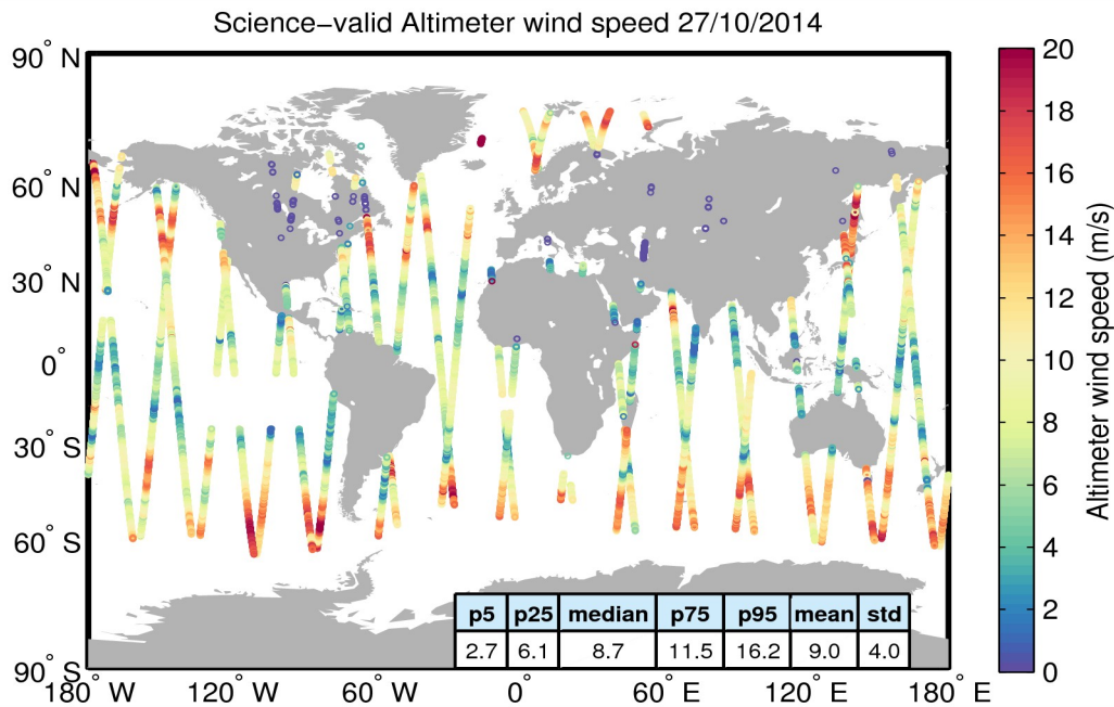
Figure 34. Geographical distribution of science-valid wind data over oceans and lakes for 27/10/2014. The statistical values shown in the table refer to the wind in m/s and are calculated over all measurements shown in the figure. Gray circles denote records that have been rejected based on the editing criteria described in Table 5.
