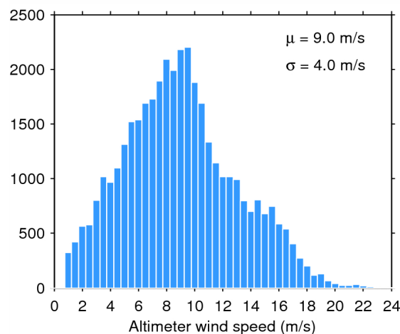
Figure 35. Histogram of science-valid wind over oceans and lakes for 27/10/2014. The mean ( \mu ) and standard deviation ( \sigma ) are also shown. Note that values larger than 24 m/s are excluded from the histogram for the sake of readability but not from the computation of \mu and \sigma .
