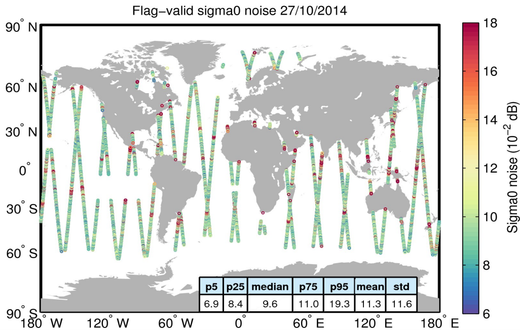
Figure 26. Geographical distribution of flag-valid 20-Hz sigma0 measurement noise over oceans and lakes for 27/10/2014. The statistical values shown in the table refer to the sigma0 noise and are calculated over all measurements shown in the figure.
