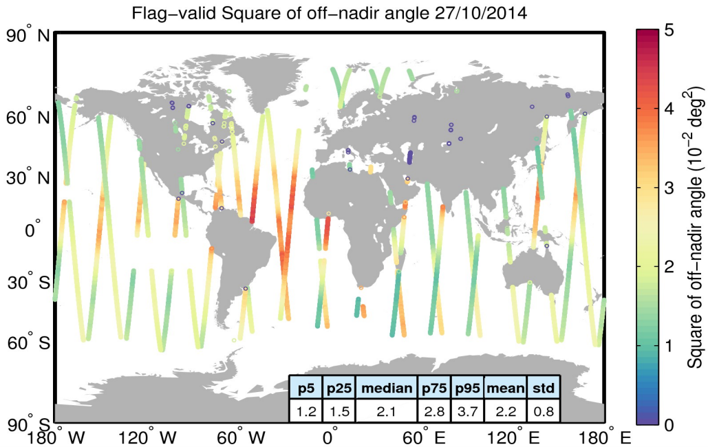
Figure 37. Geographical distribution of flag-valid mispointing data over oceans and lakes for 27/10/2014. The statistical values shown in the table refer to the mispointing in 10^{-2} \text{deg}^2 and are calculated over all measurements shown in the figure.
