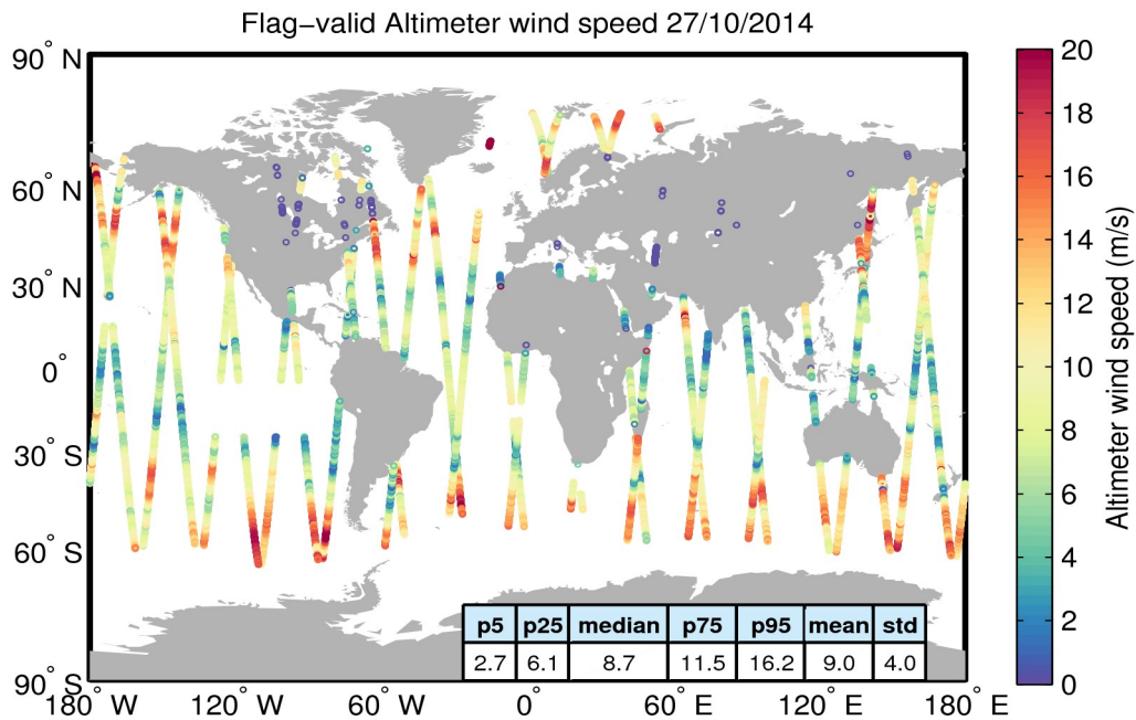
Figure 31. Geographical distribution of flag-valid wind data over oceans and lakes for 27/10/2014. The statistical values shown in the table refer to the wind in m/s and are calculated over all measurements shown in the figure.
