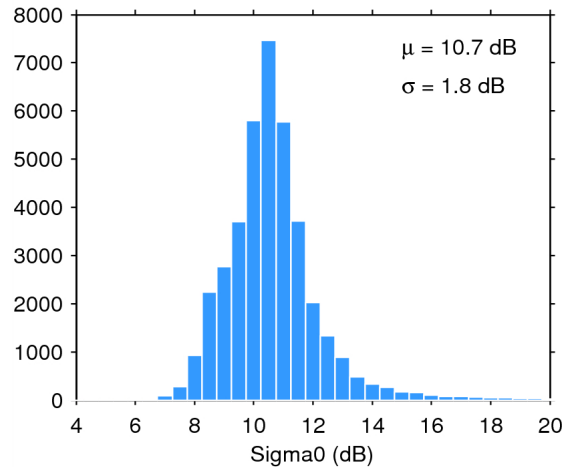
Figure 25. Histogram of flag-valid sigma0 over oceans and lakes for 27/10/2014. The mean ( \mu ) and standard deviation ( \sigma ) are also shown. Note that values outside [4 20] dB are excluded from the histogram for the sake of readability but not from the computation of \mu and \sigma .
