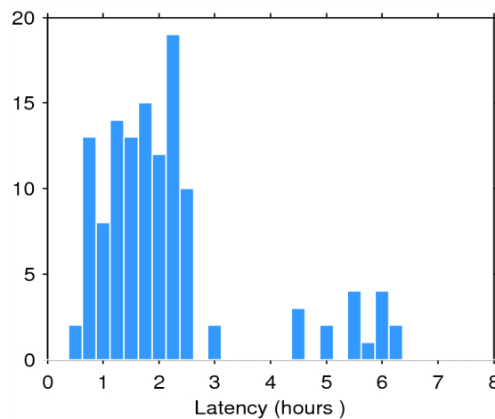
Figure 2. Histogram of the data latency for 27/10/2014. The y-axis denotes the number of files that are made available with a delay of x-hours with respect to the mean time of the records stored in the file.
