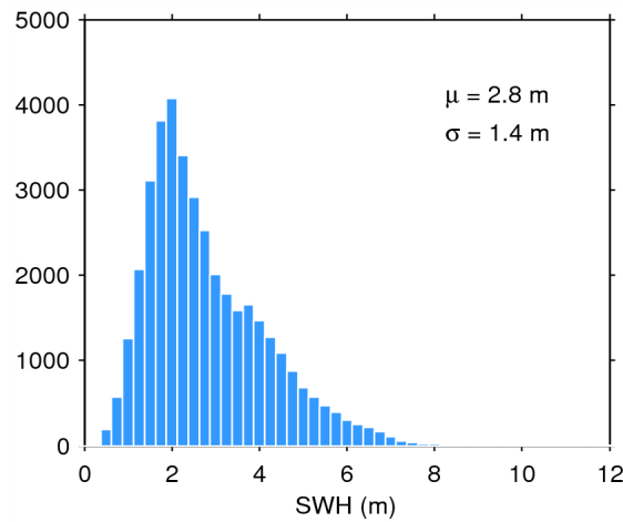
Figure 17. Histogram of flag-valid SWH over oceans and lakes for 27/10/2014. The mean ( \mu ) and standard deviation ( \sigma ) are also shown. Note that values larger than 12 m are excluded from the histogram for the sake of readability but not from the computation of \mu and \sigma .
