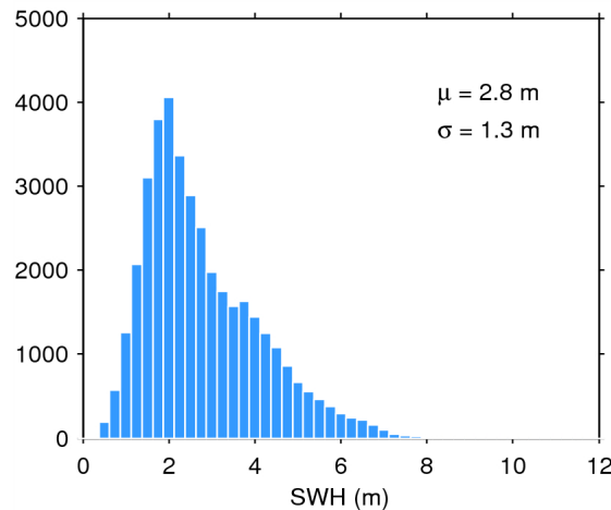
Figure 20. Histogram of science-valid SWH over oceans and lakes for 27/10/2014. The mean ( \mu ) and standard deviation ( \sigma ) are also shown. Note that values larger than 12 m are excluded from the histogram for the sake of readability but not from the computation of \mu and \sigma .
