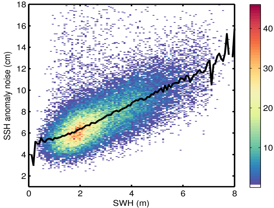
Figure 9. 2D histogram showing flag-valid SSH anomaly noise as a function of SWH for 27/10/2014. The black line denotes the median SSH anomaly as a function of SWH.
