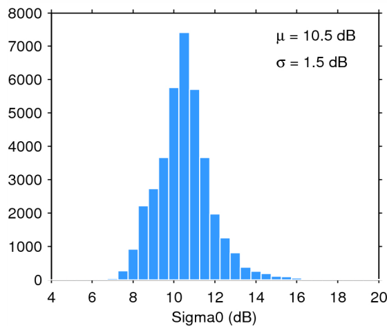
Figure 28. Histogram of science-valid sigma0 over oceans and lakes for 27/10/2014. The mean ( \mu ) and standard deviation ( \sigma ) are also shown. Note that values outside [4 20] dB are excluded from the histogram for the sake of readability but not from the computation of \mu and \sigma .
