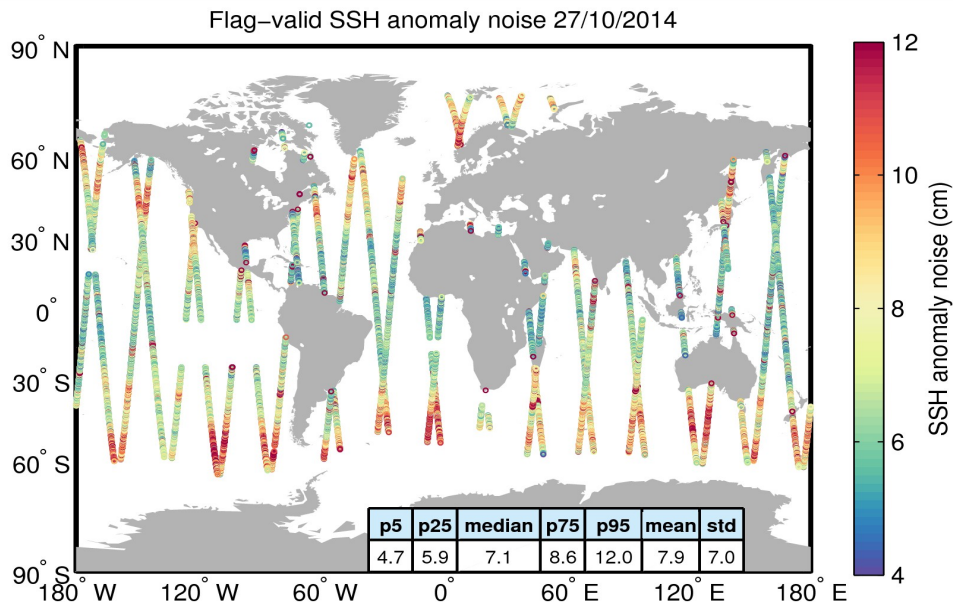
Figure 8. Geographical distribution of flag-valid 20-Hz SSH anomaly measurement noise over oceans and lakes for 27/10/2014. The statistical values shown in the table refer to the SSH anomaly noise and are calculated over all measurements shown in the figure.
