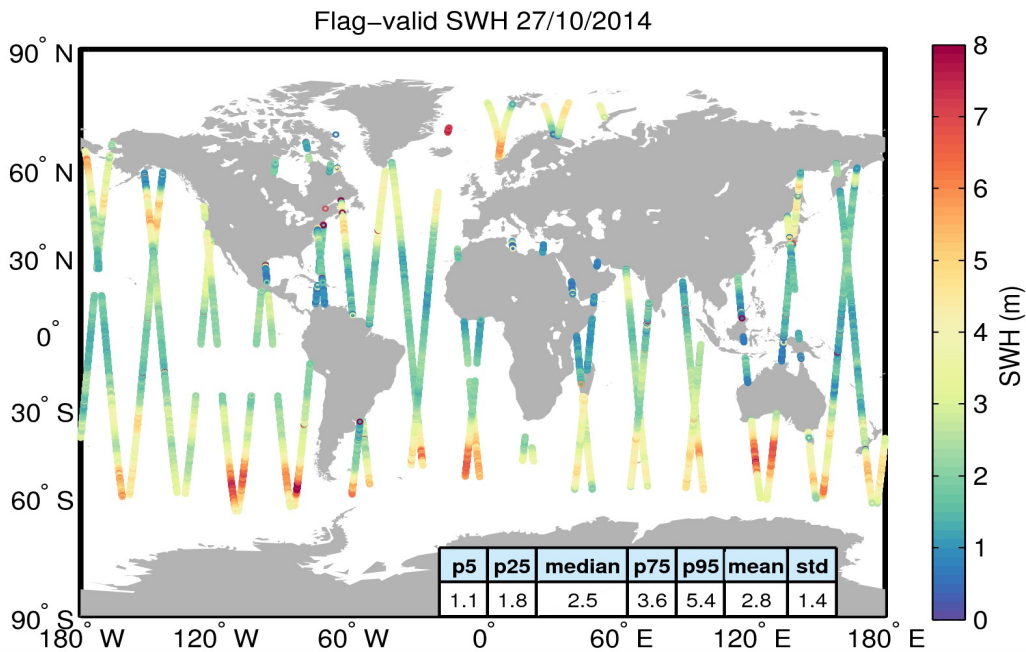
Figure 15. Geographical distribution of flag-valid SWH data over oceans and lakes for 27/10/2014. The statistical values shown in the table refer to the SWH in m and are calculated over all measurements shown in the figure.
