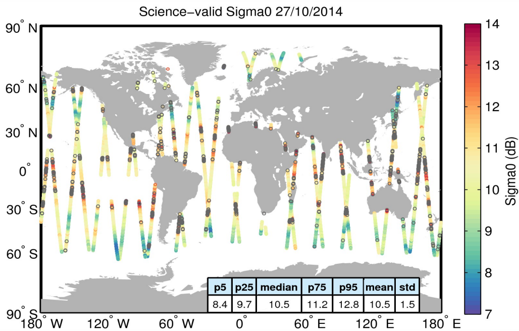
Figure 27. Geographical distribution of science-valid sigma0 data over oceans and lakes for 27/10/2014. The statistical values shown in the table refer to the sigma0 in dB and are calculated over all measurements shown in the figure. Gray circles denote records that have been rejected based on the editing criteria described in Table 4.
