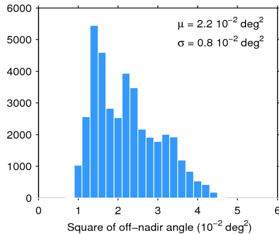
Figure 39. Histogram of flag-valid mispointing over oceans and lakes for 27/10/2014. The mean ( \mu ) and standard deviation ( \sigma ) are also shown. Note that values than 6 \cdot 10^{-2} \text{ deg}^2 are excluded from the histogram for the sake of readability but not from the computation of \mu and \sigma .
