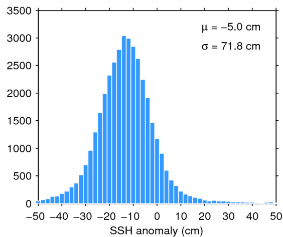
Figure 7. Histogram of flag-valid SSH anomaly over oceans and lakes for 24/10/2014. The mean ( \mu ) and standard deviation ( \sigma ) are also shown. Note that values outside [-50\ 50] cm are excluded from the histogram for the sake of readability but not from the computation of \mu and \sigma .
