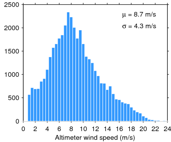
Figure 33. Histogram of flag-valid wind over oceans and lakes for 24/10/2014. The mean ( \mu ) and standard deviation ( \sigma ) are also shown. Note that values larger than 24 m/s are excluded from the histogram for the sake of readability but not from the computation of \mu and \sigma .
