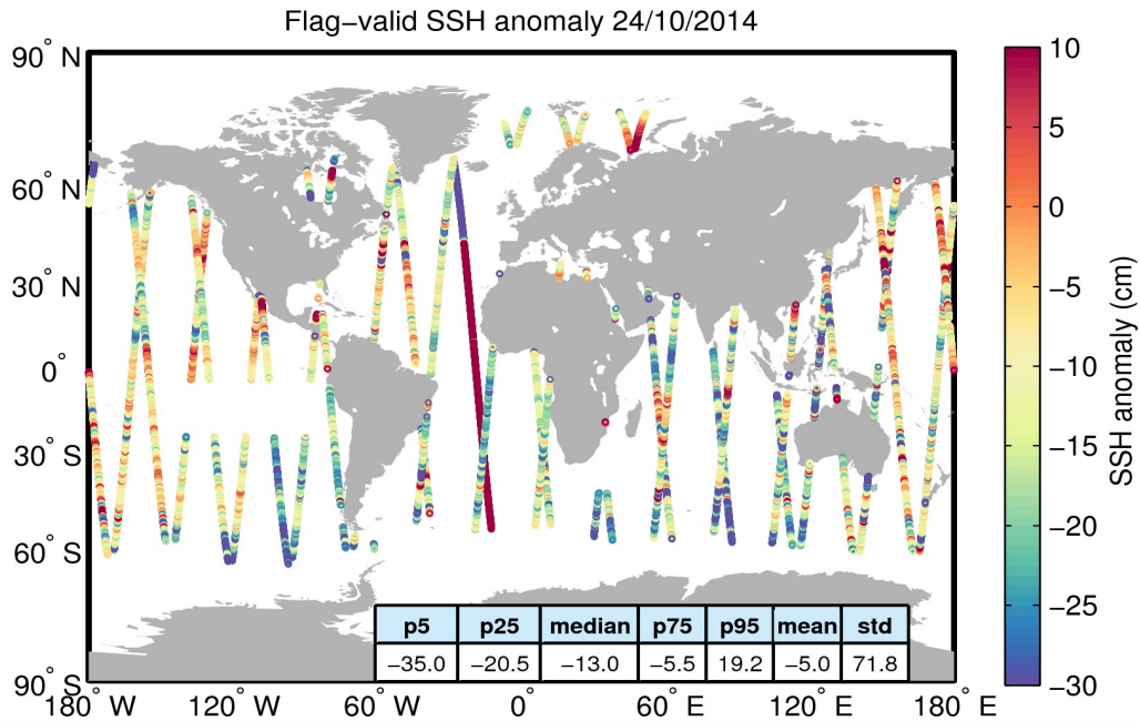
Figure 5. Geographical distribution of flag-valid 1-Hz SSH anomaly data over oceans and lakes for 24/10/2014. The statistical values shown in the table refer to the SSH anomaly in cm and are calculated over all measurements shown in the figure.
