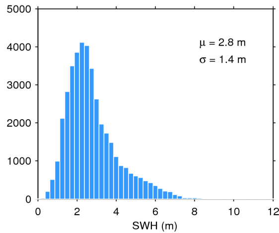
Figure 17. Histogram of flag-valid SWH over oceans and lakes for 24/10/2014. The mean ( \mu ) and standard deviation ( \sigma ) are also shown. Note that values larger than 12 m are excluded from the histogram for the sake of readability but not from the computation of \mu and \sigma .
