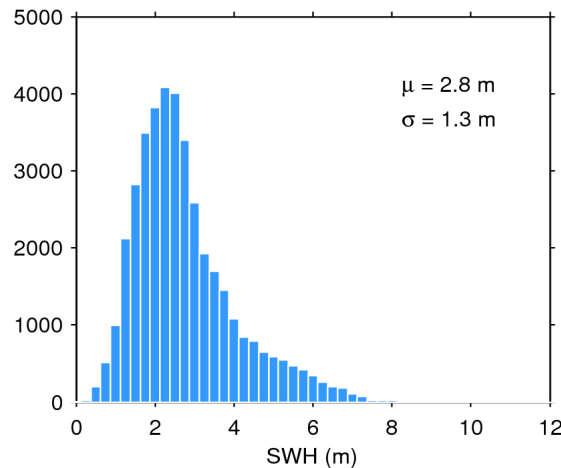
Figure 20. Histogram of science-valid SWH over oceans and lakes for 24/10/2014. The mean ( \mu ) and standard deviation ( \sigma ) are also shown. Note that values larger than 12 m are excluded from the histogram for the sake of readability but not from the computation of \mu and \sigma .
