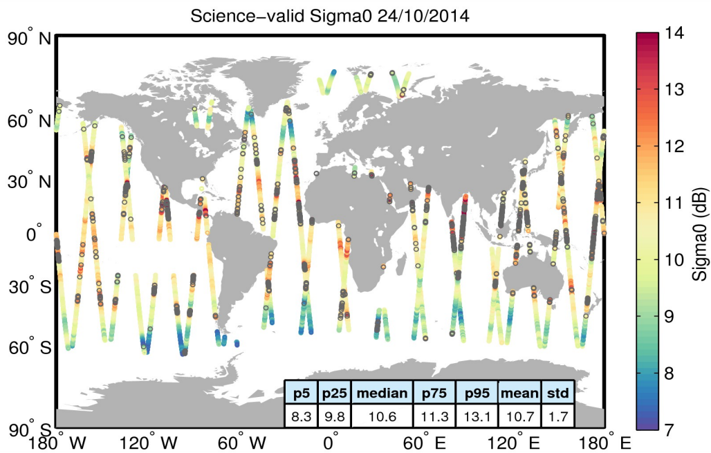
Figure 27. Geographical distribution of science-valid sigma0 data over oceans and lakes for 24/10/2014. The statistical values shown in the table refer to the sigma0 in dB and are calculated over all measurements shown in the figure. Gray circles denote records that have been rejected based on the editing criteria described in Table 4.
