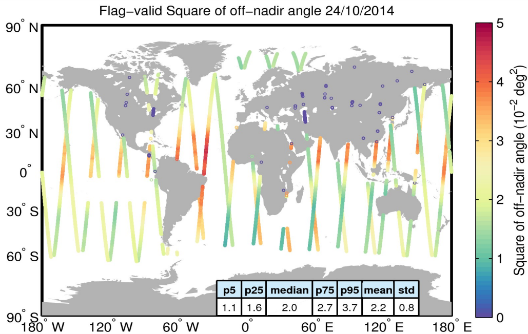
Figure 37. Geographical distribution of flag-valid mispointing data over oceans and lakes for 24/10/2014. The statistical values shown in the table refer to the mispointing in 10^{-2} \text{ deg}^2 and are calculated over all measurements shown in the figure.
