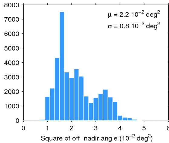
Figure 39. Histogram of flag-valid mispointing over oceans and lakes for 24/10/2014. The mean ( \mu ) and standard deviation ( \sigma ) are also shown. Note that values than 6 \cdot 10^{-2} \text{ deg}^2 are excluded from the histogram for the sake of readability but not from the computation of \mu and \sigma .
