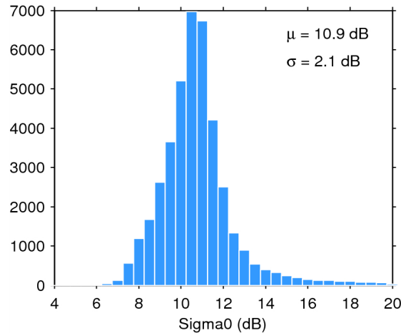
Figure 25. Histogram of flag-valid sigma0 over oceans and lakes for 24/10/2014. The mean ( \mu ) and standard deviation ( \sigma ) are also shown. Note that values outside [4 20] dB are excluded from the histogram for the sake of readability but not from the computation of \mu and \sigma .
