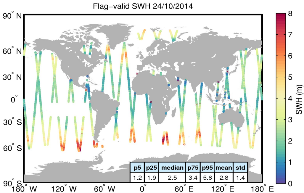
Figure 15. Geographical distribution of flag-valid SWH data over oceans and lakes for 24/10/2014. The statistical values shown in the table refer to the SWH in m and are calculated over all measurements shown in the figure.
