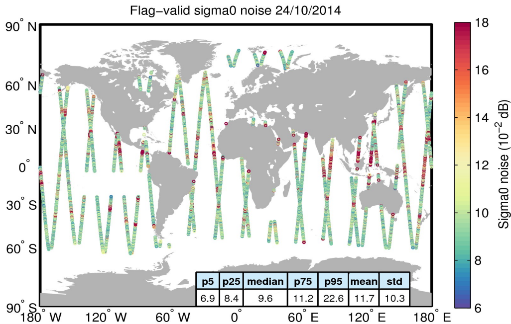
Figure 26. Geographical distribution of flag-valid 20-Hz sigma0 measurement noise over oceans and lakes for 24/10/2014. The statistical values shown in the table refer to the sigma0 noise and are calculated over all measurements shown in the figure.
