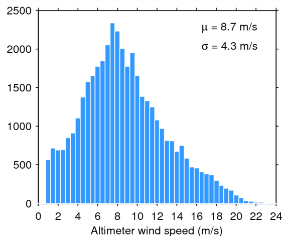
Figure 35. Histogram of science-valid wind over oceans and lakes for 24/10/2014. The mean ( \mu ) and standard deviation ( \sigma ) are also shown. Note that values larger than 24 m/s are excluded from the histogram for the sake of readability but not from the computation of \mu and \sigma .
