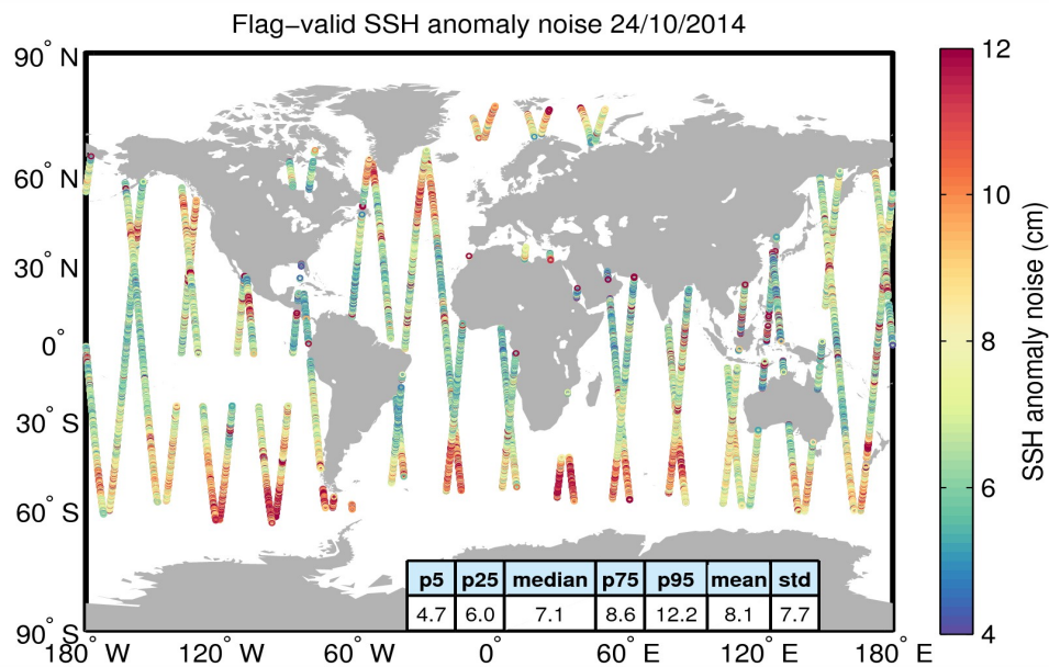
Figure 8. Geographical distribution of flag-valid 20-Hz SSH anomaly measurement noise over oceans and lakes for 24/10/2014. The statistical values shown in the table refer to the SSH anomaly noise and are calculated over all measurements shown in the figure.
