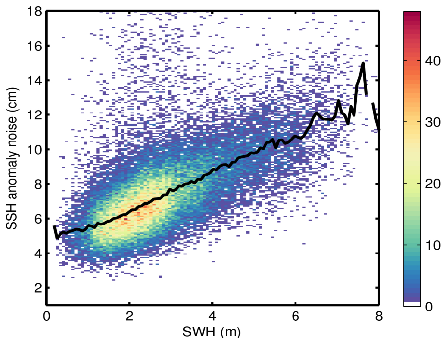
Figure 9. 2D histogram showing flag-valid SSH anomaly noise as a function of SWH for 24/10/2014. The black line denotes the median SSH anomaly as a function of SWH.
