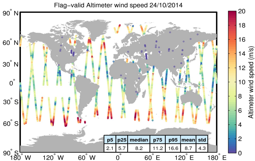
Figure 31. Geographical distribution of flag-valid wind data over oceans and lakes for 24/10/2014. The statistical values shown in the table refer to the wind in m/s and are calculated over all measurements shown in the figure.
