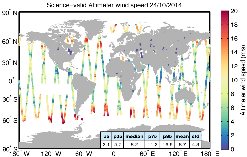
Figure 34. Geographical distribution of science-valid wind data over oceans and lakes for 24/10/2014. The statistical values shown in the table refer to the wind in m/s and are calculated over all measurements shown in the figure. Gray circles denote records that have been rejected based on the editing criteria described in Table 5.
