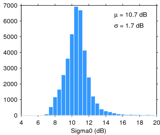
Figure 28. Histogram of science-valid sigma0 over oceans and lakes for 24/10/2014. The mean ( \mu ) and standard deviation ( \sigma ) are also shown. Note that values outside [4 20] dB are excluded from the histogram for the sake of readability but not from the computation of \mu and \sigma .
