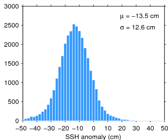
Figure 11. Histogram of science-valid SSH anomaly over oceans and lakes for 24/10/2014. The mean ( \mu ) and standard deviation ( \sigma ) are also shown. Note that values outside [-50 50] cm are excluded from the histogram for the sake of readability but not from the computation of \mu and \sigma .
