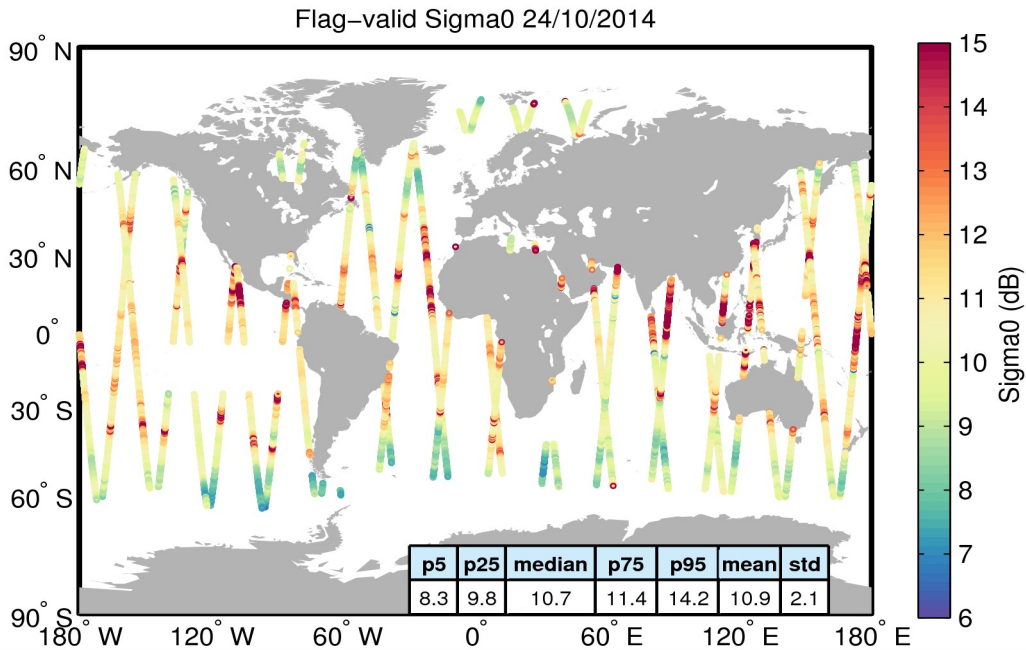
Figure 23. Geographical distribution of flag-valid sigma0 data over oceans and lakes for 24/10/2014. The statistical values shown in the table refer to the sigma0 in dB and are calculated over all measurements shown in the figure.
