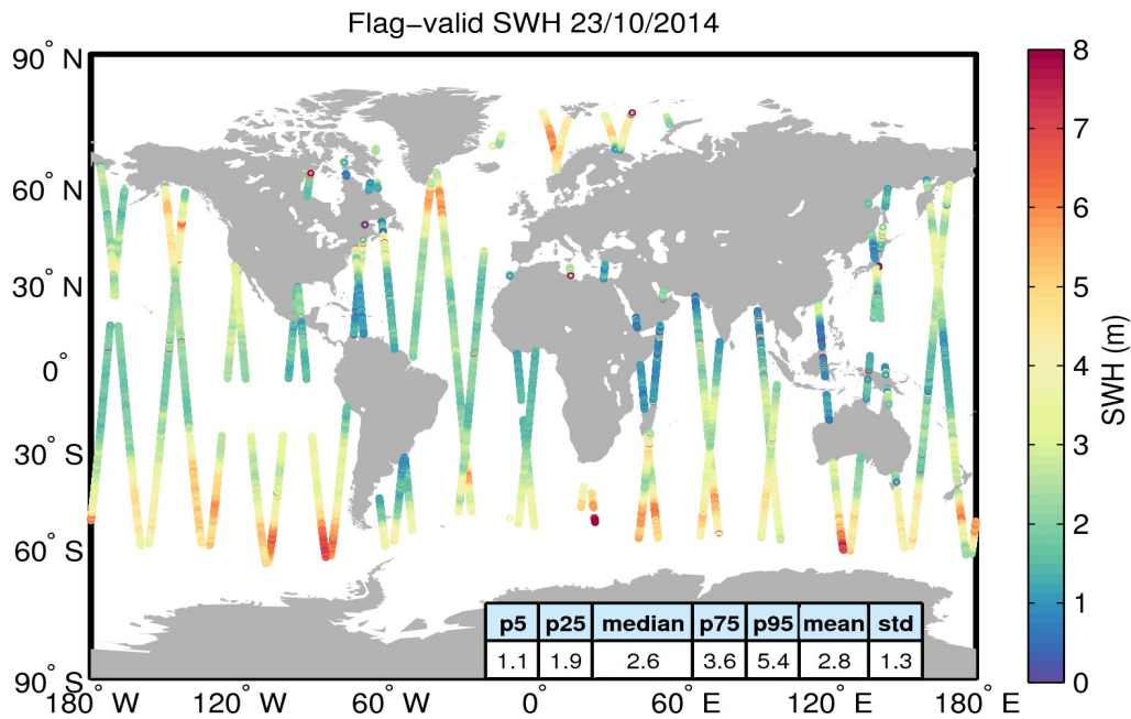
Figure 15. Geographical distribution of flag-valid SWH data over oceans and lakes for 23/10/2014. The statistical values shown in the table refer to the SWH in m and are calculated over all measurements shown in the figure.
