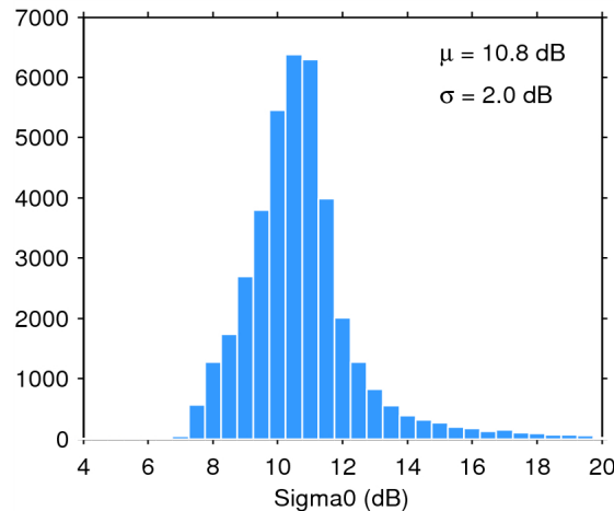
Figure 25. Histogram of flag-valid sigma0 over oceans and lakes for 23/10/2014. The mean ( \mu ) and standard deviation ( \sigma ) are also shown. Note that values outside [4 20] dB are excluded from the histogram for the sake of readability but not from the computation of \mu and \sigma .
