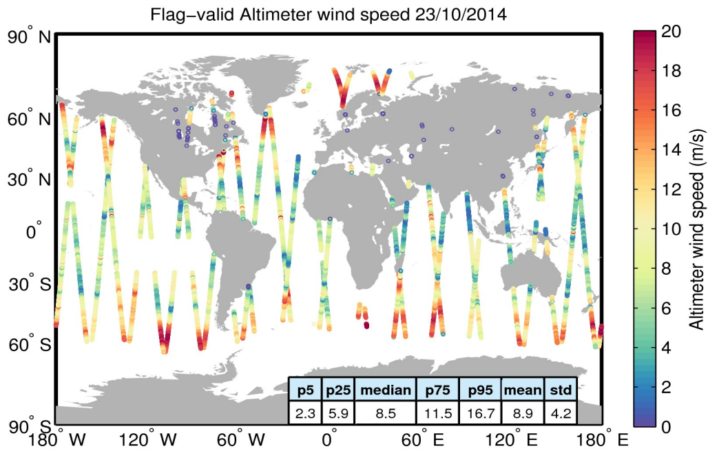
Figure 31. Geographical distribution of flag-valid wind data over oceans and lakes for 23/10/2014. The statistical values shown in the table refer to the wind in m/s and are calculated over all measurements shown in the figure.
