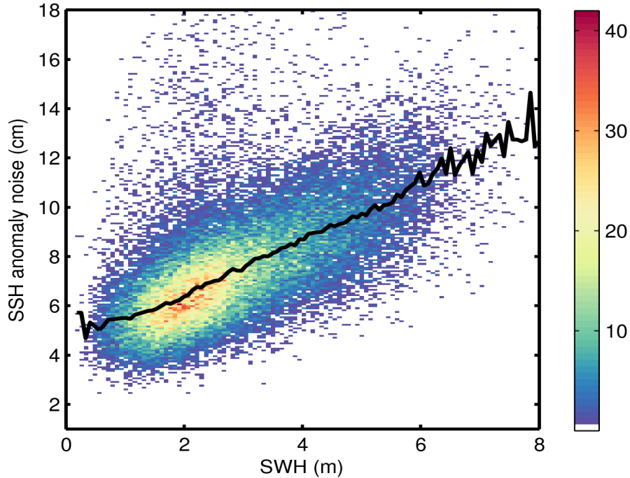
Figure 9. 2D histogram showing flag-valid SSH anomaly noise as a function of SWH for 23/10/2014. The black line denotes the median SSH anomaly as a function of SWH.
