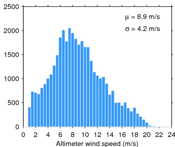
Figure 35. Histogram of science-valid wind over oceans and lakes for 23/10/2014. The mean ( \mu ) and standard deviation ( \sigma ) are also shown. Note that values larger than 24 m/s are excluded from the histogram for the sake of readability but not from the computation of \mu and \sigma .
