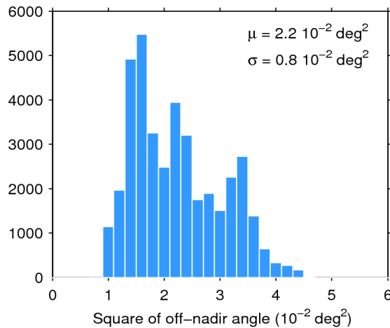
Figure 39. Histogram of flag-valid mispointing over oceans and lakes for 23/10/2014. The mean ( \mu ) and standard deviation ( \sigma ) are also shown. Note that values than 6 \cdot 10^{-2} \text{ deg}^2 are excluded from the histogram for the sake of readability but not from the computation of \mu and \sigma .
