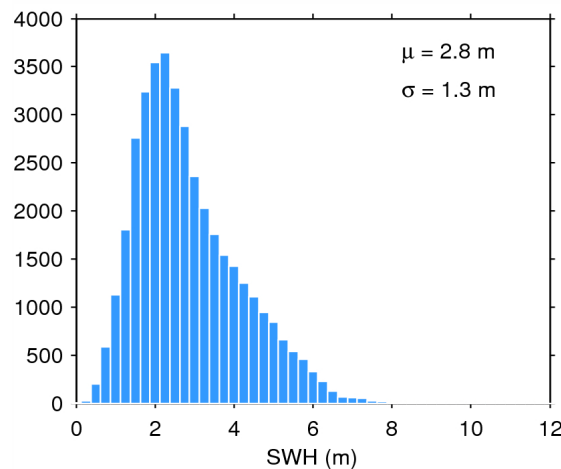
Figure 17. Histogram of flag-valid SWH over oceans and lakes for 23/10/2014. The mean ( \mu ) and standard deviation ( \sigma ) are also shown. Note that values larger than 12 m are excluded from the histogram for the sake of readability but not from the computation of \mu and \sigma .
