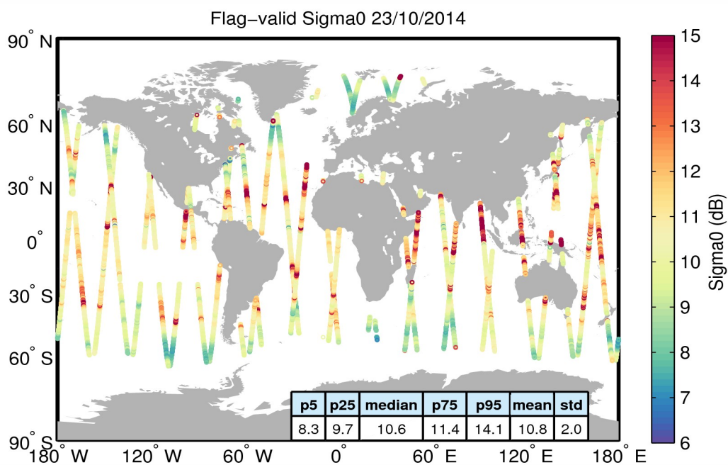
Figure 23. Geographical distribution of flag-valid sigma0 data over oceans and lakes for 23/10/2014. The statistical values shown in the table refer to the sigma0 in dB and are calculated over all measurements shown in the figure.
