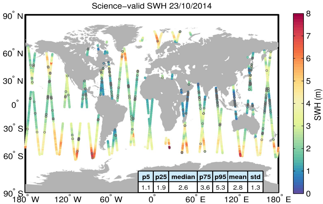
Figure 19. Geographical distribution of science-valid SWH data over oceans and lakes for 23/10/2014. The statistical values shown in the table refer to the SWH in m and are calculated over all measurements shown in the figure. Gray circles denote records that have been rejected based on the editing criteria described in Table 3.
