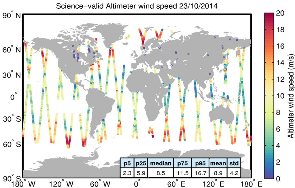
Figure 34. Geographical distribution of science-valid wind data over oceans and lakes for 23/10/2014. The statistical values shown in the table refer to the wind in m/s and are calculated over all measurements shown in the figure. Gray circles denote records that have been rejected based on the editing criteria described in Table 5.
