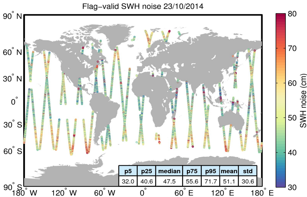
Figure 18. Geographical distribution of flag-valid 20-Hz SWH measurement noise over oceans and lakes for 23/10/2014. The statistical values shown in the figure refer to the SWH noise and are calculated over all measurements shown in the figure.
