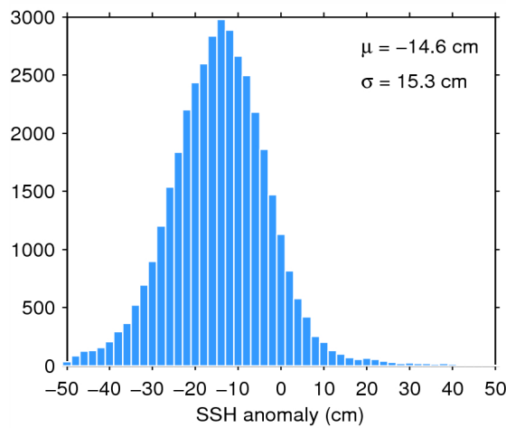
Figure 7. Histogram of flag-valid SSH anomaly over oceans and lakes for 23/10/2014. The mean ( \mu ) and standard deviation ( \sigma ) are also shown. Note that values outside [-50\ 50] cm are excluded from the histogram for the sake of readability but not from the computation of \mu and \sigma .
