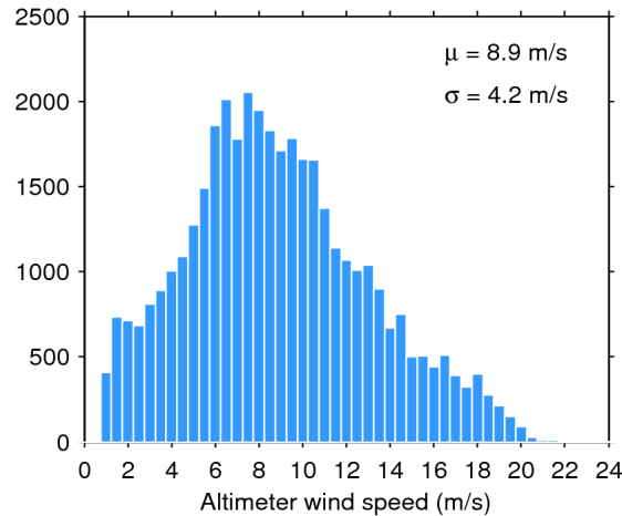
Figure 33. Histogram of flag-valid wind over oceans and lakes for 23/10/2014. The mean ( \mu ) and standard deviation ( \sigma ) are also shown. Note that values larger than 24 m/s are excluded from the histogram for the sake of readability but not from the computation of \mu and \sigma .
