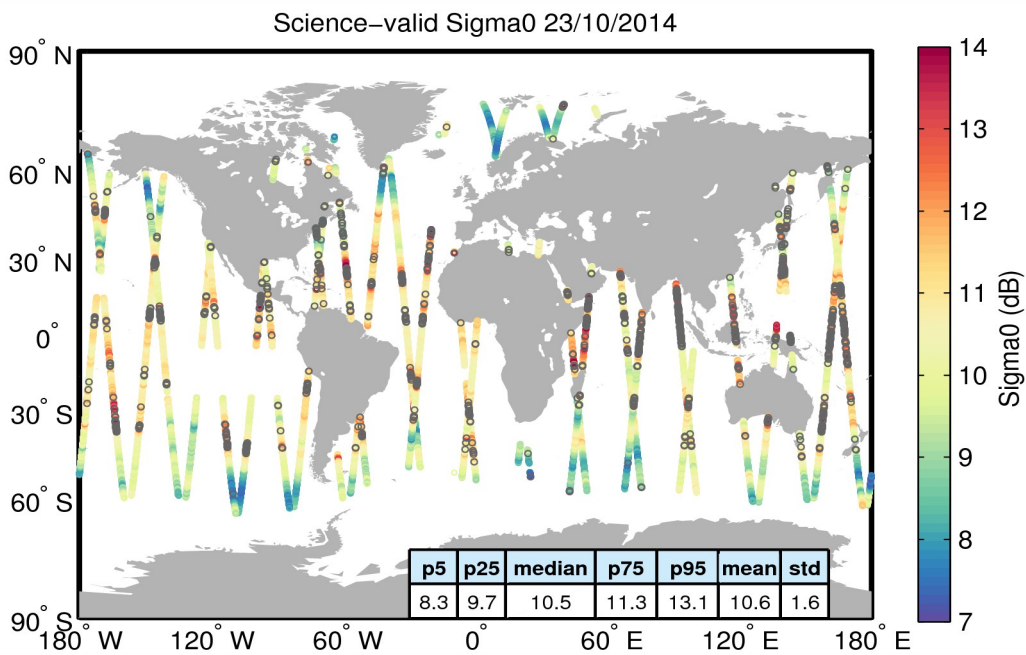
Figure 27. Geographical distribution of science-valid sigma0 data over oceans and lakes for 23/10/2014. The statistical values shown in the table refer to the sigma0 in dB and are calculated over all measurements shown in the figure. Gray circles denote records that have been rejected based on the editing criteria described in Table 4.
