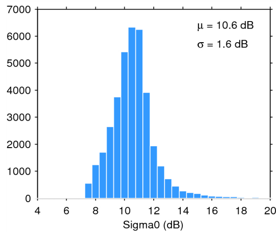
Figure 28. Histogram of science-valid sigma0 over oceans and lakes for 23/10/2014. The mean ( \mu ) and standard deviation ( \sigma ) are also shown. Note that values outside [4 20] dB are excluded from the histogram for the sake of readability but not from the computation of \mu and \sigma .
