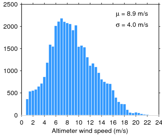
Figure 33. Histogram of flag-valid wind over oceans and lakes for 22/10/2014. The mean ( \mu ) and standard deviation ( \sigma ) are also shown. Note that values larger than 24 m/s are excluded from the histogram for the sake of readability but not from the computation of \mu and \sigma .
