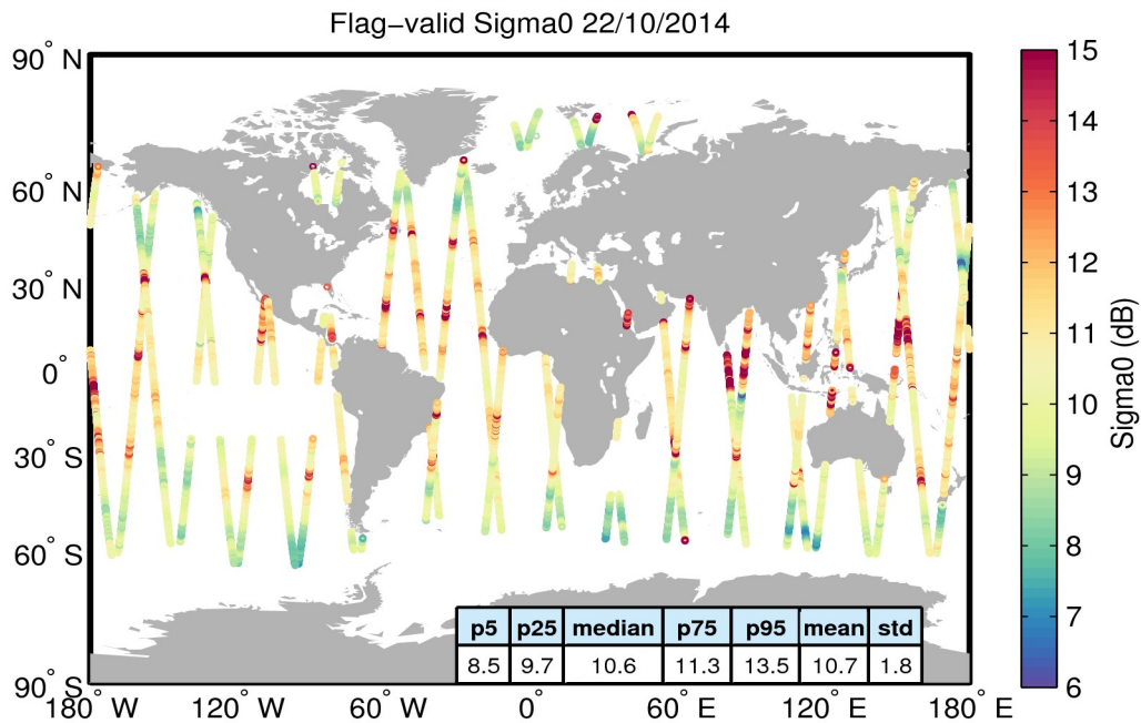
Figure 23. Geographical distribution of flag-valid sigma0 data over oceans and lakes for 22/10/2014. The statistical values shown in the table refer to the sigma0 in dB and are calculated over all measurements shown in the figure.
