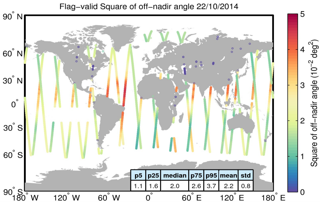
Figure 37. Geographical distribution of flag-valid mispointing data over oceans and lakes for 22/10/2014. The statistical values shown in the table refer to the mispointing in 10^{-2} \text{ deg}^2 and are calculated over all measurements shown in the figure.
