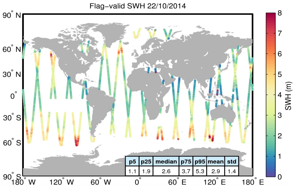
Figure 15. Geographical distribution of flag-valid SWH data over oceans and lakes for 22/10/2014. The statistical values shown in the table refer to the SWH in m and are calculated over all measurements shown in the figure.
