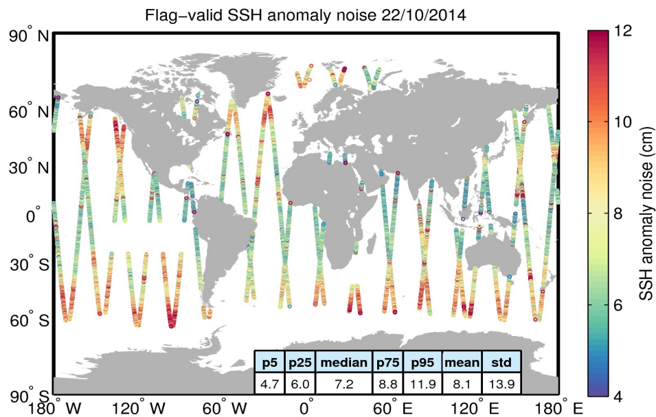
Figure 8. Geographical distribution of flag-valid 20-Hz SSH anomaly measurement noise over oceans and lakes for 22/10/2014. The statistical values shown in the table refer to the SSH anomaly noise and are calculated over all measurements shown in the figure.
