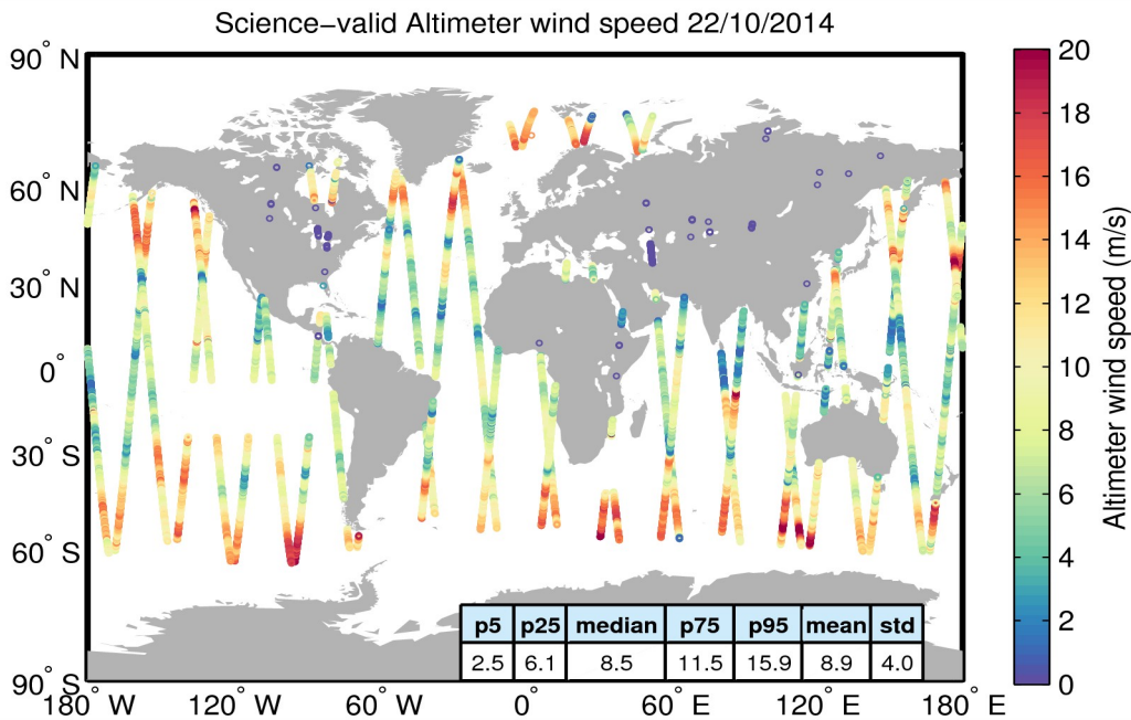
Figure 34. Geographical distribution of science-valid wind data over oceans and lakes for 22/10/2014. The statistical values shown in the table refer to the wind in m/s and are calculated over all measurements shown in the figure. Gray circles denote records that have been rejected based on the editing criteria described in Table 5.
