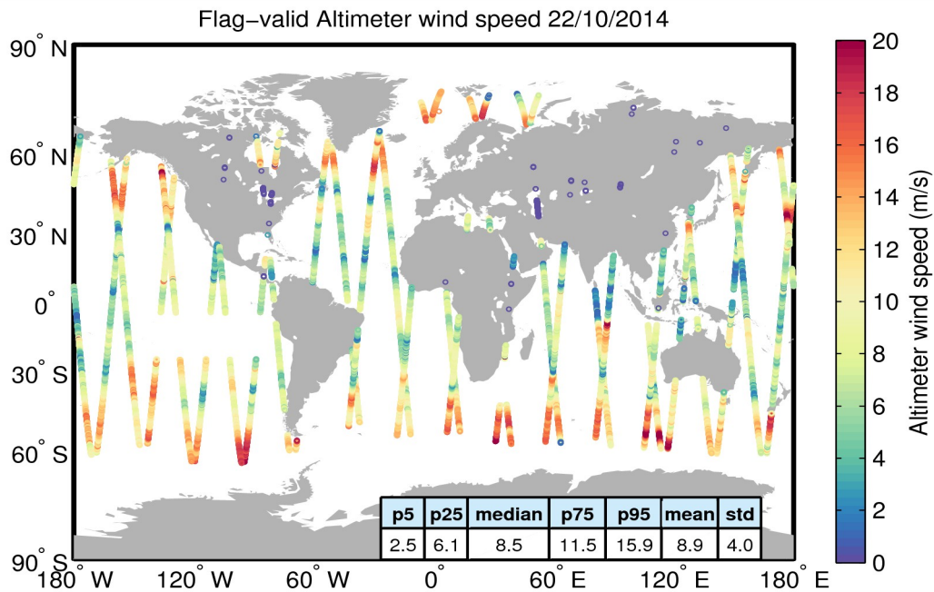
Figure 31. Geographical distribution of flag-valid wind data over oceans and lakes for 22/10/2014. The statistical values shown in the table refer to the wind in m/s and are calculated over all measurements shown in the figure.
