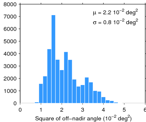
Figure 39. Histogram of flag-valid mispointing over oceans and lakes for 22/10/2014. The mean ( \mu ) and standard deviation ( \sigma ) are also shown. Note that values than 6 \cdot 10^{-2} \text{ deg}^2 are excluded from the histogram for the sake of readability but not from the computation of \mu and \sigma .
