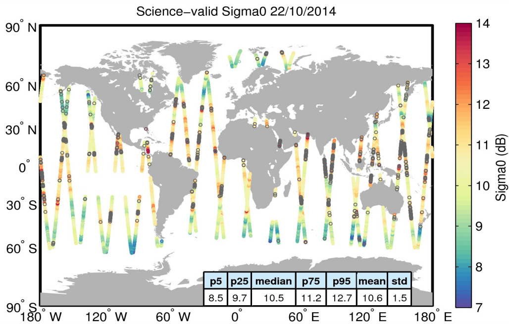
Figure 27. Geographical distribution of science-valid sigma0 data over oceans and lakes for 22/10/2014. The statistical values shown in the table refer to the sigma0 in dB and are calculated over all measurements shown in the figure. Gray circles denote records that have been rejected based on the editing criteria described in Table 4.
