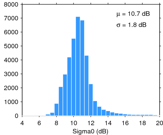
Figure 25. Histogram of flag-valid sigma0 over oceans and lakes for 22/10/2014. The mean ( \mu ) and standard deviation ( \sigma ) are also shown. Note that values outside [4 20] dB are excluded from the histogram for the sake of readability but not from the computation of \mu and \sigma .
