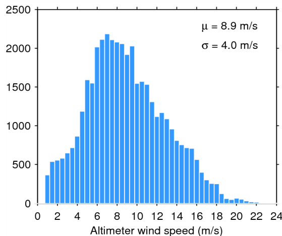
Figure 35. Histogram of science-valid wind over oceans and lakes for 22/10/2014. The mean ( \mu ) and standard deviation ( \sigma ) are also shown. Note that values larger than 24 m/s are excluded from the histogram for the sake of readability but not from the computation of \mu and \sigma .
