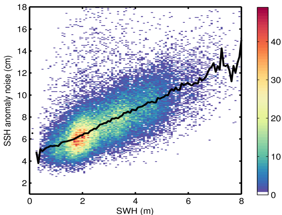
Figure 9. 2D histogram showing flag-valid SSH anomaly noise as a function of SWH for 22/10/2014. The black line denotes the median SSH anomaly as a function of SWH.
