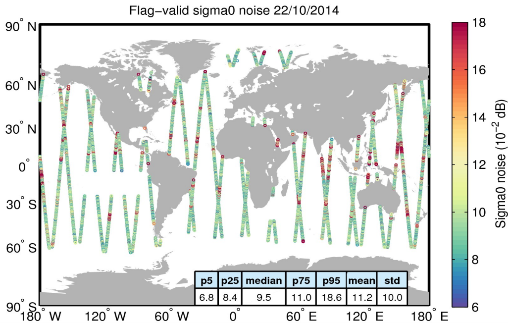
Figure 26. Geographical distribution of flag-valid 20-Hz sigma0 measurement noise over oceans and lakes for 22/10/2014. The statistical values shown in the table refer to the sigma0 noise and are calculated over all measurements shown in the figure.
