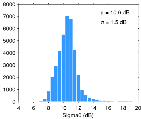
Figure 28. Histogram of science-valid sigma0 over oceans and lakes for 22/10/2014. The mean ( \mu ) and standard deviation ( \sigma ) are also shown. Note that values outside [4 20] dB are excluded from the histogram for the sake of readability but not from the computation of \mu and \sigma .
