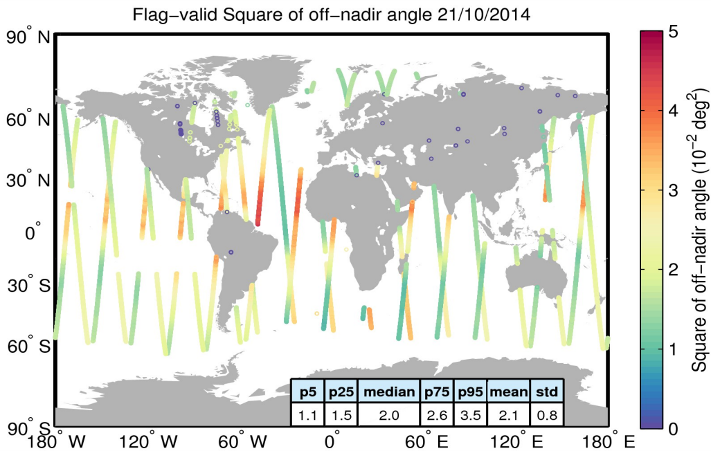
Figure 37. Geographical distribution of flag-valid mispointing data over oceans and lakes for 21/10/2014. The statistical values shown in the table refer to the mispointing in 10^{-2} \text{ deg}^2 and are calculated over all measurements shown in the figure.
