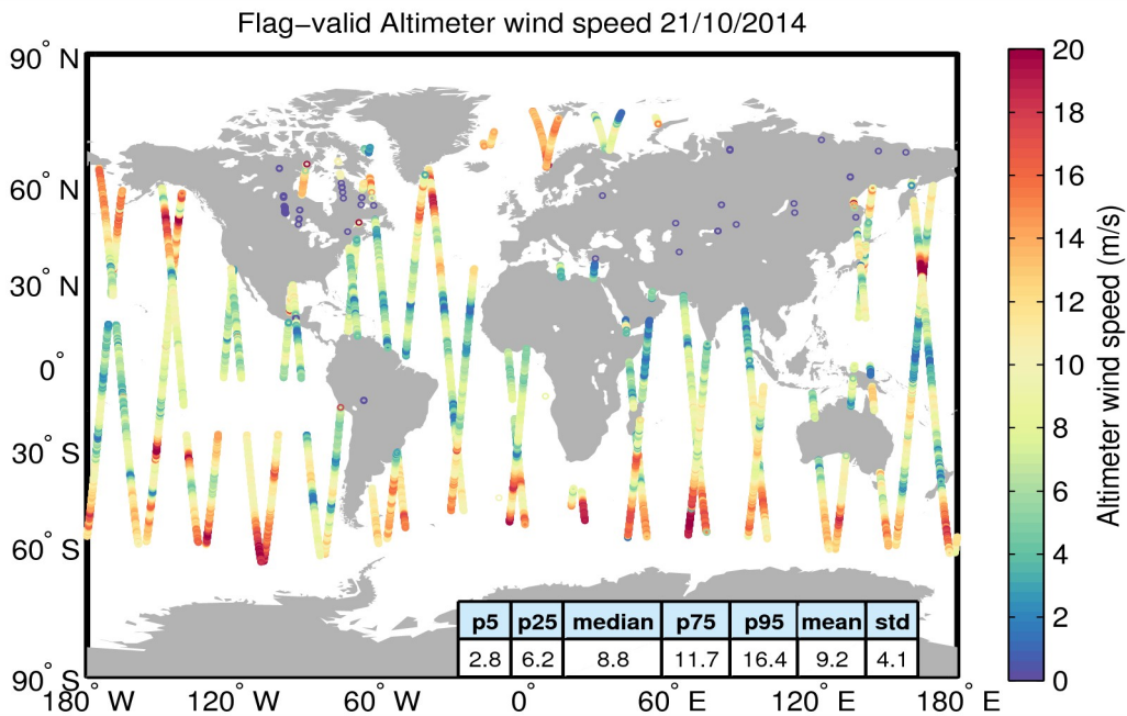
Figure 31. Geographical distribution of flag-valid wind data over oceans and lakes for 21/10/2014. The statistical values shown in the table refer to the wind in m/s and are calculated over all measurements shown in the figure.
