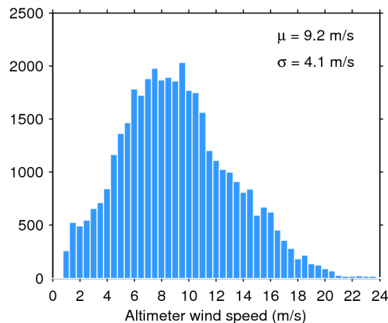
Figure 35. Histogram of science-valid wind over oceans and lakes for 21/10/2014. The mean ( \mu ) and standard deviation ( \sigma ) are also shown. Note that values larger than 24 m/s are excluded from the histogram for the sake of readability but not from the computation of \mu and \sigma .
