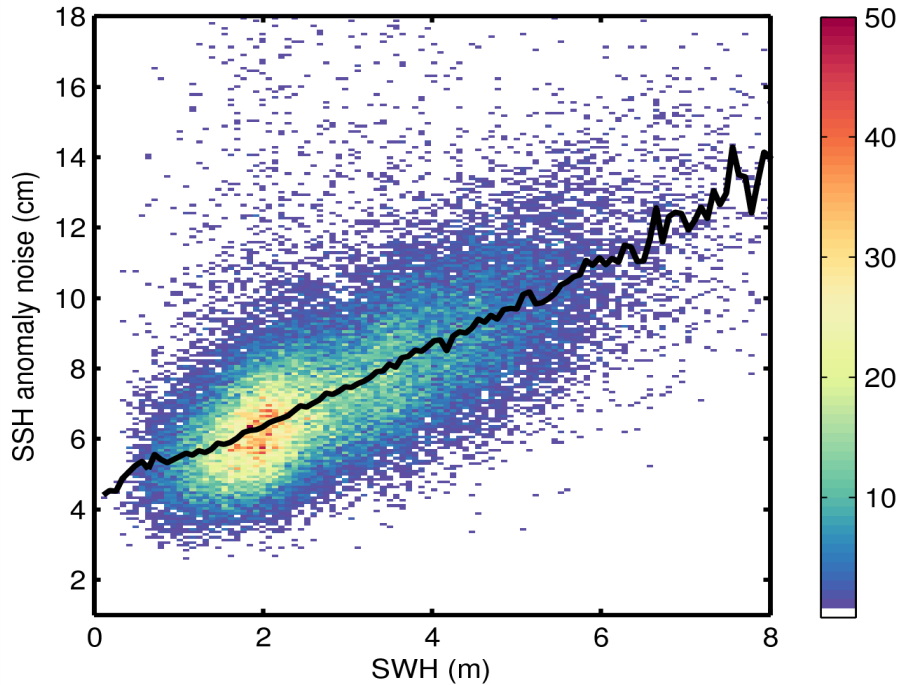
Figure 9. 2D histogram showing flag-valid SSH anomaly noise as a function of SWH for 21/10/2014. The black line denotes the median SSH anomaly as a function of SWH.
