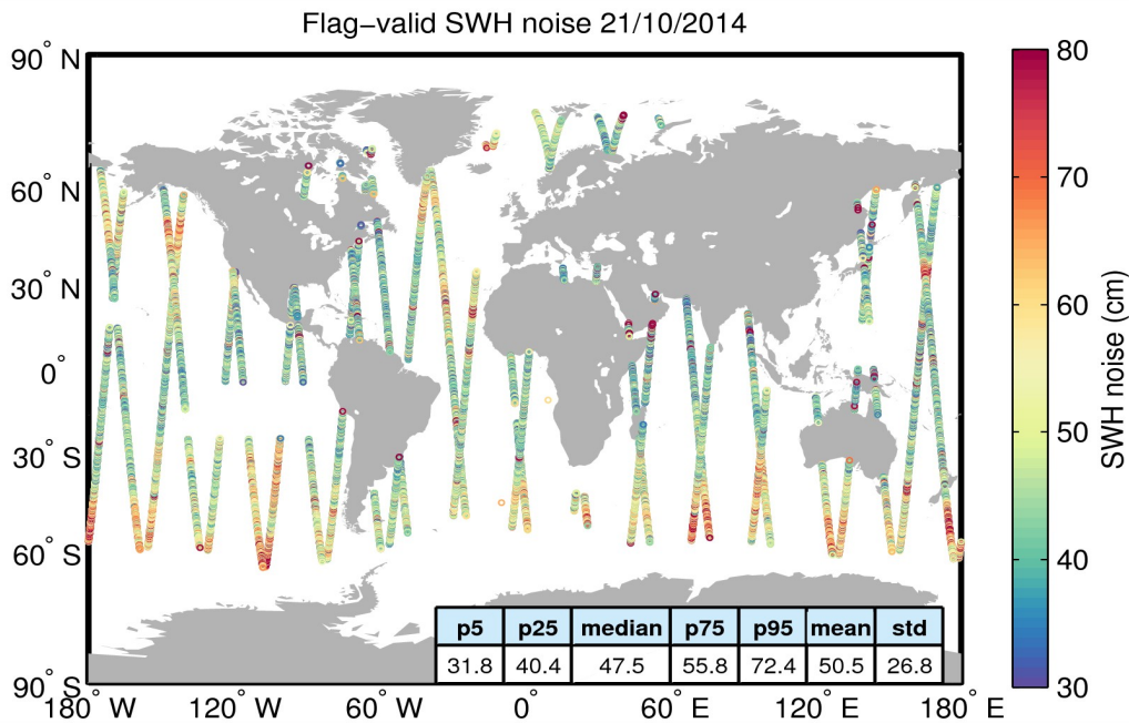
Figure 18. Geographical distribution of flag-valid 20-Hz SWH measurement noise over oceans and lakes for 21/10/2014. The statistical values shown in the figure refer to the SWH noise and are calculated over all measurements shown in the figure.
