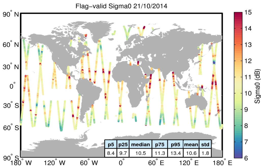
Figure 23. Geographical distribution of flag-valid sigma0 data over oceans and lakes for 21/10/2014. The statistical values shown in the table refer to the sigma0 in dB and are calculated over all measurements shown in the figure.
