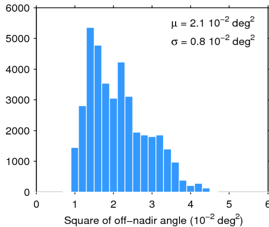
Figure 39. Histogram of flag-valid mispointing over oceans and lakes for 21/10/2014. The mean ( \mu ) and standard deviation ( \sigma ) are also shown. Note that values than 6 \cdot 10^{-2} \text{ deg}^2 are excluded from the histogram for the sake of readability but not from the computation of \mu and \sigma .
