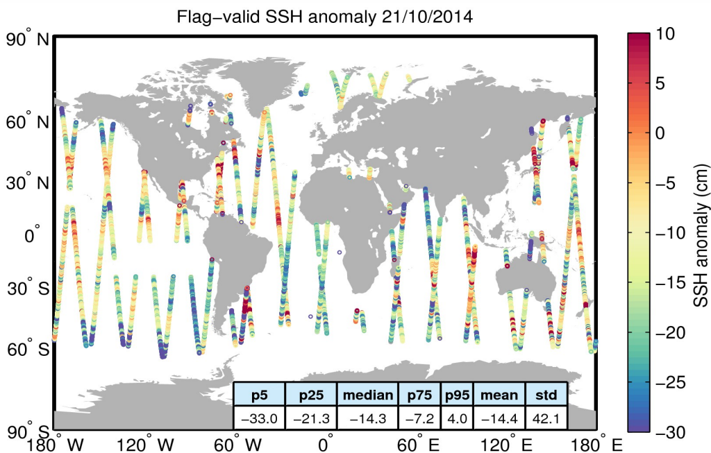
Figure 5. Geographical distribution of flag-valid 1-Hz SSH anomaly data over oceans and lakes for 21/10/2014. The statistical values shown in the table refer to the SSH anomaly in cm and are calculated over all measurements shown in the figure.
