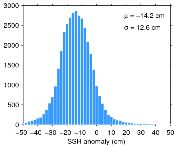
Figure 11. Histogram of science-valid SSH anomaly over oceans and lakes for 21/10/2014. The mean ( \mu ) and standard deviation ( \sigma ) are also shown. Note that values outside [-50 50] cm are excluded from the histogram for the sake of readability but not from the computation of \mu and \sigma .
