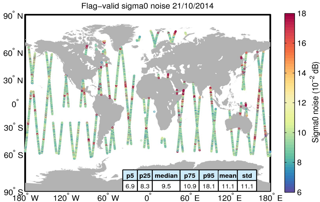
Figure 26. Geographical distribution of flag-valid 20-Hz sigma0 measurement noise over oceans and lakes for 21/10/2014. The statistical values shown in the table refer to the sigma0 noise and are calculated over all measurements shown in the figure.
