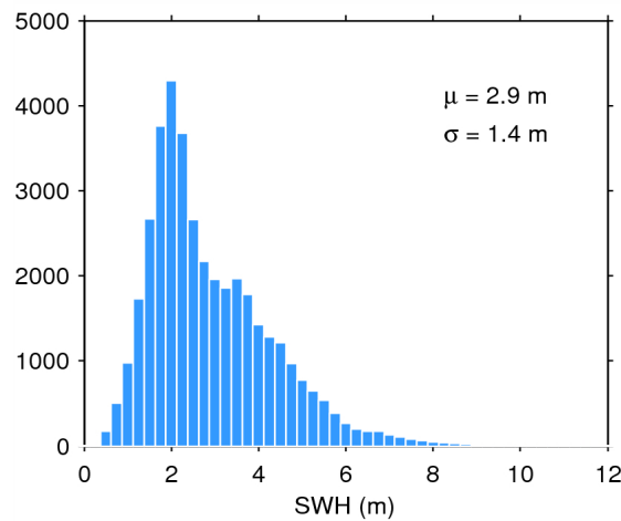
Figure 17. Histogram of flag-valid SWH over oceans and lakes for 21/10/2014. The mean ( \mu ) and standard deviation ( \sigma ) are also shown. Note that values larger than 12 m are excluded from the histogram for the sake of readability but not from the computation of \mu and \sigma .
