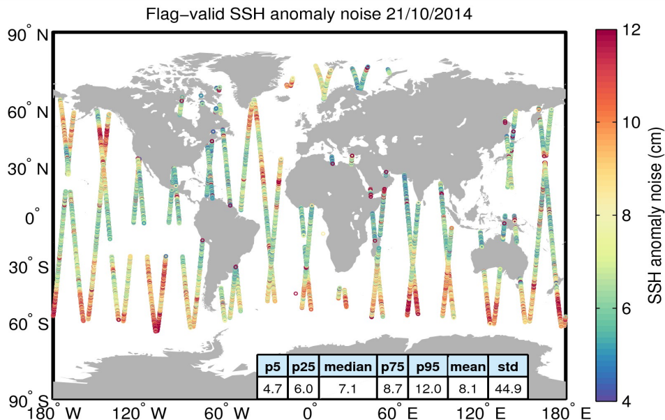
Figure 8. Geographical distribution of flag-valid 20-Hz SSH anomaly measurement noise over oceans and lakes for 21/10/2014. The statistical values shown in the table refer to the SSH anomaly noise and are calculated over all measurements shown in the figure.
