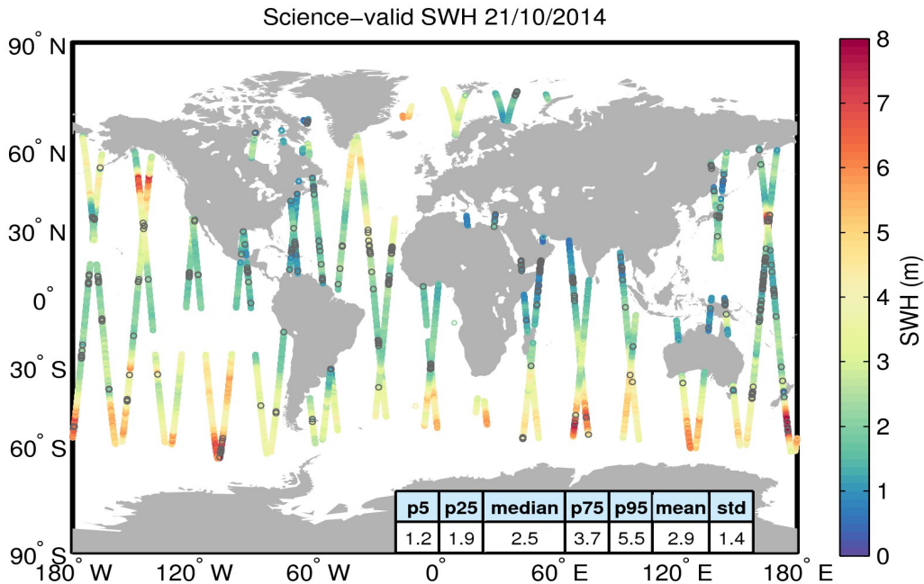
Figure 19. Geographical distribution of science-valid SWH data over oceans and lakes for 21/10/2014. The statistical values shown in the table refer to the SWH in m and are calculated over all measurements shown in the figure. Gray circles denote records that have been rejected based on the editing criteria described in Table 3.
