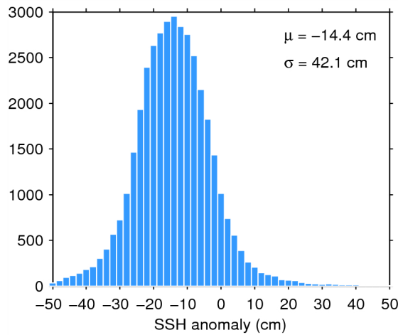
Figure 7. Histogram of flag-valid SSH anomaly over oceans and lakes for 21/10/2014. The mean ( \mu ) and standard deviation ( \sigma ) are also shown. Note that values outside [-50\ 50] cm are excluded from the histogram for the sake of readability but not from the computation of \mu and \sigma .
