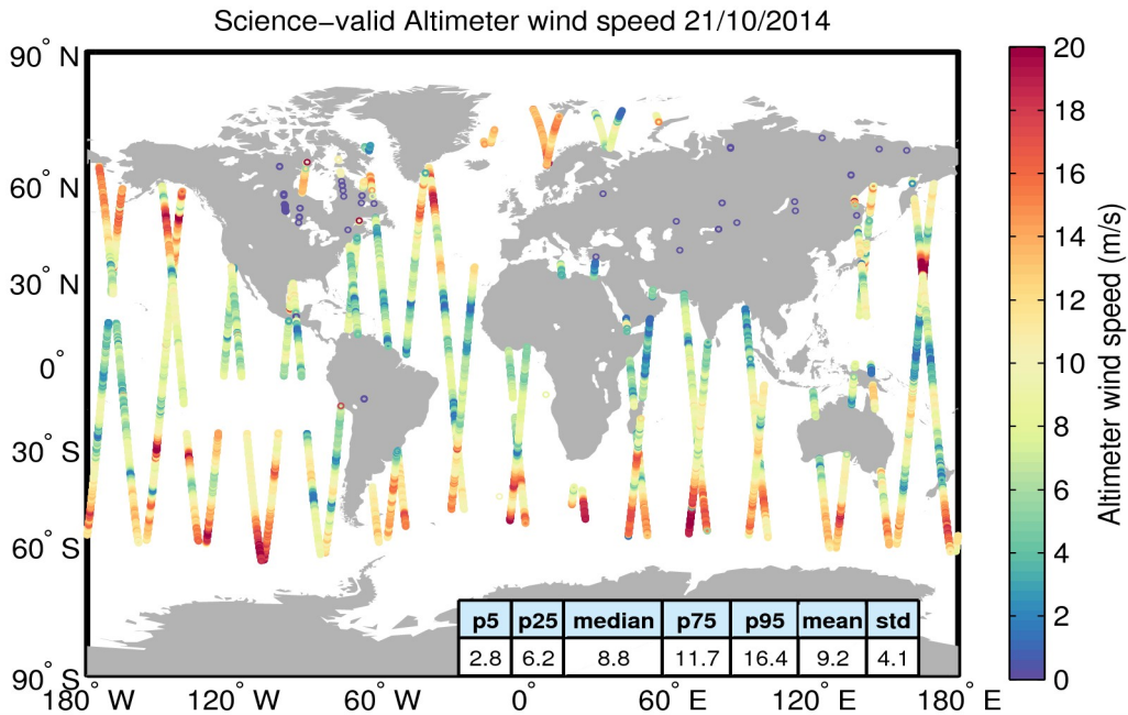
Figure 34. Geographical distribution of science-valid wind data over oceans and lakes for 21/10/2014. The statistical values shown in the table refer to the wind in m/s and are calculated over all measurements shown in the figure. Gray circles denote records that have been rejected based on the editing criteria described in Table 5.
