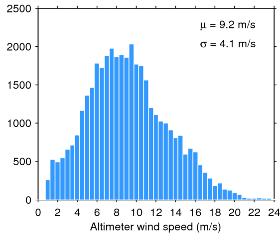
Figure 33. Histogram of flag-valid wind over oceans and lakes for 21/10/2014. The mean ( \mu ) and standard deviation ( \sigma ) are also shown. Note that values larger than 24 m/s are excluded from the histogram for the sake of readability but not from the computation of \mu and \sigma .
