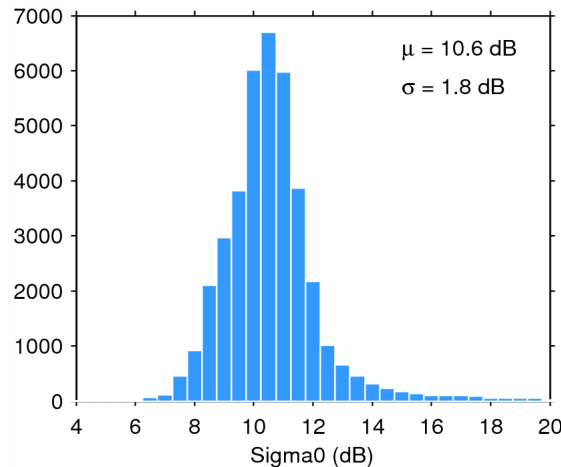
Figure 25. Histogram of flag-valid sigma0 over oceans and lakes for 21/10/2014. The mean ( \mu ) and standard deviation ( \sigma ) are also shown. Note that values outside [4 20] dB are excluded from the histogram for the sake of readability but not from the computation of \mu and \sigma .
