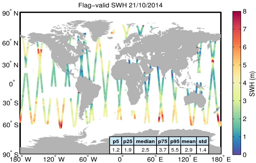
Figure 15. Geographical distribution of flag-valid SWH data over oceans and lakes for 21/10/2014. The statistical values shown in the table refer to the SWH in m and are calculated over all measurements shown in the figure.
