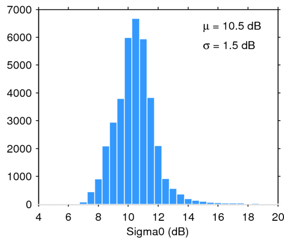
Figure 28. Histogram of science-valid sigma0 over oceans and lakes for 21/10/2014. The mean ( \mu ) and standard deviation ( \sigma ) are also shown. Note that values outside [4 20] dB are excluded from the histogram for the sake of readability but not from the computation of \mu and \sigma .
