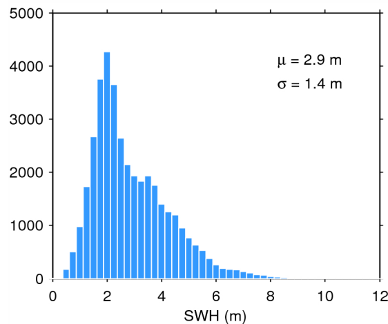
Figure 20. Histogram of science-valid SWH over oceans and lakes for 21/10/2014. The mean ( \mu ) and standard deviation ( \sigma ) are also shown. Note that values larger than 12 m are excluded from the histogram for the sake of readability but not from the computation of \mu and \sigma .
