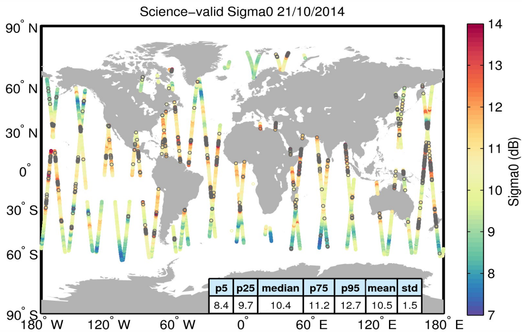
Figure 27. Geographical distribution of science-valid sigma0 data over oceans and lakes for 21/10/2014. The statistical values shown in the table refer to the sigma0 in dB and are calculated over all measurements shown in the figure. Gray circles denote records that have been rejected based on the editing criteria described in Table 4.
