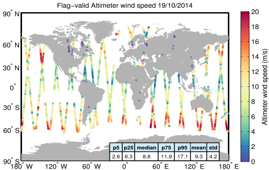
Figure 31. Geographical distribution of flag-valid wind data over oceans and lakes for 19/10/2014. The statistical values shown in the table refer to the wind in m/s and are calculated over all measurements shown in the figure.
