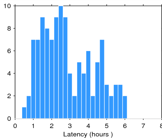
Figure 2. Histogram of the data latency for 19/10/2014. The y-axis denotes the number of files that are made available with a delay of x-hours with respect to the mean time of the records stored in the file.
