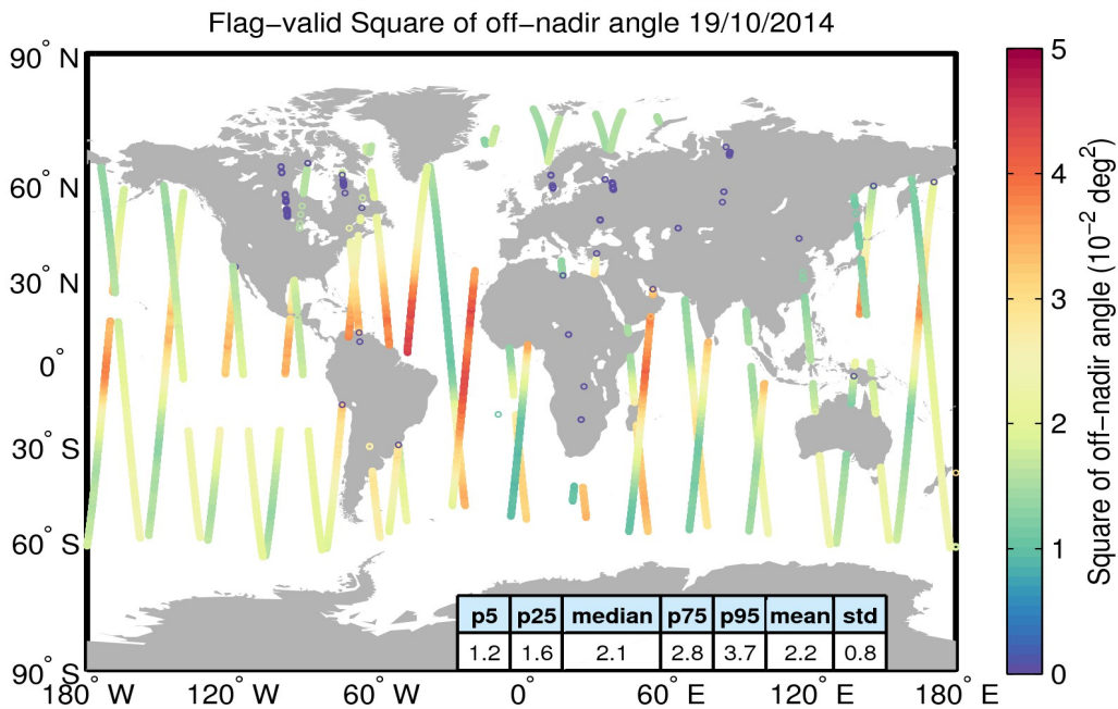
Figure 37. Geographical distribution of flag-valid mispointing data over oceans and lakes for 19/10/2014. The statistical values shown in the table refer to the mispointing in 10^{-2} \text{ deg}^2 and are calculated over all measurements shown in the figure.
