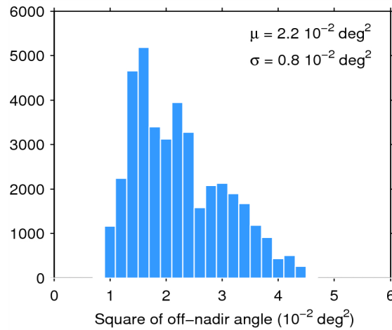
Figure 39. Histogram of flag-valid mispointing over oceans and lakes for 19/10/2014. The mean ( \mu ) and standard deviation ( \sigma ) are also shown. Note that values than 6 \cdot 10^{-2} \text{ deg}^2 are excluded from the histogram for the sake of readability but not from the computation of \mu and \sigma .
