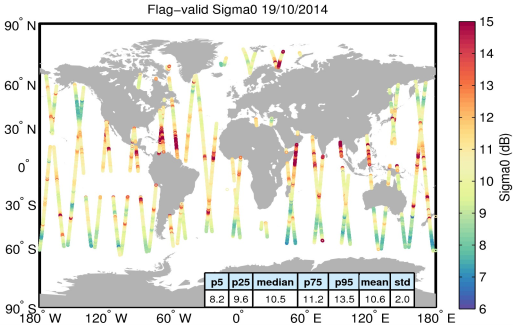
Figure 23. Geographical distribution of flag-valid sigma0 data over oceans and lakes for 19/10/2014. The statistical values shown in the table refer to the sigma0 in dB and are calculated over all measurements shown in the figure.
