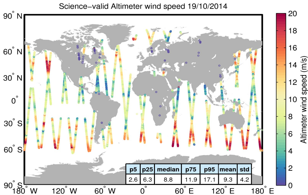
Figure 34. Geographical distribution of science-valid wind data over oceans and lakes for 19/10/2014. The statistical values shown in the table refer to the wind in m/s and are calculated over all measurements shown in the figure. Gray circles denote records that have been rejected based on the editing criteria described in Table 5.
