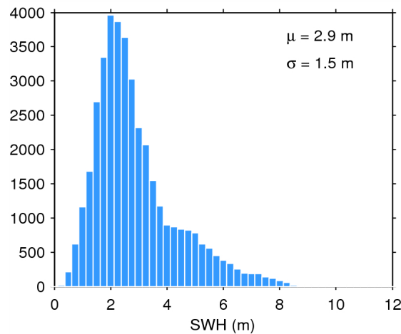
Figure 17. Histogram of flag-valid SWH over oceans and lakes for 19/10/2014. The mean ( \mu ) and standard deviation ( \sigma ) are also shown. Note that values larger than 12 m are excluded from the histogram for the sake of readability but not from the computation of \mu and \sigma .
