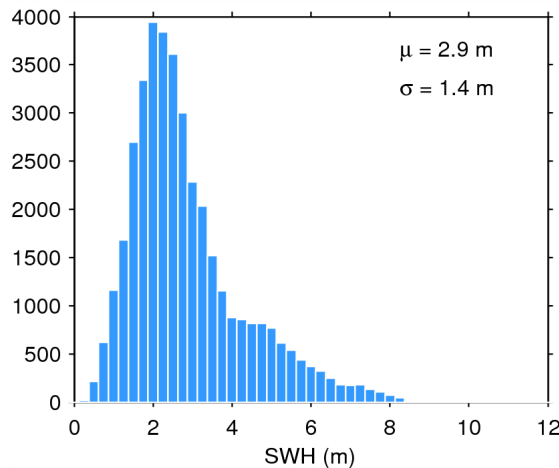
Figure 20. Histogram of science-valid SWH over oceans and lakes for 19/10/2014. The mean ( \mu ) and standard deviation ( \sigma ) are also shown. Note that values larger than 12 m are excluded from the histogram for the sake of readability but not from the computation of \mu and \sigma .
