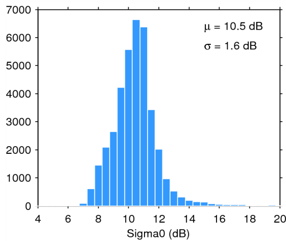
Figure 28. Histogram of science-valid sigma0 over oceans and lakes for 19/10/2014. The mean ( \mu ) and standard deviation ( \sigma ) are also shown. Note that values outside [4 20] dB are excluded from the histogram for the sake of readability but not from the computation of \mu and \sigma .
