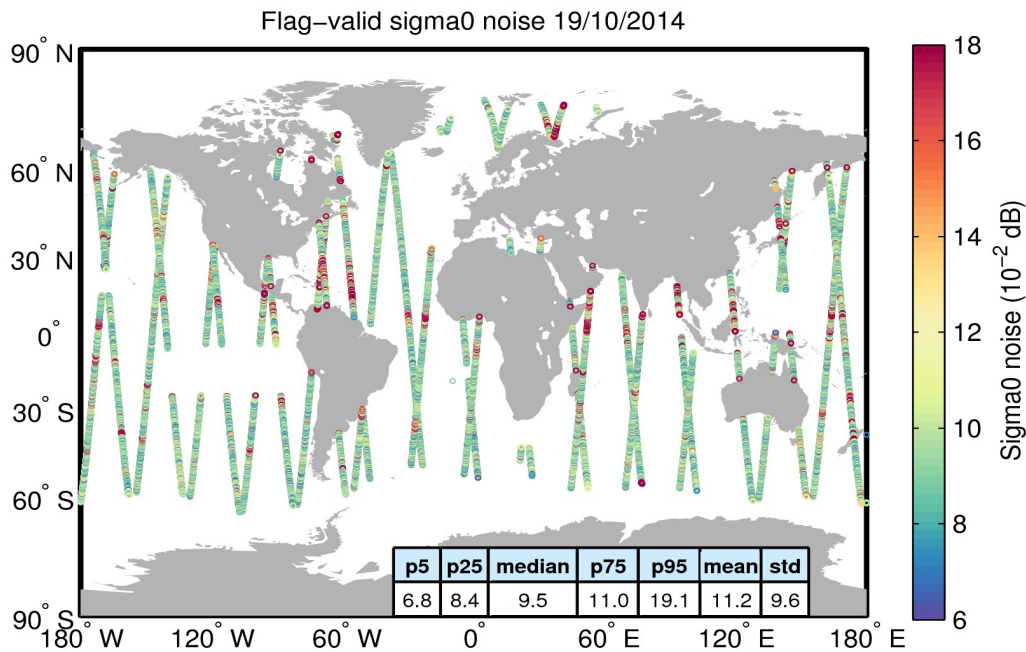
Figure 26. Geographical distribution of flag-valid 20-Hz sigma0 measurement noise over oceans and lakes for 19/10/2014. The statistical values shown in the table refer to the sigma0 noise and are calculated over all measurements shown in the figure.
