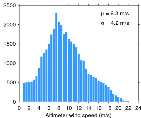
Figure 35. Histogram of science-valid wind over oceans and lakes for 19/10/2014. The mean ( \mu ) and standard deviation ( \sigma ) are also shown. Note that values larger than 24 m/s are excluded from the histogram for the sake of readability but not from the computation of \mu and \sigma .
