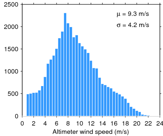
Figure 33. Histogram of flag-valid wind over oceans and lakes for 19/10/2014. The mean ( \mu ) and standard deviation ( \sigma ) are also shown. Note that values larger than 24 m/s are excluded from the histogram for the sake of readability but not from the computation of \mu and \sigma .
