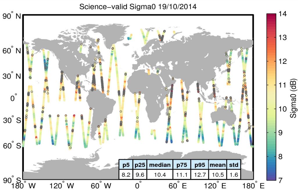
Figure 27. Geographical distribution of science-valid sigma0 data over oceans and lakes for 19/10/2014. The statistical values shown in the table refer to the sigma0 in dB and are calculated over all measurements shown in the figure. Gray circles denote records that have been rejected based on the editing criteria described in Table 4.
