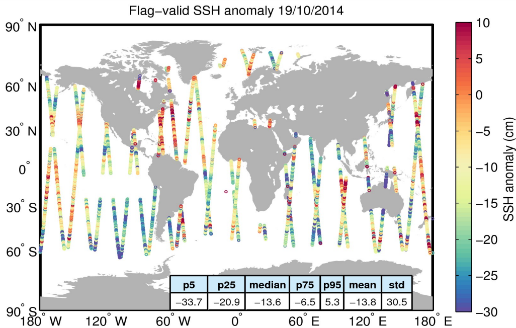
Figure 5. Geographical distribution of flag-valid 1-Hz SSH anomaly data over oceans and lakes for 19/10/2014. The statistical values shown in the table refer to the SSH anomaly in cm and are calculated over all measurements shown in the figure.
