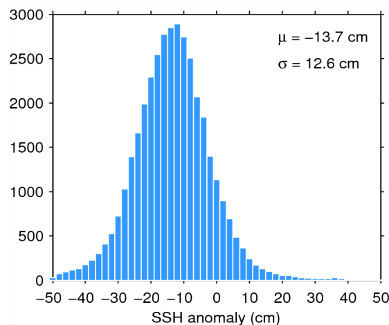
Figure 11. Histogram of science-valid SSH anomaly over oceans and lakes for 19/10/2014. The mean ( \mu ) and standard deviation ( \sigma ) are also shown. Note that values outside [-50 50] cm are excluded from the histogram for the sake of readability but not from the computation of \mu and \sigma .
