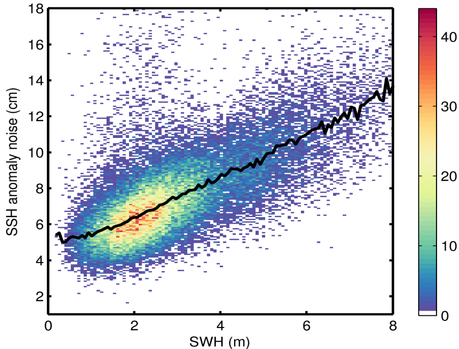
Figure 9. 2D histogram showing flag-valid SSH anomaly noise as a function of SWH for 19/10/2014. The black line denotes the median SSH anomaly as a function of SWH.
