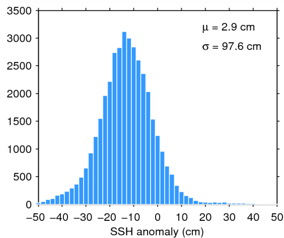
Figure 7. Histogram of flag-valid SSH anomaly over oceans and lakes for 18/10/2014. The mean ( \mu ) and standard deviation ( \sigma ) are also shown. Note that values outside [-50\ 50] cm are excluded from the histogram for the sake of readability but not from the computation of \mu and \sigma .
