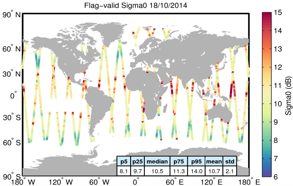
Figure 23. Geographical distribution of flag-valid sigma0 data over oceans and lakes for 18/10/2014. The statistical values shown in the table refer to the sigma0 in dB and are calculated over all measurements shown in the figure.
