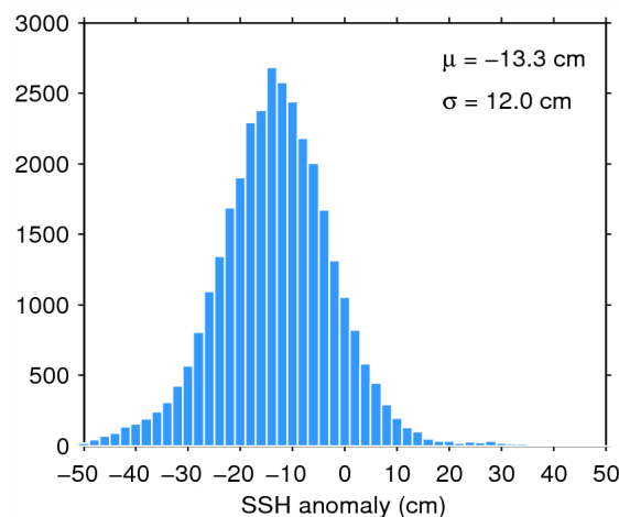
Figure 11. Histogram of science-valid SSH anomaly over oceans and lakes for 18/10/2014. The mean ( \mu ) and standard deviation ( \sigma ) are also shown. Note that values outside [-50 50] cm are excluded from the histogram for the sake of readability but not from the computation of \mu and \sigma .
