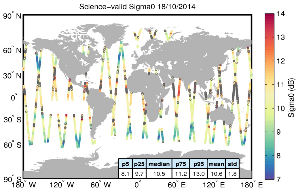
Figure 27. Geographical distribution of science-valid sigma0 data over oceans and lakes for 18/10/2014. The statistical values shown in the table refer to the sigma0 in dB and are calculated over all measurements shown in the figure. Gray circles denote records that have been rejected based on the editing criteria described in Table 4.
