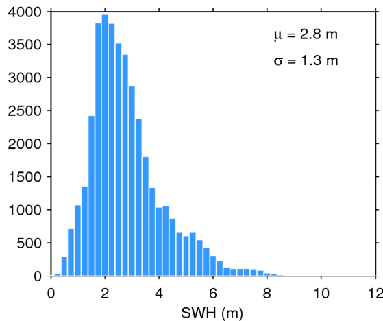
Figure 20. Histogram of science-valid SWH over oceans and lakes for 18/10/2014. The mean ( \mu ) and standard deviation ( \sigma ) are also shown. Note that values larger than 12 m are excluded from the histogram for the sake of readability but not from the computation of \mu and \sigma .
