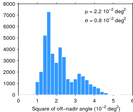
Figure 39. Histogram of flag-valid mispointing over oceans and lakes for 18/10/2014. The mean ( \mu ) and standard deviation ( \sigma ) are also shown. Note that values than 6 \cdot 10^{-2} \text{ deg}^2 are excluded from the histogram for the sake of readability but not from the computation of \mu and \sigma .
