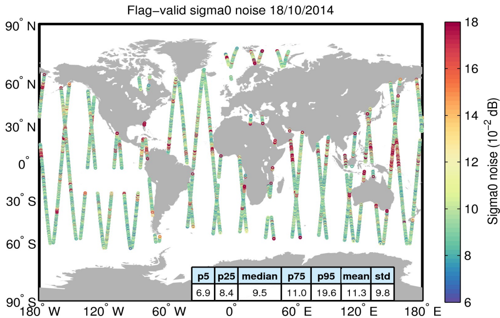
Figure 26. Geographical distribution of flag-valid 20-Hz sigma0 measurement noise over oceans and lakes for 18/10/2014. The statistical values shown in the table refer to the sigma0 noise and are calculated over all measurements shown in the figure.
