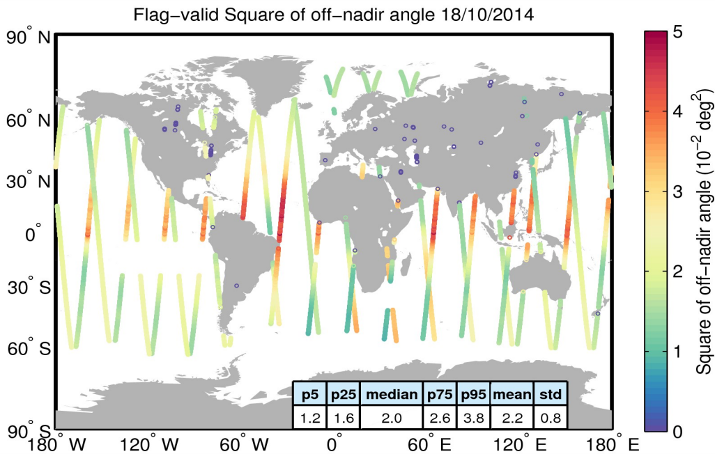
Figure 37. Geographical distribution of flag-valid mispointing data over oceans and lakes for 18/10/2014. The statistical values shown in the table refer to the mispointing in 10^{-2} \text{deg}^2 and are calculated over all measurements shown in the figure.
