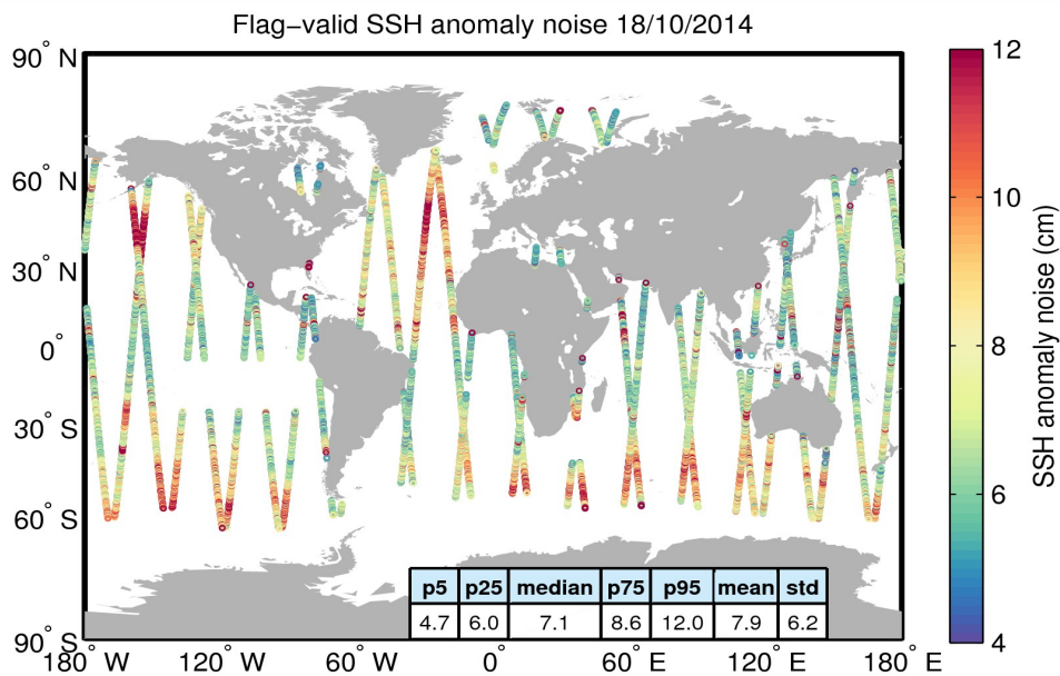
Figure 8. Geographical distribution of flag-valid 20-Hz SSH anomaly measurement noise over oceans and lakes for 18/10/2014. The statistical values shown in the table refer to the SSH anomaly noise and are calculated over all measurements shown in the figure.
