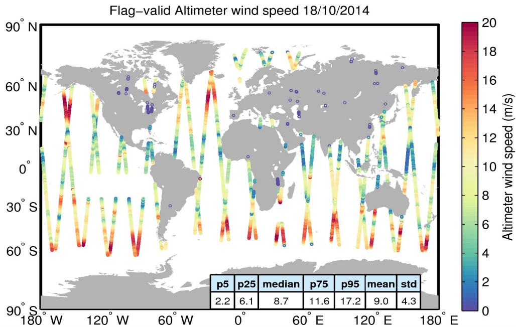
Figure 31. Geographical distribution of flag-valid wind data over oceans and lakes for 18/10/2014. The statistical values shown in the table refer to the wind in m/s and are calculated over all measurements shown in the figure.
