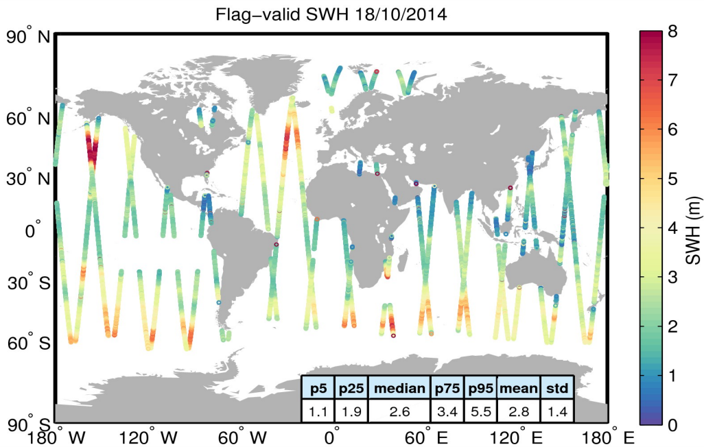
Figure 15. Geographical distribution of flag-valid SWH data over oceans and lakes for 18/10/2014. The statistical values shown in the table refer to the SWH in m and are calculated over all measurements shown in the figure.
