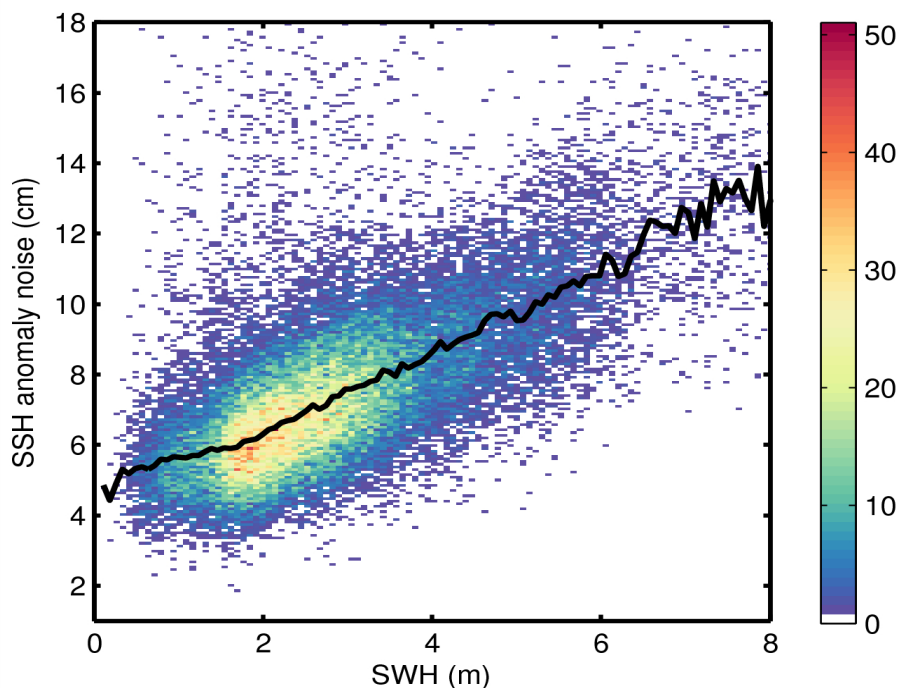
Figure 9. 2D histogram showing flag-valid SSH anomaly noise as a function of SWH for 18/10/2014. The black line denotes the median SSH anomaly as a function of SWH.
