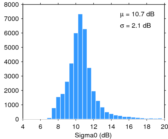
Figure 25. Histogram of flag-valid sigma0 over oceans and lakes for 18/10/2014. The mean ( \mu ) and standard deviation ( \sigma ) are also shown. Note that values outside [4 20] dB are excluded from the histogram for the sake of readability but not from the computation of \mu and \sigma .
