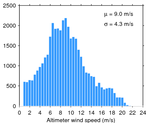
Figure 35. Histogram of science-valid wind over oceans and lakes for 18/10/2014. The mean ( \mu ) and standard deviation ( \sigma ) are also shown. Note that values larger than 24 m/s are excluded from the histogram for the sake of readability but not from the computation of \mu and \sigma .
