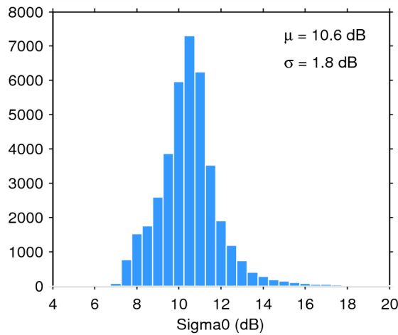
Figure 28. Histogram of science-valid sigma0 over oceans and lakes for 18/10/2014. The mean ( \mu ) and standard deviation ( \sigma ) are also shown. Note that values outside [4 20] dB are excluded from the histogram for the sake of readability but not from the computation of \mu and \sigma .
