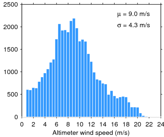
Figure 33. Histogram of flag-valid wind over oceans and lakes for 18/10/2014. The mean ( \mu ) and standard deviation ( \sigma ) are also shown. Note that values larger than 24 m/s are excluded from the histogram for the sake of readability but not from the computation of \mu and \sigma .
