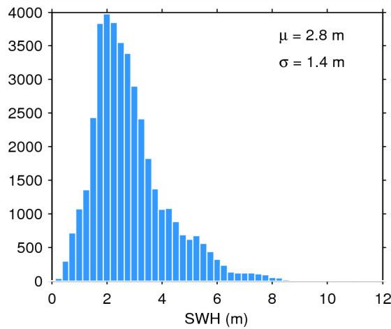
Figure 17. Histogram of flag-valid SWH over oceans and lakes for 18/10/2014. The mean ( \mu ) and standard deviation ( \sigma ) are also shown. Note that values larger than 12 m are excluded from the histogram for the sake of readability but not from the computation of \mu and \sigma .
