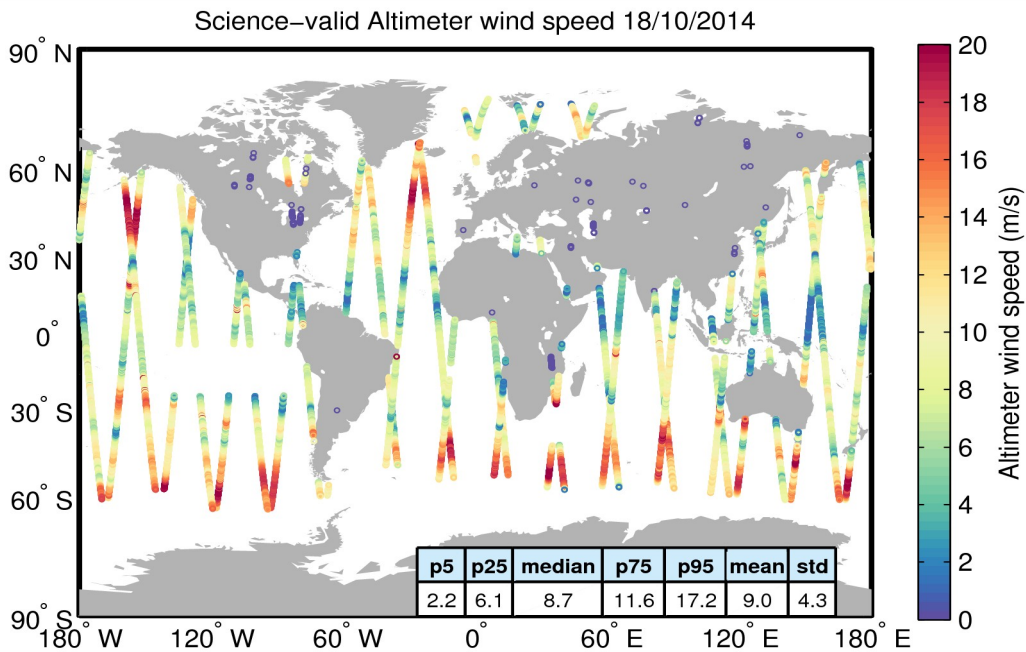
Figure 34. Geographical distribution of science-valid wind data over oceans and lakes for 18/10/2014. The statistical values shown in the table refer to the wind in m/s and are calculated over all measurements shown in the figure. Gray circles denote records that have been rejected based on the editing criteria described in Table 5.
