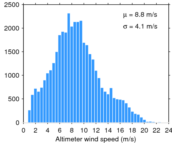
Figure 33. Histogram of flag-valid wind over oceans and lakes for 17/10/2014. The mean ( \mu ) and standard deviation ( \sigma ) are also shown. Note that values larger than 24 m/s are excluded from the histogram for the sake of readability but not from the computation of \mu and \sigma .
