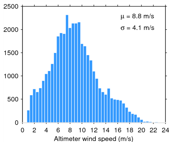
Figure 35. Histogram of science-valid wind over oceans and lakes for 17/10/2014. The mean ( \mu ) and standard deviation ( \sigma ) are also shown. Note that values larger than 24 m/s are excluded from the histogram for the sake of readability but not from the computation of \mu and \sigma .
