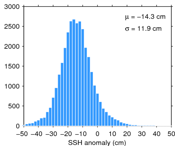
Figure 11. Histogram of science-valid SSH anomaly over oceans and lakes for 17/10/2014. The mean ( \mu ) and standard deviation ( \sigma ) are also shown. Note that values outside [-50 50] cm are excluded from the histogram for the sake of readability but not from the computation of \mu and \sigma .
