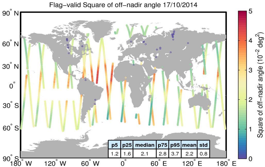
Figure 37. Geographical distribution of flag-valid mispointing data over oceans and lakes for 17/10/2014. The statistical values shown in the table refer to the mispointing in 10^{-2} \text{ deg}^2 and are calculated over all measurements shown in the figure.
