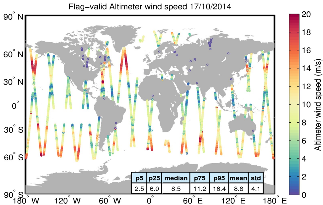
Figure 31. Geographical distribution of flag-valid wind data over oceans and lakes for 17/10/2014. The statistical values shown in the table refer to the wind in m/s and are calculated over all measurements shown in the figure.
