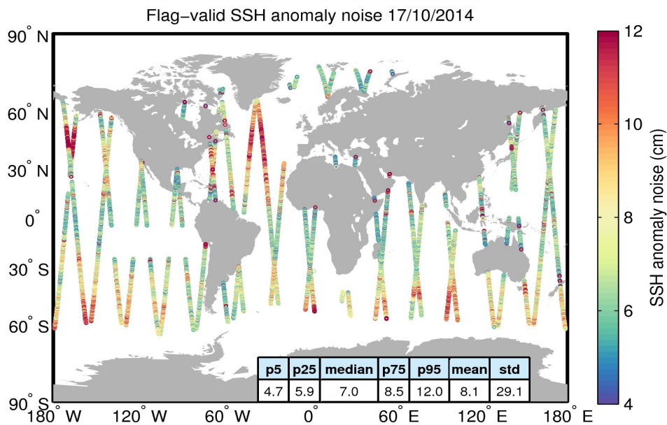
Figure 8. Geographical distribution of flag-valid 20-Hz SSH anomaly measurement noise over oceans and lakes for 17/10/2014. The statistical values shown in the table refer to the SSH anomaly noise and are calculated over all measurements shown in the figure.
