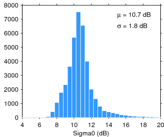
Figure 25. Histogram of flag-valid sigma0 over oceans and lakes for 17/10/2014. The mean ( \mu ) and standard deviation ( \sigma ) are also shown. Note that values outside [4 20] dB are excluded from the histogram for the sake of readability but not from the computation of \mu and \sigma .
