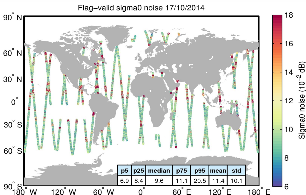
Figure 26. Geographical distribution of flag-valid 20-Hz sigma0 measurement noise over oceans and lakes for 17/10/2014. The statistical values shown in the table refer to the sigma0 noise and are calculated over all measurements shown in the figure.
