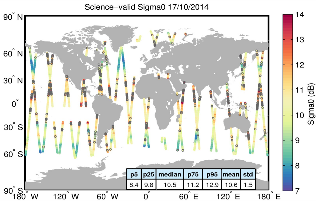
Figure 27. Geographical distribution of science-valid sigma0 data over oceans and lakes for 17/10/2014. The statistical values shown in the table refer to the sigma0 in dB and are calculated over all measurements shown in the figure. Gray circles denote records that have been rejected based on the editing criteria described in Table 4.
