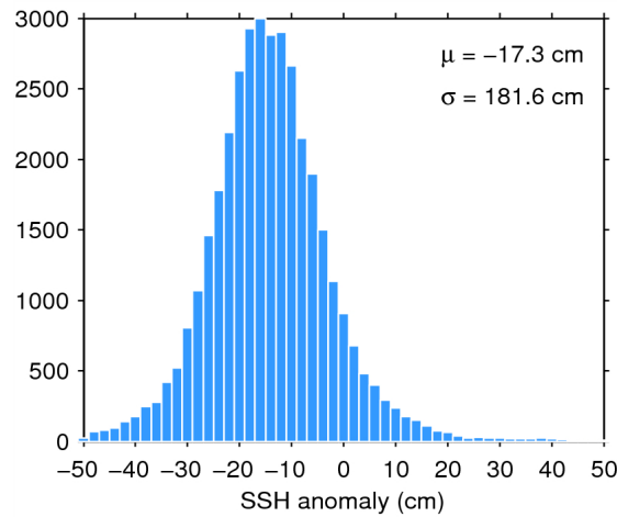
Figure 7. Histogram of flag-valid SSH anomaly over oceans and lakes for 17/10/2014. The mean ( \mu ) and standard deviation ( \sigma ) are also shown. Note that values outside [-50 50] cm are excluded from the histogram for the sake of readability but not from the computation of \mu and \sigma .
