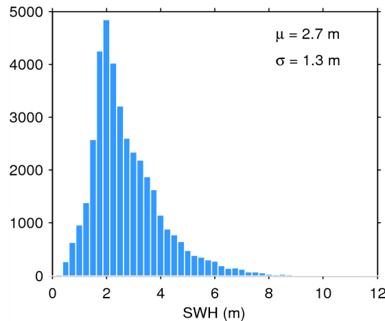
Figure 20. Histogram of science-valid SWH over oceans and lakes for 17/10/2014. The mean ( \mu ) and standard deviation ( \sigma ) are also shown. Note that values larger than 12 m are excluded from the histogram for the sake of readability but not from the computation of \mu and \sigma .
