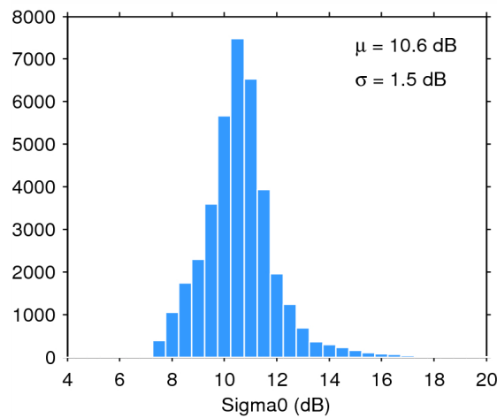
Figure 28. Histogram of science-valid sigma0 over oceans and lakes for 17/10/2014. The mean ( \mu ) and standard deviation ( \sigma ) are also shown. Note that values outside [4 20] dB are excluded from the histogram for the sake of readability but not from the computation of \mu and \sigma .
