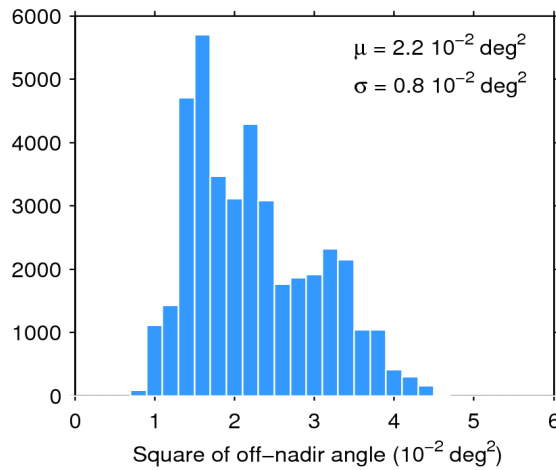
Figure 39. Histogram of flag-valid mispointing over oceans and lakes for 17/10/2014. The mean ( \mu ) and standard deviation ( \sigma ) are also shown. Note that values than 6 \cdot 10^{-2} \text{ deg}^2 are excluded from the histogram for the sake of readability but not from the computation of \mu and \sigma .
