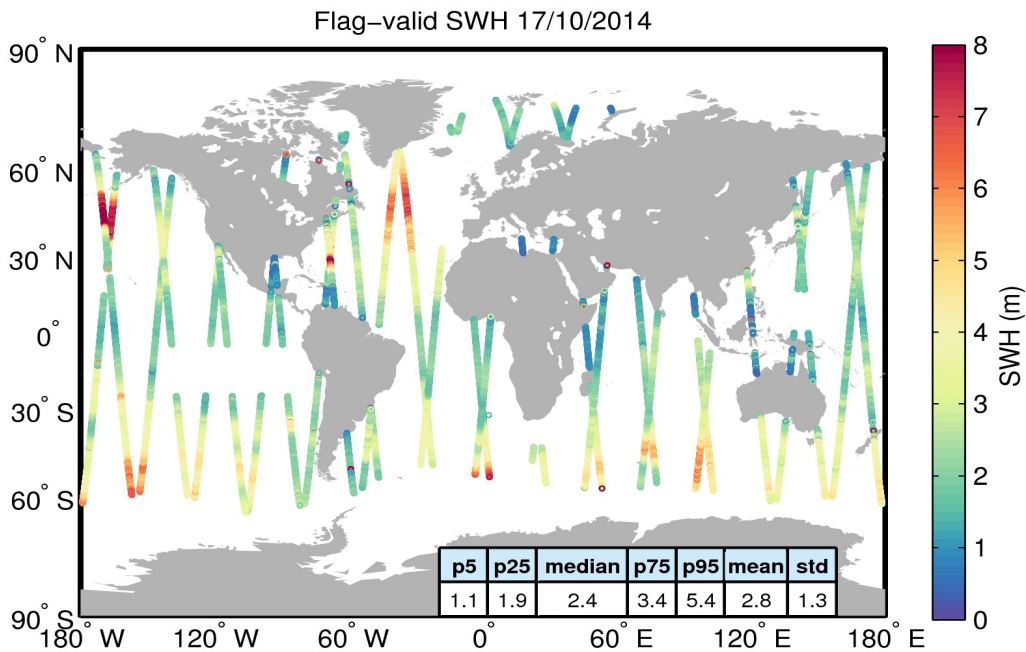
Figure 15. Geographical distribution of flag-valid SWH data over oceans and lakes for 17/10/2014. The statistical values shown in the table refer to the SWH in m and are calculated over all measurements shown in the figure.
