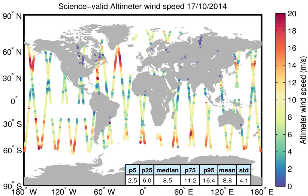
Figure 34. Geographical distribution of science-valid wind data over oceans and lakes for 17/10/2014. The statistical values shown in the table refer to the wind in m/s and are calculated over all measurements shown in the figure. Gray circles denote records that have been rejected based on the editing criteria described in Table 5.
