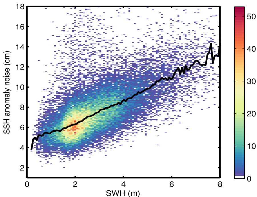
Figure 9. 2D histogram showing flag-valid SSH anomaly noise as a function of SWH for 17/10/2014. The black line denotes the median SSH anomaly as a function of SWH.
