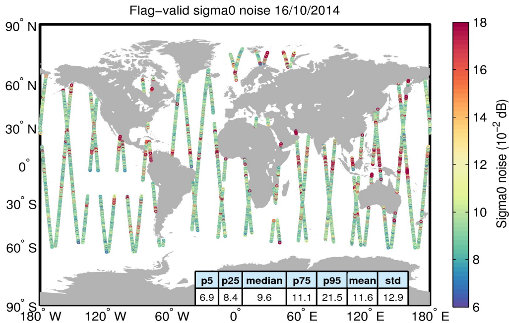
Figure 26. Geographical distribution of flag-valid 20-Hz sigma0 measurement noise over oceans and lakes for 16/10/2014. The statistical values shown in the figure refer to the sigma0 noise and are calculated over all measurements shown in the figure.
