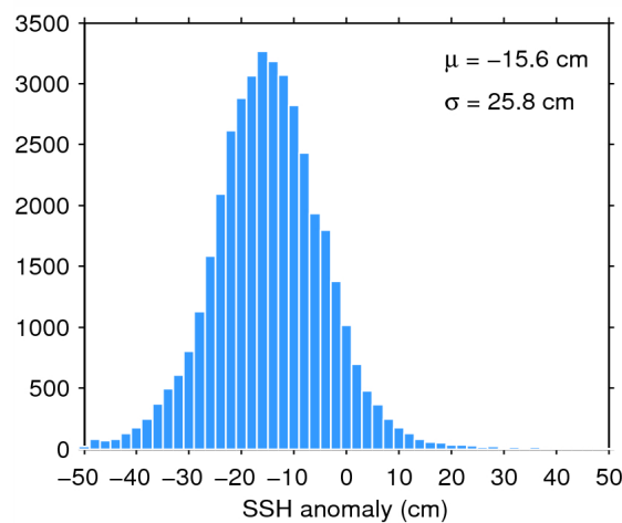
Figure 7. Histogram of flag-valid SSH anomaly over oceans and lakes for 16/10/2014. The mean ( \mu ) and standard deviation ( \sigma ) are also shown. Note that values outside [-50 50] cm are excluded from the histogram for the sake of readability but not from the computation of \mu and \sigma .
