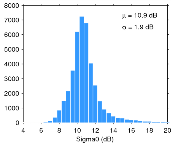
Figure 25. Histogram of flag-valid sigma0 over oceans and lakes for 16/10/2014. The mean ( \mu ) and standard deviation ( \sigma ) are also shown. Note that values outside [4 20] dB are excluded from the histogram for the sake of readability but not from the computation of \mu and \sigma .
