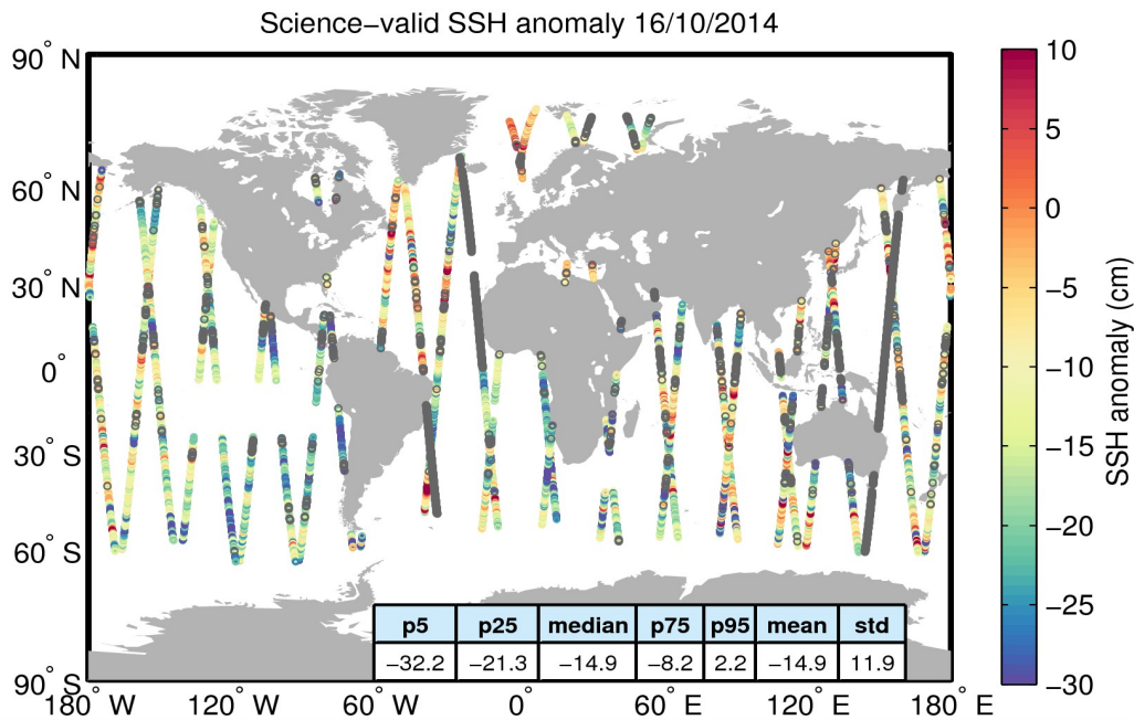
Figure 10. Geographical distribution of science-valid SSH anomaly data over oceans and lakes for 16/10/2014. The statistical values shown in the table refer to the SSH anomaly in cm and are calculated over all measurements shown in the figure. Gray circles denote records that have been rejected based on the editing criteria described in Table 2.
