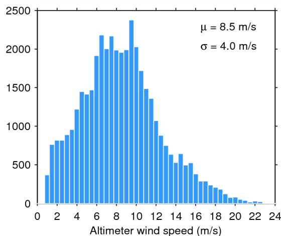
Figure 35. Histogram of science-valid wind over oceans and lakes for 16/10/2014. The mean ( \mu ) and standard deviation ( \sigma ) are also shown. Note that values larger than 24 m/s are excluded from the histogram for the sake of readability but not from the computation of \mu and \sigma .
