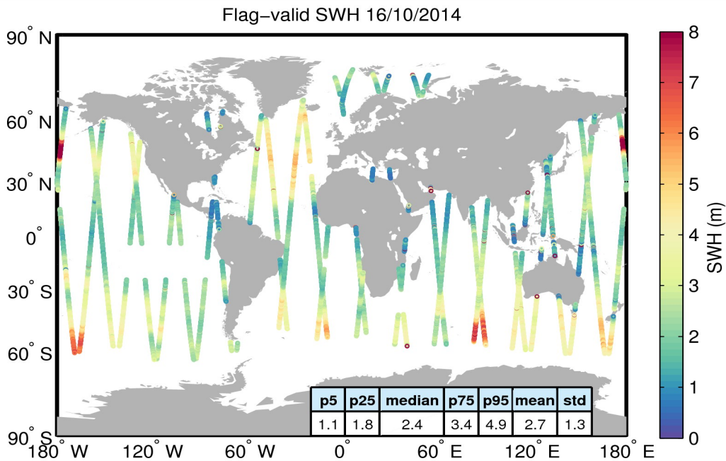
Figure 15. Geographical distribution of flag-valid SWH data over oceans and lakes for 16/10/2014. The statistical values shown in the table refer to the SWH in m and are calculated over all measurements shown in the figure.
