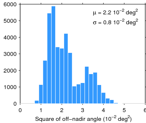
Figure 39. Histogram of flag-valid mispointing over oceans and lakes for 16/10/2014. The mean ( \mu ) and standard deviation ( \sigma ) are also shown. Note that values than 6 \cdot 10^{-2} \text{ deg}^2 are excluded from the histogram for the sake of readability but not from the computation of \mu and \sigma .
