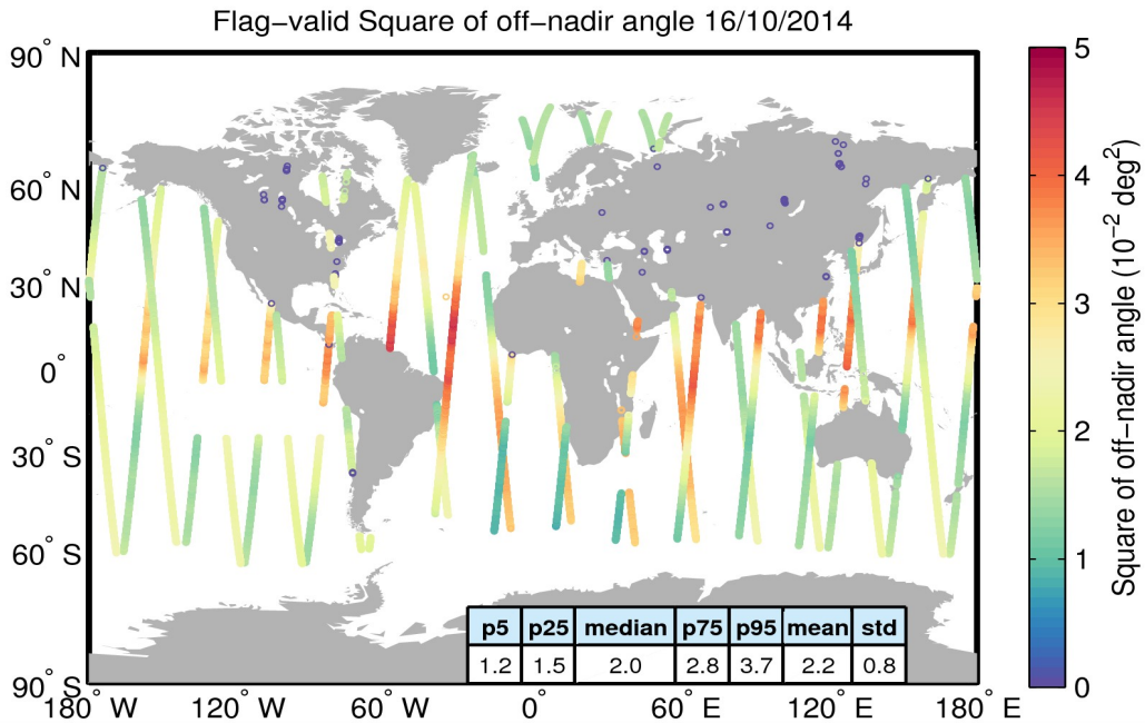
Figure 37. Geographical distribution of flag-valid mispointing data over oceans and lakes for 16/10/2014. The statistical values shown in the table refer to the mispointing in 10^{-2} \text{deg}^2 and are calculated over all measurements shown in the figure.
