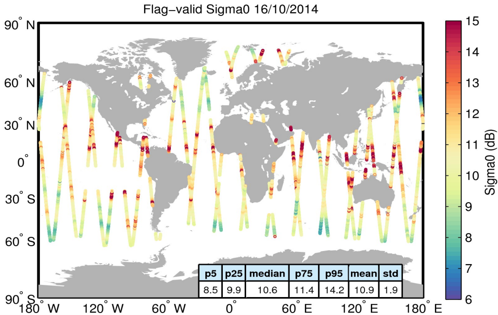
Figure 23. Geographical distribution of flag-valid sigma0 data over oceans and lakes for 16/10/2014. The statistical values shown in the table refer to the sigma0 in dB and are calculated over all measurements shown in the figure.
