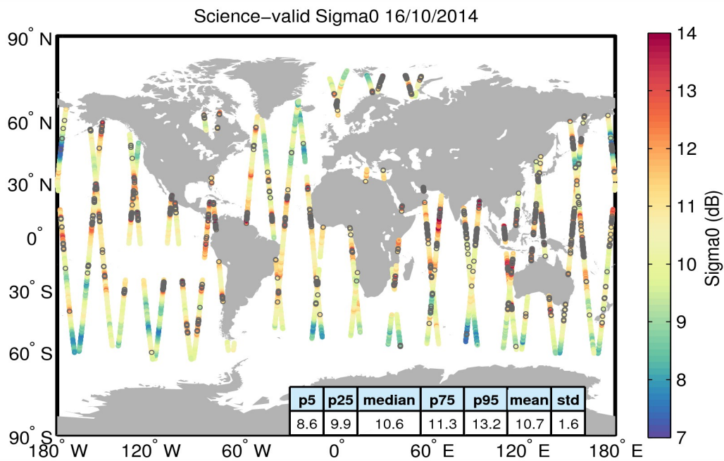
Figure 27. Geographical distribution of science-valid sigma0 data over oceans and lakes for 16/10/2014. The statistical values shown in the table refer to the sigma0 in dB and are calculated over all measurements shown in the figure. Gray circles denote records that have been rejected based on the editing criteria described in Table 4.
