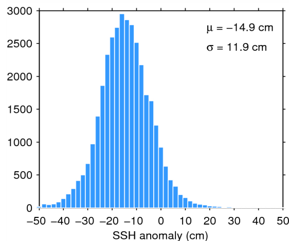
Figure 11. Histogram of science-valid SSH anomaly over oceans and lakes for 16/10/2014. The mean ( \mu ) and standard deviation ( \sigma ) are also shown. Note that values outside [-50 50] cm are excluded from the histogram for the sake of readability but not from the computation of \mu and \sigma .
