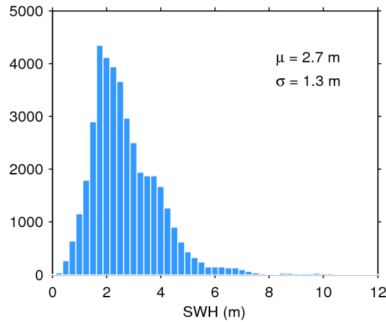
Figure 17. Histogram of flag-valid SWH over oceans and lakes for 16/10/2014. The mean ( \mu ) and standard deviation ( \sigma ) are also shown. Note that values larger than 12 m are excluded from the histogram for the sake of readability but not from the computation of \mu and \sigma .
