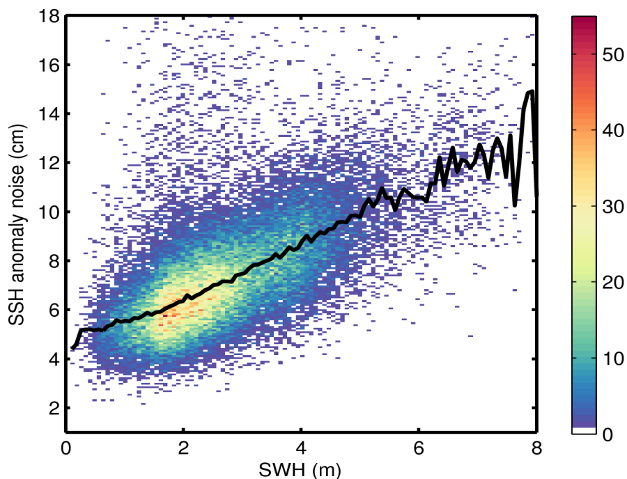
Figure 9. 2D histogram showing flag-valid SSH anomaly noise as a function of SWH for 16/10/2014. The black line denotes the median SSH anomaly as a function of SWH.
