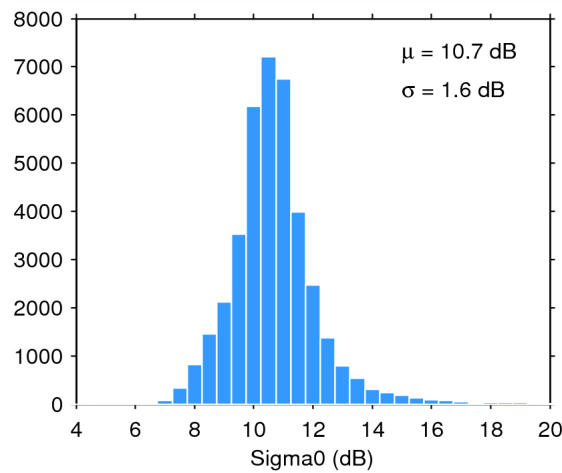
Figure 28. Histogram of science-valid sigma0 over oceans and lakes for 16/10/2014. The mean ( \mu ) and standard deviation ( \sigma ) are also shown. Note that values outside [4 20] dB are excluded from the histogram for the sake of readability but not from the computation of \mu and \sigma .
