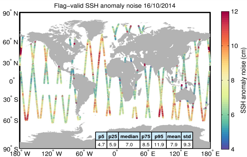
Figure 8. Geographical distribution of flag-valid 20-Hz SSH anomaly measurement noise over oceans and lakes for 16/10/2014. The statistical values shown in the table refer to the SSH anomaly noise and are calculated over all measurements shown in the figure.
