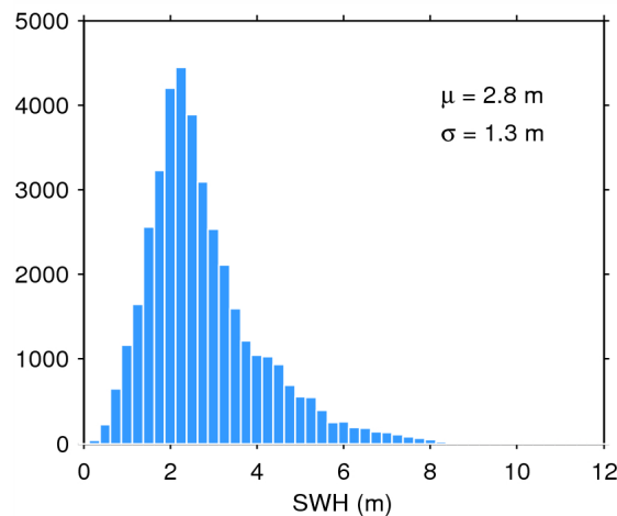
Figure 20. Histogram of science-valid SWH over oceans and lakes for 15/10/2014. The mean ( \mu ) and standard deviation ( \sigma ) are also shown. Note that values larger than 12 m are excluded from the histogram for the sake of readability but not from the computation of \mu and \sigma .
