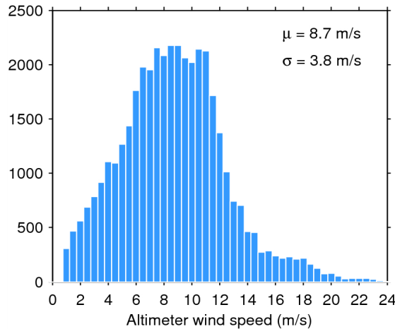
Figure 33. Histogram of flag-valid wind over oceans and lakes for 15/10/2014. The mean ( \mu ) and standard deviation ( \sigma ) are also shown. Note that values larger than 24 m/s are excluded from the histogram for the sake of readability but not from the computation of \mu and \sigma .
