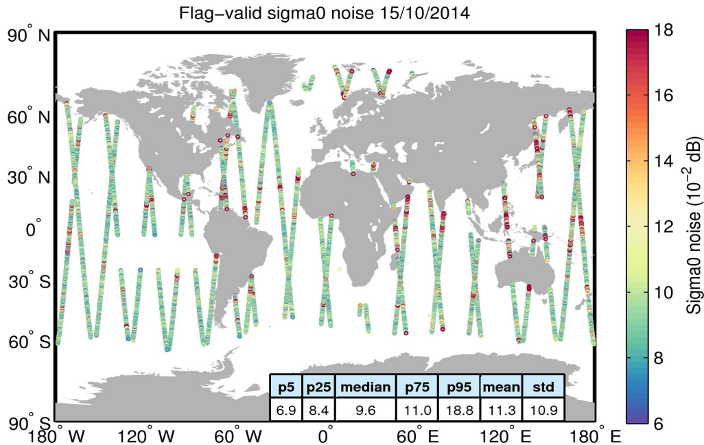
Figure 26. Geographical distribution of flag-valid 20-Hz sigma0 measurement noise over oceans and lakes for 15/10/2014. The statistical values shown in the table refer to the sigma0 noise and are calculated over all measurements shown in the figure.
