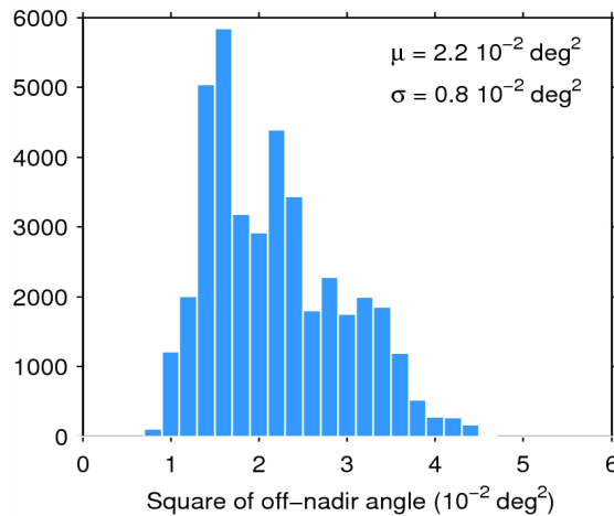
Figure 39. Histogram of flag-valid mispointing over oceans and lakes for 15/10/2014. The mean ( \mu ) and standard deviation ( \sigma ) are also shown. Note that values than 6 \cdot 10^{-2} \text{ deg}^2 are excluded from the histogram for the sake of readability but not from the computation of \mu and \sigma .
