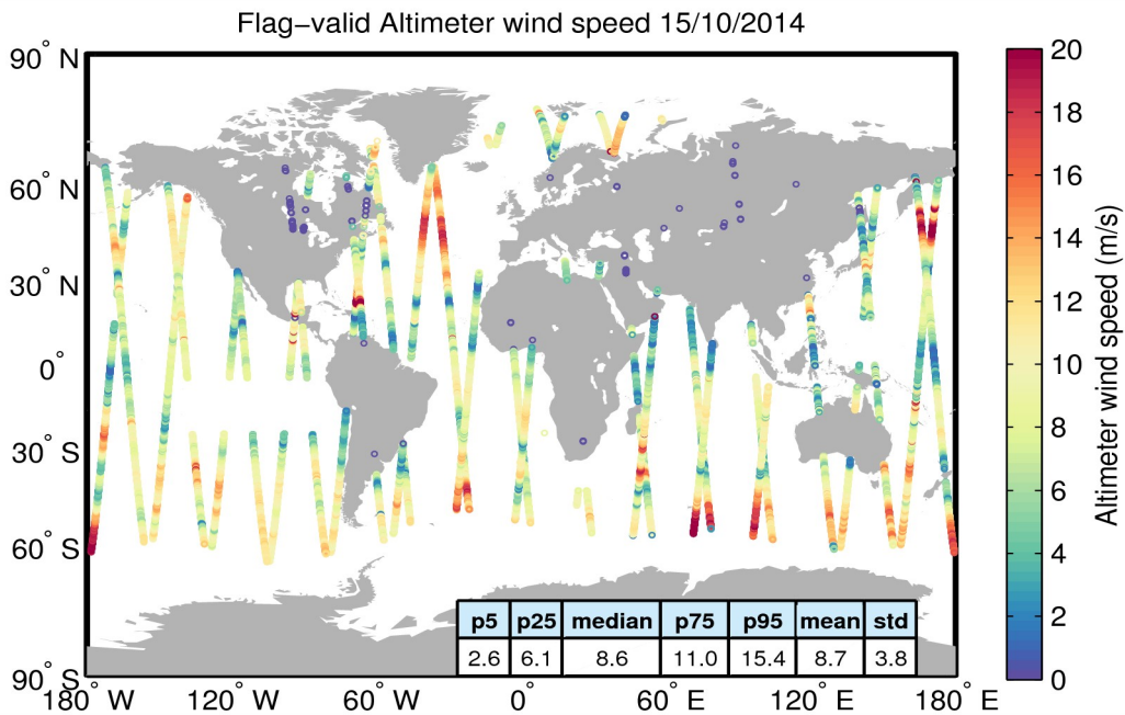
Figure 31. Geographical distribution of flag-valid wind data over oceans and lakes for 15/10/2014. The statistical values shown in the table refer to the wind in m/s and are calculated over all measurements shown in the figure.
