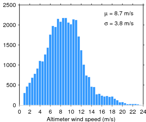
Figure 35. Histogram of science-valid wind over oceans and lakes for 15/10/2014. The mean ( \mu ) and standard deviation ( \sigma ) are also shown. Note that values larger than 24 m/s are excluded from the histogram for the sake of readability but not from the computation of \mu and \sigma .
