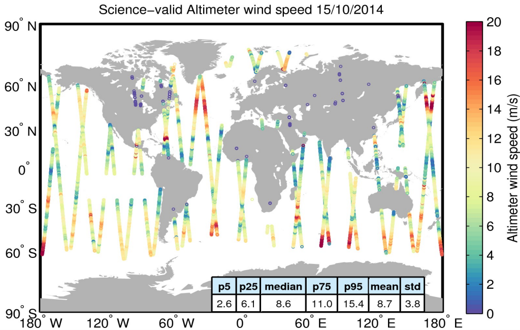
Figure 34. Geographical distribution of science-valid wind data over oceans and lakes for 15/10/2014. The statistical values shown in the table refer to the wind in m/s and are calculated over all measurements shown in the figure. Gray circles denote records that have been rejected based on the editing criteria described in Table 5.
