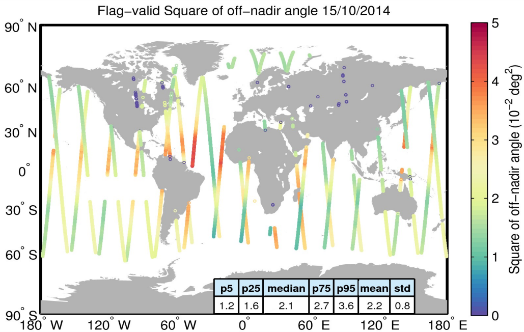
Figure 37. Geographical distribution of flag-valid mispointing data over oceans and lakes for 15/10/2014. The statistical values shown in the table refer to the mispointing in 10^{-2} \text{ deg}^2 and are calculated over all measurements shown in the figure.
