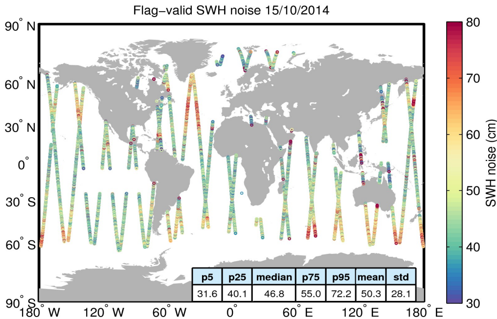
Figure 18. Geographical distribution of flag-valid 20-Hz SWH measurement noise over oceans and lakes for 15/10/2014. The statistical values shown in the figure refer to the SWH noise and are calculated over all measurements shown in the figure.
