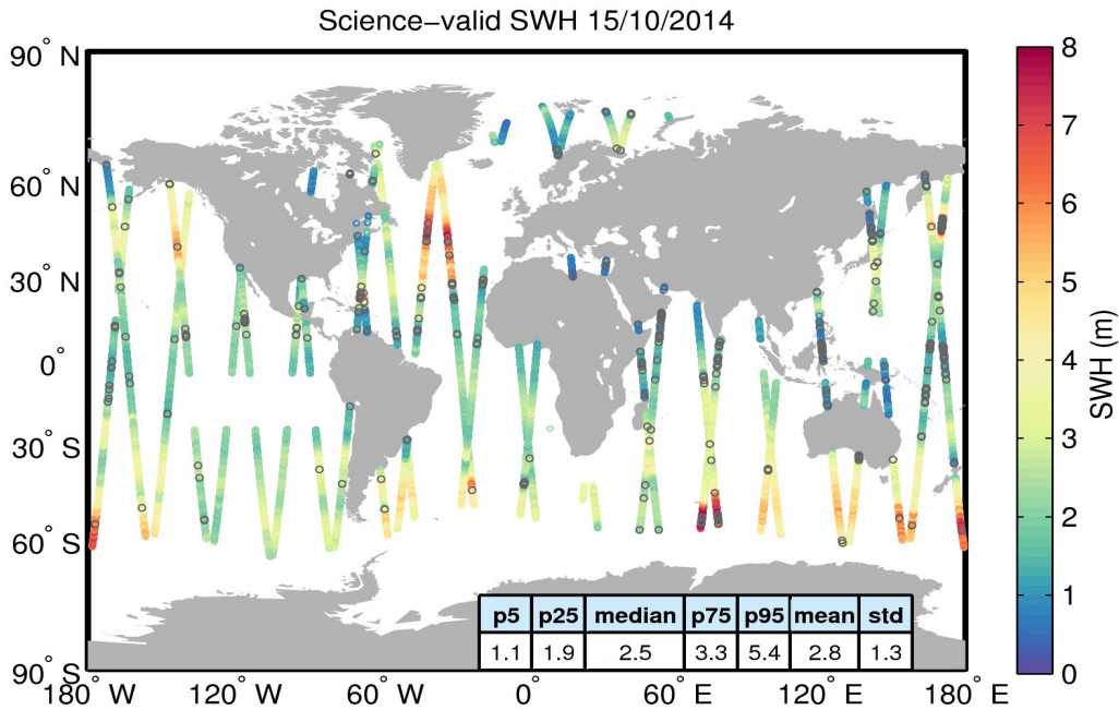
Figure 19. Geographical distribution of science-valid SWH data over oceans and lakes for 15/10/2014. The statistical values shown in the table refer to the SWH in m and are calculated over all measurements shown in the figure. Gray circles denote records that have been rejected based on the editing criteria described in Table 3.
