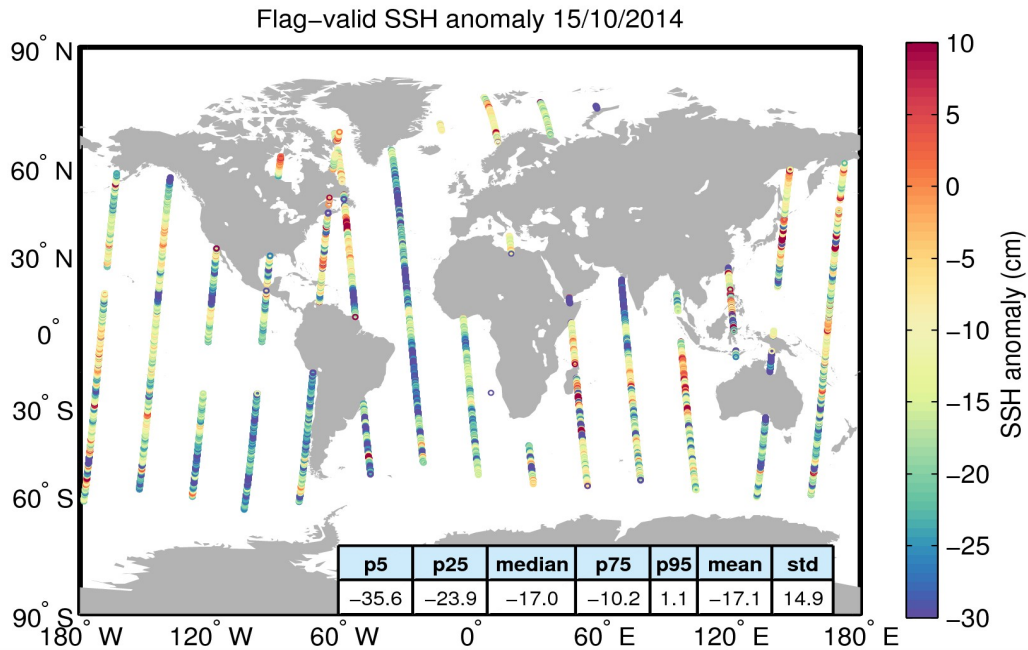
Figure 5. Geographical distribution of flag-valid 1-Hz SSH anomaly data over oceans and lakes for 15/10/2014. The statistical values shown in the table refer to the SSH anomaly in cm and are calculated over all measurements shown in the figure.
