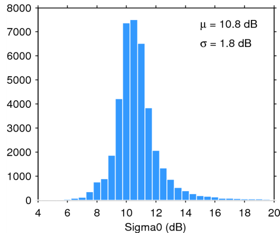
Figure 25. Histogram of flag-valid sigma0 over oceans and lakes for 15/10/2014. The mean ( \mu ) and standard deviation ( \sigma ) are also shown. Note that values outside [4 20] dB are excluded from the histogram for the sake of readability but not from the computation of \mu and \sigma .
