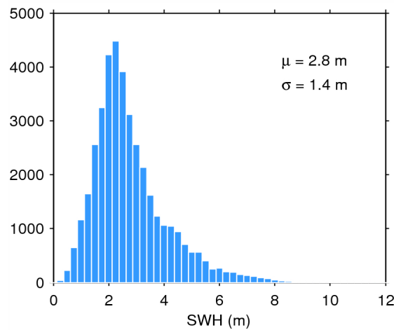
Figure 17. Histogram of flag-valid SWH over oceans and lakes for 15/10/2014. The mean ( \mu ) and standard deviation ( \sigma ) are also shown. Note that values larger than 12 m are excluded from the histogram for the sake of readability but not from the computation of \mu and \sigma .
