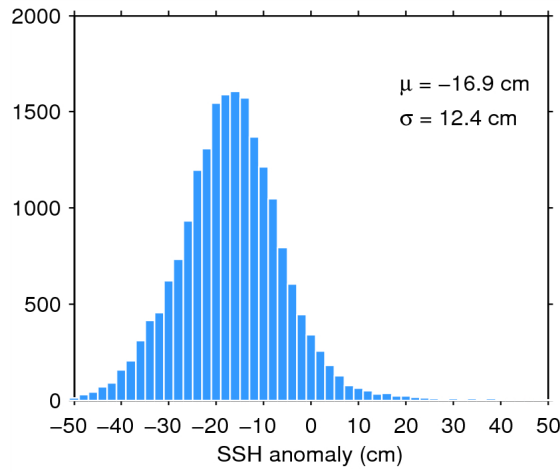
Figure 11. Histogram of science-valid SSH anomaly over oceans and lakes for 15/10/2014. The mean ( \mu ) and standard deviation ( \sigma ) are also shown. Note that values outside [-50 50] cm are excluded from the histogram for the sake of readability but not from the computation of \mu and \sigma .
