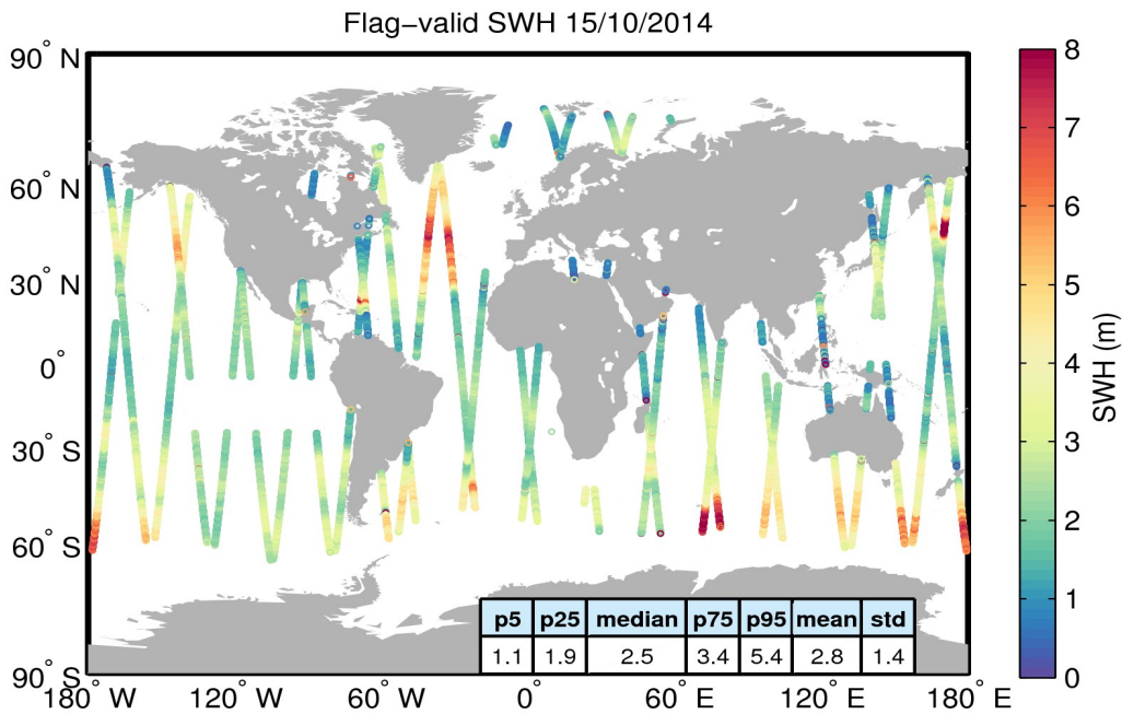
Figure 15. Geographical distribution of flag-valid SWH data over oceans and lakes for 15/10/2014. The statistical values shown in the table refer to the SWH in m and are calculated over all measurements shown in the figure.
