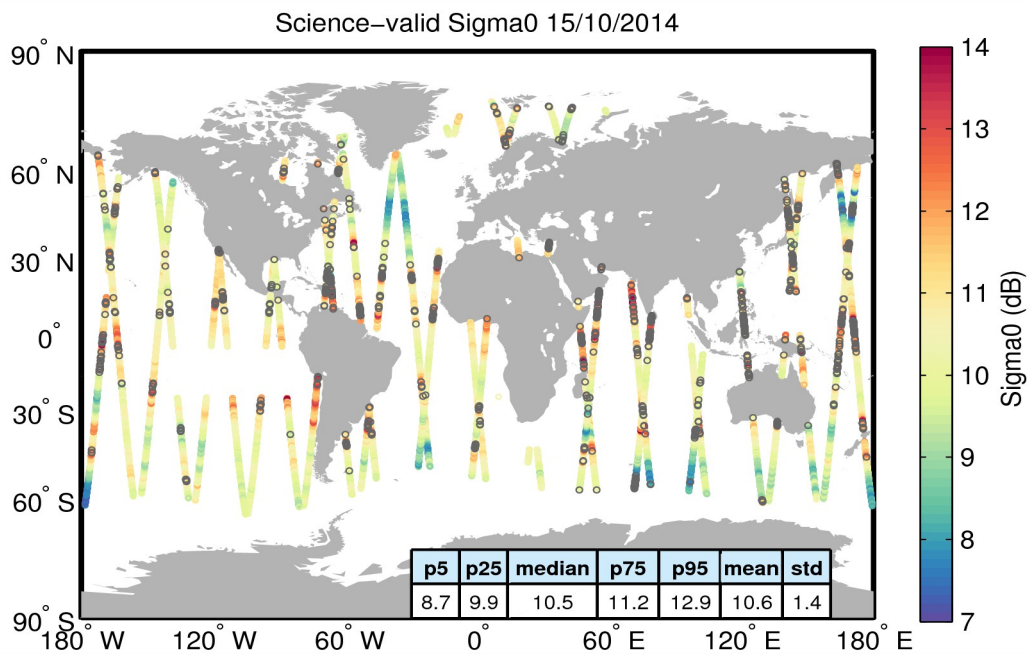
Figure 27. Geographical distribution of science-valid sigma0 data over oceans and lakes for 15/10/2014. The statistical values shown in the table refer to the sigma0 in dB and are calculated over all measurements shown in the figure. Gray circles denote records that have been rejected based on the editing criteria described in Table 4.
