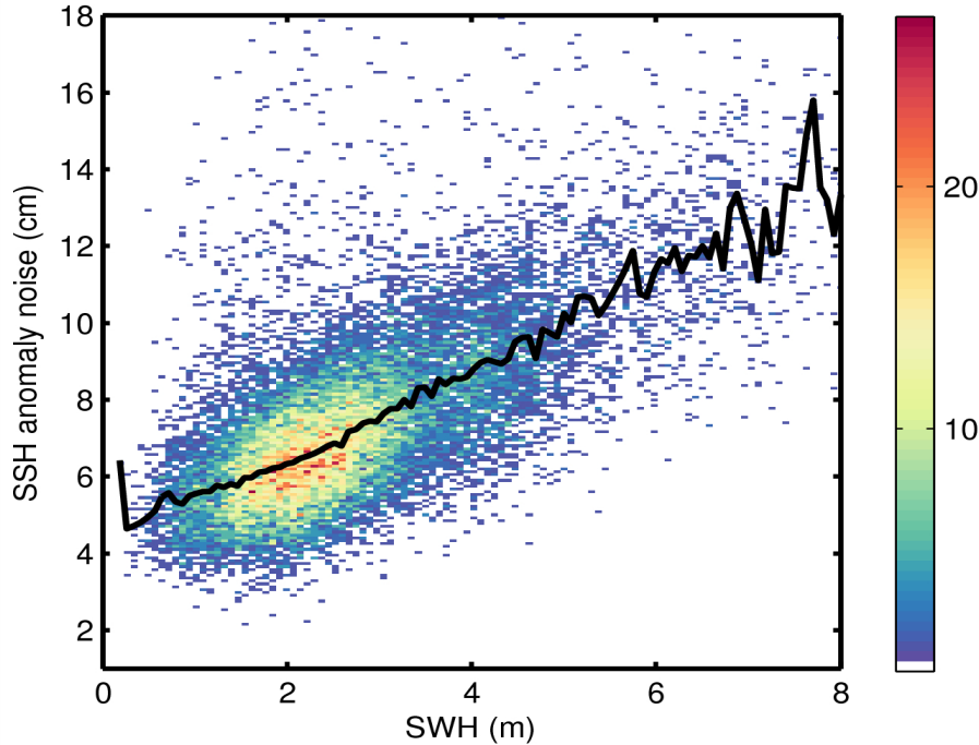
Figure 9. 2D histogram showing flag-valid SSH anomaly noise as a function of SWH for 15/10/2014. The black line denotes the median SSH anomaly as a function of SWH.
