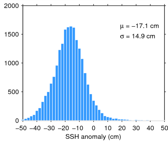
Figure 7. Histogram of flag-valid SSH anomaly over oceans and lakes for 15/10/2014. The mean ( \mu ) and standard deviation ( \sigma ) are also shown. Note that values outside [-50 50] cm are excluded from the histogram for the sake of readability but not from the computation of \mu and \sigma .
