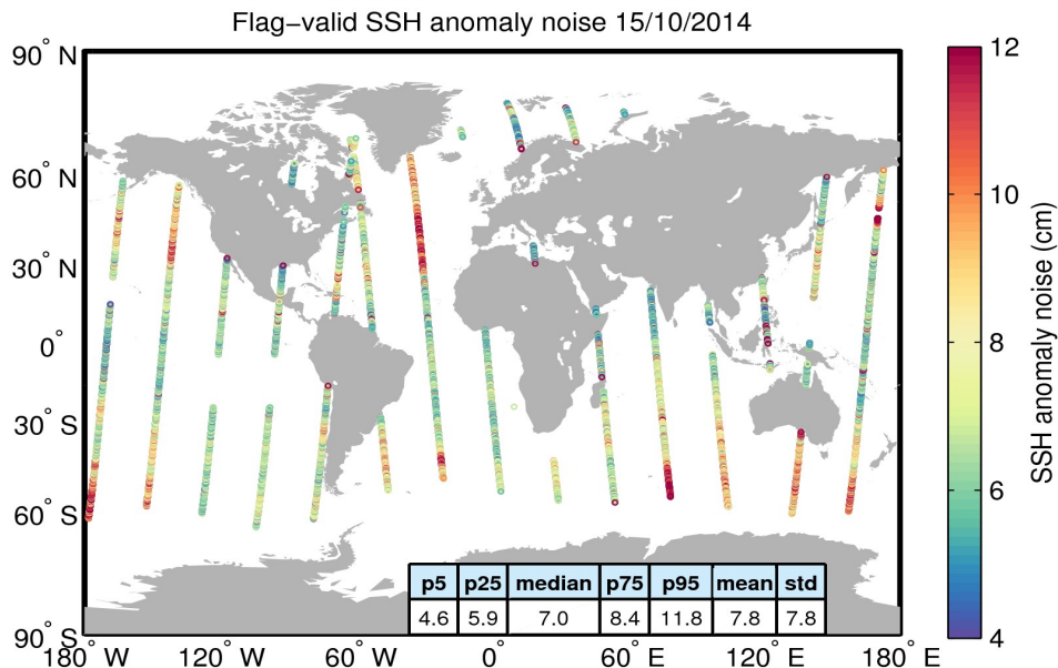
Figure 8. Geographical distribution of flag-valid 20-Hz SSH anomaly measurement noise over oceans and lakes for 15/10/2014. The statistical values shown in the table refer to the SSH anomaly noise and are calculated over all measurements shown in the figure.
