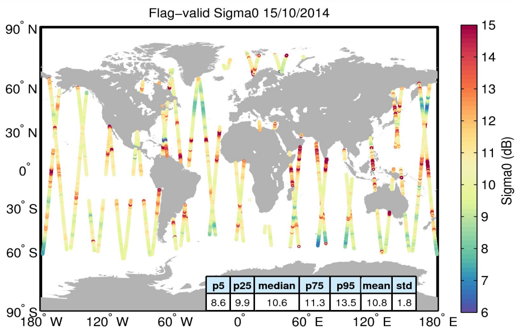
Figure 23. Geographical distribution of flag-valid sigma0 data over oceans and lakes for 15/10/2014. The statistical values shown in the table refer to the sigma0 in dB and are calculated over all measurements shown in the figure.
