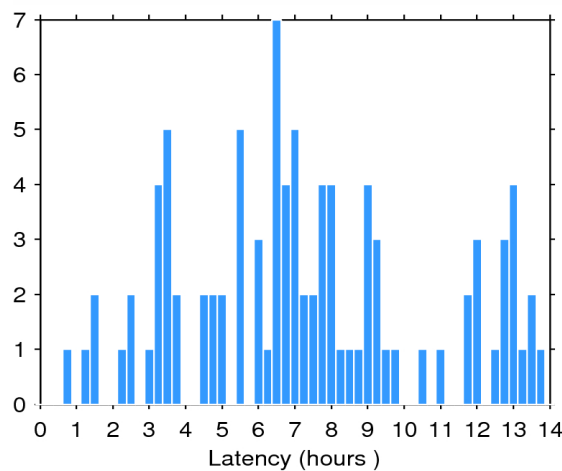
Figure 2. Histogram of the data latency for 15/10/2014. The y-axis denotes the number of files that are made available with a delay of x-hours with respect to the mean time of the records stored in the file.
