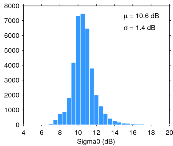
Figure 28. Histogram of science-valid sigma0 over oceans and lakes for 15/10/2014. The mean ( \mu ) and standard deviation ( \sigma ) are also shown. Note that values outside [4 20] dB are excluded from the histogram for the sake of readability but not from the computation of \mu and \sigma .
