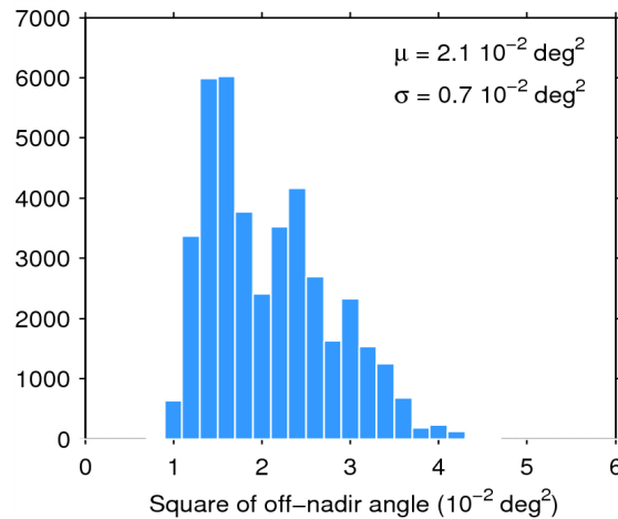
Figure 39. Histogram of flag-valid mispointing over oceans and lakes for 14/10/2014. The mean ( \mu ) and standard deviation ( \sigma ) are also shown. Note that values than 6 \cdot 10^{-2} \text{ deg}^2 are excluded from the histogram for the sake of readability but not from the computation of \mu and \sigma .
