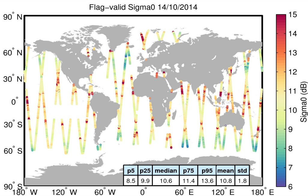
Figure 23. Geographical distribution of flag-valid sigma0 data over oceans and lakes for 14/10/2014. The statistical values shown in the table refer to the sigma0 in dB and are calculated over all measurements shown in the figure.
