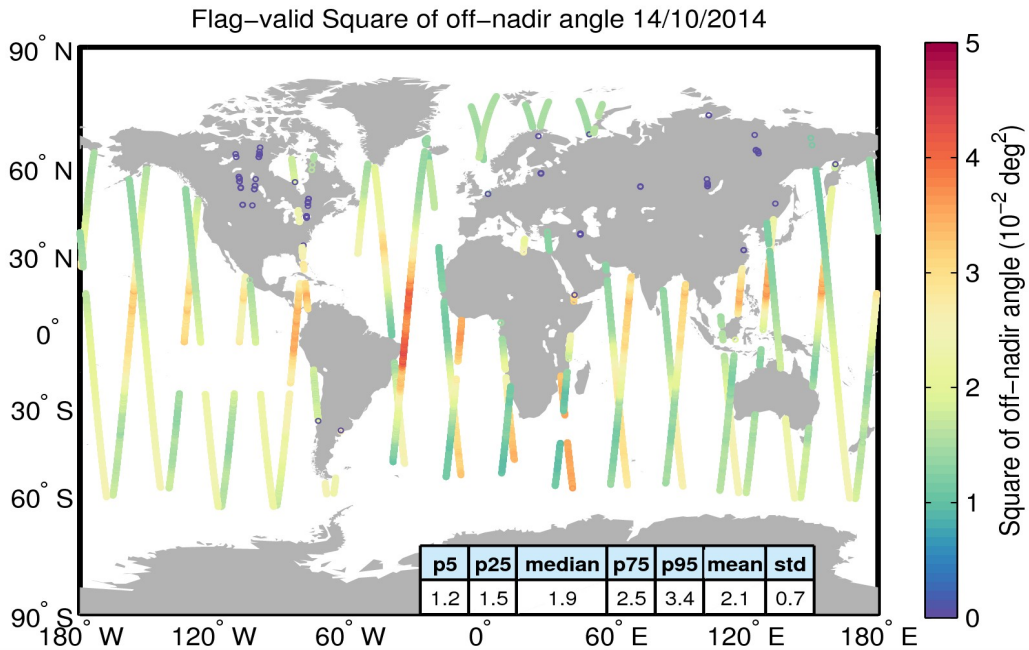
Figure 37. Geographical distribution of flag-valid mispointing data over oceans and lakes for 14/10/2014. The statistical values shown in the table refer to the mispointing in 10^{-2} deg 2 and are calculated over all measurements shown in the figure.
