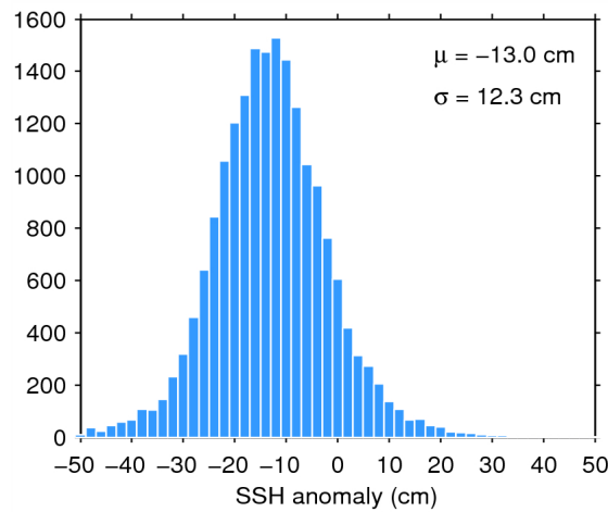
Figure 11. Histogram of science-valid SSH anomaly over oceans and lakes for 14/10/2014. The mean ( \mu ) and standard deviation ( \sigma ) are also shown. Note that values outside [-50 50] cm are excluded from the histogram for the sake of readability but not from the computation of \mu and \sigma .
