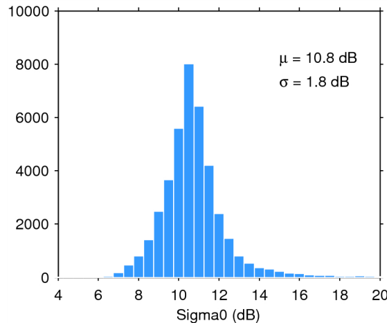
Figure 25. Histogram of flag-valid sigma0 over oceans and lakes for 14/10/2014. The mean ( \mu ) and standard deviation ( \sigma ) are also shown. Note that values outside [4 20] dB are excluded from the histogram for the sake of readability but not from the computation of \mu and \sigma .
