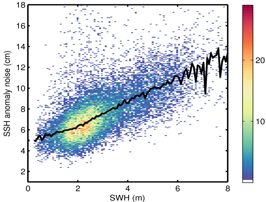
Figure 9. 2D histogram showing flag-valid SSH anomaly noise as a function of SWH for 14/10/2014. The black line denotes the median SSH anomaly as a function of SWH.
