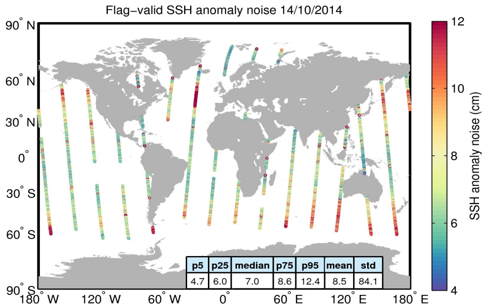
Figure 8. Geographical distribution of flag-valid 20-Hz SSH anomaly measurement noise over oceans and lakes for 14/10/2014. The statistical values shown in the table refer to the SSH anomaly noise and are calculated over all measurements shown in the figure.
