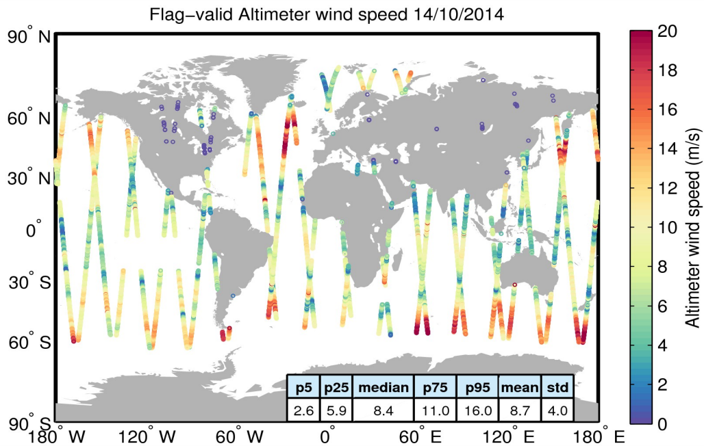
Figure 31. Geographical distribution of flag-valid wind data over oceans and lakes for 14/10/2014. The statistical values shown in the table refer to the wind in m/s and are calculated over all measurements shown in the figure.
