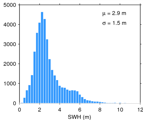
Figure 17. Histogram of flag-valid SWH over oceans and lakes for 14/10/2014. The mean ( \mu ) and standard deviation ( \sigma ) are also shown. Note that values larger than 12 m are excluded from the histogram for the sake of readability but not from the computation of \mu and \sigma .
