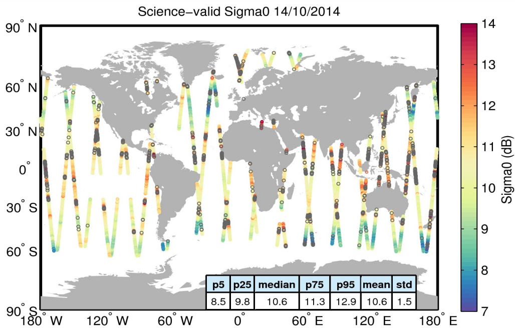
Figure 27. Geographical distribution of science-valid sigma0 data over oceans and lakes for 14/10/2014. The statistical values shown in the table refer to the sigma0 in dB and are calculated over all measurements shown in the figure. Gray circles denote records that have been rejected based on the editing criteria described in Table 4.
