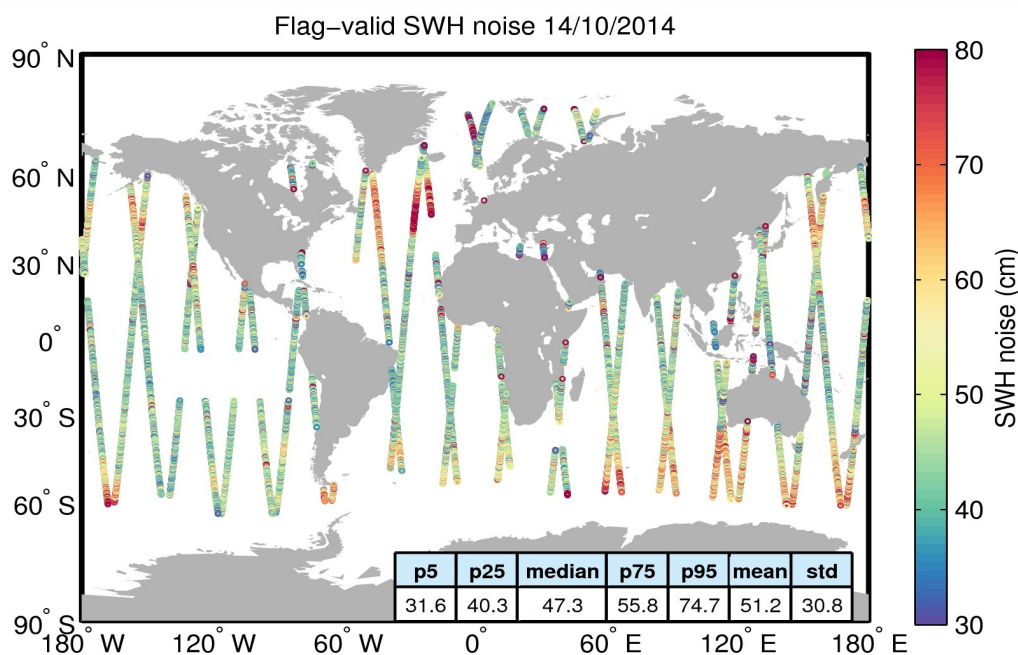
Figure 18. Geographical distribution of flag-valid 20-Hz SWH measurement noise over oceans and lakes for 14/10/2014. The statistical values shown in the figure refer to the SWH noise and are calculated over all measurements shown in the figure.
