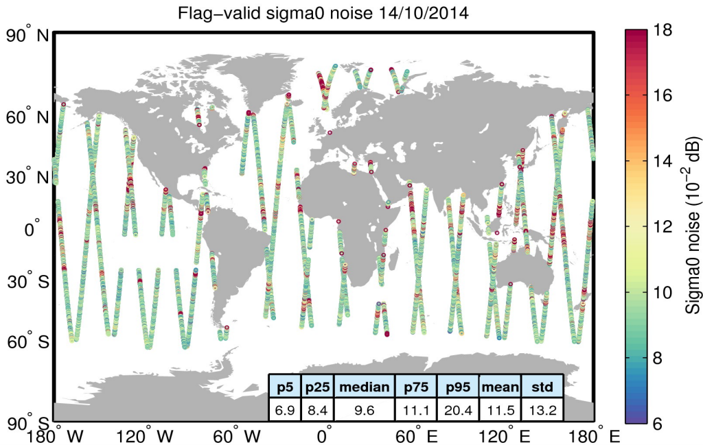
Figure 26. Geographical distribution of flag-valid 20-Hz sigma0 measurement noise over oceans and lakes for 14/10/2014. The statistical values shown in the table refer to the sigma0 noise and are calculated over all measurements shown in the figure.
