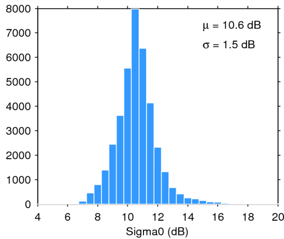
Figure 28. Histogram of science-valid sigma0 over oceans and lakes for 14/10/2014. The mean ( \mu ) and standard deviation ( \sigma ) are also shown. Note that values outside [4 20] dB are excluded from the histogram for the sake of readability but not from the computation of \mu and \sigma .
