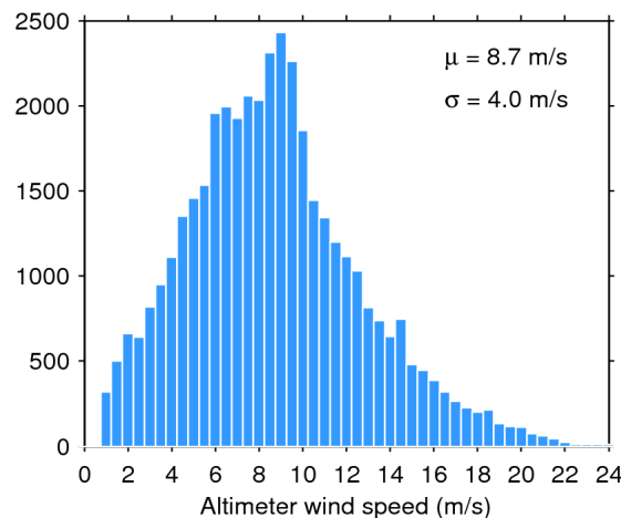
Figure 35. Histogram of science-valid wind over oceans and lakes for 14/10/2014. The mean ( \mu ) and standard deviation ( \sigma ) are also shown. Note that values larger than 24 m/s are excluded from the histogram for the sake of readability but not from the computation of \mu and \sigma .
