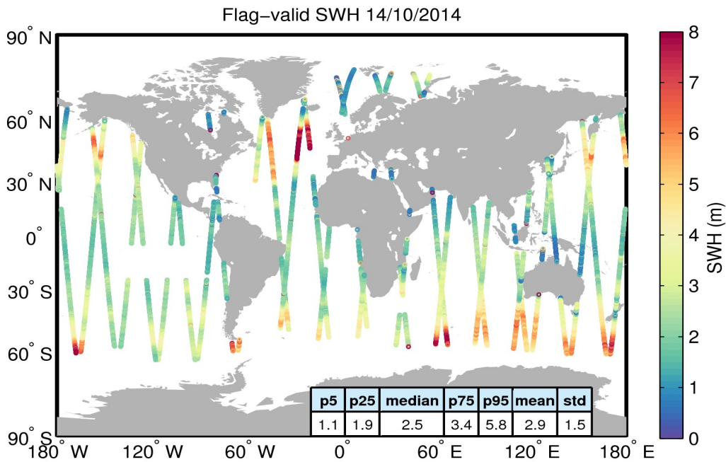
Figure 15. Geographical distribution of flag-valid SWH data over oceans and lakes for 14/10/2014. The statistical values shown in the table refer to the SWH in m and are calculated over all measurements shown in the figure.
