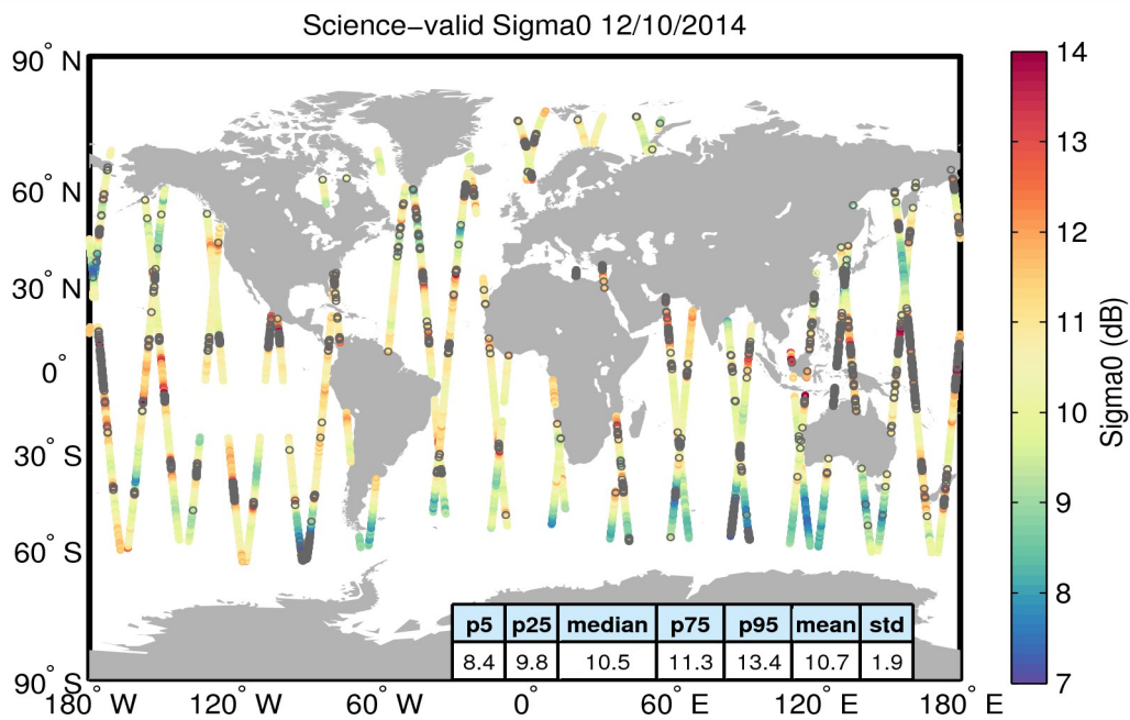
Figure 27. Geographical distribution of science-valid sigma0 data over oceans and lakes for 12/10/2014. The statistical values shown in the table refer to the sigma0 in dB and are calculated over all measurements shown in the figure. Gray circles denote records that have been rejected based on the editing criteria described in Table 4.
