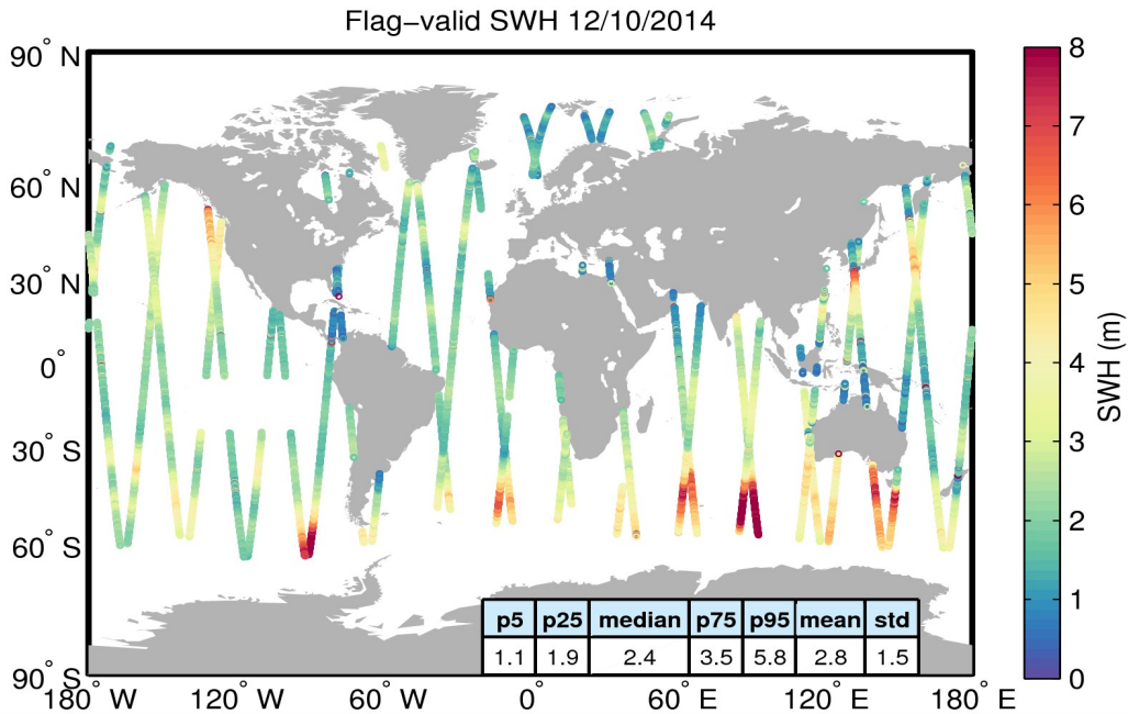
Figure 15. Geographical distribution of flag-valid SWH data over oceans and lakes for 12/10/2014. The statistical values shown in the table refer to the SWH in m and are calculated over all measurements shown in the figure.
