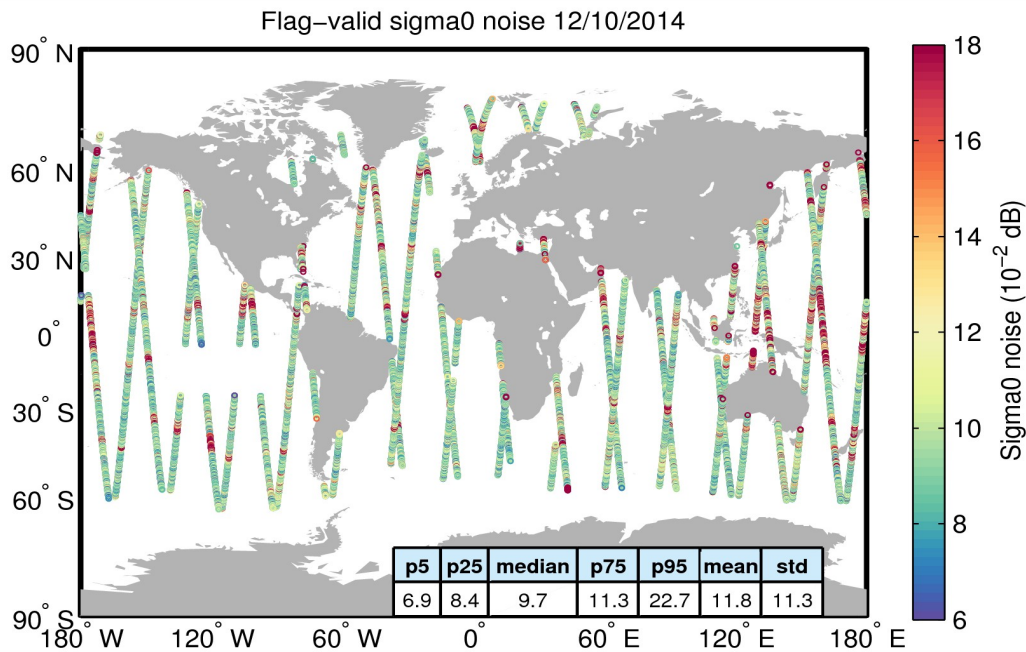
Figure 26. Geographical distribution of flag-valid 20-Hz sigma0 measurement noise over oceans and lakes for 12/10/2014. The statistical values shown in the table refer to the sigma0 noise and are calculated over all measurements shown in the figure.
