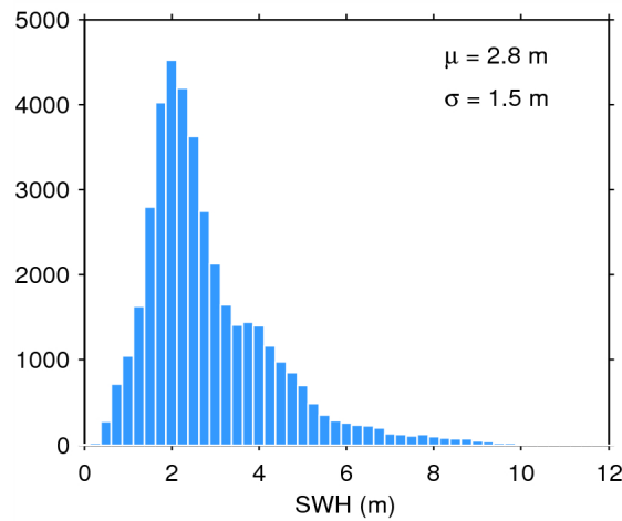
Figure 17. Histogram of flag-valid SWH over oceans and lakes for 12/10/2014. The mean ( \mu ) and standard deviation ( \sigma ) are also shown. Note that values larger than 12 m are excluded from the histogram for the sake of readability but not from the computation of \mu and \sigma .
