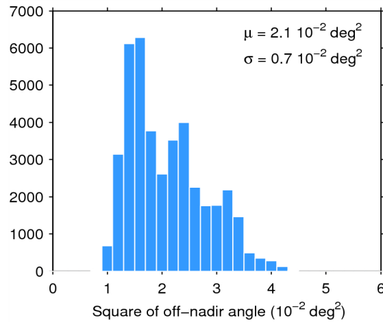
Figure 39. Histogram of flag-valid mispointing over oceans and lakes for 12/10/2014. The mean ( \mu ) and standard deviation ( \sigma ) are also shown. Note that values than 6 \cdot 10^{-2} \text{ deg}^2 are excluded from the histogram for the sake of readability but not from the computation of \mu and \sigma .
