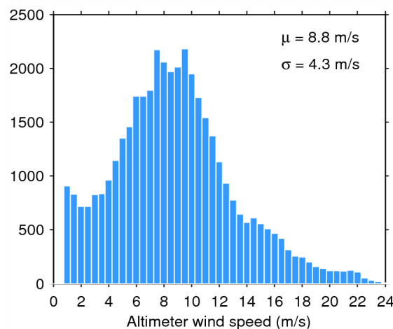
Figure 35. Histogram of science-valid wind over oceans and lakes for 12/10/2014. The mean ( \mu ) and standard deviation ( \sigma ) are also shown. Note that values larger than 24 m/s are excluded from the histogram for the sake of readability but not from the computation of \mu and \sigma .
