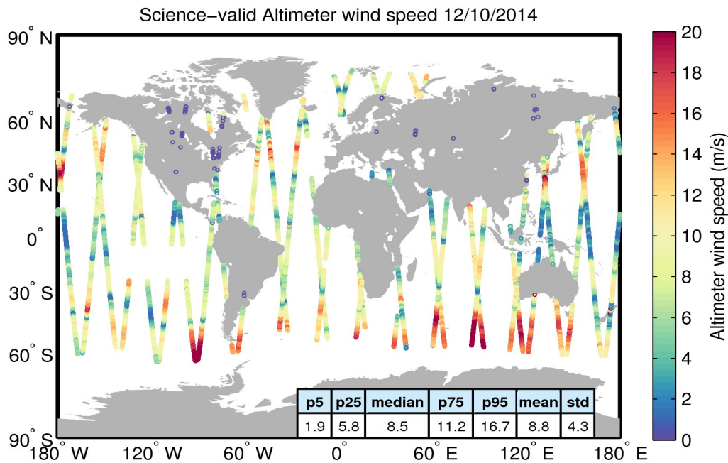
Figure 34. Geographical distribution of science-valid wind data over oceans and lakes for 12/10/2014. The statistical values shown in the table refer to the wind in m/s and are calculated over all measurements shown in the figure. Gray circles denote records that have been rejected based on the editing criteria described in Table 5.
