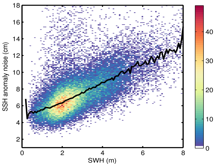
Figure 9. 2D histogram showing flag-valid SSH anomaly noise as a function of SWH for 12/10/2014. The black line denotes the median SSH anomaly as a function of SWH.
