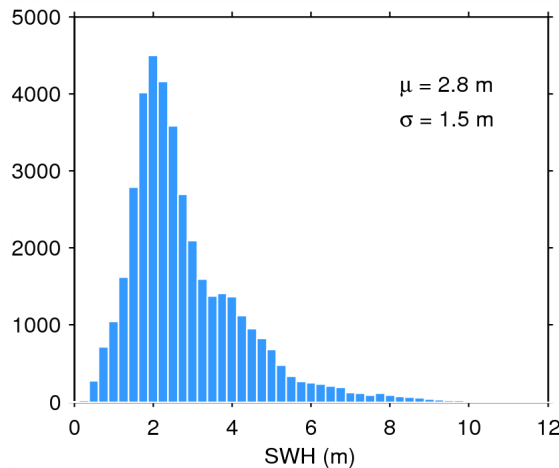
Figure 20. Histogram of science-valid SWH over oceans and lakes for 12/10/2014. The mean ( \mu ) and standard deviation ( \sigma ) are also shown. Note that values larger than 12 m are excluded from the histogram for the sake of readability but not from the computation of \mu and \sigma .
