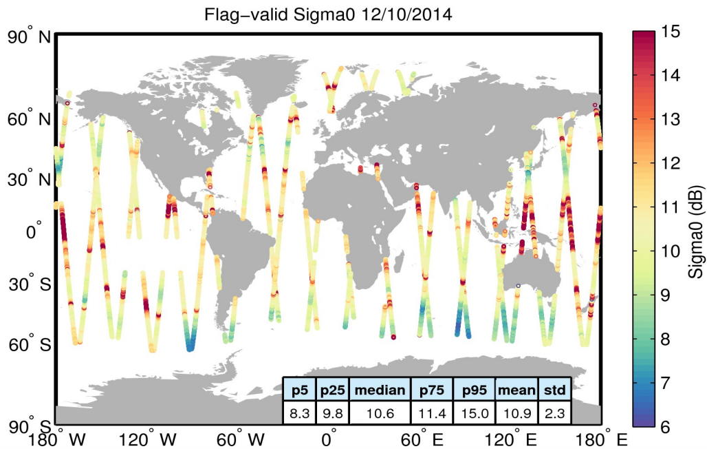
Figure 23. Geographical distribution of flag-valid sigma0 data over oceans and lakes for 12/10/2014. The statistical values shown in the table refer to the sigma0 in dB and are calculated over all measurements shown in the figure.
