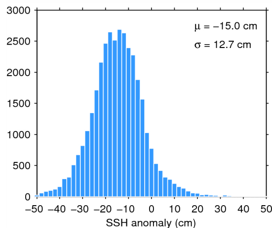
Figure 11. Histogram of science-valid SSH anomaly over oceans and lakes for 12/10/2014. The mean ( \mu ) and standard deviation ( \sigma ) are also shown. Note that values outside [-50 50] cm are excluded from the histogram for the sake of readability but not from the computation of \mu and \sigma .
