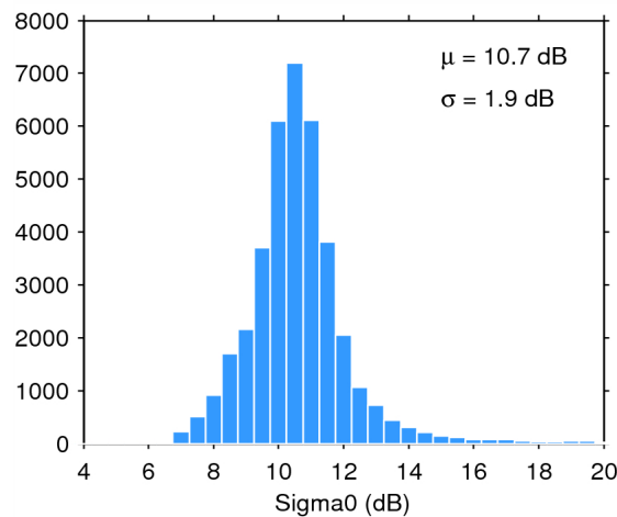
Figure 28. Histogram of science-valid sigma0 over oceans and lakes for 12/10/2014. The mean ( \mu ) and standard deviation ( \sigma ) are also shown. Note that values outside [4 20] dB are excluded from the histogram for the sake of readability but not from the computation of \mu and \sigma .
