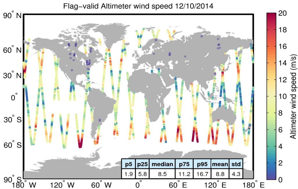
Figure 31. Geographical distribution of flag-valid wind data over oceans and lakes for 12/10/2014. The statistical values shown in the table refer to the wind in m/s and are calculated over all measurements shown in the figure.
