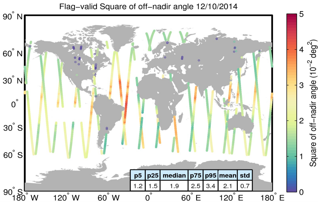
Figure 37. Geographical distribution of flag-valid mispointing data over oceans and lakes for 12/10/2014. The statistical values shown in the table refer to the mispointing in 10^{-2} \text{ deg}^2 and are calculated over all measurements shown in the figure.
