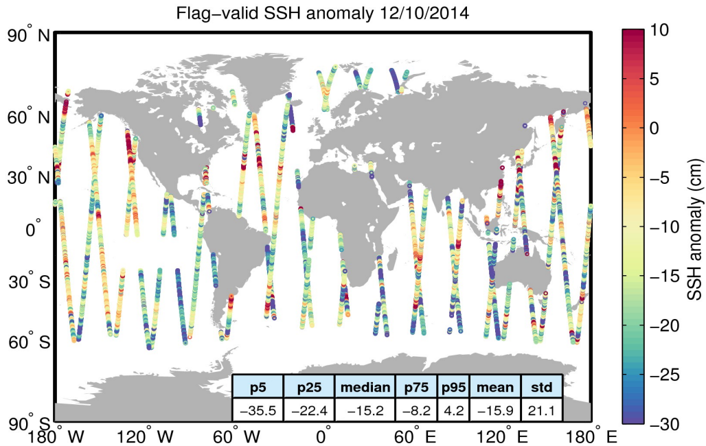
Figure 5. Geographical distribution of flag-valid 1-Hz SSH anomaly data over oceans and lakes for 12/10/2014. The statistical values shown in the table refer to the SSH anomaly in cm and are calculated over all measurements shown in the figure.
