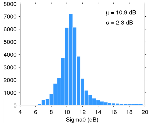
Figure 25. Histogram of flag-valid sigma0 over oceans and lakes for 12/10/2014. The mean ( \mu ) and standard deviation ( \sigma ) are also shown. Note that values outside [4 20] dB are excluded from the histogram for the sake of readability but not from the computation of \mu and \sigma .
