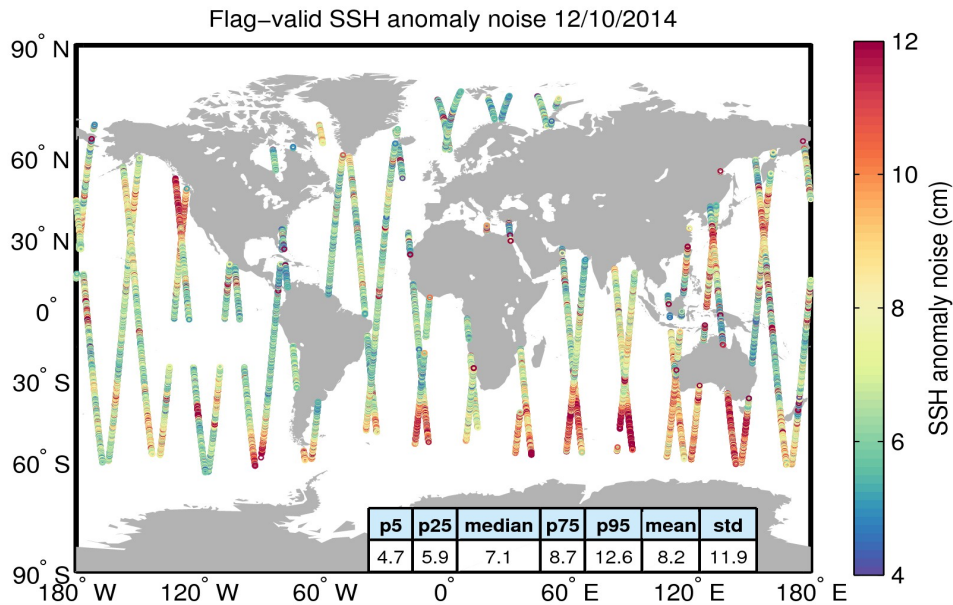
Figure 8. Geographical distribution of flag-valid 20-Hz SSH anomaly measurement noise over oceans and lakes for 12/10/2014. The statistical values shown in the table refer to the SSH anomaly noise and are calculated over all measurements shown in the figure.
