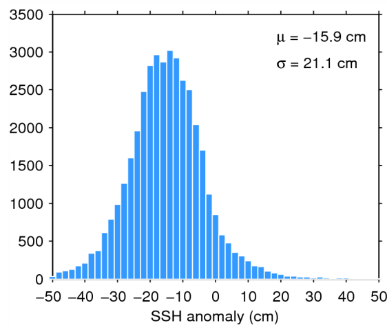
Figure 7. Histogram of flag-valid SSH anomaly over oceans and lakes for 12/10/2014. The mean ( \mu ) and standard deviation ( \sigma ) are also shown. Note that values outside [-50 50] cm are excluded from the histogram for the sake of readability but not from the computation of \mu and \sigma .
