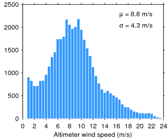
Figure 33. Histogram of flag-valid wind over oceans and lakes for 12/10/2014. The mean ( \mu ) and standard deviation ( \sigma ) are also shown. Note that values larger than 24 m/s are excluded from the histogram for the sake of readability but not from the computation of \mu and \sigma .
