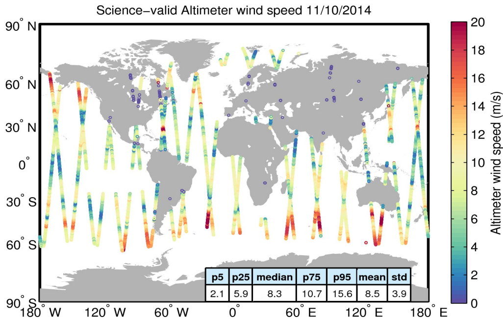
Figure 34. Geographical distribution of science-valid wind data over oceans and lakes for 11/10/2014. The statistical values shown in the table refer to the wind in m/s and are calculated over all measurements shown in the figure. Gray circles denote records that have been rejected based on the editing criteria described in Table 5.
