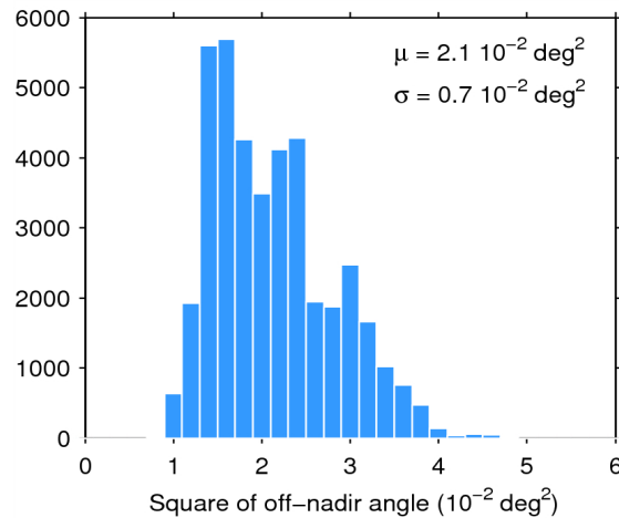
Figure 39. Histogram of flag-valid mispointing over oceans and lakes for 11/10/2014. The mean ( \mu ) and standard deviation ( \sigma ) are also shown. Note that values than 6 \cdot 10^{-2} \text{ deg}^2 are excluded from the histogram for the sake of readability but not from the computation of \mu and \sigma .
