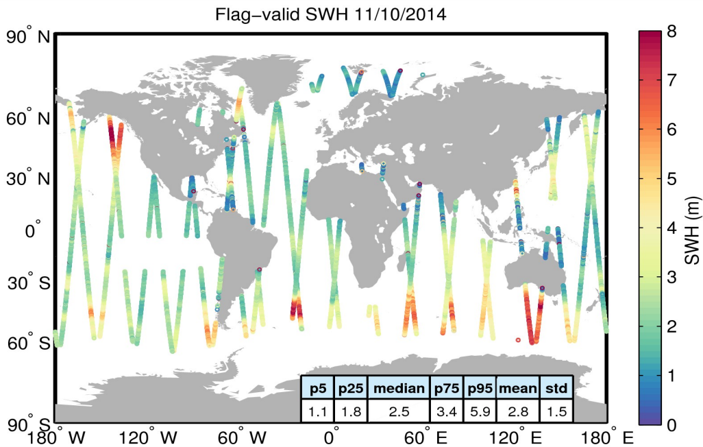
Figure 15. Geographical distribution of flag-valid SWH data over oceans and lakes for 11/10/2014. The statistical values shown in the table refer to the SWH in m and are calculated over all measurements shown in the figure.
