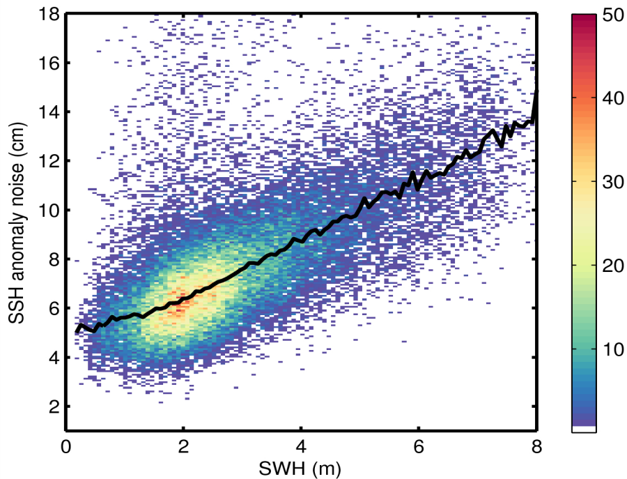
Figure 9. 2D histogram showing flag-valid SSH anomaly noise as a function of SWH for 11/10/2014. The black line denotes the median SSH anomaly as a function of SWH.
