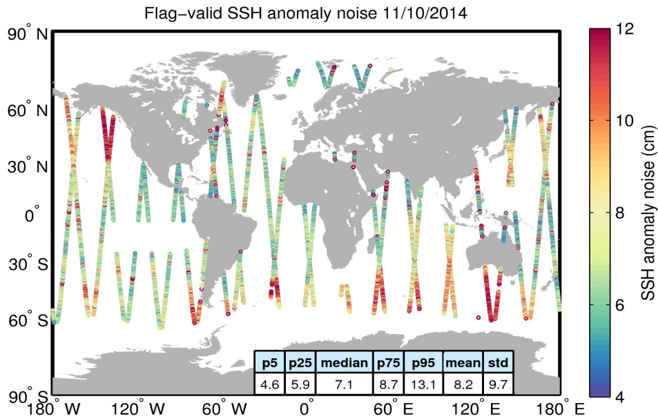
Figure 8. Geographical distribution of flag-valid 20-Hz SSH anomaly measurement noise over oceans and lakes for 11/10/2014. The statistical values shown in the table refer to the SSH anomaly noise and are calculated over all measurements shown in the figure.
