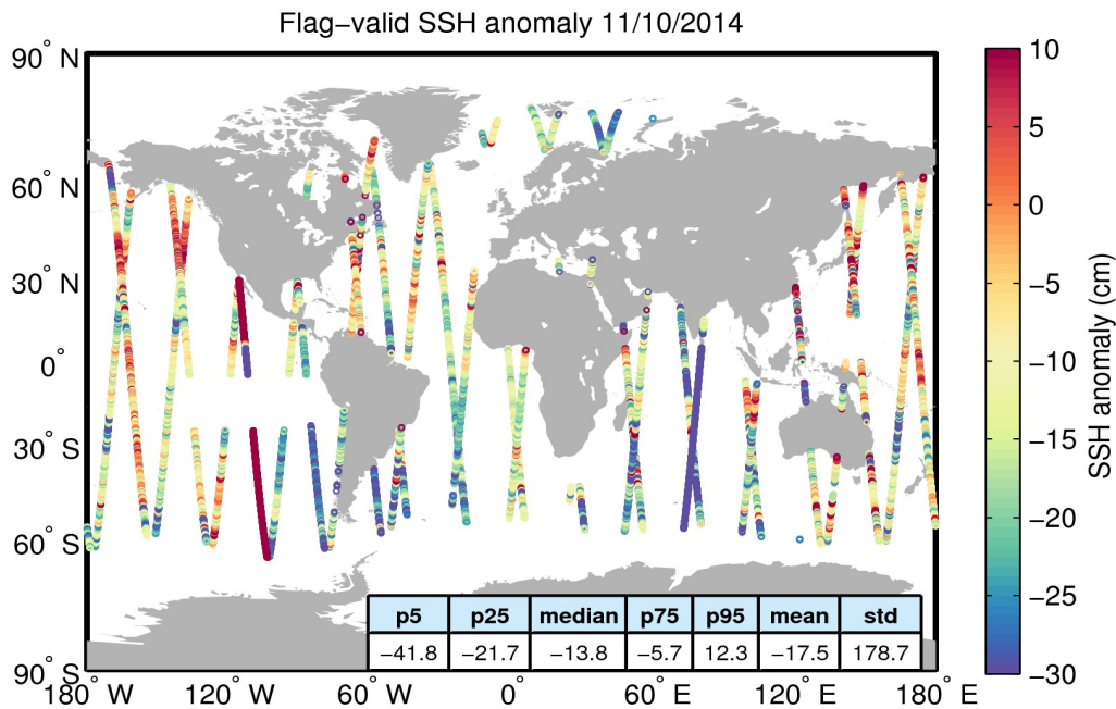
Figure 5. Geographical distribution of flag-valid 1-Hz SSH anomaly data over oceans and lakes for 11/10/2014. The statistical values shown in the table refer to the SSH anomaly in cm and are calculated over all measurements shown in the figure.
