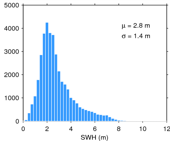
Figure 20. Histogram of science-valid SWH over oceans and lakes for 11/10/2014. The mean ( \mu ) and standard deviation ( \sigma ) are also shown. Note that values larger than 12 m are excluded from the histogram for the sake of readability but not from the computation of \mu and \sigma .
