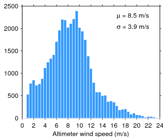
Figure 35. Histogram of science-valid wind over oceans and lakes for 11/10/2014. The mean ( \mu ) and standard deviation ( \sigma ) are also shown. Note that values larger than 24 m/s are excluded from the histogram for the sake of readability but not from the computation of \mu and \sigma .
