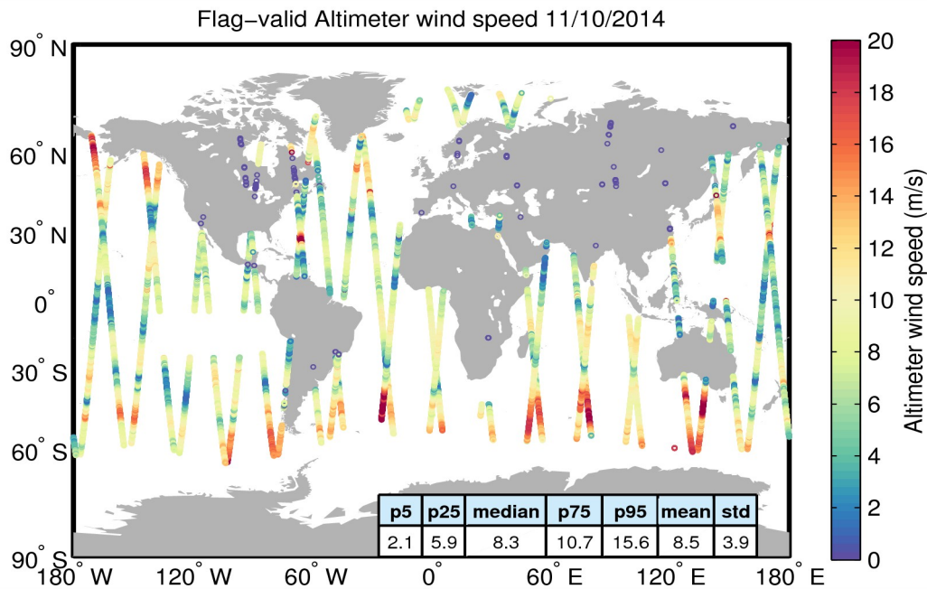
Figure 31. Geographical distribution of flag-valid wind data over oceans and lakes for 11/10/2014. The statistical values shown in the figure refer to the wind in m/s and are calculated over all measurements shown in the figure.
