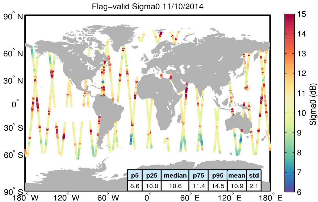
Figure 23. Geographical distribution of flag-valid sigma0 data over oceans and lakes for 11/10/2014. The statistical values shown in the table refer to the sigma0 in dB and are calculated over all measurements shown in the figure.
