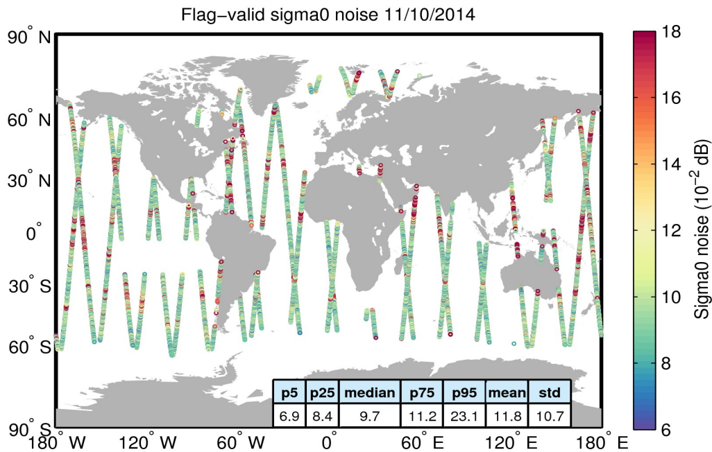
Figure 26. Geographical distribution of flag-valid 20-Hz sigma0 measurement noise over oceans and lakes for 11/10/2014. The statistical values shown in the table refer to the sigma0 noise and are calculated over all measurements shown in the figure.
