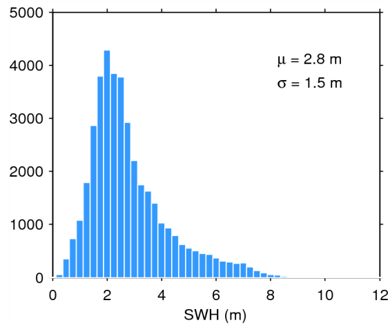
Figure 17. Histogram of flag-valid SWH over oceans and lakes for 11/10/2014. The mean ( \mu ) and standard deviation ( \sigma ) are also shown. Note that values larger than 12 m are excluded from the histogram for the sake of readability but not from the computation of \mu and \sigma .
