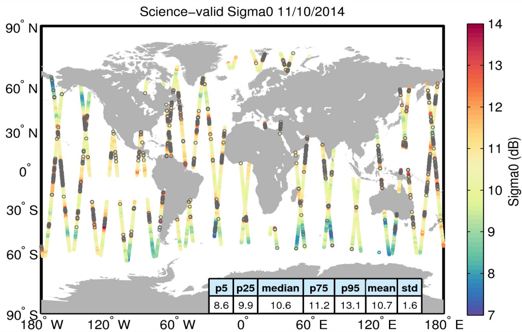
Figure 27. Geographical distribution of science-valid sigma0 data over oceans and lakes for 11/10/2014. The statistical values shown in the table refer to the sigma0 in dB and are calculated over all measurements shown in the figure. Gray circles denote records that have been rejected based on the editing criteria described in Table 4.
