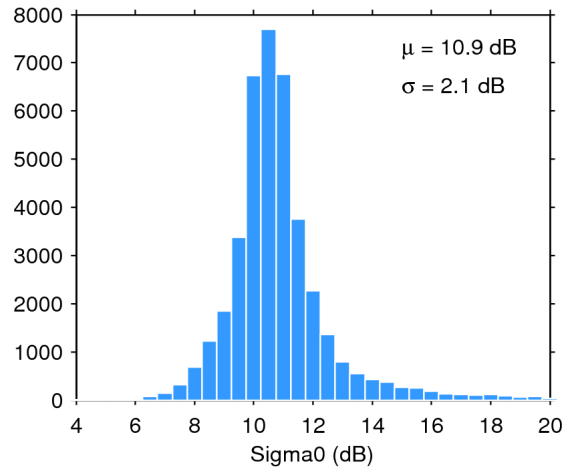
Figure 25. Histogram of flag-valid sigma0 over oceans and lakes for 11/10/2014. The mean ( \mu ) and standard deviation ( \sigma ) are also shown. Note that values outside [4 20] dB are excluded from the histogram for the sake of readability but not from the computation of \mu and \sigma .
