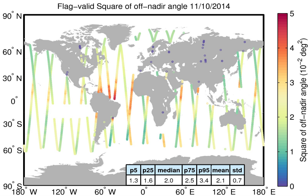
Figure 37. Geographical distribution of flag-valid mispointing data over oceans and lakes for 11/10/2014. The statistical values shown in the table refer to the mispointing in 10^{-2} \text{deg}^2 and are calculated over all measurements shown in the figure.
