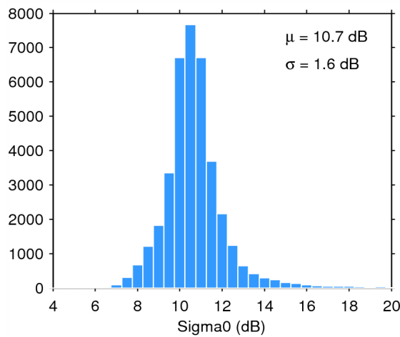
Figure 28. Histogram of science-valid sigma0 over oceans and lakes for 11/10/2014. The mean ( \mu ) and standard deviation ( \sigma ) are also shown. Note that values outside [4 20] dB are excluded from the histogram for the sake of readability but not from the computation of \mu and \sigma .
