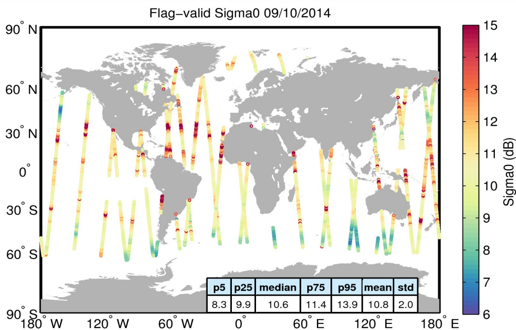
Figure 23. Geographical distribution of flag-valid sigma0 data over oceans and lakes for 09/10/2014. The statistical values shown in the table refer to the sigma0 in dB and are calculated over all measurements shown in the figure.
