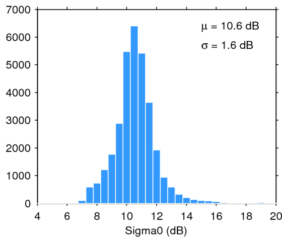
Figure 28. Histogram of science-valid sigma0 over oceans and lakes for 09/10/2014. The mean ( \mu ) and standard deviation ( \sigma ) are also shown. Note that values outside [4 20] dB are excluded from the histogram for the sake of readability but not from the computation of \mu and \sigma .
