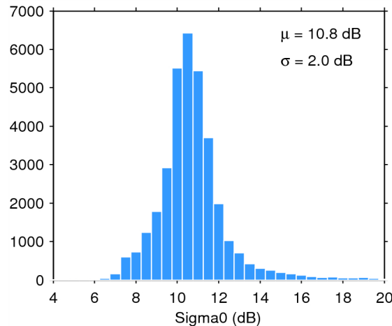
Figure 25. Histogram of flag-valid sigma0 over oceans and lakes for 09/10/2014. The mean ( \mu ) and standard deviation ( \sigma ) are also shown. Note that values outside [4 20] dB are excluded from the histogram for the sake of readability but not from the computation of \mu and \sigma .
