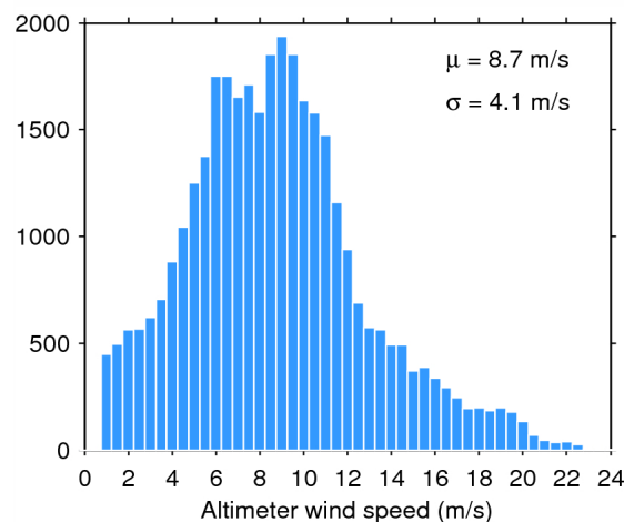
Figure 35. Histogram of science-valid wind over oceans and lakes for 09/10/2014. The mean ( \mu ) and standard deviation ( \sigma ) are also shown. Note that values larger than 24 m/s are excluded from the histogram for the sake of readability but not from the computation of \mu and \sigma .
