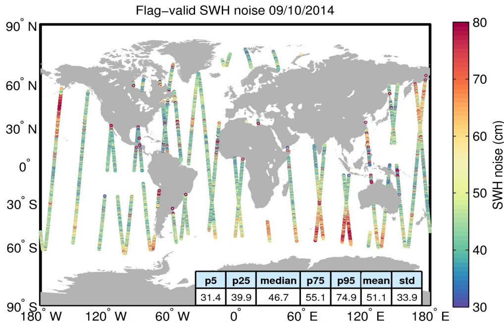
Figure 18. Geographical distribution of flag-valid 20-Hz SWH measurement noise over oceans and lakes for 09/10/2014. The statistical values shown in the figure refer to the SWH noise and are calculated over all measurements shown in the figure.
