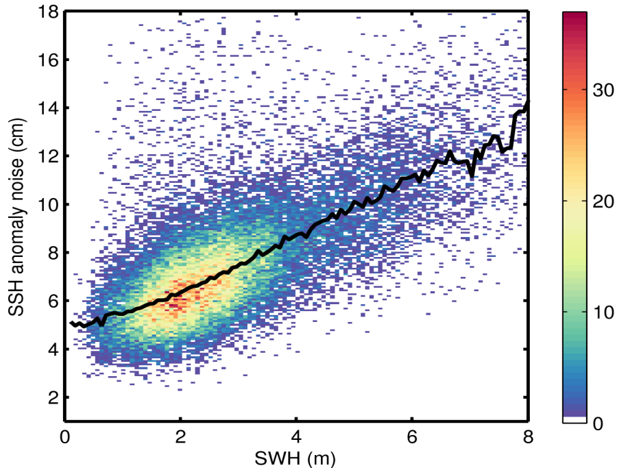
Figure 9. 2D histogram showing flag-valid SSH anomaly noise as a function of SWH for 09/10/2014. The black line denotes the median SSH anomaly as a function of SWH.
