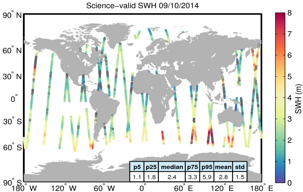
Figure 19. Geographical distribution of science-valid SWH data over oceans and lakes for 09/10/2014. The statistical values shown in the table refer to the SWH in m and are calculated over all measurements shown in the figure. Gray circles denote records that have been rejected based on the editing criteria described in Table 3.
