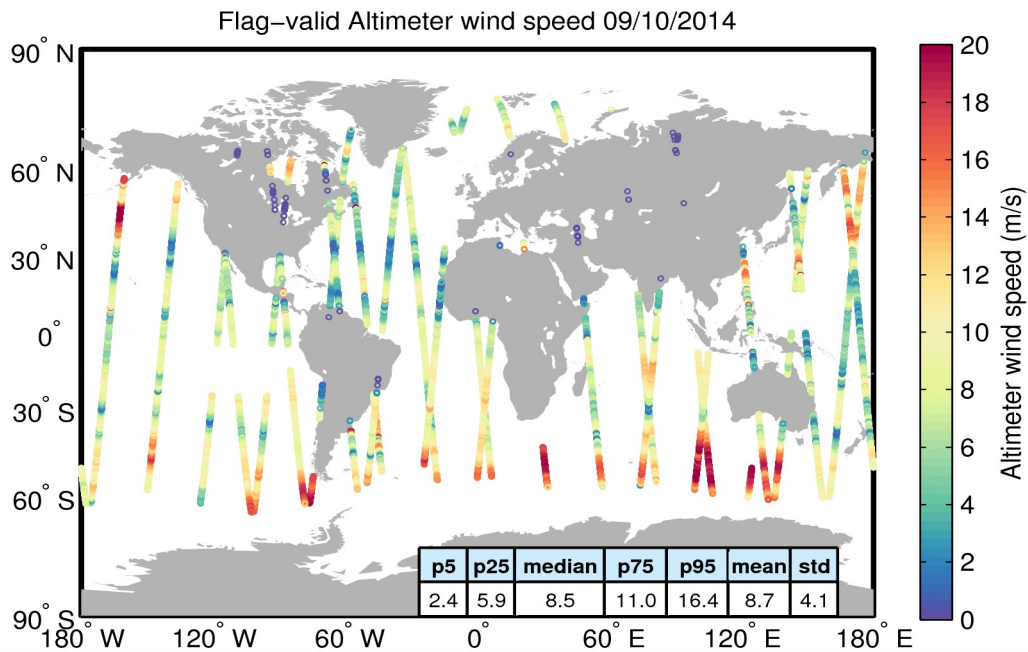
Figure 31. Geographical distribution of flag-valid wind data over oceans and lakes for 09/10/2014. The statistical values shown in the table refer to the wind in m/s and are calculated over all measurements shown in the figure.
