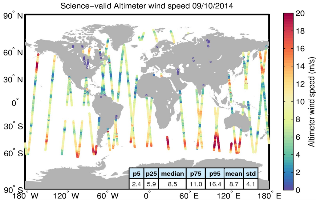
Figure 34. Geographical distribution of science-valid wind data over oceans and lakes for 09/10/2014. The statistical values shown in the table refer to the wind in m/s and are calculated over all measurements shown in the figure. Gray circles denote records that have been rejected based on the editing criteria described in Table 5.
