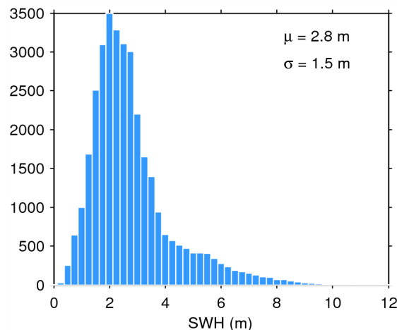
Figure 20. Histogram of science-valid SWH over oceans and lakes for 09/10/2014. The mean ( \mu ) and standard deviation ( \sigma ) are also shown. Note that values larger than 12 m are excluded from the histogram for the sake of readability but not from the computation of \mu and \sigma .
