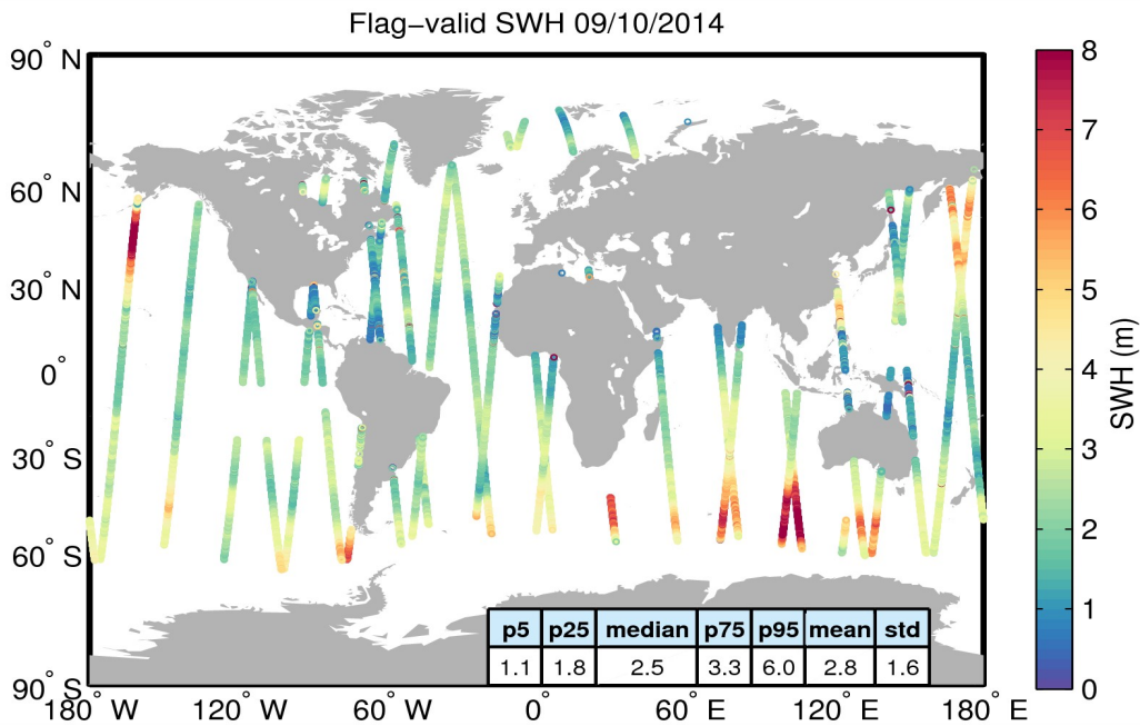
Figure 15. Geographical distribution of flag-valid SWH data over oceans and lakes for 09/10/2014. The statistical values shown in the table refer to the SWH in m and are calculated over all measurements shown in the figure.
