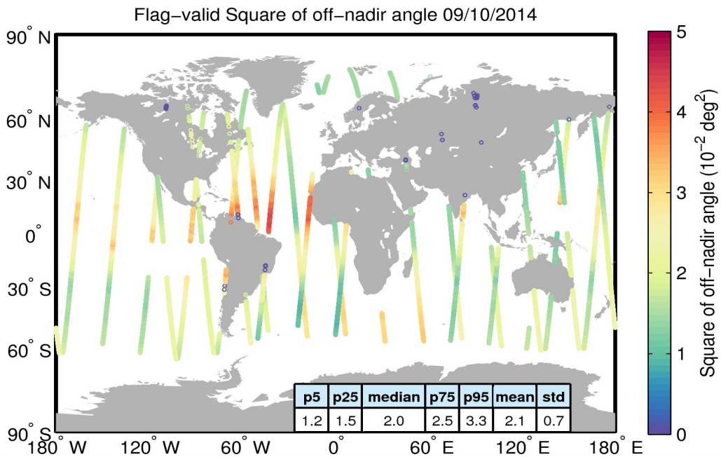
Figure 37. Geographical distribution of flag-valid mispointing data over oceans and lakes for 09/10/2014. The statistical values shown in the table refer to the mispointing in 10^{-2} \text{ deg}^2 and are calculated over all measurements shown in the figure.
