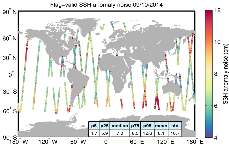
Figure 8. Geographical distribution of flag-valid 20-Hz SSH anomaly measurement noise over oceans and lakes for 09/10/2014. The statistical values shown in the table refer to the SSH anomaly noise and are calculated over all measurements shown in the figure.
