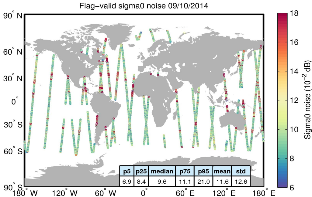
Figure 26. Geographical distribution of flag-valid 20-Hz sigma0 measurement noise over oceans and lakes for 09/10/2014. The statistical values shown in the table refer to the sigma0 noise and are calculated over all measurements shown in the figure.
