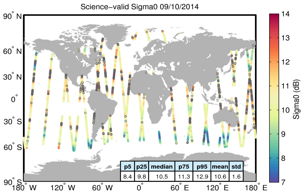
Figure 27. Geographical distribution of science-valid sigma0 data over oceans and lakes for 09/10/2014. The statistical values shown in the figure are calculated over all measurements shown in the figure. Gray circles denote records that have been rejected based on the editing criteria described in Table 4.
