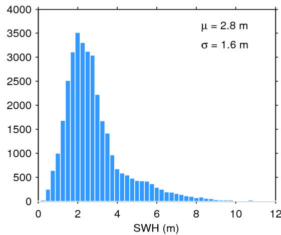
Figure 17. Histogram of flag-valid SWH over oceans and lakes for 09/10/2014. The mean ( \mu ) and standard deviation ( \sigma ) are also shown. Note that values larger than 12 m are excluded from the histogram for the sake of readability but not from the computation of \mu and \sigma .
