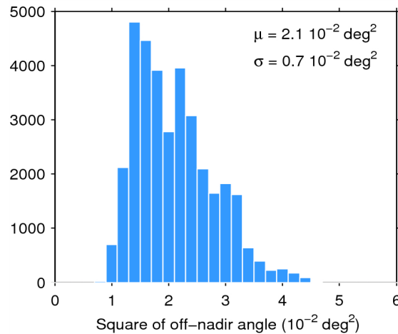
Figure 39. Histogram of flag-valid mispointing over oceans and lakes for 09/10/2014. The mean ( \mu ) and standard deviation ( \sigma ) are also shown. Note that values than 6 \cdot 10^{-2} \text{ deg}^2 are excluded from the histogram for the sake of readability but not from the computation of \mu and \sigma .
