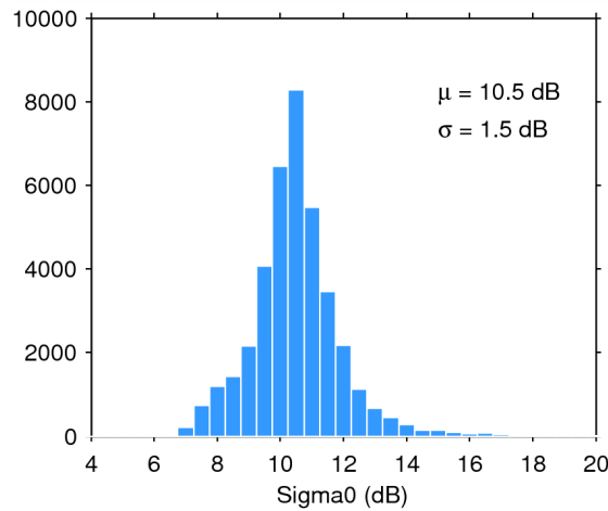
Figure 28. Histogram of science-valid sigma0 over oceans and lakes for 08/10/2014. The mean ( \mu ) and standard deviation ( \sigma ) are also shown. Note that values outside [4 20] dB are excluded from the histogram for the sake of readability but not from the computation of \mu and \sigma .
