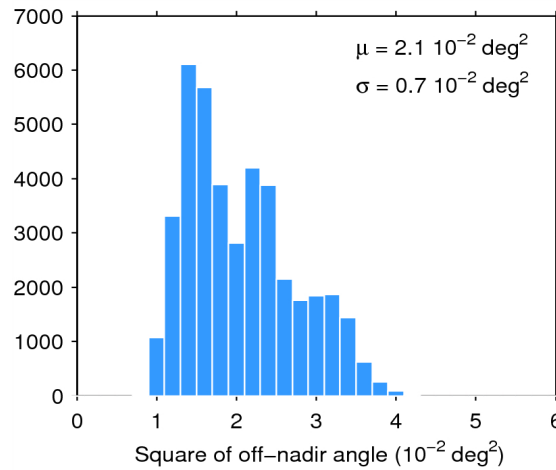
Figure 39. Histogram of flag-valid mispointing over oceans and lakes for 08/10/2014. The mean ( \mu ) and standard deviation ( \sigma ) are also shown. Note that values than 6 \cdot 10^{-2} \text{ deg}^2 are excluded from the histogram for the sake of readability but not from the computation of \mu and \sigma .
