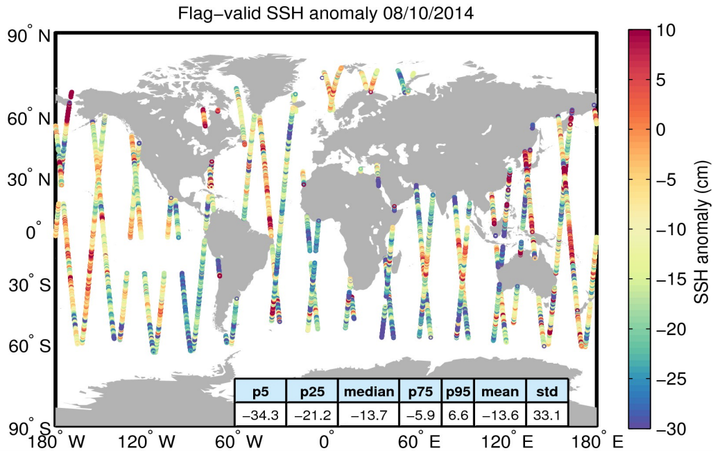
Figure 5. Geographical distribution of flag-valid 1-Hz SSH anomaly data over oceans and lakes for 08/10/2014. The statistical values shown in the table refer to the SSH anomaly in cm and are calculated over all measurements shown in the figure.
