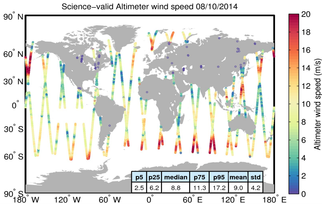
Figure 34. Geographical distribution of science-valid wind data over oceans and lakes for 08/10/2014. The statistical values shown in the table refer to the wind in m/s and are calculated over all measurements shown in the figure. Gray circles denote records that have been rejected based on the editing criteria described in Table 5.
