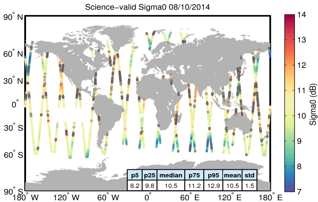
Figure 27. Geographical distribution of science-valid sigma0 data over oceans and lakes for 08/10/2014. The statistical values shown in the table refer to the sigma0 in dB and are calculated over all measurements shown in the figure. Gray circles denote records that have been rejected based on the editing criteria described in Table 4.
