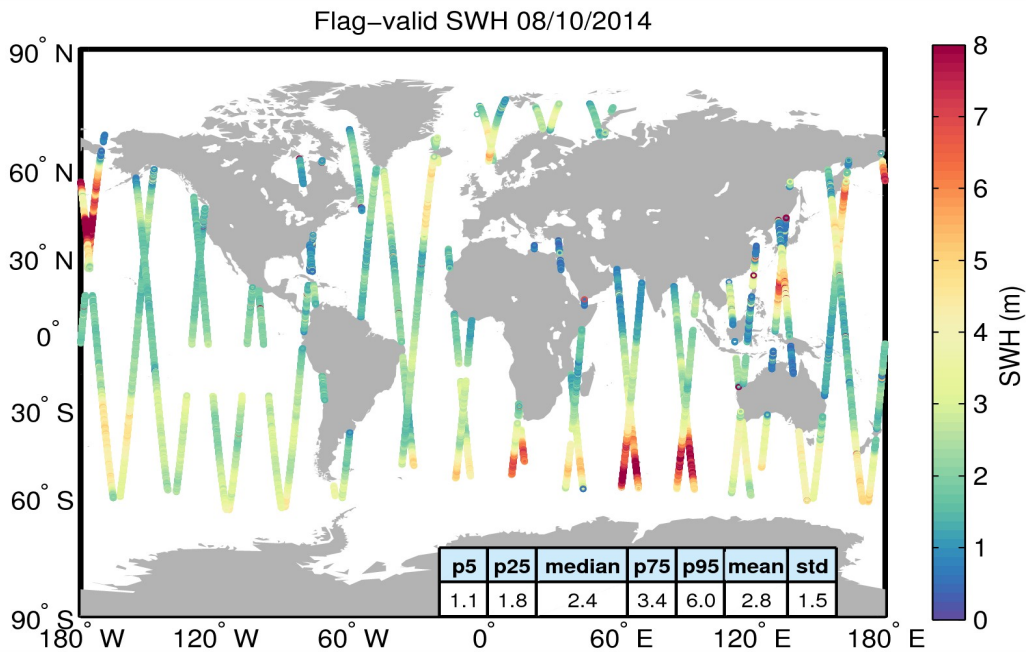
Figure 15. Geographical distribution of flag-valid SWH data over oceans and lakes for 08/10/2014. The statistical values shown in the figure refer to the SWH in m and are calculated over all measurements shown in the figure.
