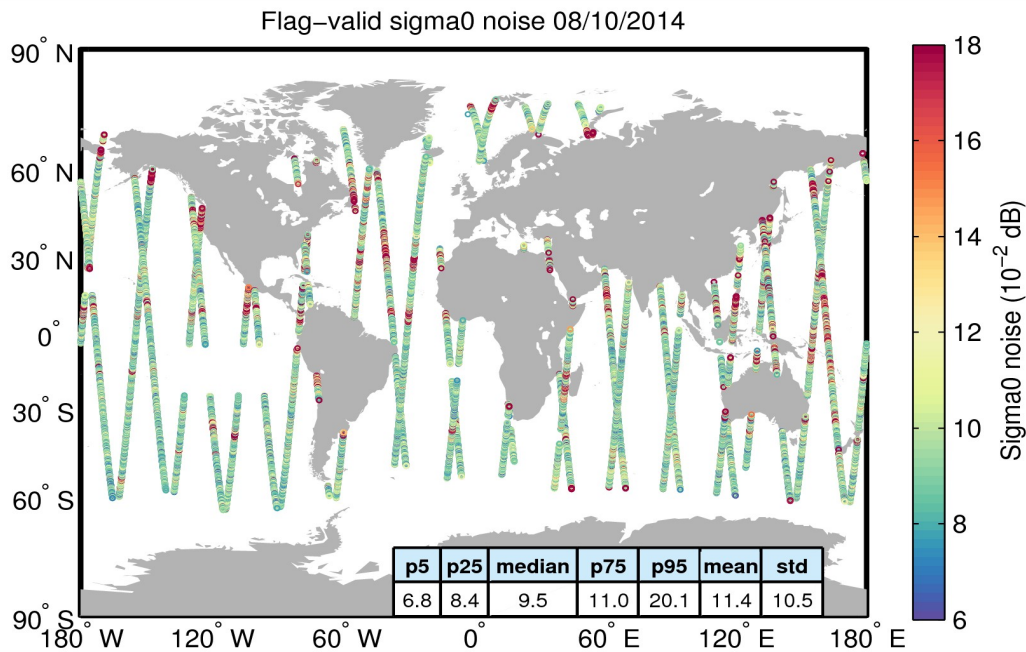
Figure 26. Geographical distribution of flag-valid 20-Hz sigma0 measurement noise over oceans and lakes for 08/10/2014. The statistical values shown in the table refer to the sigma0 noise and are calculated over all measurements shown in the figure.
