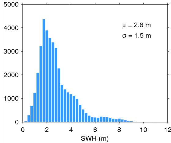
Figure 20. Histogram of science-valid SWH over oceans and lakes for 08/10/2014. The mean ( \mu ) and standard deviation ( \sigma ) are also shown. Note that values larger than 12 m are excluded from the histogram for the sake of readability but not from the computation of \mu and \sigma .
