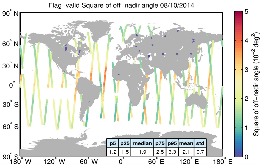
Figure 37. Geographical distribution of flag-valid mispointing data over oceans and lakes for 08/10/2014. The statistical values shown in the table refer to the mispointing in 10^{-2} \text{ deg}^2 and are calculated over all measurements shown in the figure.
