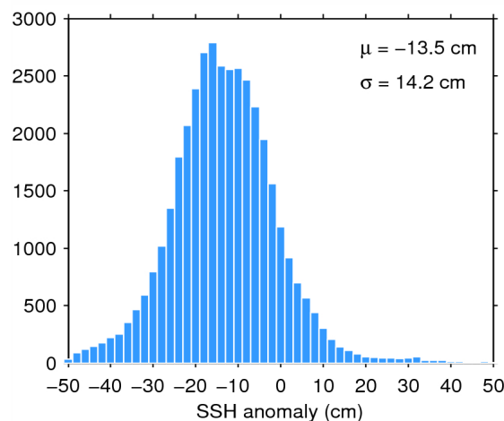
Figure 11. Histogram of science-valid SSH anomaly over oceans and lakes for 08/10/2014. The mean ( \mu ) and standard deviation ( \sigma ) are also shown. Note that values outside [-50 50] cm are excluded from the histogram for the sake of readability but not from the computation of \mu and \sigma .
