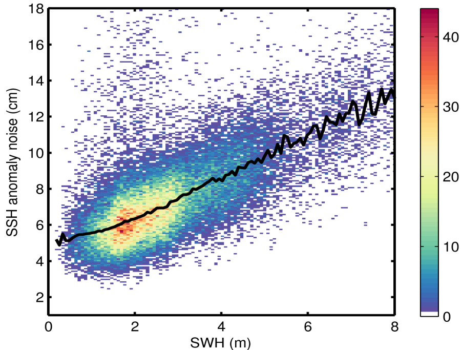
Figure 9. 2D histogram showing flag-valid SSH anomaly noise as a function of SWH for 08/10/2014. The black line denotes the median SSH anomaly as a function of SWH.
