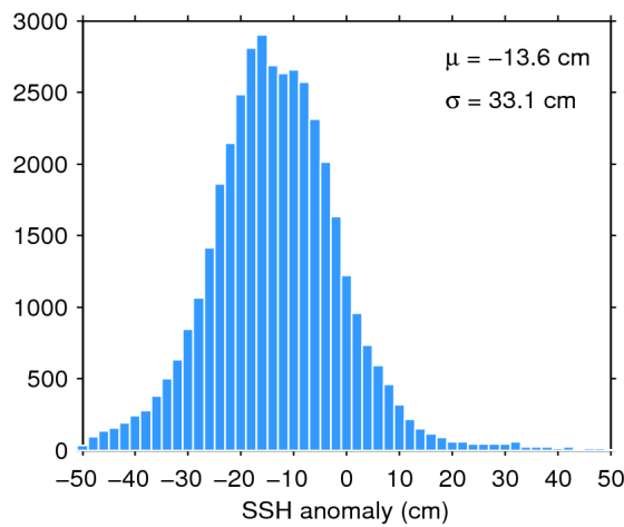
Figure 7. Histogram of flag-valid SSH anomaly over oceans and lakes for 08/10/2014. The mean ( \mu ) and standard deviation ( \sigma ) are also shown. Note that values outside [-50 50] cm are excluded from the histogram for the sake of readability but not from the computation of \mu and \sigma .
