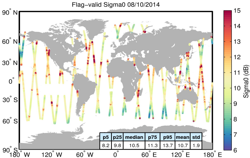
Figure 23. Geographical distribution of flag-valid sigma0 data over oceans and lakes for 08/10/2014. The statistical values shown in the table refer to the sigma0 in dB and are calculated over all measurements shown in the figure.
