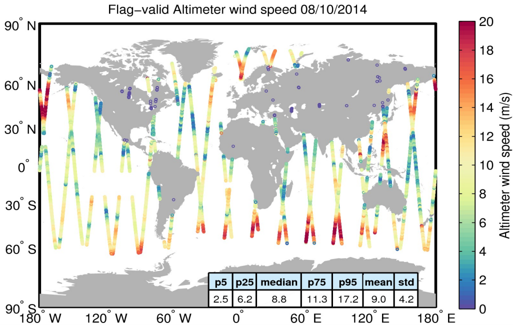
Figure 31. Geographical distribution of flag-valid wind data over oceans and lakes for 08/10/2014. The statistical values shown in the table refer to the wind in m/s and are calculated over all measurements shown in the figure.
