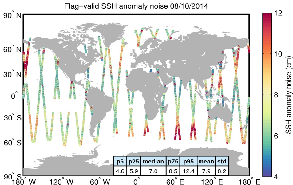
Figure 8. Geographical distribution of flag-valid 20-Hz SSH anomaly measurement noise over oceans and lakes for 08/10/2014. The statistical values shown in the table refer to the SSH anomaly noise and are calculated over all measurements shown in the figure.
