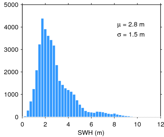
Figure 17. Histogram of flag-valid SWH over oceans and lakes for 08/10/2014. The mean ( \mu ) and standard deviation ( \sigma ) are also shown. Note that values larger than 12 m are excluded from the histogram for the sake of readability but not from the computation of \mu and \sigma .
