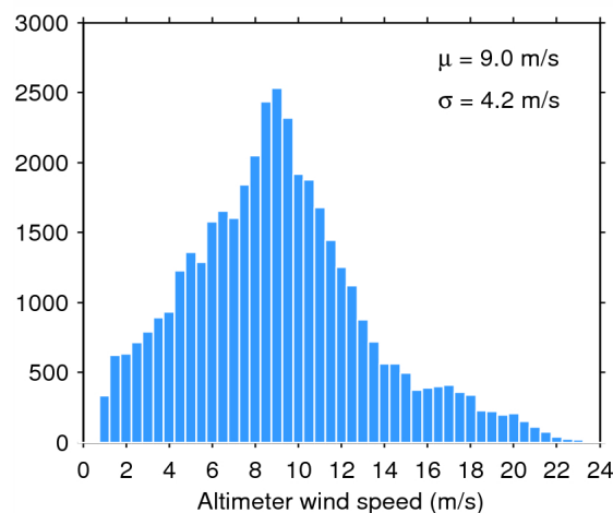
Figure 35. Histogram of science-valid wind over oceans and lakes for 08/10/2014. The mean ( \mu ) and standard deviation ( \sigma ) are also shown. Note that values larger than 24 m/s are excluded from the histogram for the sake of readability but not from the computation of \mu and \sigma .
