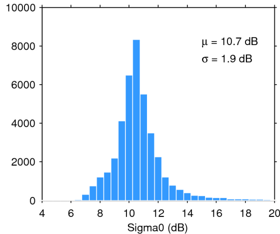
Figure 25. Histogram of flag-valid sigma0 over oceans and lakes for 08/10/2014. The mean ( \mu ) and standard deviation ( \sigma ) are also shown. Note that values outside [4 20] dB are excluded from the histogram for the sake of readability but not from the computation of \mu and \sigma .
