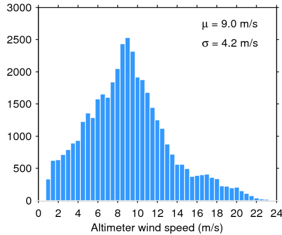
Figure 33. Histogram of flag-valid wind over oceans and lakes for 08/10/2014. The mean ( \mu ) and standard deviation ( \sigma ) are also shown. Note that values larger than 24 m/s are excluded from the histogram for the sake of readability but not from the computation of \mu and \sigma .
