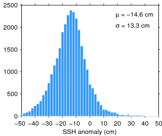
Figure 11. Histogram of science-valid SSH anomaly over oceans and lakes for 07/10/2014. The mean ( \mu ) and standard deviation ( \sigma ) are also shown. Note that values outside [-50 50] cm are excluded from the histogram for the sake of readability but not from the computation of \mu and \sigma .
