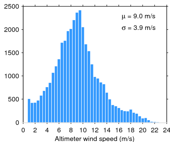
Figure 35. Histogram of science-valid wind over oceans and lakes for 07/10/2014. The mean ( \mu ) and standard deviation ( \sigma ) are also shown. Note that values larger than 24 m/s are excluded from the histogram for the sake of readability but not from the computation of \mu and \sigma .
