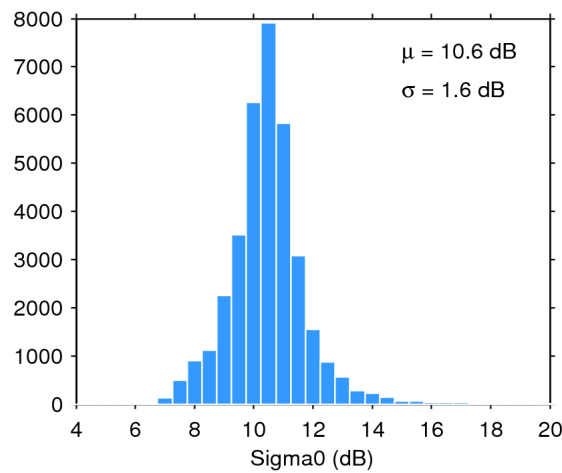
Figure 28. Histogram of science-valid sigma0 over oceans and lakes for 07/10/2014. The mean ( \mu ) and standard deviation ( \sigma ) are also shown. Note that values outside [4 20] dB are excluded from the histogram for the sake of readability but not from the computation of \mu and \sigma .
