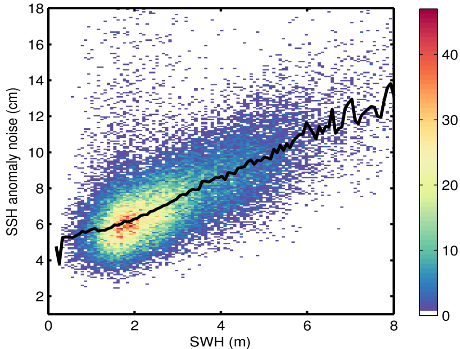
Figure 9. 2D histogram showing flag-valid SSH anomaly noise as a function of SWH for 07/10/2014. The black line denotes the median SSH anomaly as a function of SWH.
