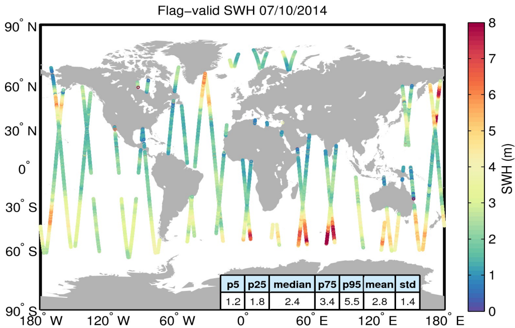
Figure 15. Geographical distribution of flag-valid SWH data over oceans and lakes for 07/10/2014. The statistical values shown in the table refer to the SWH in m and are calculated over all measurements shown in the figure.
