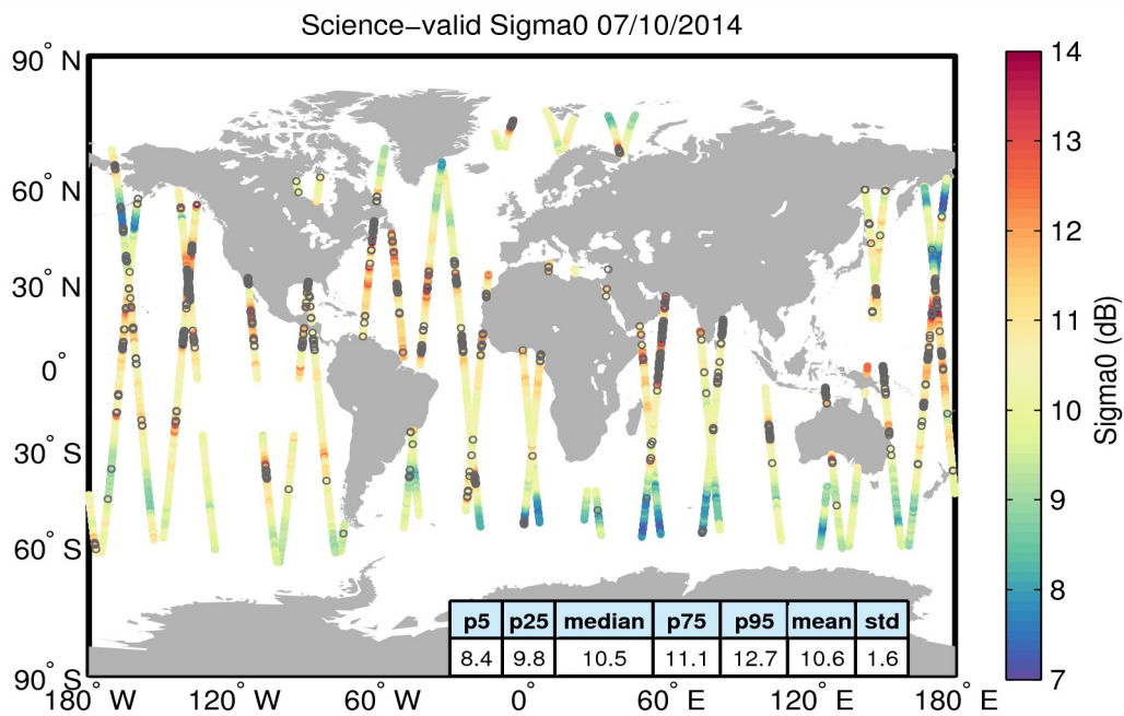
Figure 27. Geographical distribution of science-valid sigma0 data over oceans and lakes for 07/10/2014. The statistical values shown in the table refer to the sigma0 in dB and are calculated over all measurements shown in the figure. Gray circles denote records that have been rejected based on the editing criteria described in Table 4.
