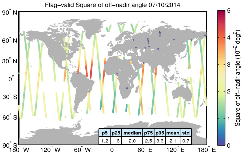
Figure 37. Geographical distribution of flag-valid mispointing data over oceans and lakes for 07/10/2014. The statistical values shown in the table refer to the mispointing in 10^{-2} \text{ deg}^2 and are calculated over all measurements shown in the figure.
