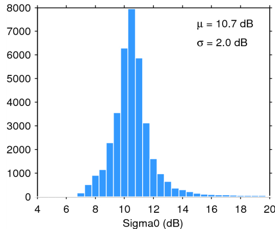
Figure 25. Histogram of flag-valid sigma0 over oceans and lakes for 07/10/2014. The mean ( \mu ) and standard deviation ( \sigma ) are also shown. Note that values outside [4 20] dB are excluded from the histogram for the sake of readability but not from the computation of \mu and \sigma .
