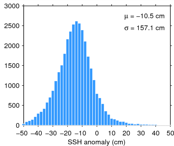
Figure 7. Histogram of flag-valid SSH anomaly over oceans and lakes for 07/10/2014. The mean ( \mu ) and standard deviation ( \sigma ) are also shown. Note that values outside [-50\ 50] cm are excluded from the histogram for the sake of readability but not from the computation of \mu and \sigma .
