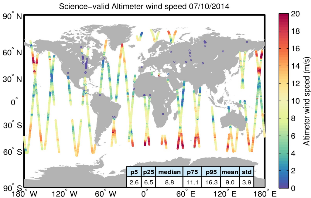
Figure 34. Geographical distribution of science-valid wind data over oceans and lakes for 07/10/2014. The statistical values shown in the table refer to the wind in m/s and are calculated over all measurements shown in the figure. Gray circles denote records that have been rejected based on the editing criteria described in Table 5.
