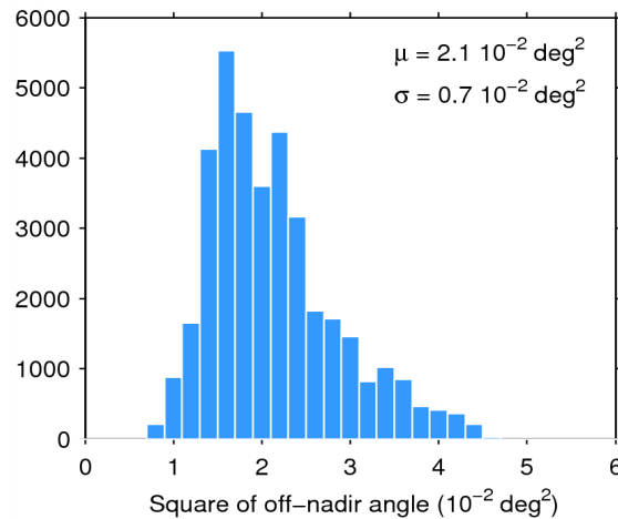
Figure 39. Histogram of flag-valid mispointing over oceans and lakes for 07/10/2014. The mean ( \mu ) and standard deviation ( \sigma ) are also shown. Note that values than 6 \cdot 10^{-2} \text{ deg}^2 are excluded from the histogram for the sake of readability but not from the computation of \mu and \sigma .
