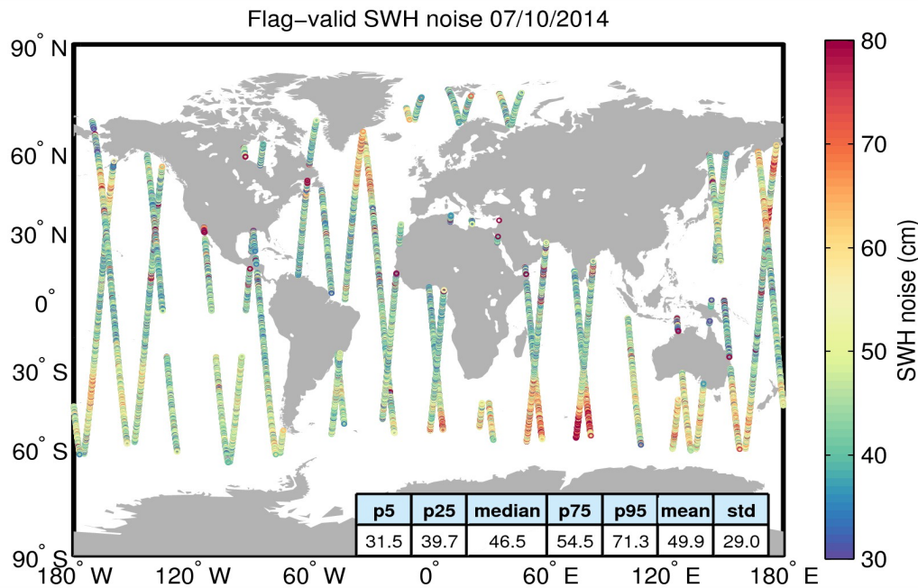
Figure 18. Geographical distribution of flag-valid 20-Hz SWH measurement noise over oceans and lakes for 07/10/2014. The statistical values shown in the figure refer to the SWH noise and are calculated over all measurements shown in the figure.
