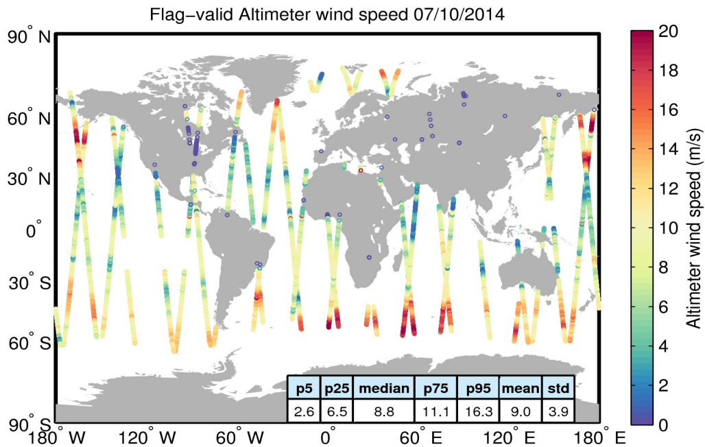
Figure 31. Geographical distribution of flag-valid wind data over oceans and lakes for 07/10/2014. The statistical values shown in the table refer to the wind in m/s and are calculated over all measurements shown in the figure.
