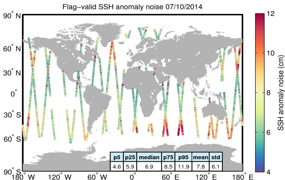
Figure 8. Geographical distribution of flag-valid 20-Hz SSH anomaly measurement noise over oceans and lakes for 07/10/2014. The statistical values shown in the table refer to the SSH anomaly noise and are calculated over all measurements shown in the figure.
