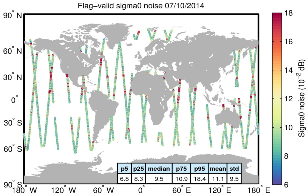
Figure 26. Geographical distribution of flag-valid 20-Hz sigma0 measurement noise over oceans and lakes for 07/10/2014. The statistical values shown in the table refer to the sigma0 noise and are calculated over all measurements shown in the figure.
