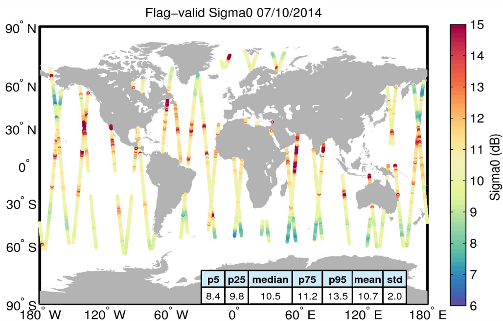
Figure 23. Geographical distribution of flag-valid sigma0 data over oceans and lakes for 07/10/2014. The statistical values shown in the table refer to the sigma0 in dB and are calculated over all measurements shown in the figure.
