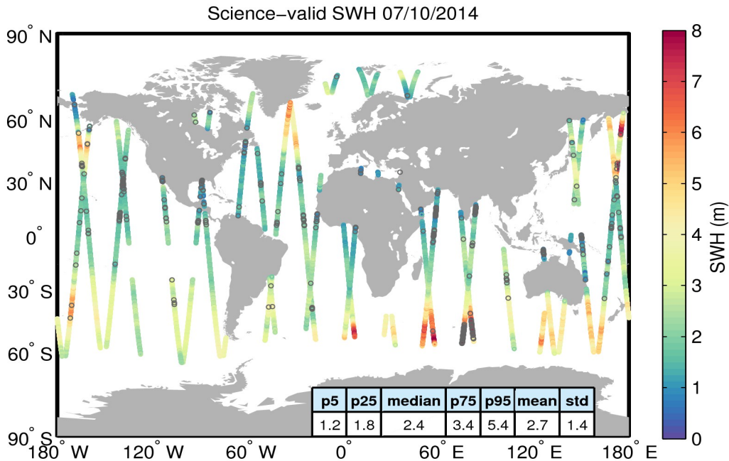
Figure 19. Geographical distribution of science-valid SWH data over oceans and lakes for 07/10/2014. The statistical values shown in the table refer to the SWH in m and are calculated over all measurements shown in the figure. Gray circles denote records that have been rejected based on the editing criteria described in Table 3.
