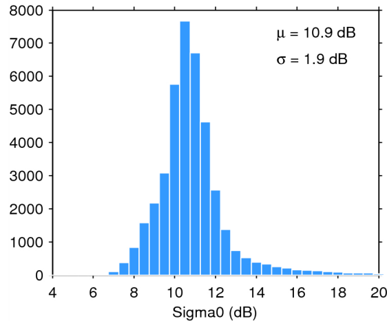
Figure 25. Histogram of flag-valid sigma0 over oceans and lakes for 06/10/2014. The mean ( \mu ) and standard deviation ( \sigma ) are also shown. Note that values outside [4 20] dB are excluded from the histogram for the sake of readability but not from the computation of \mu and \sigma .
