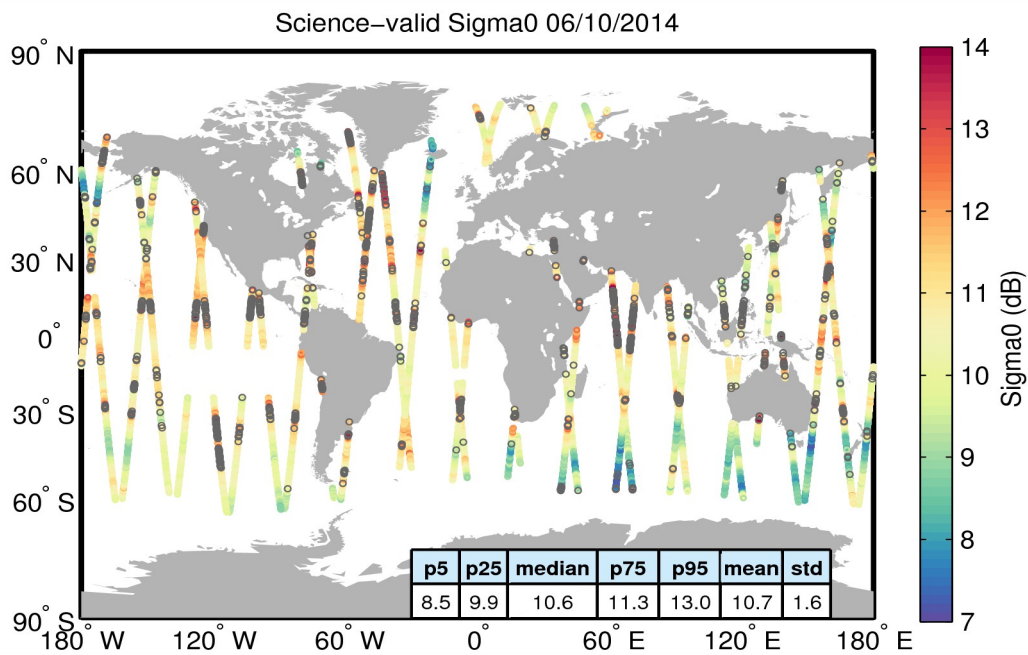
Figure 27. Geographical distribution of science-valid sigma0 data over oceans and lakes for 06/10/2014. The statistical values shown in the table refer to the sigma0 in dB and are calculated over all measurements shown in the figure. Gray circles denote records that have been rejected based on the editing criteria described in Table 4.
