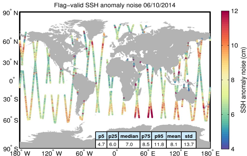
Figure 8. Geographical distribution of flag-valid 20-Hz SSH anomaly measurement noise over oceans and lakes for 06/10/2014. The statistical values shown in the table refer to the SSH anomaly noise and are calculated over all measurements shown in the figure.
