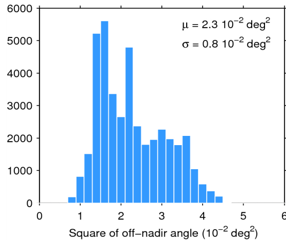
Figure 39. Histogram of flag-valid mispointing over oceans and lakes for 06/10/2014. The mean ( \mu ) and standard deviation ( \sigma ) are also shown. Note that values than 6 \cdot 10^{-2} \text{ deg}^2 are excluded from the histogram for the sake of readability but not from the computation of \mu and \sigma .
