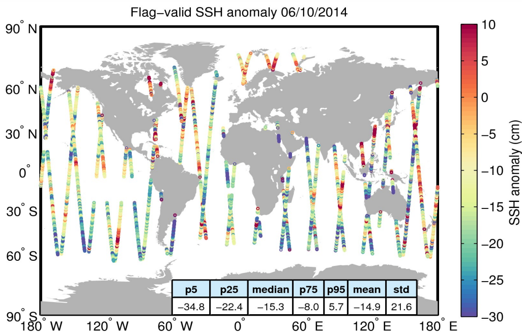
Figure 5. Geographical distribution of flag-valid 1-Hz SSH anomaly data over oceans and lakes for 06/10/2014. The statistical values shown in the table refer to the SSH anomaly in cm and are calculated over all measurements shown in the figure.
