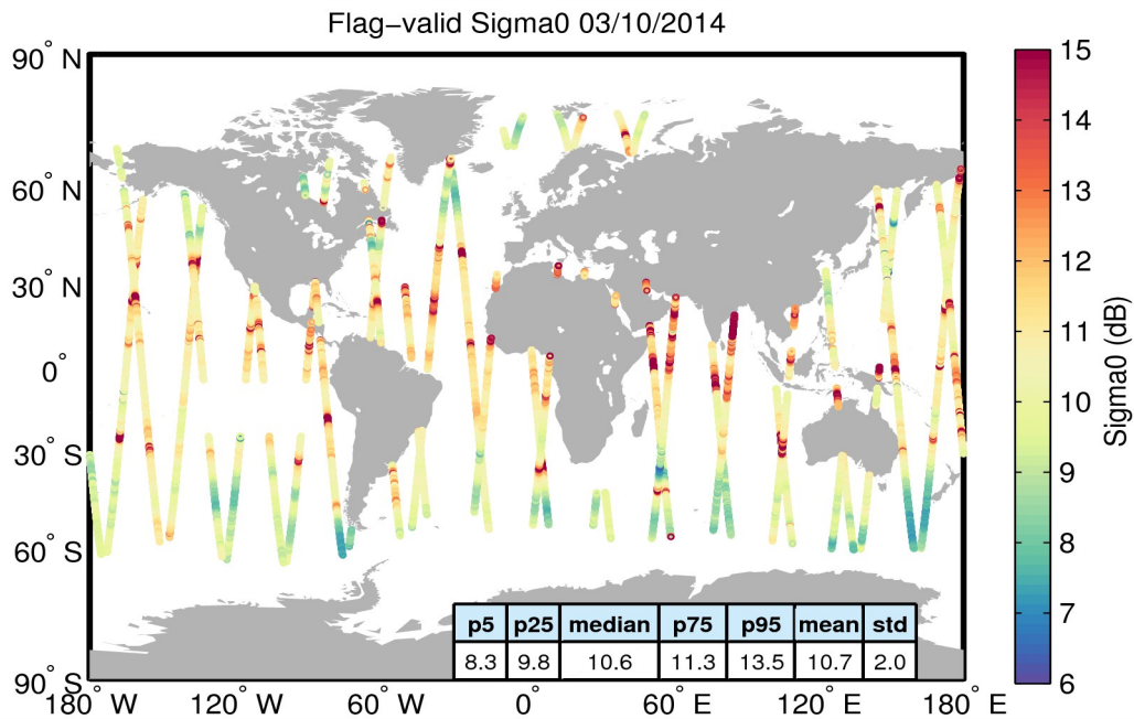
Figure 23. Geographical distribution of flag-valid sigma0 data over oceans and lakes for 03/10/2014. The statistical values shown in the table refer to the sigma0 in dB and are calculated over all measurements shown in the figure.
