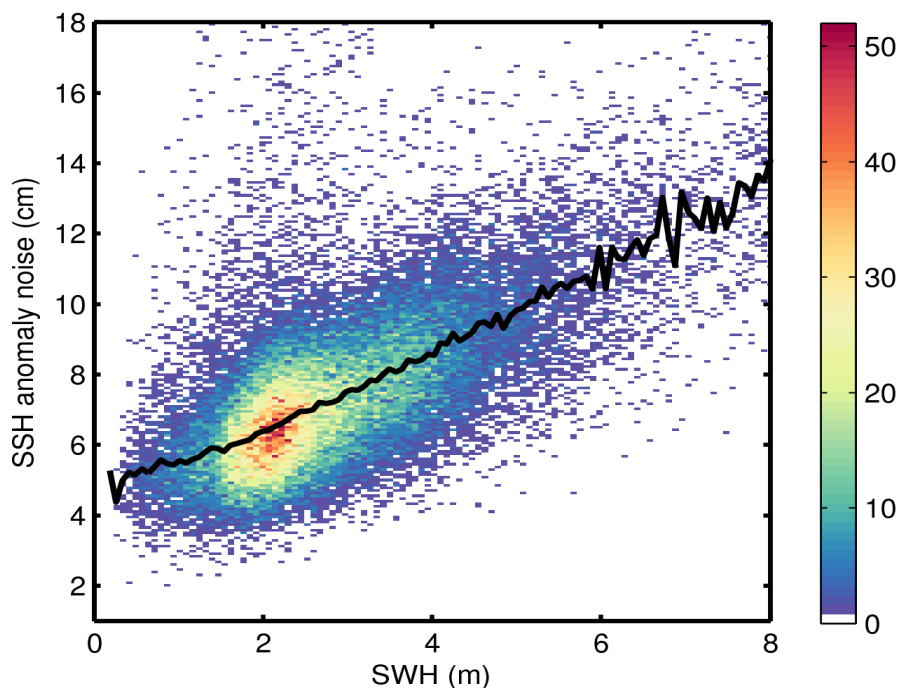
Figure 9. 2D histogram showing flag-valid SSH anomaly noise as a function of SWH for 03/10/2014. The black line denotes the median SSH anomaly as a function of SWH.
