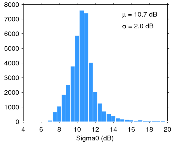
Figure 25. Histogram of flag-valid sigma0 over oceans and lakes for 03/10/2014. The mean ( \mu ) and standard deviation ( \sigma ) are also shown. Note that values outside [4 20] dB are excluded from the histogram for the sake of readability but not from the computation of \mu and \sigma .
