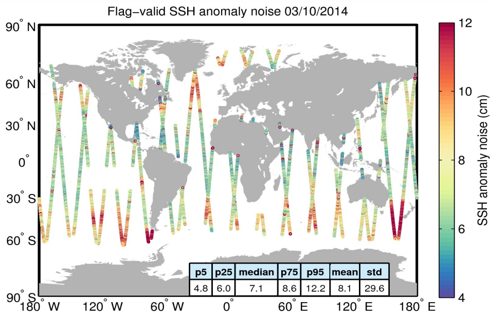
Figure 8. Geographical distribution of flag-valid 20-Hz SSH anomaly measurement noise over oceans and lakes for 03/10/2014. The statistical values shown in the table refer to the SSH anomaly noise and are calculated over all measurements shown in the figure.
