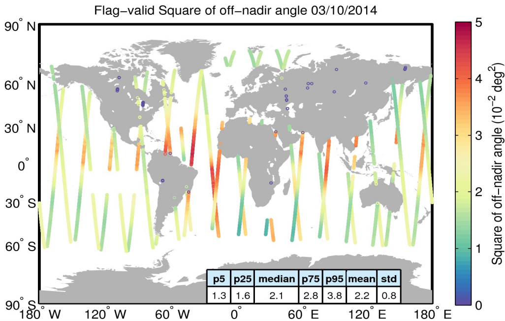
Figure 37. Geographical distribution of flag-valid mispointing data over oceans and lakes for 03/10/2014. The statistical values shown in the table refer to the mispointing in 10^{-2} \text{ deg}^2 and are calculated over all measurements shown in the figure.
