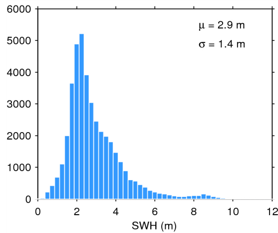
Figure 17. Histogram of flag-valid SWH over oceans and lakes for 03/10/2014. The mean ( \mu ) and standard deviation ( \sigma ) are also shown. Note that values larger than 12 m are excluded from the histogram for the sake of readability but not from the computation of \mu and \sigma .
