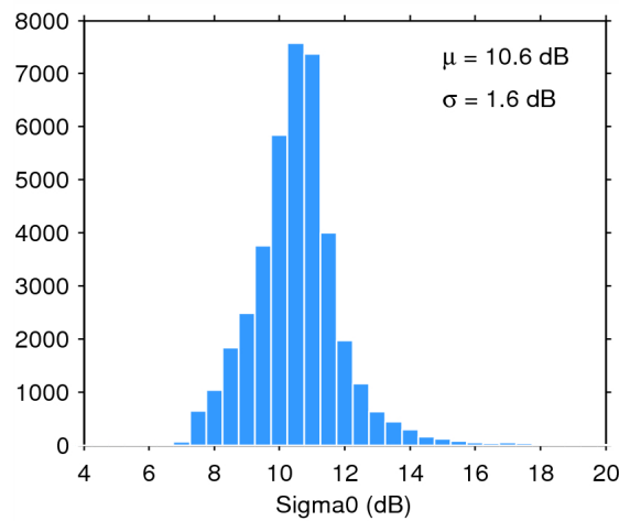
Figure 28. Histogram of science-valid sigma0 over oceans and lakes for 03/10/2014. The mean ( \mu ) and standard deviation ( \sigma ) are also shown. Note that values outside [4 20] dB are excluded from the histogram for the sake of readability but not from the computation of \mu and \sigma .
