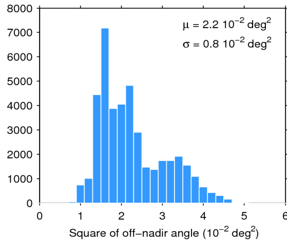
Figure 39. Histogram of flag-valid mispointing over oceans and lakes for 03/10/2014. The mean ( \mu ) and standard deviation ( \sigma ) are also shown. Note that values than 6 \cdot 10^{-2} \text{ deg}^2 are excluded from the histogram for the sake of readability but not from the computation of \mu and \sigma .
