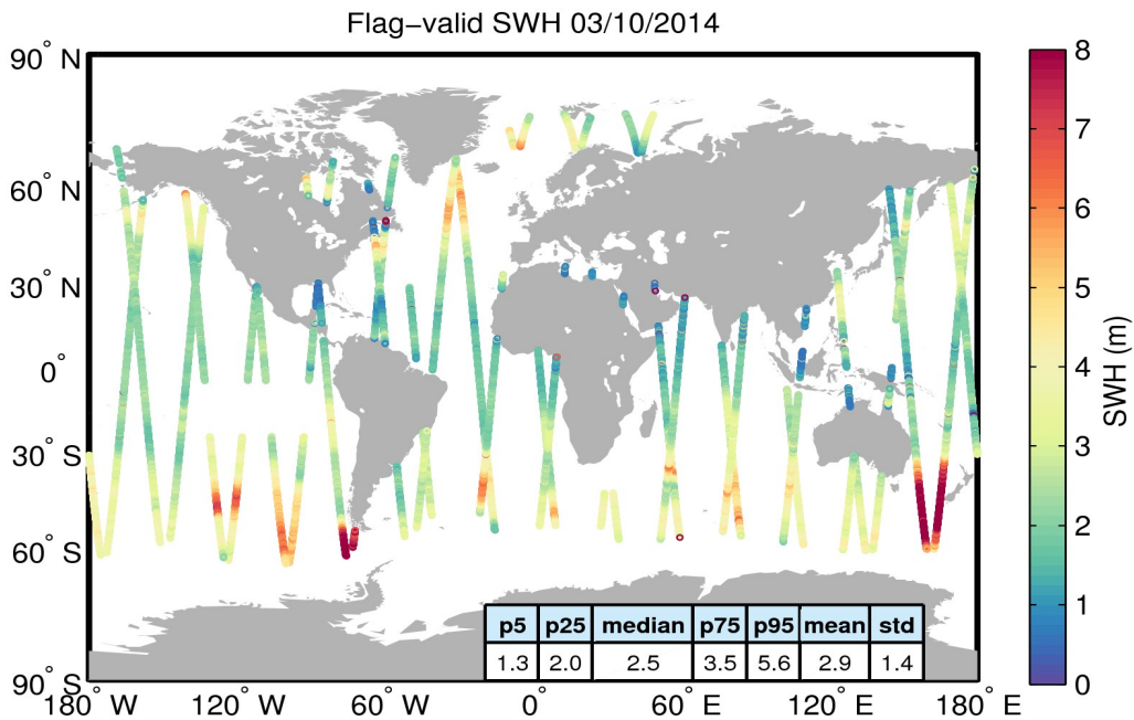
Figure 15. Geographical distribution of flag-valid SWH data over oceans and lakes for 03/10/2014. The statistical values shown in the table refer to the SWH in m and are calculated over all measurements shown in the figure.
