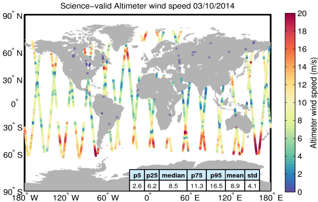
Figure 34. Geographical distribution of science-valid wind data over oceans and lakes for 03/10/2014. The statistical values shown in the table refer to the wind in m/s and are calculated over all measurements shown in the figure. Gray circles denote records that have been rejected based on the editing criteria described in Table 5.
