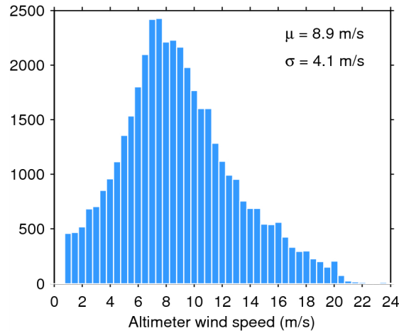
Figure 33. Histogram of flag-valid wind over oceans and lakes for 03/10/2014. The mean ( \mu ) and standard deviation ( \sigma ) are also shown. Note that values larger than 24 m/s are excluded from the histogram for the sake of readability but not from the computation of \mu and \sigma .
