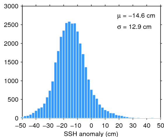
Figure 11. Histogram of science-valid SSH anomaly over oceans and lakes for 03/10/2014. The mean ( \mu ) and standard deviation ( \sigma ) are also shown. Note that values outside [-50 50] cm are excluded from the histogram for the sake of readability but not from the computation of \mu and \sigma .
