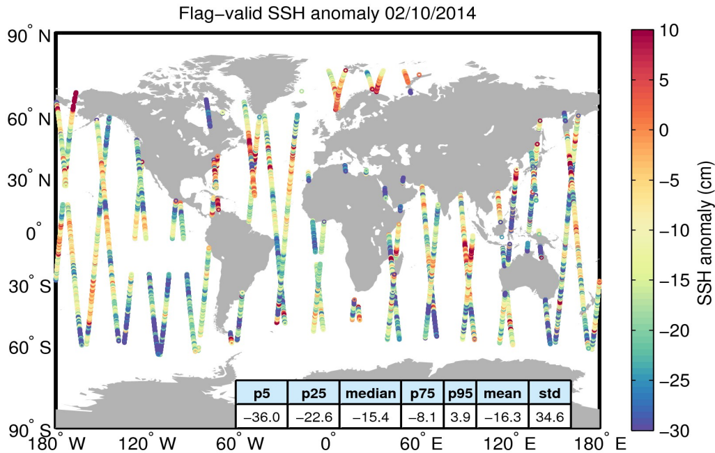
Figure 5. Geographical distribution of flag-valid 1-Hz SSH anomaly data over oceans and lakes for 02/10/2014. The statistical values shown in the table refer to the SSH anomaly in cm and are calculated over all measurements shown in the figure.
