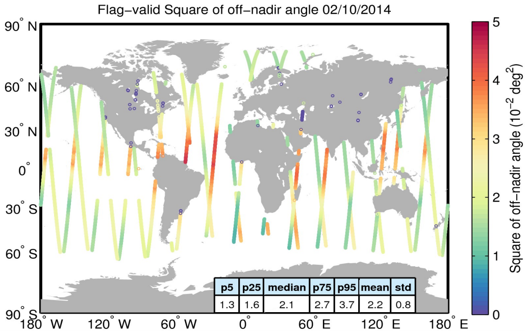
Figure 37. Geographical distribution of flag-valid mispointing data over oceans and lakes for 02/10/2014. The statistical values shown in the table refer to the mispointing in 10^{-2} \text{ deg}^2 and are calculated over all measurements shown in the figure.
