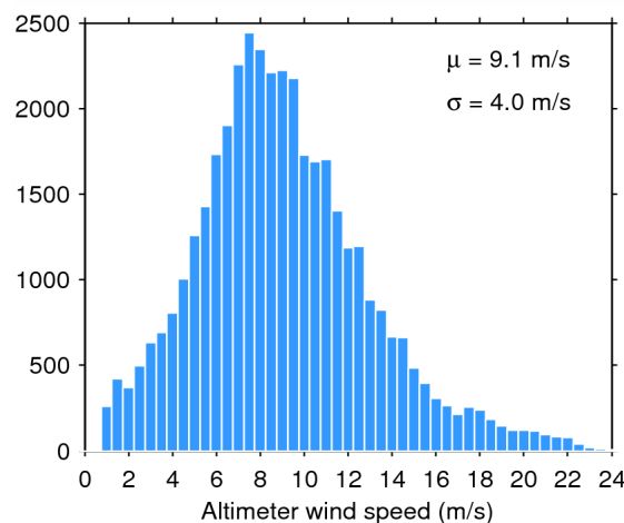
Figure 35. Histogram of science-valid wind over oceans and lakes for 02/10/2014. The mean ( \mu ) and standard deviation ( \sigma ) are also shown. Note that values larger than 24 m/s are excluded from the histogram for the sake of readability but not from the computation of \mu and \sigma .
