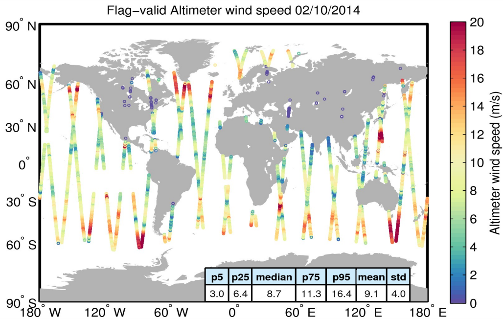
Figure 31. Geographical distribution of flag-valid wind data over oceans and lakes for 02/10/2014. The statistical values shown in the table refer to the wind in m/s and are calculated over all measurements shown in the figure.
