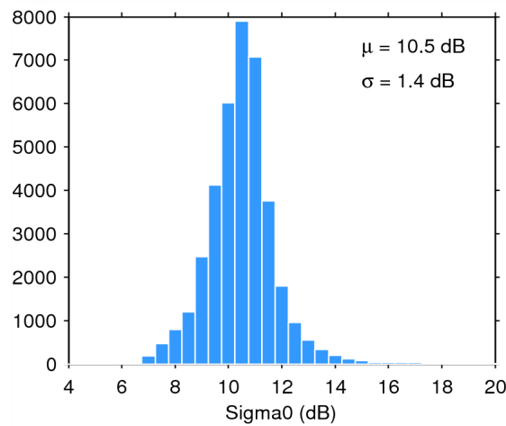
Figure 28. Histogram of science-valid sigma0 over oceans and lakes for 02/10/2014. The mean ( \mu ) and standard deviation ( \sigma ) are also shown. Note that values outside [4 20] dB are excluded from the histogram for the sake of readability but not from the computation of \mu and \sigma .
