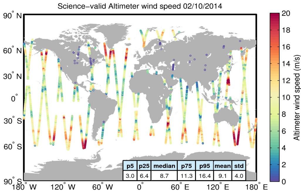
Figure 34. Geographical distribution of science-valid wind data over oceans and lakes for 02/10/2014. The statistical values shown in the table refer to the wind in m/s and are calculated over all measurements shown in the figure. Gray circles denote records that have been rejected based on the editing criteria described in Table 5.
