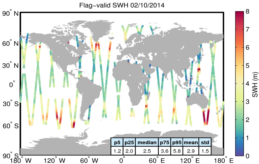
Figure 15. Geographical distribution of flag-valid SWH data over oceans and lakes for 02/10/2014. The statistical values shown in the table refer to the SWH in m and are calculated over all measurements shown in the figure.
