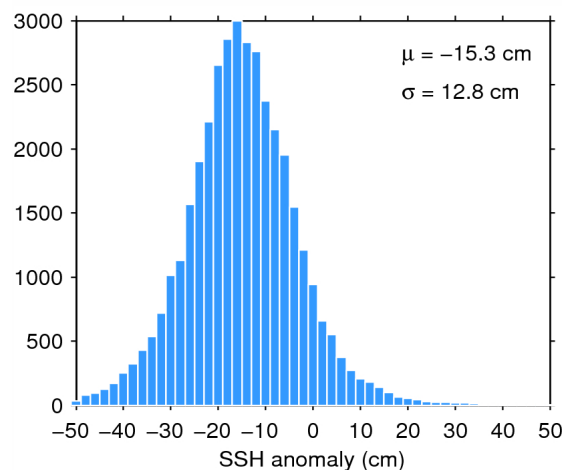
Figure 11. Histogram of science-valid SSH anomaly over oceans and lakes for 02/10/2014. The mean ( \mu ) and standard deviation ( \sigma ) are also shown. Note that values outside [-50 50] cm are excluded from the histogram for the sake of readability but not from the computation of \mu and \sigma .
