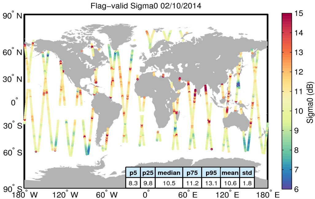
Figure 23. Geographical distribution of flag-valid sigma0 data over oceans and lakes for 02/10/2014. The statistical values shown in the table refer to the sigma0 in dB and are calculated over all measurements shown in the figure.
