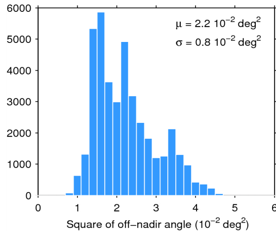
Figure 39. Histogram of flag-valid mispointing over oceans and lakes for 02/10/2014. The mean ( \mu ) and standard deviation ( \sigma ) are also shown. Note that values than 6 \cdot 10^{-2} \text{ deg}^2 are excluded from the histogram for the sake of readability but not from the computation of \mu and \sigma .
