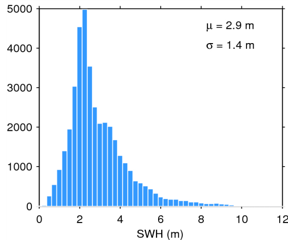
Figure 20. Histogram of science-valid SWH over oceans and lakes for 02/10/2014. The mean ( \mu ) and standard deviation ( \sigma ) are also shown. Note that values larger than 12 m are excluded from the histogram for the sake of readability but not from the computation of \mu and \sigma .
