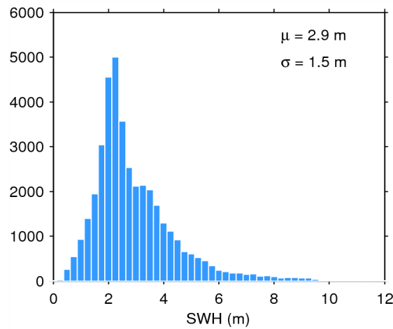
Figure 17. Histogram of flag-valid SWH over oceans and lakes for 02/10/2014. The mean ( \mu ) and standard deviation ( \sigma ) are also shown. Note that values larger than 12 m are excluded from the histogram for the sake of readability but not from the computation of \mu and \sigma .
