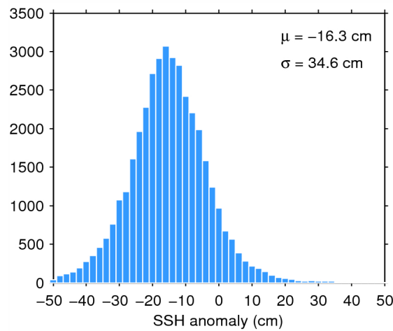
Figure 7. Histogram of flag-valid SSH anomaly over oceans and lakes for 02/10/2014. The mean ( \mu ) and standard deviation ( \sigma ) are also shown. Note that values outside [-50\ 50] cm are excluded from the histogram for the sake of readability but not from the computation of \mu and \sigma .
