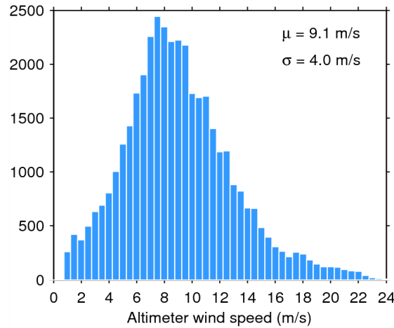
Figure 33. Histogram of flag-valid wind over oceans and lakes for 02/10/2014. The mean ( \mu ) and standard deviation ( \sigma ) are also shown. Note that values larger than 24 m/s are excluded from the histogram for the sake of readability but not from the computation of \mu and \sigma .
