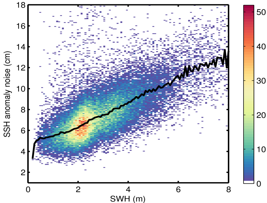
Figure 9. 2D histogram showing flag-valid SSH anomaly noise as a function of SWH for 02/10/2014. The black line denotes the median SSH anomaly as a function of SWH.
