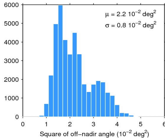
Figure 39. Histogram of flag-valid mispointing over oceans and lakes for 01/10/2014. The mean ( \mu ) and standard deviation ( \sigma ) are also shown. Note that values than 6 \cdot 10^{-2} \text{ deg}^2 are excluded from the histogram for the sake of readability but not from the computation of \mu and \sigma .
