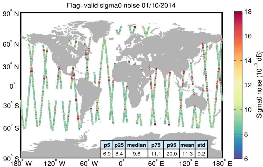
Figure 26. Geographical distribution of flag-valid 20-Hz sigma0 measurement noise over oceans and lakes for 01/10/2014. The statistical values shown in the table refer to the sigma0 noise and are calculated over all measurements shown in the figure.
