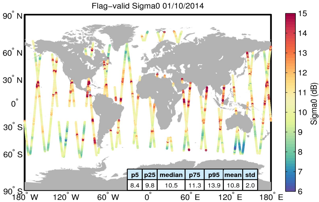
Figure 23. Geographical distribution of flag-valid sigma0 data over oceans and lakes for 01/10/2014. The statistical values shown in the table refer to the sigma0 in dB and are calculated over all measurements shown in the figure.
