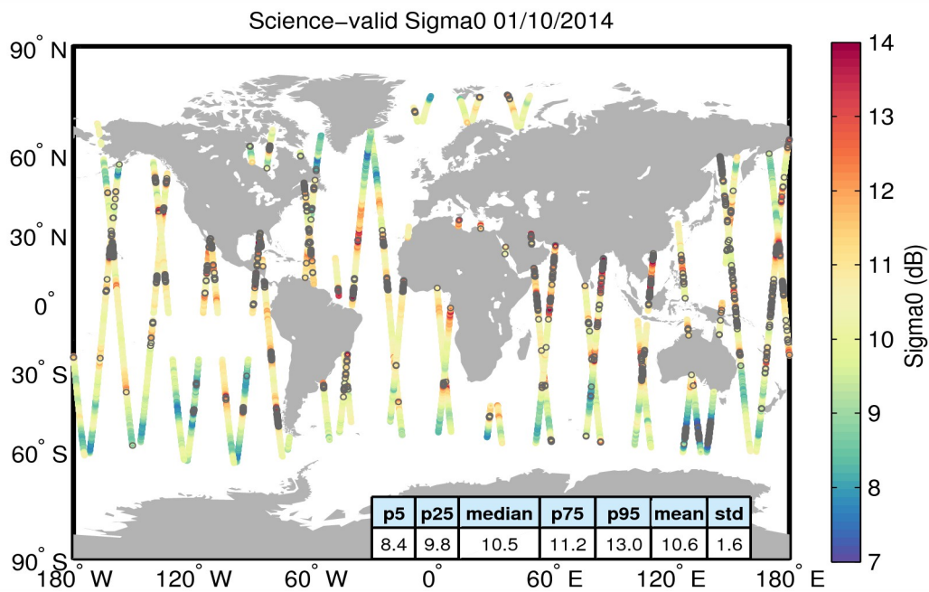
Figure 27. Geographical distribution of science-valid sigma0 data over oceans and lakes for 01/10/2014. The statistical values shown in the table refer to the sigma0 in dB and are calculated over all measurements shown in the figure. Gray circles denote records that have been rejected based on the editing criteria described in Table 4.
