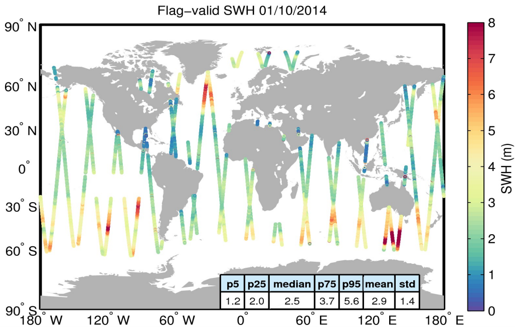
Figure 15. Geographical distribution of flag-valid SWH data over oceans and lakes for 01/10/2014. The statistical values shown in the figure refer to the SWH in m and are calculated over all measurements shown in the figure.
