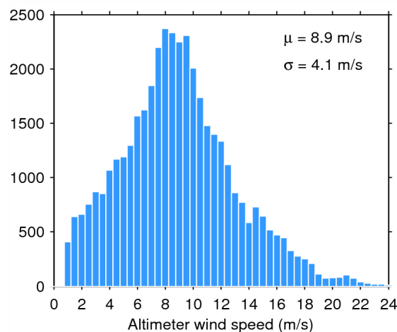
Figure 35. Histogram of science-valid wind over oceans and lakes for 01/10/2014. The mean ( \mu ) and standard deviation ( \sigma ) are also shown. Note that values larger than 24 m/s are excluded from the histogram for the sake of readability but not from the computation of \mu and \sigma .
