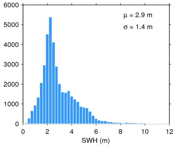
Figure 17. Histogram of flag-valid SWH over oceans and lakes for 01/10/2014. The mean ( \mu ) and standard deviation ( \sigma ) are also shown. Note that values larger than 12 m are excluded from the histogram for the sake of readability but not from the computation of \mu and \sigma .
