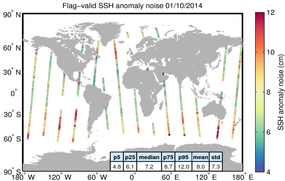
Figure 8. Geographical distribution of flag-valid 20-Hz SSH anomaly measurement noise over oceans and lakes for 01/10/2014. The statistical values shown in the table refer to the SSH anomaly noise and are calculated over all measurements shown in the figure.
