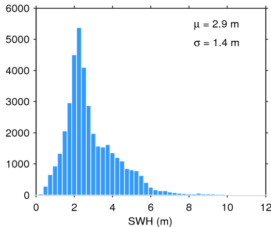
Figure 20. Histogram of science-valid SWH over oceans and lakes for 01/10/2014. The mean ( \mu ) and standard deviation ( \sigma ) are also shown. Note that values larger than 12 m are excluded from the histogram for the sake of readability but not from the computation of \mu and \sigma .
