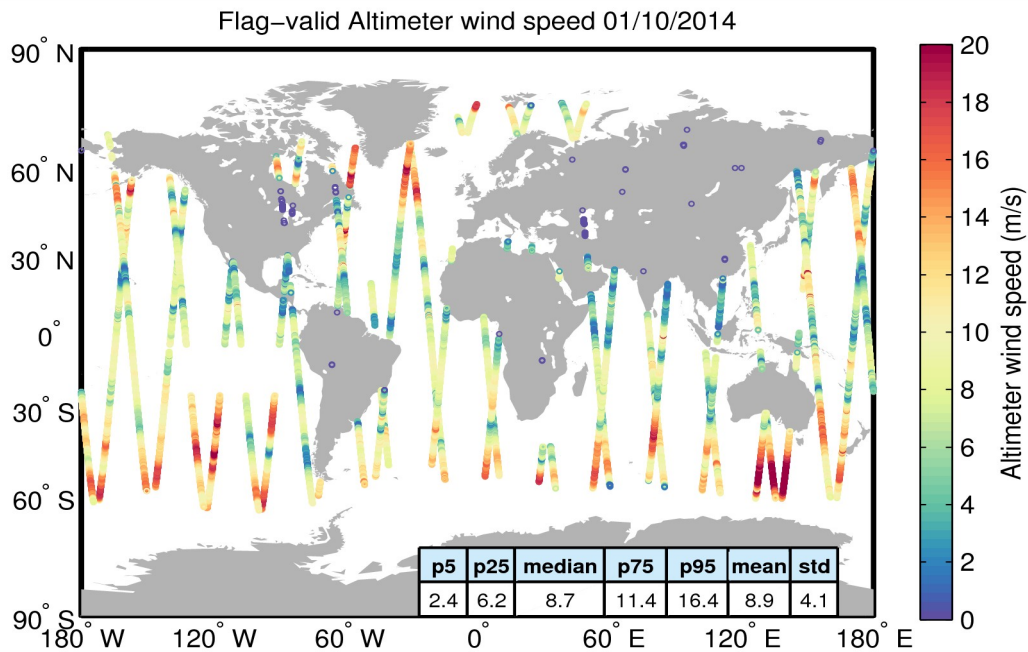
Figure 31. Geographical distribution of flag-valid wind data over oceans and lakes for 01/10/2014. The statistical values shown in the table refer to the wind in m/s and are calculated over all measurements shown in the figure.
