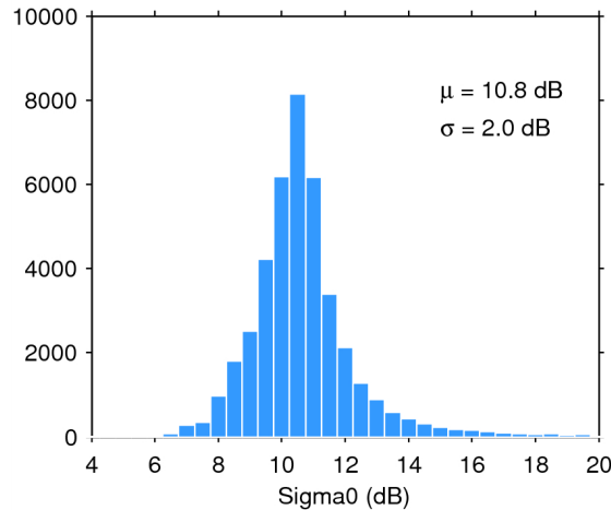
Figure 25. Histogram of flag-valid sigma0 over oceans and lakes for 01/10/2014. The mean ( \mu ) and standard deviation ( \sigma ) are also shown. Note that values outside [4 20] dB are excluded from the histogram for the sake of readability but not from the computation of \mu and \sigma .
