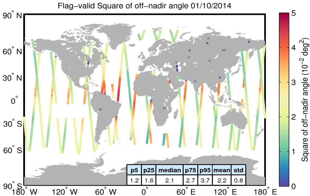
Figure 37. Geographical distribution of flag-valid mispointing data over oceans and lakes for 01/10/2014. The statistical values shown in the table refer to the mispointing in 10^{-2} \text{ deg}^2 and are calculated over all measurements shown in the figure.
