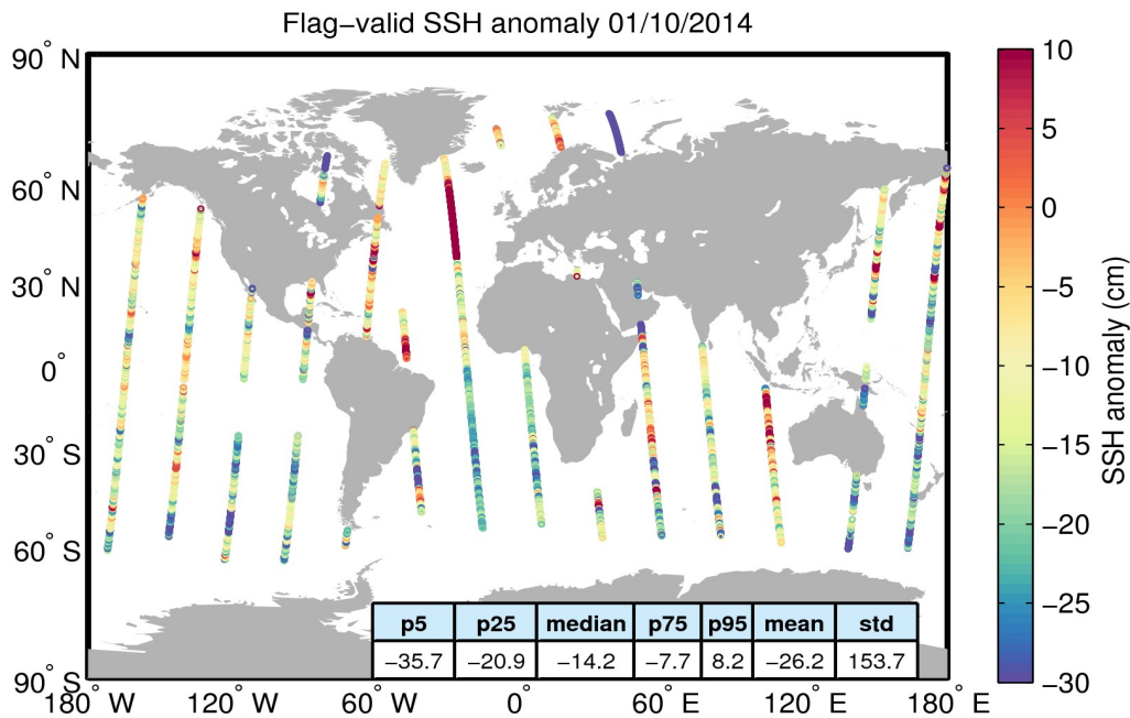
Figure 5. Geographical distribution of flag-valid 1-Hz SSH anomaly data over oceans and lakes for 01/10/2014. The statistical values shown in the table refer to the SSH anomaly in cm and are calculated over all measurements shown in the figure.
