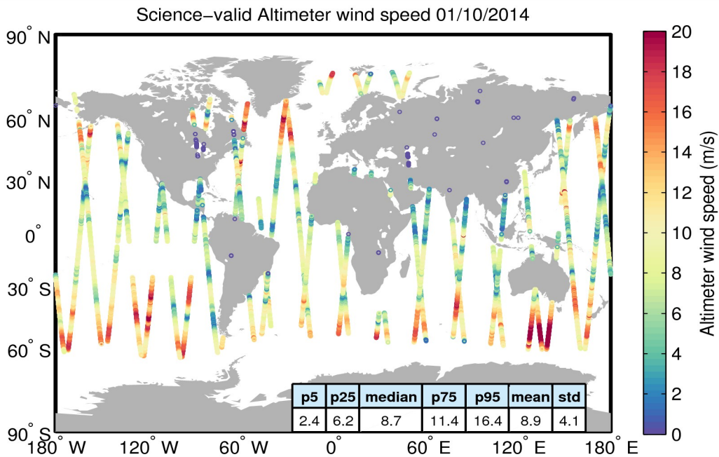
Figure 34. Geographical distribution of science-valid wind data over oceans and lakes for 01/10/2014. The statistical values shown in the table refer to the wind in m/s and are calculated over all measurements shown in the figure. Gray circles denote records that have been rejected based on the editing criteria described in Table 5.
