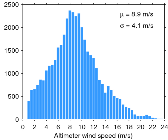
Figure 33. Histogram of flag-valid wind over oceans and lakes for 01/10/2014. The mean ( \mu ) and standard deviation ( \sigma ) are also shown. Note that values larger than 24 m/s are excluded from the histogram for the sake of readability but not from the computation of \mu and \sigma .
