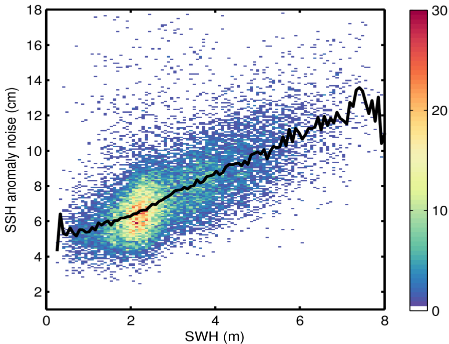
Figure 9. 2D histogram showing flag-valid SSH anomaly noise as a function of SWH for 01/10/2014. The black line denotes the median SSH anomaly as a function of SWH.
