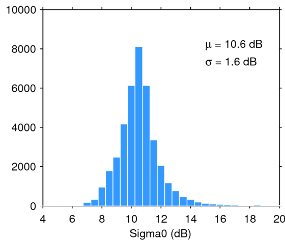
Figure 28. Histogram of science-valid sigma0 over oceans and lakes for 01/10/2014. The mean ( \mu ) and standard deviation ( \sigma ) are also shown. Note that values outside [4 20] dB are excluded from the histogram for the sake of readability but not from the computation of \mu and \sigma .
