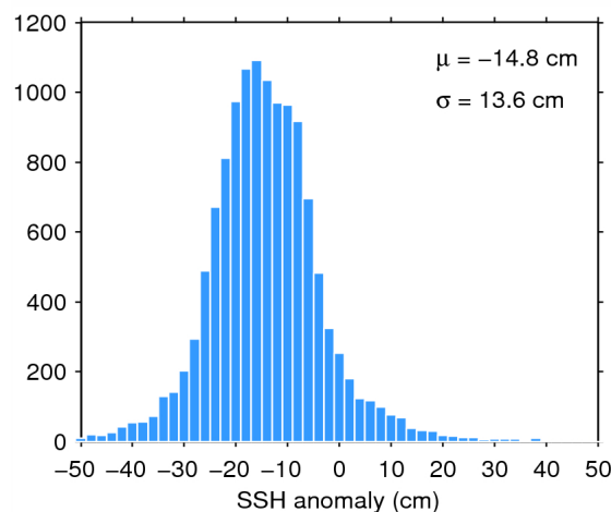
Figure 11. Histogram of science-valid SSH anomaly over oceans and lakes for 01/10/2014. The mean ( \mu ) and standard deviation ( \sigma ) are also shown. Note that values outside [-50 50] cm are excluded from the histogram for the sake of readability but not from the computation of \mu and \sigma .
