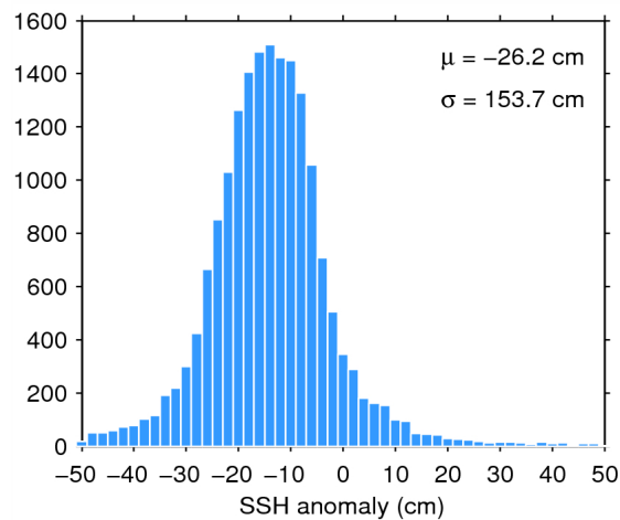
Figure 7. Histogram of flag-valid SSH anomaly over oceans and lakes for 01/10/2014. The mean ( \mu ) and standard deviation ( \sigma ) are also shown. Note that values outside [-50 50] cm are excluded from the histogram for the sake of readability but not from the computation of \mu and \sigma .
