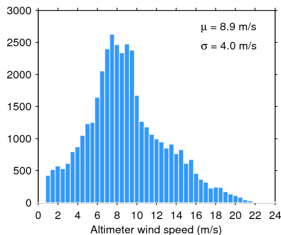
Figure 35. Histogram of science-valid wind over oceans and lakes for 30/09/2014. The mean ( \mu ) and standard deviation ( \sigma ) are also shown. Note that values larger than 24 m/s are excluded from the histogram for the sake of readability but not from the computation of \mu and \sigma .
