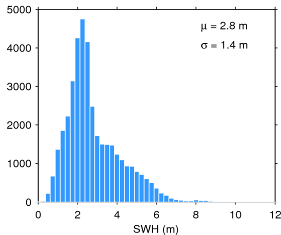
Figure 20. Histogram of science-valid SWH over oceans and lakes for 30/09/2014. The mean ( \mu ) and standard deviation ( \sigma ) are also shown. Note that values larger than 12 m are excluded from the histogram for the sake of readability but not from the computation of \mu and \sigma .
