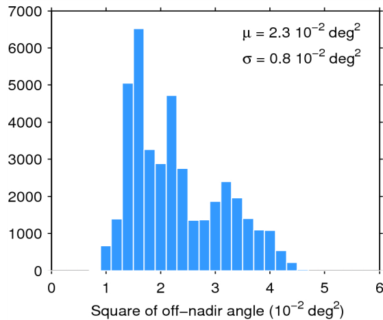
Figure 39. Histogram of flag-valid mispointing over oceans and lakes for 30/09/2014. The mean ( \mu ) and standard deviation ( \sigma ) are also shown. Note that values than 6 \cdot 10^{-2} \text{ deg}^2 are excluded from the histogram for the sake of readability but not from the computation of \mu and \sigma .
