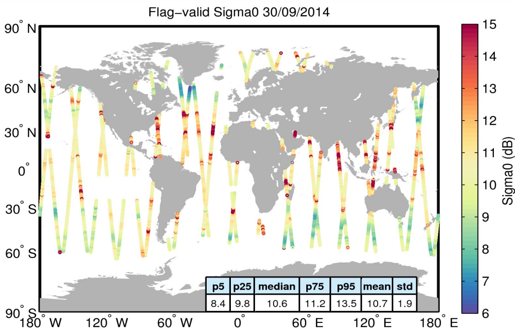
Figure 23. Geographical distribution of flag-valid sigma0 data over oceans and lakes for 30/09/2014. The statistical values shown in the table refer to the sigma0 in dB and are calculated over all measurements shown in the figure.
