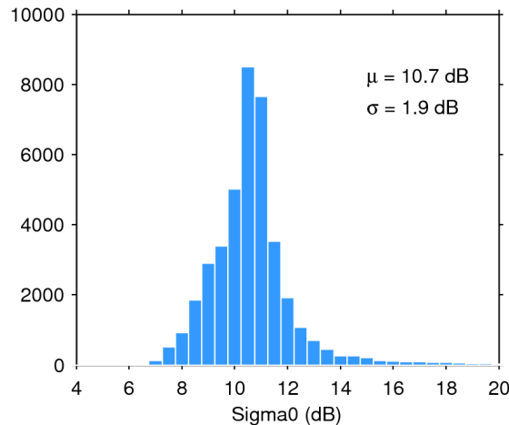
Figure 25. Histogram of flag-valid sigma0 over oceans and lakes for 30/09/2014. The mean ( \mu ) and standard deviation ( \sigma ) are also shown. Note that values outside [4 20] dB are excluded from the histogram for the sake of readability but not from the computation of \mu and \sigma .
