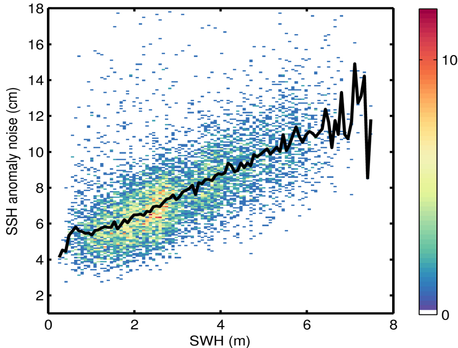
Figure 9. 2D histogram showing flag-valid SSH anomaly noise as a function of SWH for 30/09/2014. The black line denotes the median SSH anomaly as a function of SWH.
