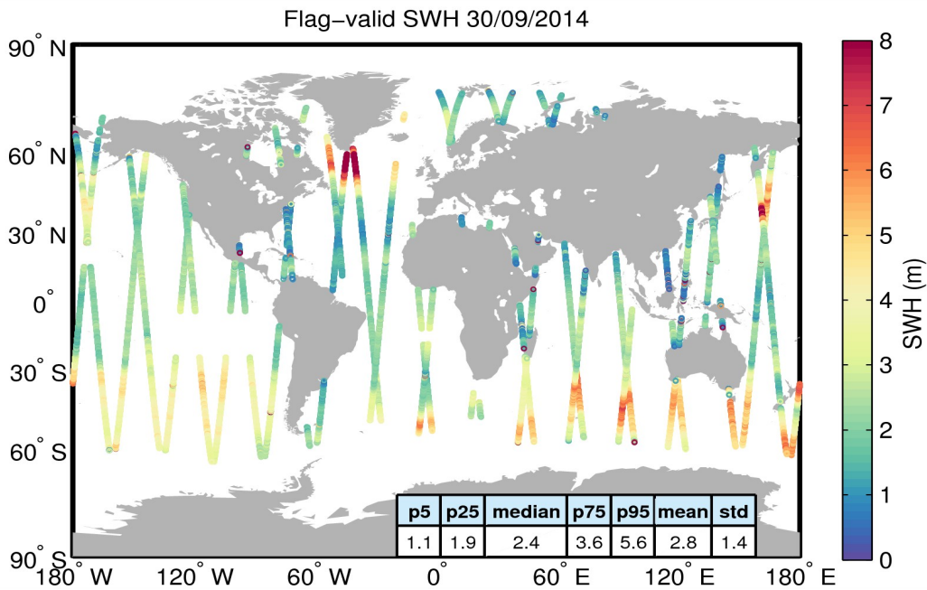
Figure 15. Geographical distribution of flag-valid SWH data over oceans and lakes for 30/09/2014. The statistical values shown in the table refer to the SWH in m and are calculated over all measurements shown in the figure.
