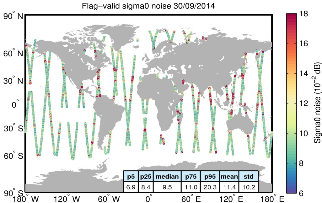
Figure 26. Geographical distribution of flag-valid 20-Hz sigma0 measurement noise over oceans and lakes for 30/09/2014. The statistical values shown in the table refer to the sigma0 noise and are calculated over all measurements shown in the figure.
