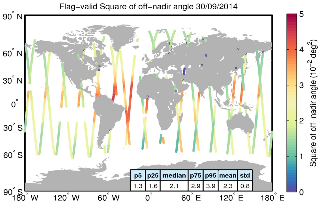
Figure 37. Geographical distribution of flag-valid mispointing data over oceans and lakes for 30/09/2014. The statistical values shown in the table refer to the mispointing in 10^{-2} \text{ deg}^2 and are calculated over all measurements shown in the figure.
