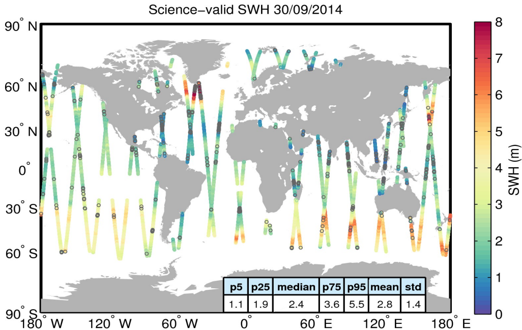
Figure 19. Geographical distribution of science-valid SWH data over oceans and lakes for 30/09/2014. The statistical values shown in the table refer to the SWH in m and are calculated over all measurements shown in the figure. Gray circles denote records that have been rejected based on the editing criteria described in Table 3.
