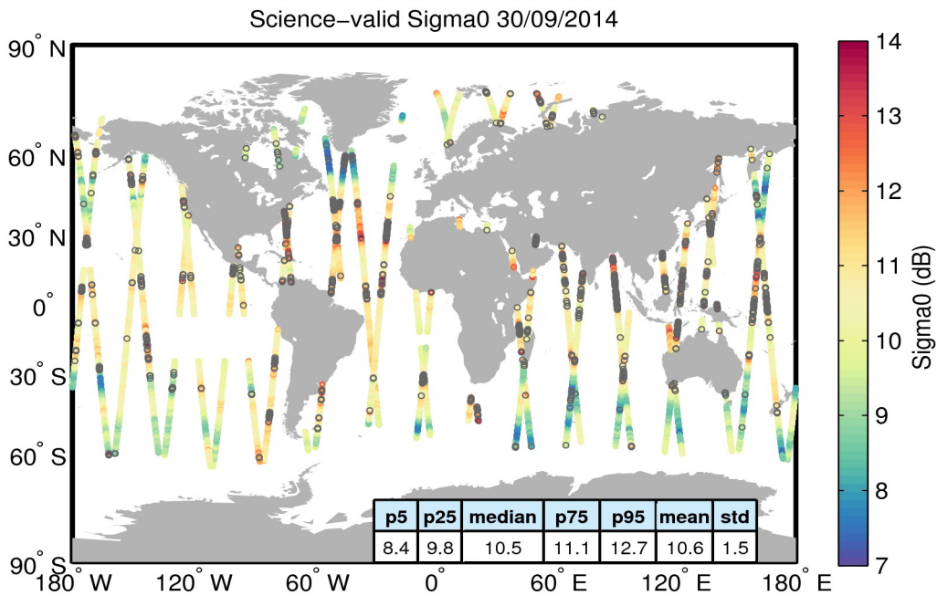
Figure 27. Geographical distribution of science-valid sigma0 data over oceans and lakes for 30/09/2014. The statistical values shown in the table refer to the sigma0 in dB and are calculated over all measurements shown in the figure. Gray circles denote records that have been rejected based on the editing criteria described in Table 4.
