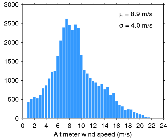
Figure 33. Histogram of flag-valid wind over oceans and lakes for 30/09/2014. The mean ( \mu ) and standard deviation ( \sigma ) are also shown. Note that values larger than 24 m/s are excluded from the histogram for the sake of readability but not from the computation of \mu and \sigma .
