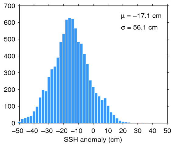
Figure 7. Histogram of flag-valid SSH anomaly over oceans and lakes for 30/09/2014. The mean ( \mu ) and standard deviation ( \sigma ) are also shown. Note that values outside [-50\ 50] cm are excluded from the histogram for the sake of readability but not from the computation of \mu and \sigma .
