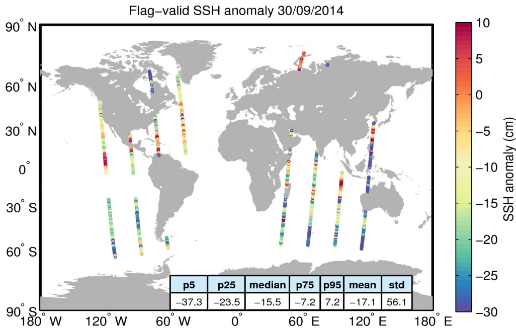
Figure 5. Geographical distribution of flag-valid 1-Hz SSH anomaly data over oceans and lakes for 30/09/2014. The statistical values shown in the table refer to the SSH anomaly in cm and are calculated over all measurements shown in the figure.
