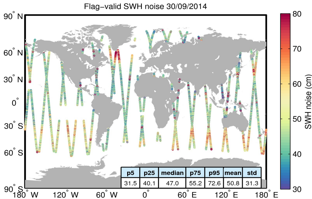
Figure 18. Geographical distribution of flag-valid 20-Hz SWH measurement noise over oceans and lakes for 30/09/2014. The statistical values shown in the figure refer to the SWH noise and are calculated over all measurements shown in the figure.
