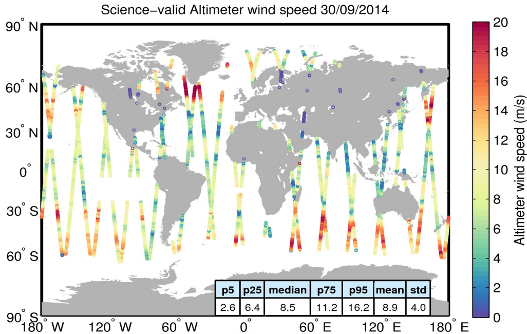
Figure 34. Geographical distribution of science-valid wind data over oceans and lakes for 30/09/2014. The statistical values shown in the table refer to the wind in m/s and are calculated over all measurements shown in the figure. Gray circles denote records that have been rejected based on the editing criteria described in Table 5.
