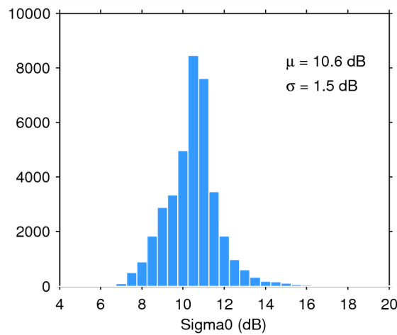
Figure 28. Histogram of science-valid sigma0 over oceans and lakes for 30/09/2014. The mean ( \mu ) and standard deviation ( \sigma ) are also shown. Note that values outside [4 20] dB are excluded from the histogram for the sake of readability but not from the computation of \mu and \sigma .
