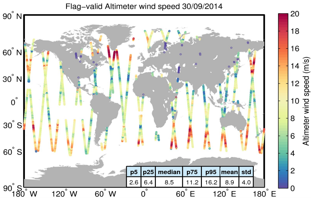
Figure 31. Geographical distribution of flag-valid wind data over oceans and lakes for 30/09/2014. The statistical values shown in the table refer to the wind in m/s and are calculated over all measurements shown in the figure.
