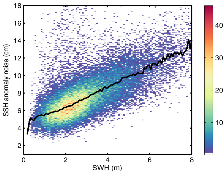
Figure 9. 2D histogram showing flag-valid SSH anomaly noise as a function of SWH for 29/09/2014. The black line denotes the median SSH anomaly as a function of SWH.
