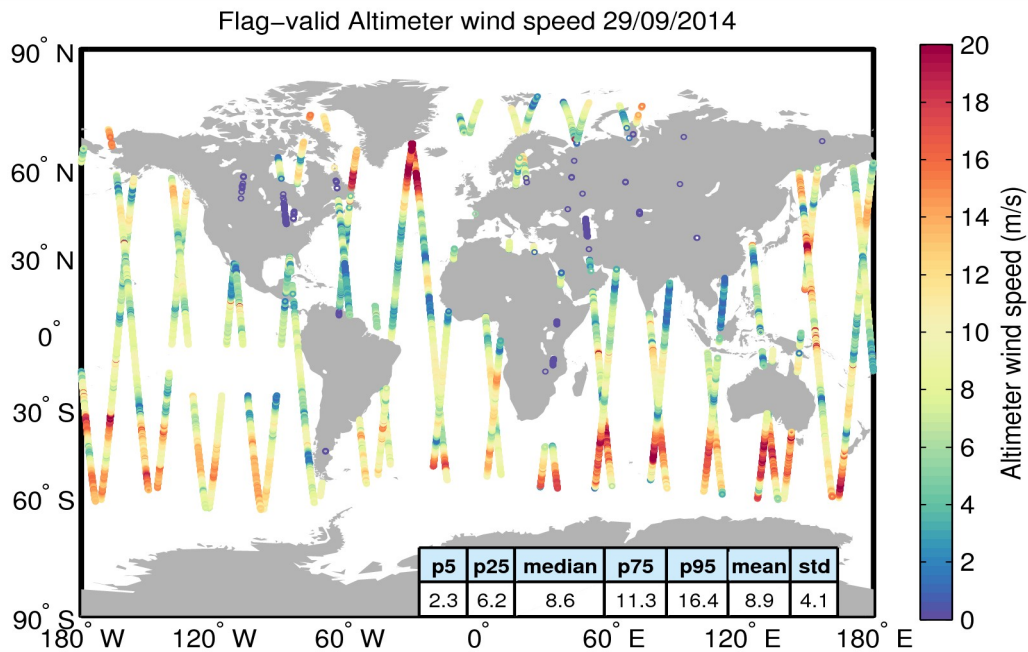
Figure 31. Geographical distribution of flag-valid wind data over oceans and lakes for 29/09/2014. The statistical values shown in the table refer to the wind in m/s and are calculated over all measurements shown in the figure.
