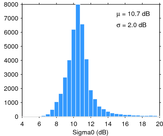
Figure 25. Histogram of flag-valid sigma0 over oceans and lakes for 29/09/2014. The mean ( \mu ) and standard deviation ( \sigma ) are also shown. Note that values outside [4 20] dB are excluded from the histogram for the sake of readability but not from the computation of \mu and \sigma .
