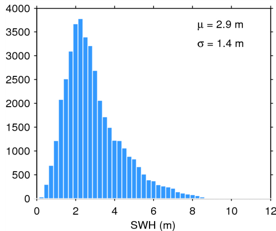
Figure 20. Histogram of science-valid SWH over oceans and lakes for 29/09/2014. The mean ( \mu ) and standard deviation ( \sigma ) are also shown. Note that values larger than 12 m are excluded from the histogram for the sake of readability but not from the computation of \mu and \sigma .
