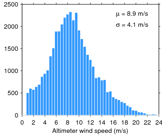
Figure 33. Histogram of flag-valid wind over oceans and lakes for 29/09/2014. The mean ( \mu ) and standard deviation ( \sigma ) are also shown. Note that values larger than 24 m/s are excluded from the histogram for the sake of readability but not from the computation of \mu and \sigma .
