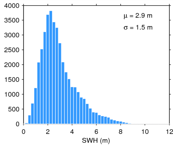
Figure 17. Histogram of flag-valid SWH over oceans and lakes for 29/09/2014. The mean ( \mu ) and standard deviation ( \sigma ) are also shown. Note that values larger than 12 m are excluded from the histogram for the sake of readability but not from the computation of \mu and \sigma .
