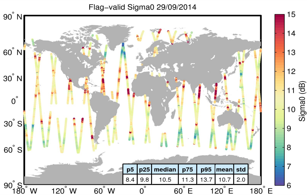
Figure 23. Geographical distribution of flag-valid sigma0 data over oceans and lakes for 29/09/2014. The statistical values shown in the table refer to the sigma0 in dB and are calculated over all measurements shown in the figure.
