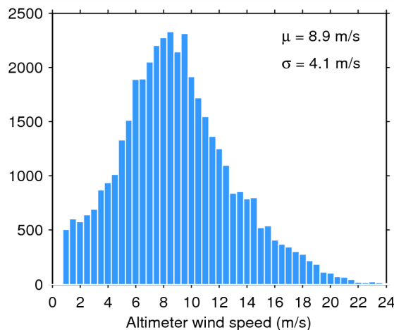
Figure 35. Histogram of science-valid wind over oceans and lakes for 29/09/2014. The mean ( \mu ) and standard deviation ( \sigma ) are also shown. Note that values larger than 24 m/s are excluded from the histogram for the sake of readability but not from the computation of \mu and \sigma .
