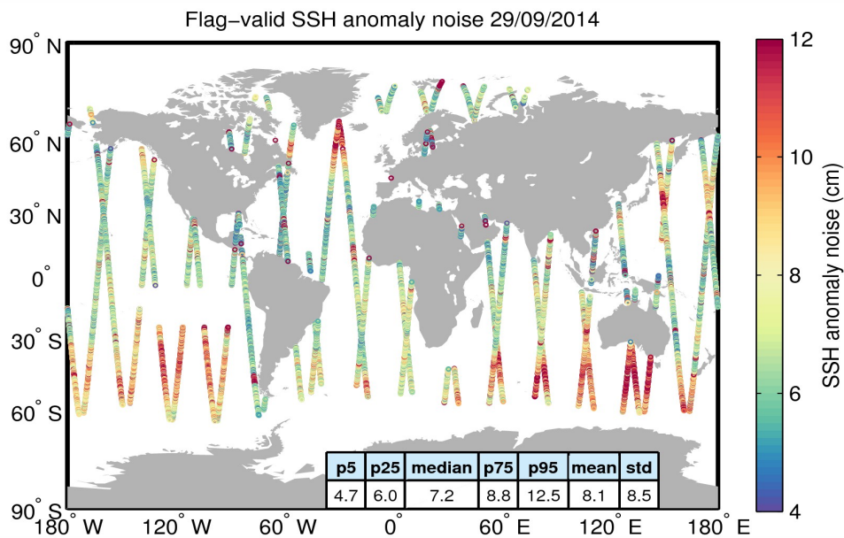
Figure 8. Geographical distribution of flag-valid 20-Hz SSH anomaly measurement noise over oceans and lakes for 29/09/2014. The statistical values shown in the table refer to the SSH anomaly noise and are calculated over all measurements shown in the figure.
