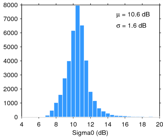
Figure 28. Histogram of science-valid sigma0 over oceans and lakes for 29/09/2014. The mean ( \mu ) and standard deviation ( \sigma ) are also shown. Note that values outside [4 20] dB are excluded from the histogram for the sake of readability but not from the computation of \mu and \sigma .
