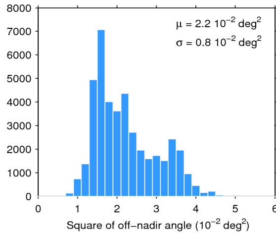
Figure 39. Histogram of flag-valid mispointing over oceans and lakes for 29/09/2014. The mean ( \mu ) and standard deviation ( \sigma ) are also shown. Note that values than 6 \cdot 10^{-2} \text{ deg}^2 are excluded from the histogram for the sake of readability but not from the computation of \mu and \sigma .
