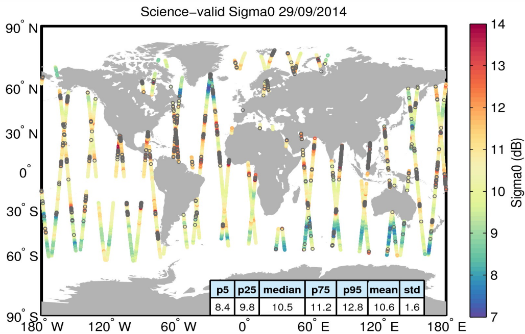
Figure 27. Geographical distribution of science-valid sigma0 data over oceans and lakes for 29/09/2014. The statistical values shown in the table refer to the sigma0 in dB and are calculated over all measurements shown in the figure. Gray circles denote records that have been rejected based on the editing criteria described in Table 4.
