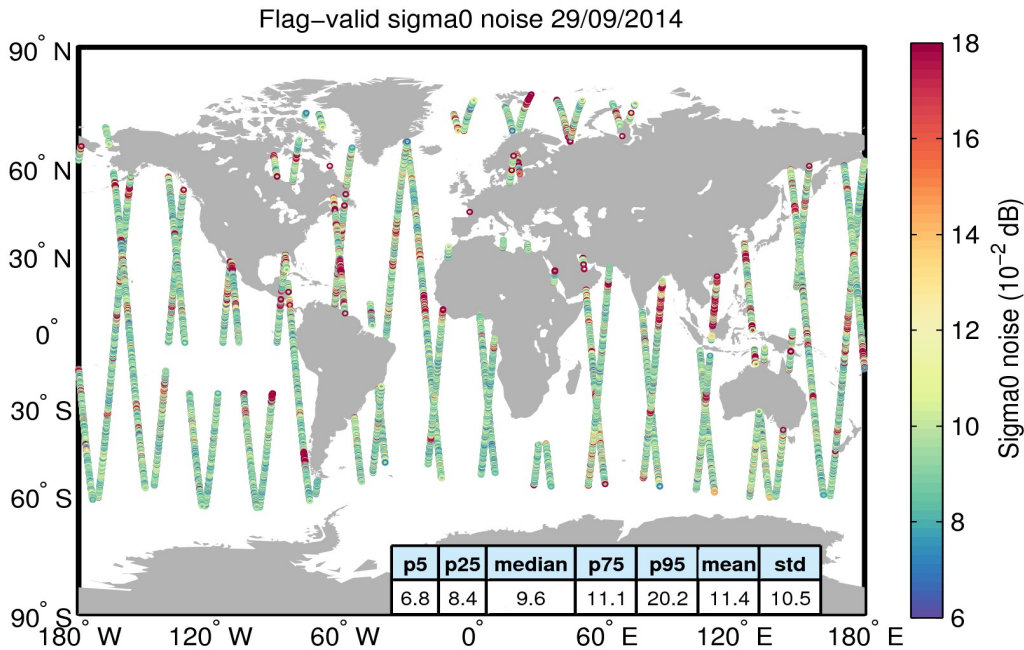
Figure 26. Geographical distribution of flag-valid 20-Hz sigma0 measurement noise over oceans and lakes for 29/09/2014. The statistical values shown in the table refer to the sigma0 noise and are calculated over all measurements shown in the figure.
