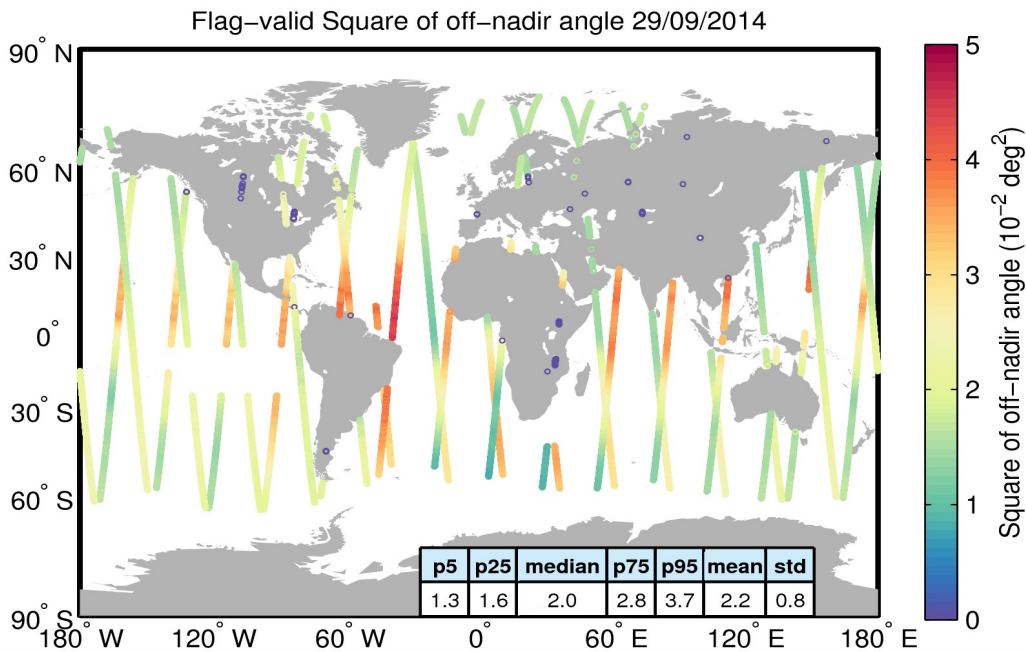
Figure 37. Geographical distribution of flag-valid mispointing data over oceans and lakes for 29/09/2014. The statistical values shown in the table refer to the mispointing in 10^{-2} \text{ deg}^2 and are calculated over all measurements shown in the figure.
