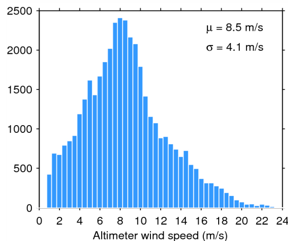
Figure 35. Histogram of science-valid wind over oceans and lakes for 28/09/2014. The mean ( \mu ) and standard deviation ( \sigma ) are also shown. Note that values larger than 24 m/s are excluded from the histogram for the sake of readability but not from the computation of \mu and \sigma .
