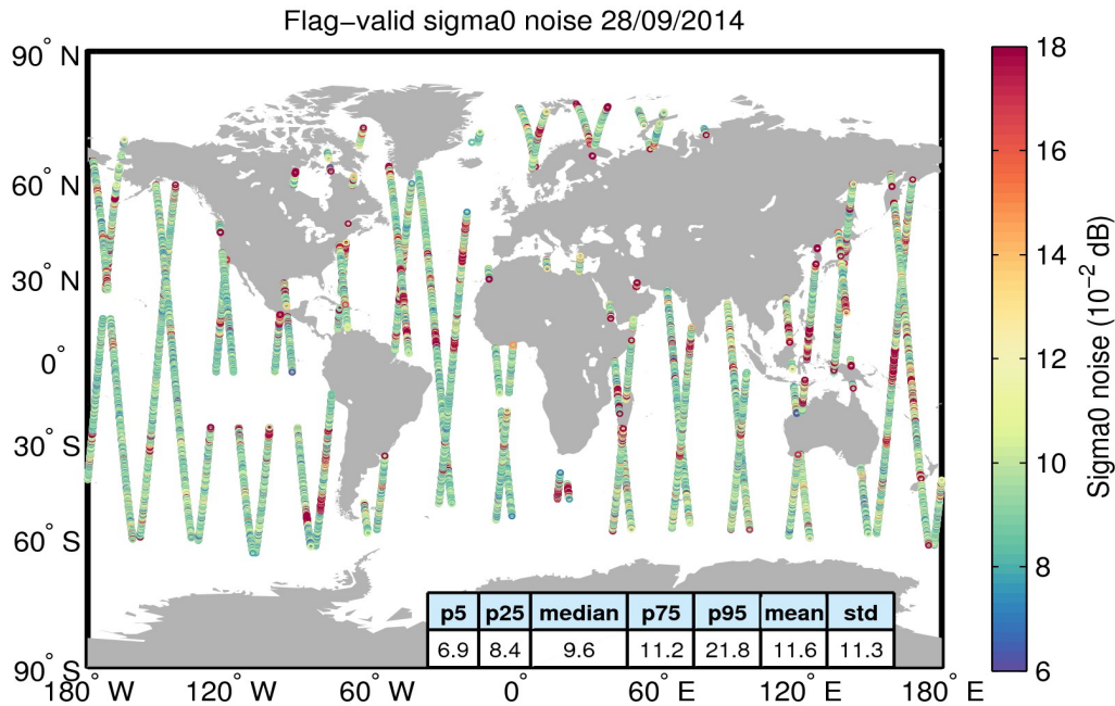
Figure 26. Geographical distribution of flag-valid 20-Hz sigma0 measurement noise over oceans and lakes for 28/09/2014. The statistical values shown in the table refer to the sigma0 noise and are calculated over all measurements shown in the figure.
