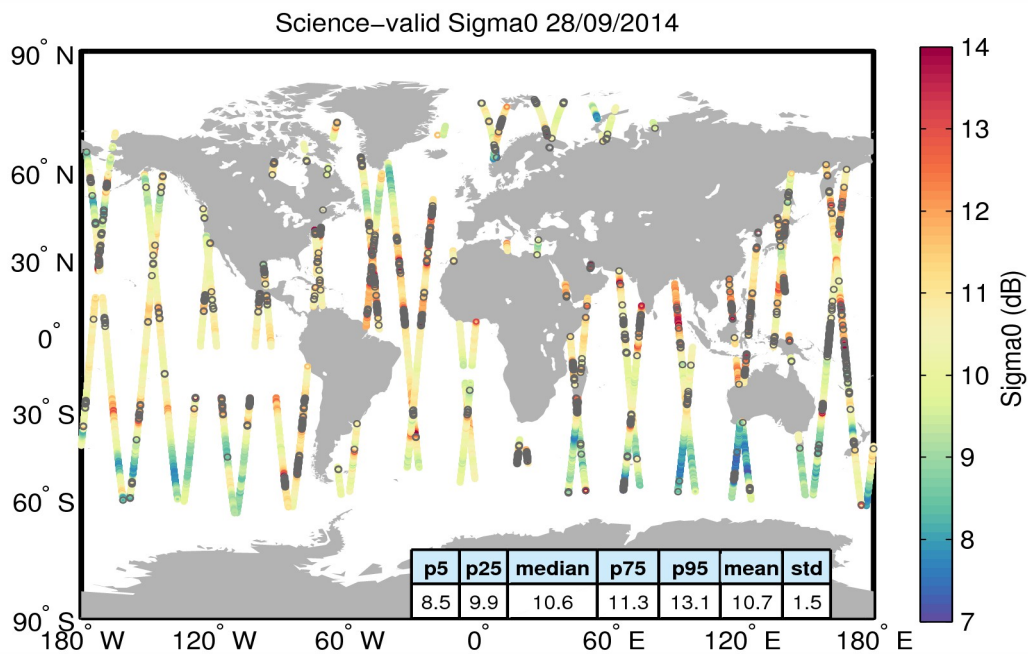
Figure 27. Geographical distribution of science-valid sigma0 data over oceans and lakes for 28/09/2014. The statistical values shown in the table refer to the sigma0 in dB and are calculated over all measurements shown in the figure. Gray circles denote records that have been rejected based on the editing criteria described in Table 4.
