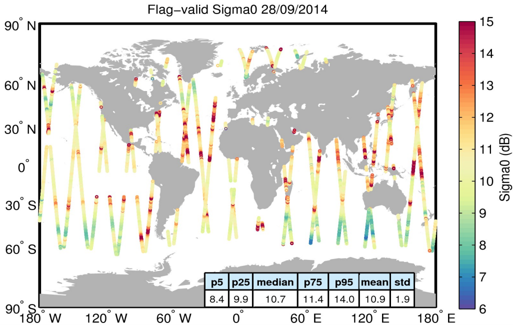
Figure 23. Geographical distribution of flag-valid sigma0 data over oceans and lakes for 28/09/2014. The statistical values shown in the table refer to the sigma0 in dB and are calculated over all measurements shown in the figure.
