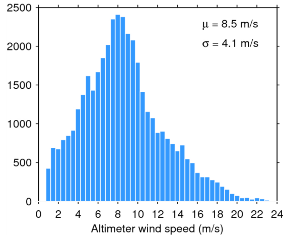
Figure 33. Histogram of flag-valid wind over oceans and lakes for 28/09/2014. The mean ( \mu ) and standard deviation ( \sigma ) are also shown. Note that values larger than 24 m/s are excluded from the histogram for the sake of readability but not from the computation of \mu and \sigma .
