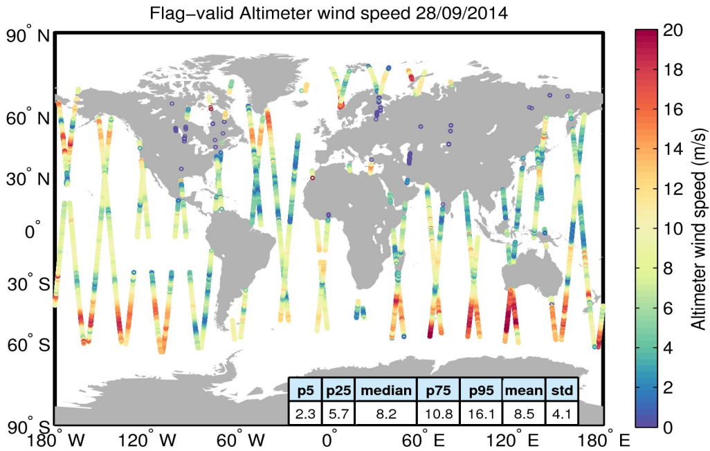
Figure 31. Geographical distribution of flag-valid wind data over oceans and lakes for 28/09/2014. The statistical values shown in the table refer to the wind in m/s and are calculated over all measurements shown in the figure.
