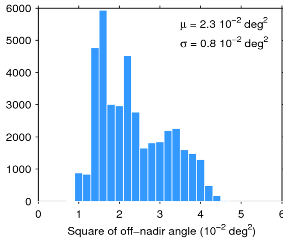
Figure 39. Histogram of flag-valid mispointing over oceans and lakes for 28/09/2014. The mean ( \mu ) and standard deviation ( \sigma ) are also shown. Note that values than 6 \cdot 10^{-2} \text{ deg}^2 are excluded from the histogram for the sake of readability but not from the computation of \mu and \sigma .
