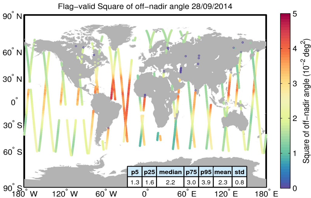
Figure 37. Geographical distribution of flag-valid mispointing data over oceans and lakes for 28/09/2014. The statistical values shown in the table refer to the mispointing in 10^{-2} \text{ deg}^2 and are calculated over all measurements shown in the figure.
