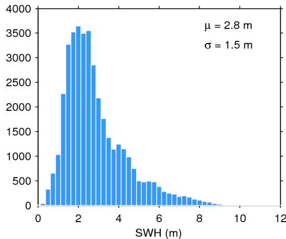
Figure 20. Histogram of science-valid SWH over oceans and lakes for 28/09/2014. The mean ( \mu ) and standard deviation ( \sigma ) are also shown. Note that values larger than 12 m are excluded from the histogram for the sake of readability but not from the computation of \mu and \sigma .
