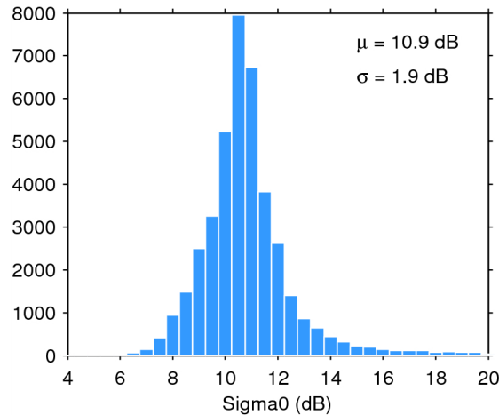
Figure 25. Histogram of flag-valid sigma0 over oceans and lakes for 28/09/2014. The mean ( \mu ) and standard deviation ( \sigma ) are also shown. Note that values outside [4 20] dB are excluded from the histogram for the sake of readability but not from the computation of \mu and \sigma .
