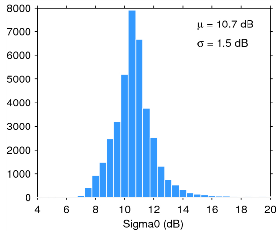
Figure 28. Histogram of science-valid sigma0 over oceans and lakes for 28/09/2014. The mean ( \mu ) and standard deviation ( \sigma ) are also shown. Note that values outside [4 20] dB are excluded from the histogram for the sake of readability but not from the computation of \mu and \sigma .
