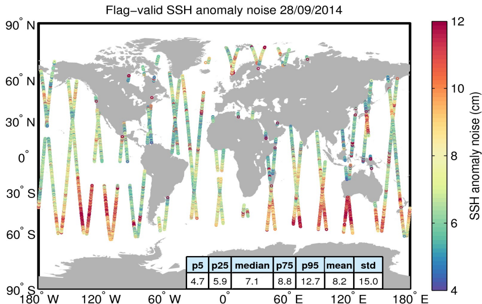
Figure 8. Geographical distribution of flag-valid 20-Hz SSH anomaly measurement noise over oceans and lakes for 28/09/2014. The statistical values shown in the table refer to the SSH anomaly noise and are calculated over all measurements shown in the figure.
