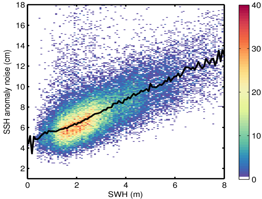
Figure 9. 2D histogram showing flag-valid SSH anomaly noise as a function of SWH for 28/09/2014. The black line denotes the median SSH anomaly as a function of SWH.
