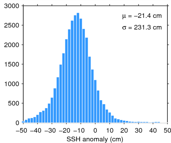
Figure 7. Histogram of flag-valid SSH anomaly over oceans and lakes for 27/09/2014. The mean ( \mu ) and standard deviation ( \sigma ) are also shown. Note that values outside [-50\ 50] cm are excluded from the histogram for the sake of readability but not from the computation of \mu and \sigma .
