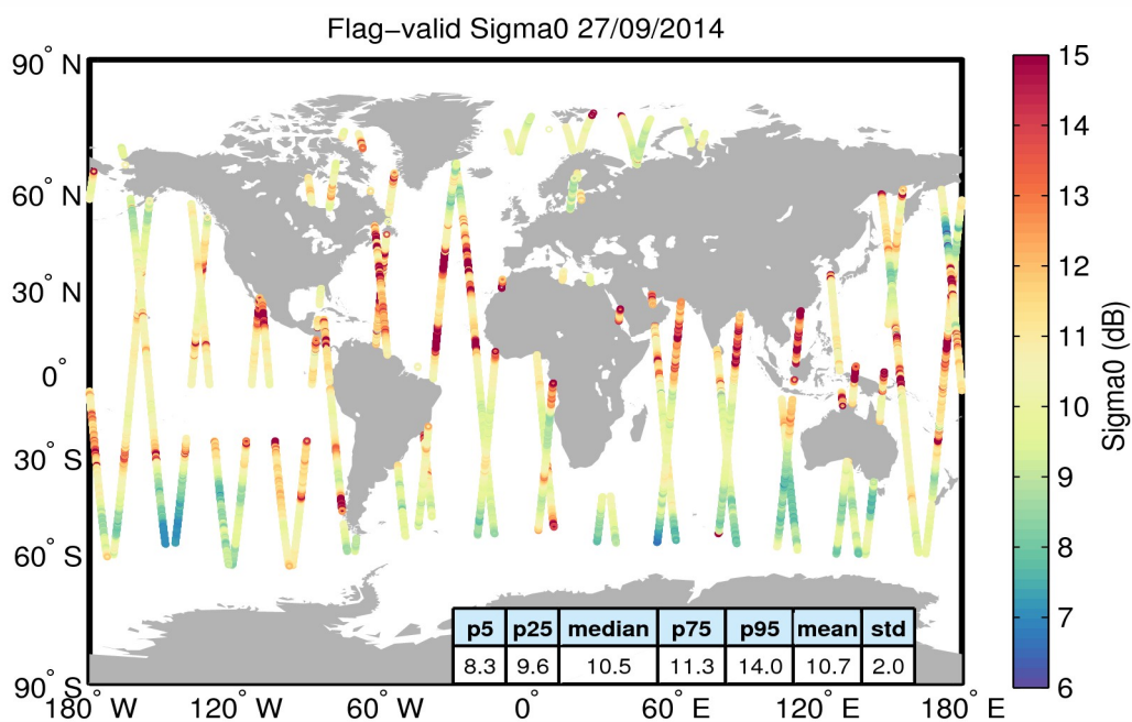
Figure 23. Geographical distribution of flag-valid sigma0 data over oceans and lakes for 27/09/2014. The statistical values shown in the table refer to the sigma0 in dB and are calculated over all measurements shown in the figure.
