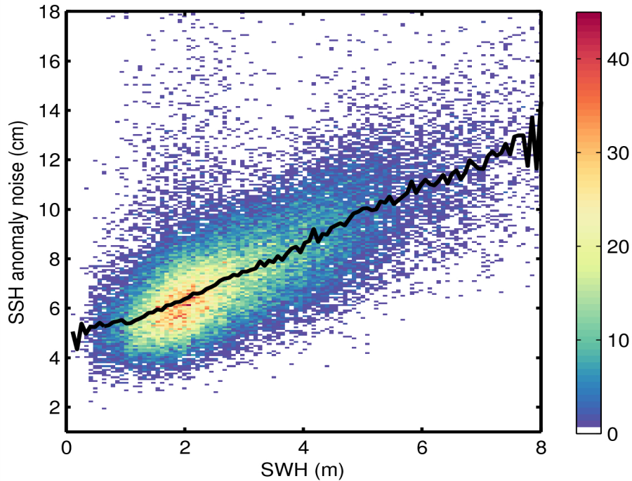
Figure 9. 2D histogram showing flag-valid SSH anomaly noise as a function of SWH for 27/09/2014. The black line denotes the median SSH anomaly as a function of SWH.
