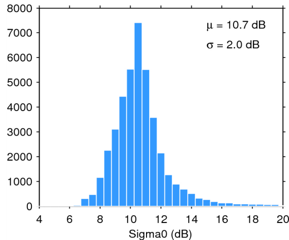
Figure 25. Histogram of flag-valid sigma0 over oceans and lakes for 27/09/2014. The mean ( \mu ) and standard deviation ( \sigma ) are also shown. Note that values outside [4 20] dB are excluded from the histogram for the sake of readability but not from the computation of \mu and \sigma .
