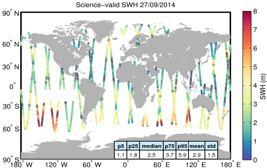
Figure 19. Geographical distribution of science-valid SWH data over oceans and lakes for 27/09/2014. The statistical values shown in the table refer to the SWH in m and are calculated over all measurements shown in the figure. Gray circles denote records that have been rejected based on the editing criteria described in Table 3.
