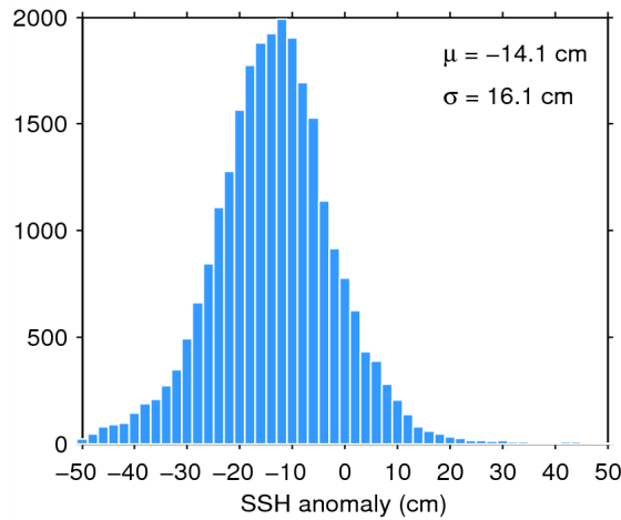
Figure 11. Histogram of science-valid SSH anomaly over oceans and lakes for 27/09/2014. The mean ( \mu ) and standard deviation ( \sigma ) are also shown. Note that values outside [-50 50] cm are excluded from the histogram for the sake of readability but not from the computation of \mu and \sigma .
