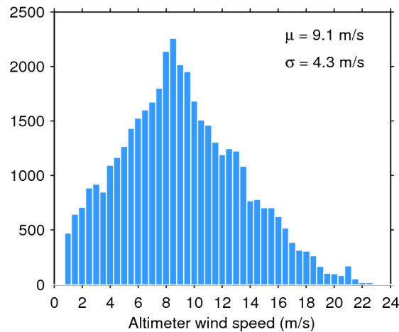
Figure 33. Histogram of flag-valid wind over oceans and lakes for 27/09/2014. The mean ( \mu ) and standard deviation ( \sigma ) are also shown. Note that values larger than 24 m/s are excluded from the histogram for the sake of readability but not from the computation of \mu and \sigma .
