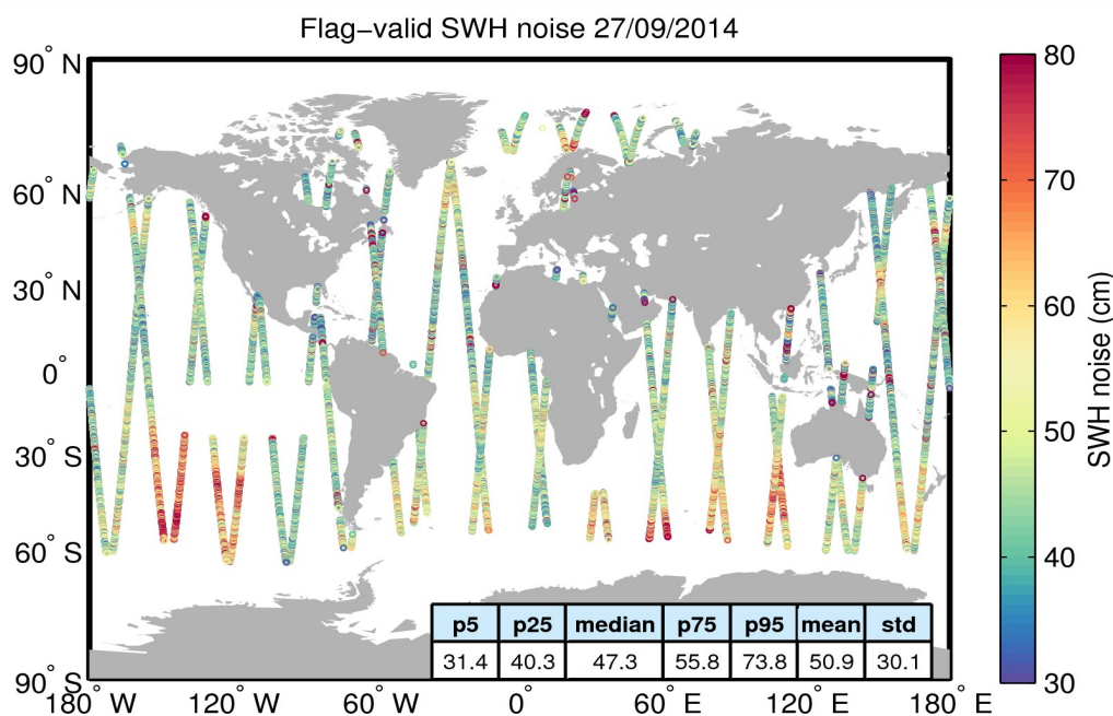
Figure 18. Geographical distribution of flag-valid 20-Hz SWH measurement noise over oceans and lakes for 27/09/2014. The statistical values shown in the figure refer to the SWH noise and are calculated over all measurements shown in the figure.
