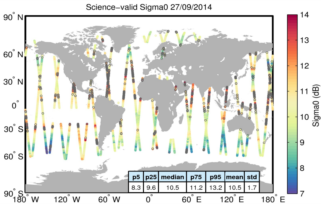
Figure 27. Geographical distribution of science-valid sigma0 data over oceans and lakes for 27/09/2014. The statistical values shown in the table refer to the sigma0 in dB and are calculated over all measurements shown in the figure. Gray circles denote records that have been rejected based on the editing criteria described in Table 4.
