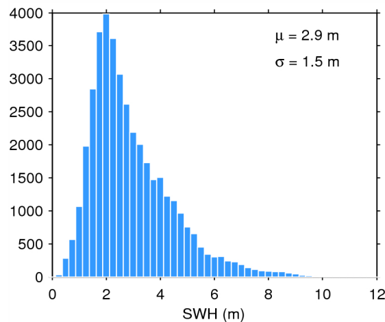
Figure 20. Histogram of science-valid SWH over oceans and lakes for 27/09/2014. The mean ( \mu ) and standard deviation ( \sigma ) are also shown. Note that values larger than 12 m are excluded from the histogram for the sake of readability but not from the computation of \mu and \sigma .
