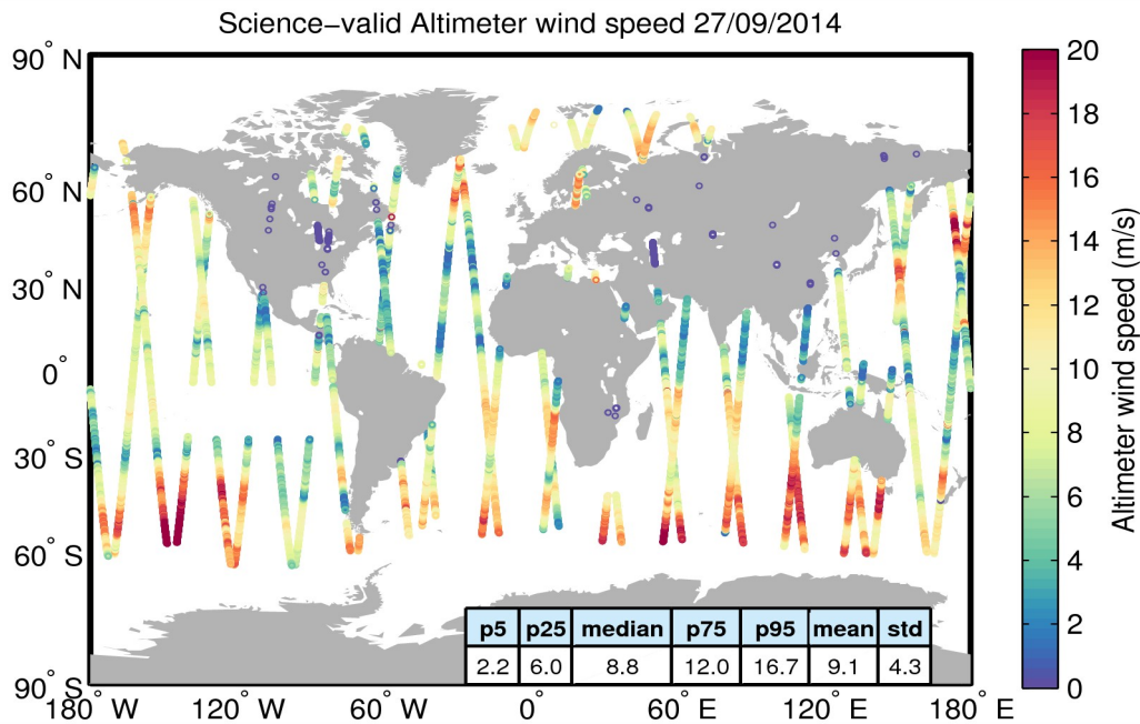
Figure 34. Geographical distribution of science-valid wind data over oceans and lakes for 27/09/2014. The statistical values shown in the table refer to the wind in m/s and are calculated over all measurements shown in the figure. Gray circles denote records that have been rejected based on the editing criteria described in Table 5.
