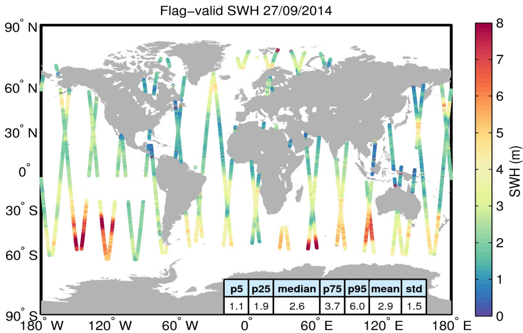
Figure 15. Geographical distribution of flag-valid SWH data over oceans and lakes for 27/09/2014. The statistical values shown in the table refer to the SWH in m and are calculated over all measurements shown in the figure.
