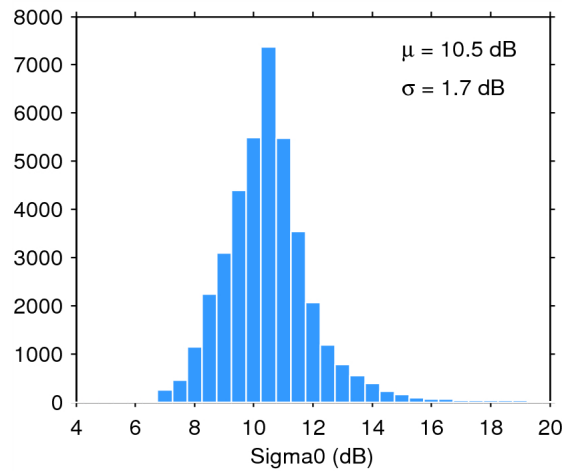
Figure 28. Histogram of science-valid sigma0 over oceans and lakes for 27/09/2014. The mean ( \mu ) and standard deviation ( \sigma ) are also shown. Note that values outside [4 20] dB are excluded from the histogram for the sake of readability but not from the computation of \mu and \sigma .
