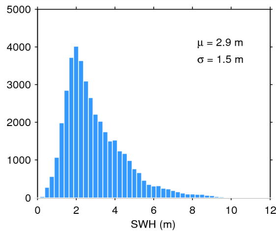
Figure 17. Histogram of flag-valid SWH over oceans and lakes for 27/09/2014. The mean ( \mu ) and standard deviation ( \sigma ) are also shown. Note that values larger than 12 m are excluded from the histogram for the sake of readability but not from the computation of \mu and \sigma .
