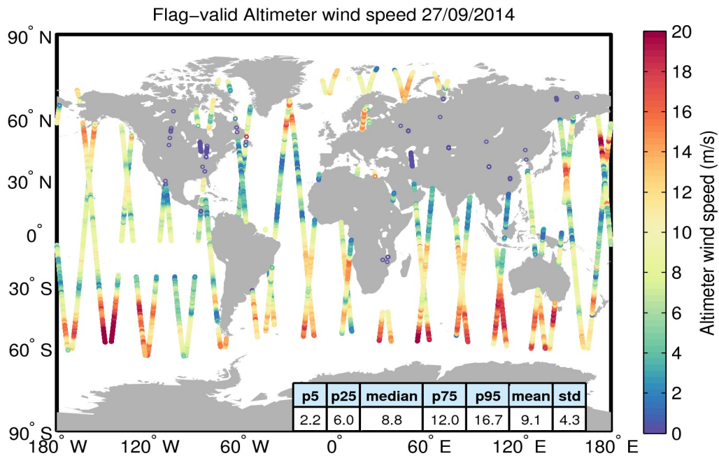
Figure 31. Geographical distribution of flag-valid wind data over oceans and lakes for 27/09/2014. The statistical values shown in the table refer to the wind in m/s and are calculated over all measurements shown in the figure.
