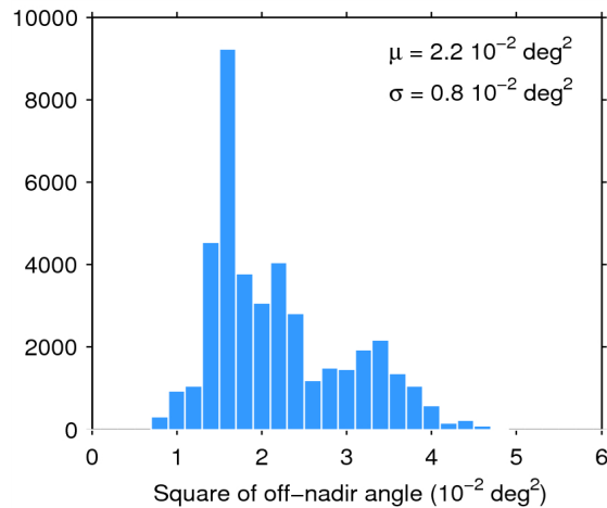
Figure 39. Histogram of flag-valid mispointing over oceans and lakes for 27/09/2014. The mean ( \mu ) and standard deviation ( \sigma ) are also shown. Note that values than 6 \cdot 10^{-2} \text{ deg}^2 are excluded from the histogram for the sake of readability but not from the computation of \mu and \sigma .
