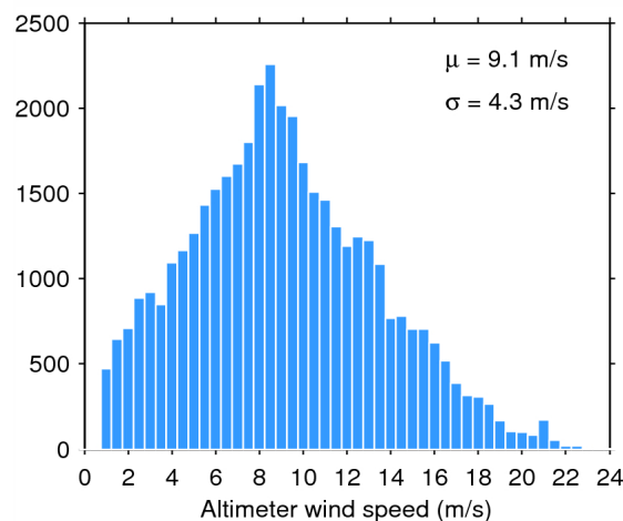
Figure 35. Histogram of science-valid wind over oceans and lakes for 27/09/2014. The mean ( \mu ) and standard deviation ( \sigma ) are also shown. Note that values larger than 24 m/s are excluded from the histogram for the sake of readability but not from the computation of \mu and \sigma .
