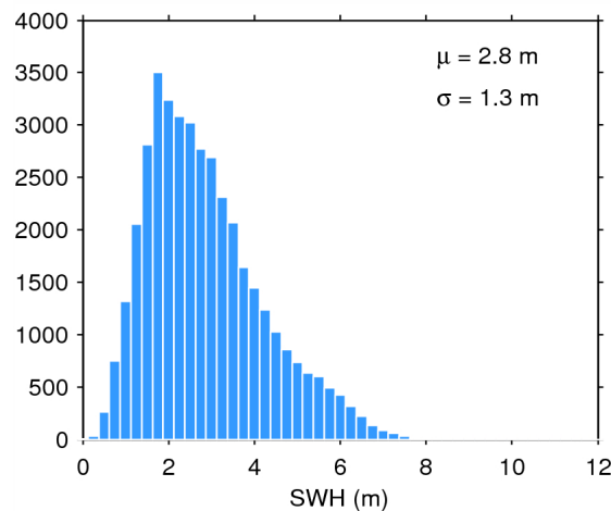
Figure 20. Histogram of science-valid SWH over oceans and lakes for 25/09/2014. The mean ( \mu ) and standard deviation ( \sigma ) are also shown. Note that values larger than 12 m are excluded from the histogram for the sake of readability but not from the computation of \mu and \sigma .
