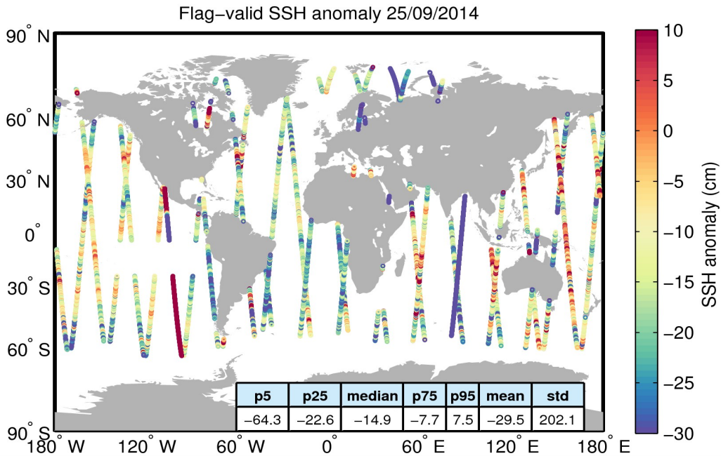
Figure 5. Geographical distribution of flag-valid 1-Hz SSH anomaly data over oceans and lakes for 25/09/2014. The statistical values shown in the table refer to the SSH anomaly in cm and are calculated over all measurements shown in the figure.
