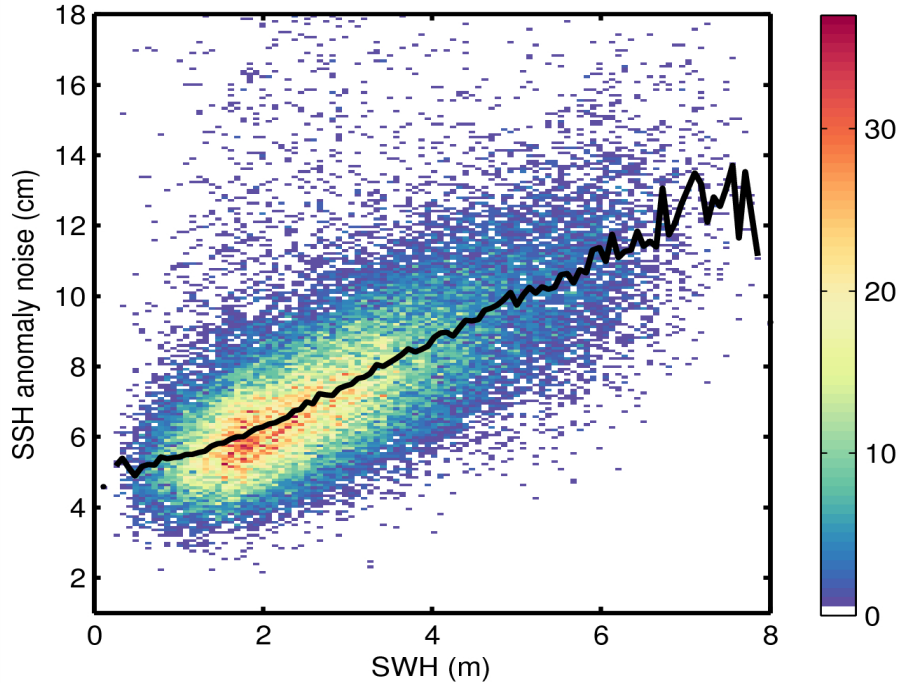
Figure 9. 2D histogram showing flag-valid SSH anomaly noise as a function of SWH for 25/09/2014. The black line denotes the median SSH anomaly as a function of SWH.
