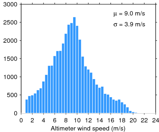
Figure 33. Histogram of flag-valid wind over oceans and lakes for 25/09/2014. The mean ( \mu ) and standard deviation ( \sigma ) are also shown. Note that values larger than 24 m/s are excluded from the histogram for the sake of readability but not from the computation of \mu and \sigma .
