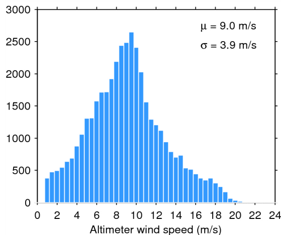
Figure 35. Histogram of science-valid wind over oceans and lakes for 25/09/2014. The mean ( \mu ) and standard deviation ( \sigma ) are also shown. Note that values larger than 24 m/s are excluded from the histogram for the sake of readability but not from the computation of \mu and \sigma .
