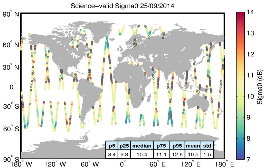
Figure 27. Geographical distribution of science-valid sigma0 data over oceans and lakes for 25/09/2014. The statistical values shown in the table refer to the sigma0 in dB and are calculated over all measurements shown in the figure. Gray circles denote records that have been rejected based on the editing criteria described in Table 4.
