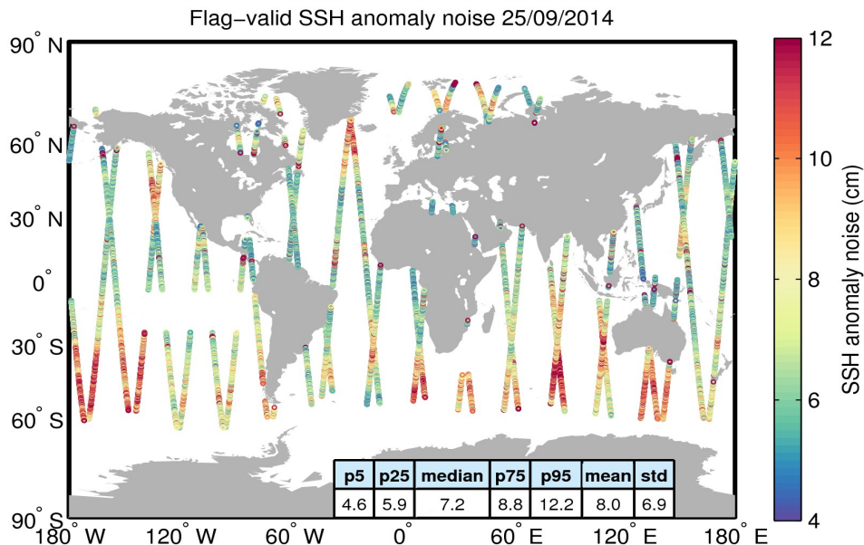
Figure 8. Geographical distribution of flag-valid 20-Hz SSH anomaly measurement noise over oceans and lakes for 25/09/2014. The statistical values shown in the table refer to the SSH anomaly noise and are calculated over all measurements shown in the figure.
