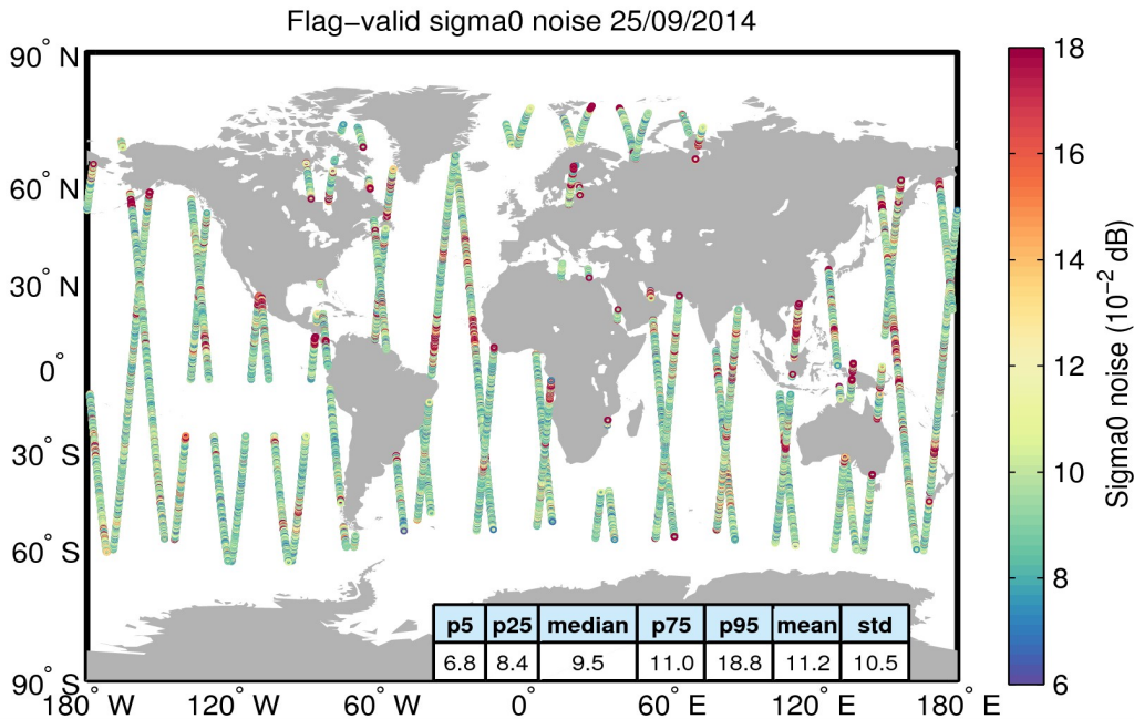
Figure 26. Geographical distribution of flag-valid 20-Hz sigma0 measurement noise over oceans and lakes for 25/09/2014. The statistical values shown in the table refer to the sigma0 noise and are calculated over all measurements shown in the figure.
