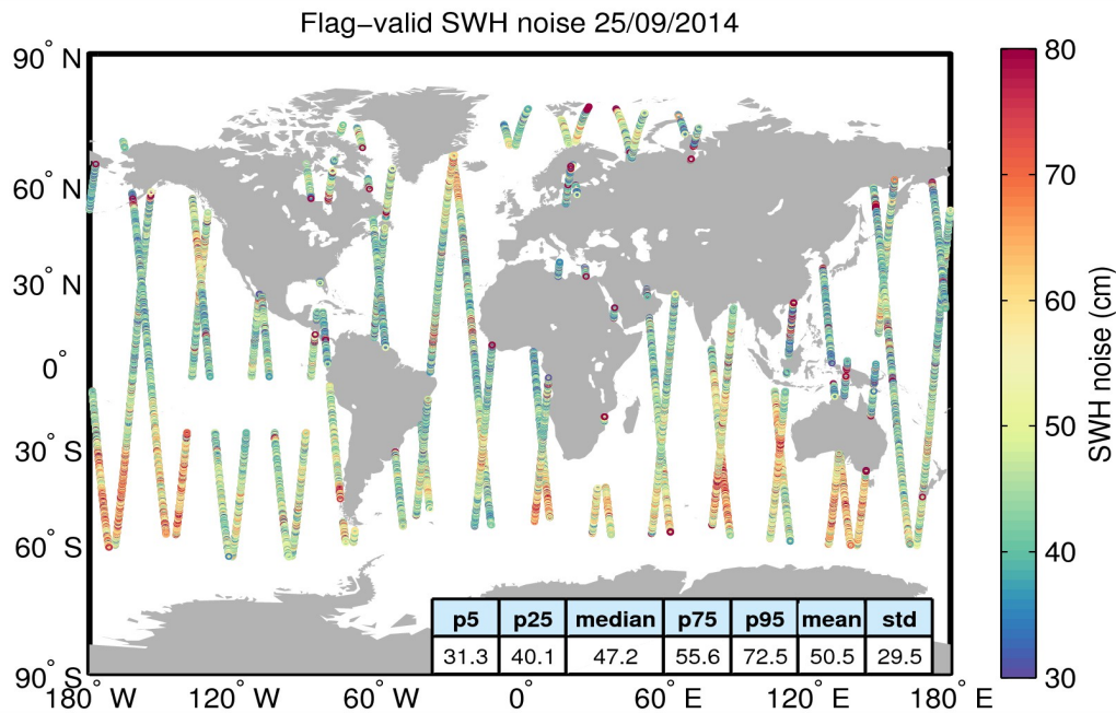
Figure 18. Geographical distribution of flag-valid 20-Hz SWH measurement noise over oceans and lakes for 25/09/2014. The statistical values shown in the figure refer to the SWH noise and are calculated over all measurements shown in the figure.
