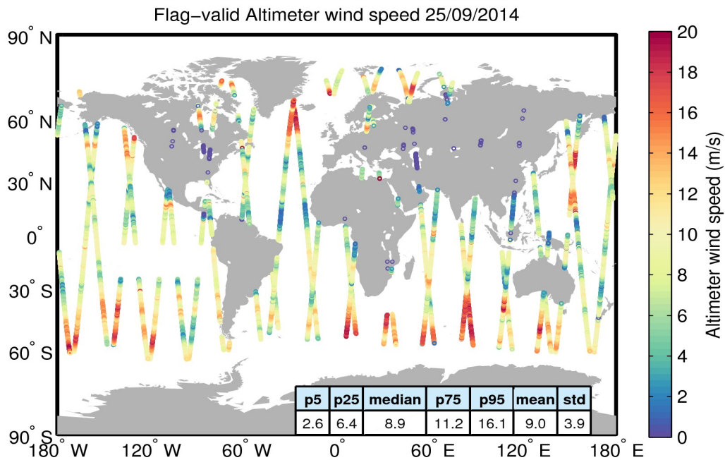
Figure 31. Geographical distribution of flag-valid wind data over oceans and lakes for 25/09/2014. The statistical values shown in the table refer to the wind in m/s and are calculated over all measurements shown in the figure.
