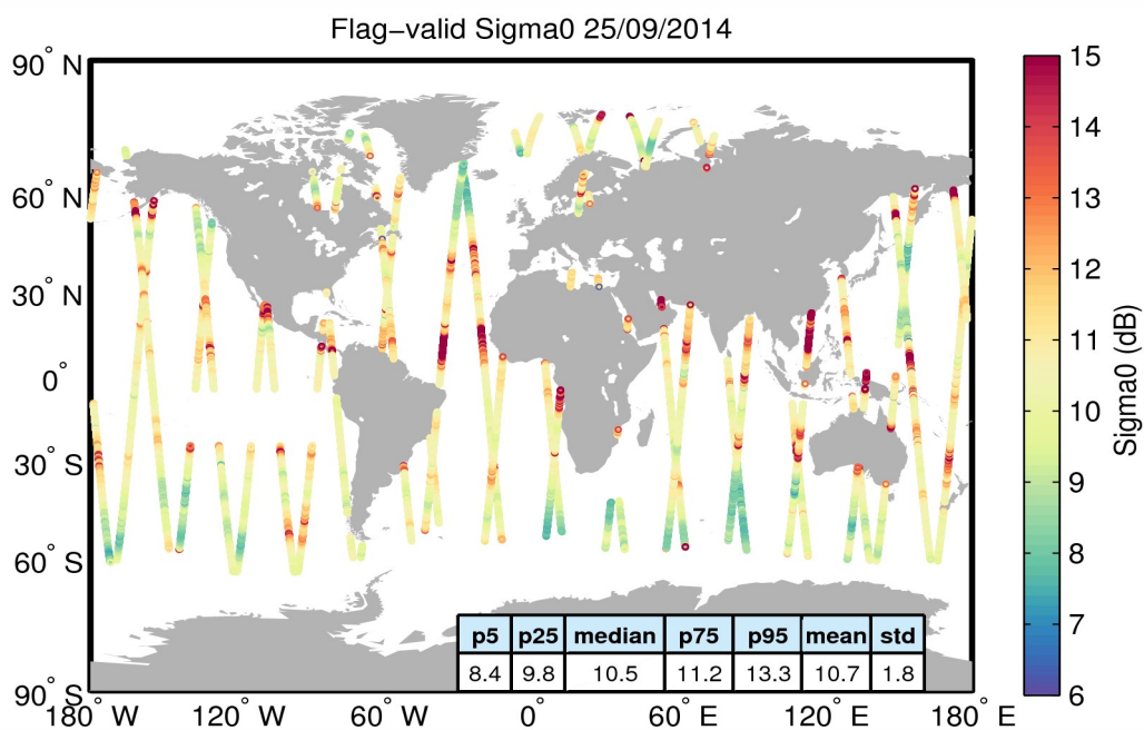
Figure 23. Geographical distribution of flag-valid sigma0 data over oceans and lakes for 25/09/2014. The statistical values shown in the table refer to the sigma0 in dB and are calculated over all measurements shown in the figure.
