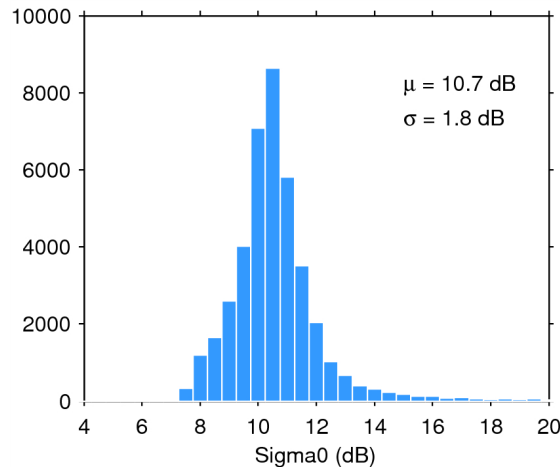
Figure 25. Histogram of flag-valid sigma0 over oceans and lakes for 25/09/2014. The mean ( \mu ) and standard deviation ( \sigma ) are also shown. Note that values outside [4 20] dB are excluded from the histogram for the sake of readability but not from the computation of \mu and \sigma .
