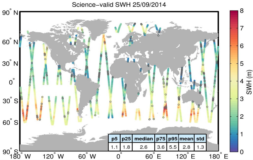
Figure 19. Geographical distribution of science-valid SWH data over oceans and lakes for 25/09/2014. The statistical values shown in the table refer to the SWH in m and are calculated over all measurements shown in the figure. Gray circles denote records that have been rejected based on the editing criteria described in Table 3.
