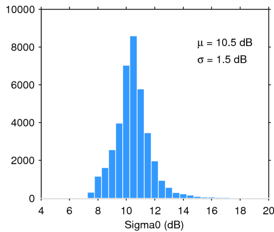
Figure 28. Histogram of science-valid sigma0 over oceans and lakes for 25/09/2014. The mean ( \mu ) and standard deviation ( \sigma ) are also shown. Note that values outside [4 20] dB are excluded from the histogram for the sake of readability but not from the computation of \mu and \sigma .
