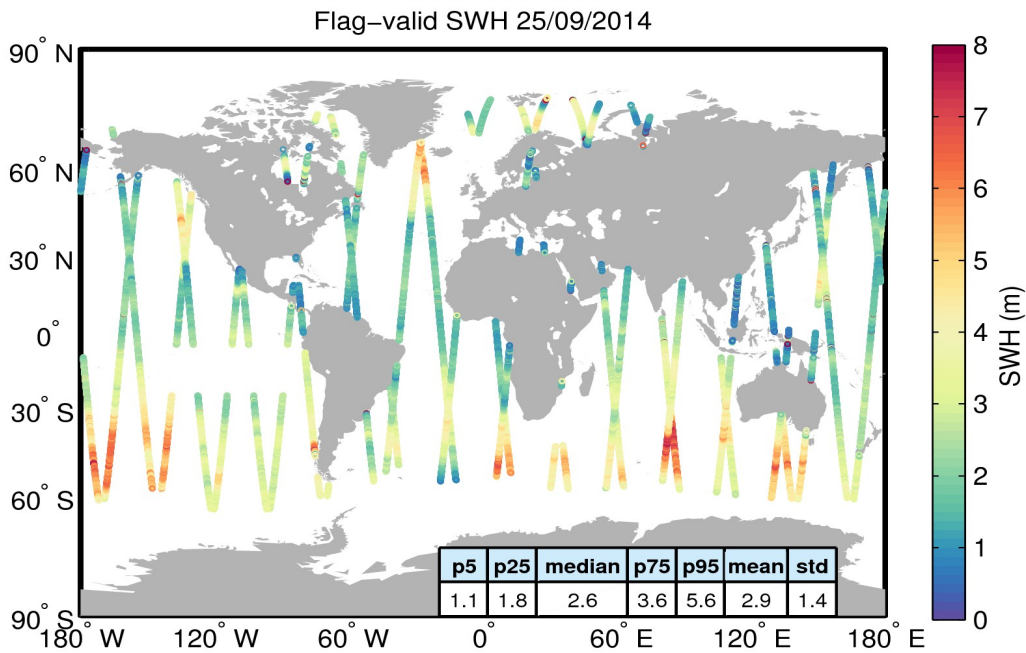
Figure 15. Geographical distribution of flag-valid SWH data over oceans and lakes for 25/09/2014. The statistical values shown in the table refer to the SWH in m and are calculated over all measurements shown in the figure.
