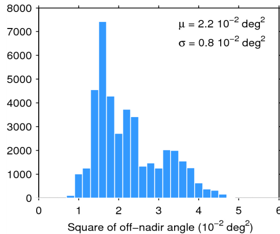
Figure 39. Histogram of flag-valid mispointing over oceans and lakes for 25/09/2014. The mean ( \mu ) and standard deviation ( \sigma ) are also shown. Note that values than 6 \cdot 10^{-2} \text{ deg}^2 are excluded from the histogram for the sake of readability but not from the computation of \mu and \sigma .
