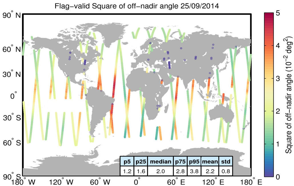
Figure 37. Geographical distribution of flag-valid mispointing data over oceans and lakes for 25/09/2014. The statistical values shown in the table refer to the mispointing in 10^{-2} \text{ deg}^2 and are calculated over all measurements shown in the figure.
