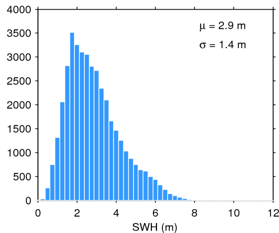
Figure 17. Histogram of flag-valid SWH over oceans and lakes for 25/09/2014. The mean ( \mu ) and standard deviation ( \sigma ) are also shown. Note that values larger than 12 m are excluded from the histogram for the sake of readability but not from the computation of \mu and \sigma .
