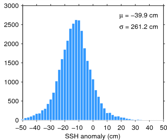
Figure 7. Histogram of flag-valid SSH anomaly over oceans and lakes for 24/09/2014. The mean ( \mu ) and standard deviation ( \sigma ) are also shown. Note that values outside [-50\ 50] cm are excluded from the histogram for the sake of readability but not from the computation of \mu and \sigma .
