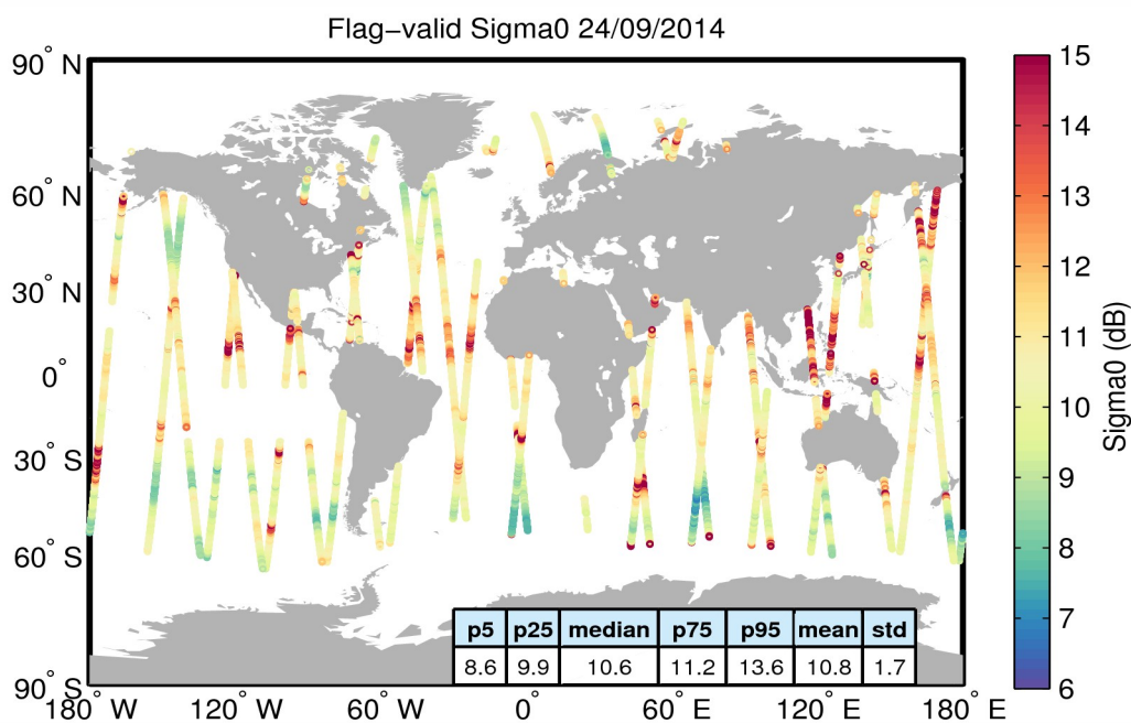
Figure 23. Geographical distribution of flag-valid sigma0 data over oceans and lakes for 24/09/2014. The statistical values shown in the table refer to the sigma0 in dB and are calculated over all measurements shown in the figure.
