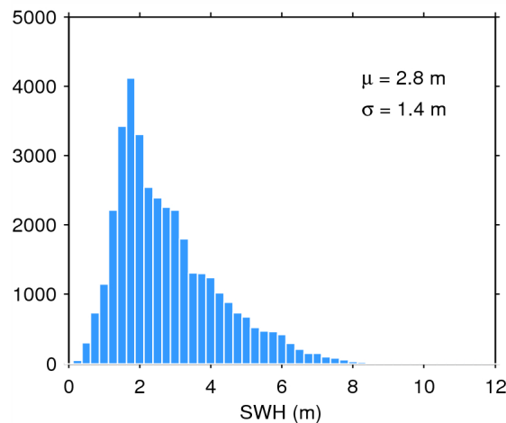
Figure 20. Histogram of science-valid SWH over oceans and lakes for 24/09/2014. The mean ( \mu ) and standard deviation ( \sigma ) are also shown. Note that values larger than 12 m are excluded from the histogram for the sake of readability but not from the computation of \mu and \sigma .
