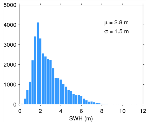
Figure 17. Histogram of flag-valid SWH over oceans and lakes for 24/09/2014. The mean ( \mu ) and standard deviation ( \sigma ) are also shown. Note that values larger than 12 m are excluded from the histogram for the sake of readability but not from the computation of \mu and \sigma .
