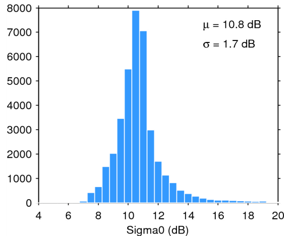
Figure 25. Histogram of flag-valid sigma0 over oceans and lakes for 24/09/2014. The mean ( \mu ) and standard deviation ( \sigma ) are also shown. Note that values outside [4 20] dB are excluded from the histogram for the sake of readability but not from the computation of \mu and \sigma .
