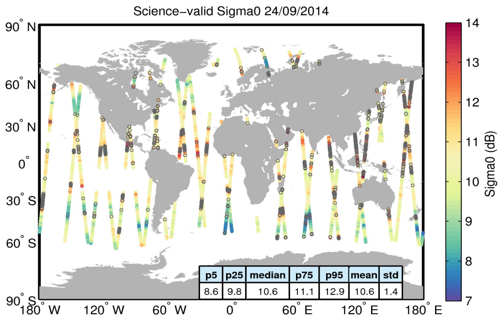
Figure 27. Geographical distribution of science-valid sigma0 data over oceans and lakes for 24/09/2014. The statistical values shown in the table refer to the sigma0 in dB and are calculated over all measurements shown in the figure. Gray circles denote records that have been rejected based on the editing criteria described in Table 4.
