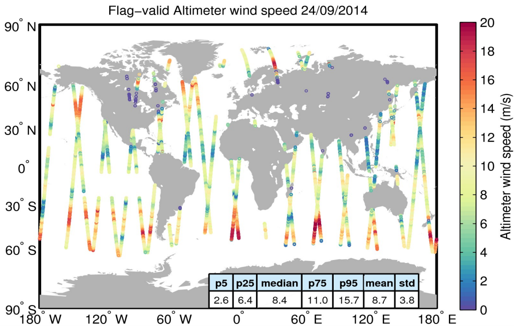
Figure 31. Geographical distribution of flag-valid wind data over oceans and lakes for 24/09/2014. The statistical values shown in the table refer to the wind in m/s and are calculated over all measurements shown in the figure.
