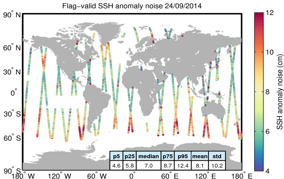
Figure 8. Geographical distribution of flag-valid 20-Hz SSH anomaly measurement noise over oceans and lakes for 24/09/2014. The statistical values shown in the table refer to the SSH anomaly noise and are calculated over all measurements shown in the figure.
