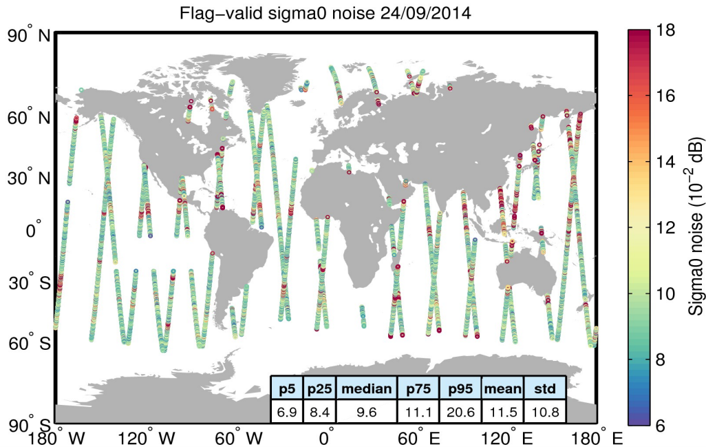
Figure 26. Geographical distribution of flag-valid 20-Hz sigma0 measurement noise over oceans and lakes for 24/09/2014. The statistical values shown in the table refer to the sigma0 noise and are calculated over all measurements shown in the figure.
