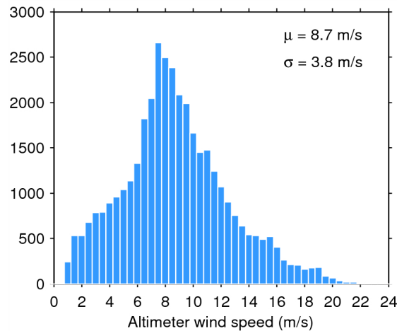
Figure 33. Histogram of flag-valid wind over oceans and lakes for 24/09/2014. The mean ( \mu ) and standard deviation ( \sigma ) are also shown. Note that values larger than 24 m/s are excluded from the histogram for the sake of readability but not from the computation of \mu and \sigma .
