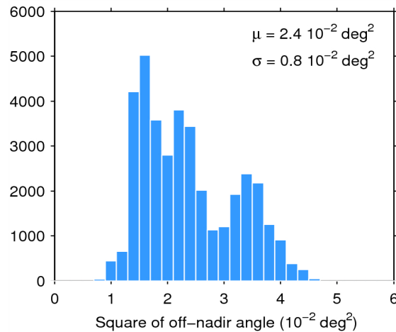
Figure 39. Histogram of flag-valid mispointing over oceans and lakes for 24/09/2014. The mean ( \mu ) and standard deviation ( \sigma ) are also shown. Note that values than 6 \cdot 10^{-2} \text{ deg}^2 are excluded from the histogram for the sake of readability but not from the computation of \mu and \sigma .
