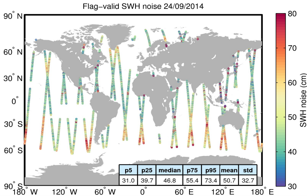
Figure 18. Geographical distribution of flag-valid 20-Hz SWH measurement noise over oceans and lakes for 24/09/2014. The statistical values shown in the figure refer to the SWH noise and are calculated over all measurements shown in the figure.
