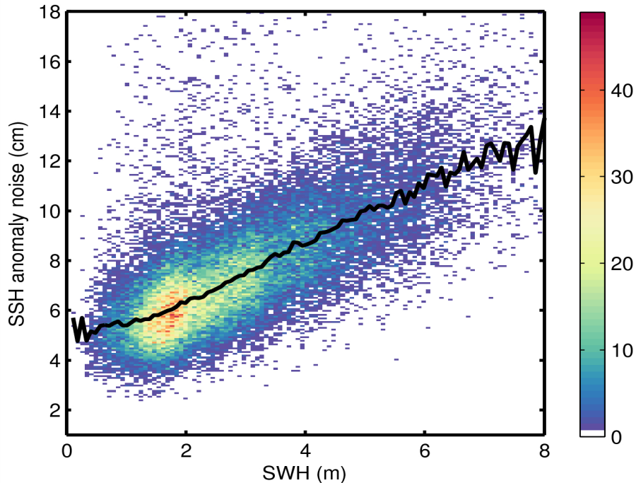
Figure 9. 2D histogram showing flag-valid SSH anomaly noise as a function of SWH for 24/09/2014. The black line denotes the median SSH anomaly as a function of SWH.
