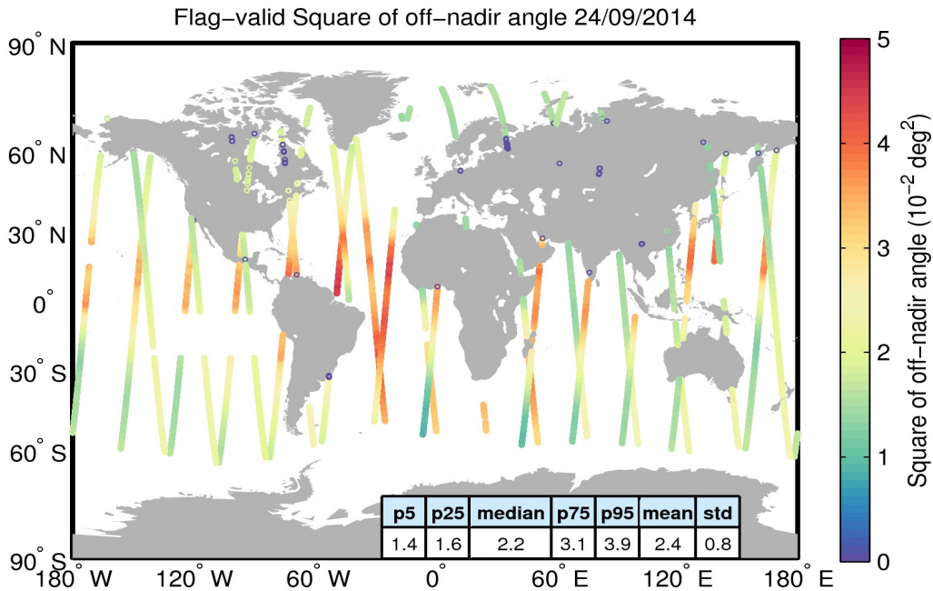
Figure 37. Geographical distribution of flag-valid mispointing data over oceans and lakes for 24/09/2014. The statistical values shown in the table refer to the mispointing in 10^{-2} \text{ deg}^2 and are calculated over all measurements shown in the figure.
