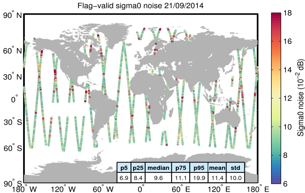
Figure 26. Geographical distribution of flag-valid 20-Hz sigma0 measurement noise over oceans and lakes for 21/09/2014. The statistical values shown in the table refer to the sigma0 noise and are calculated over all measurements shown in the figure.
