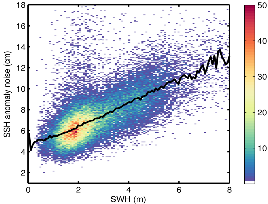
Figure 9. 2D histogram showing flag-valid SSH anomaly noise as a function of SWH for 21/09/2014. The black line denotes the median SSH anomaly as a function of SWH.
