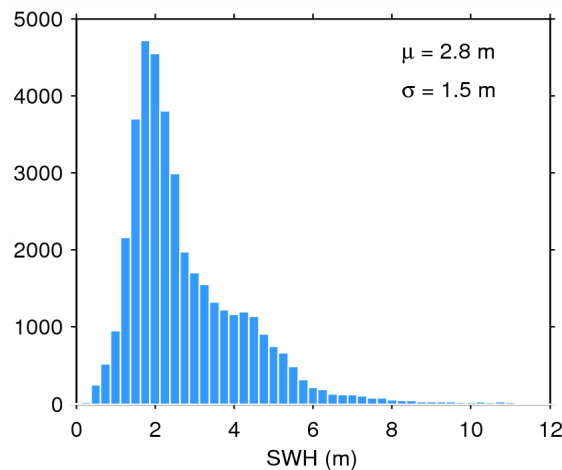
Figure 20. Histogram of science-valid SWH over oceans and lakes for 21/09/2014. The mean ( \mu ) and standard deviation ( \sigma ) are also shown. Note that values larger than 12 m are excluded from the histogram for the sake of readability but not from the computation of \mu and \sigma .
