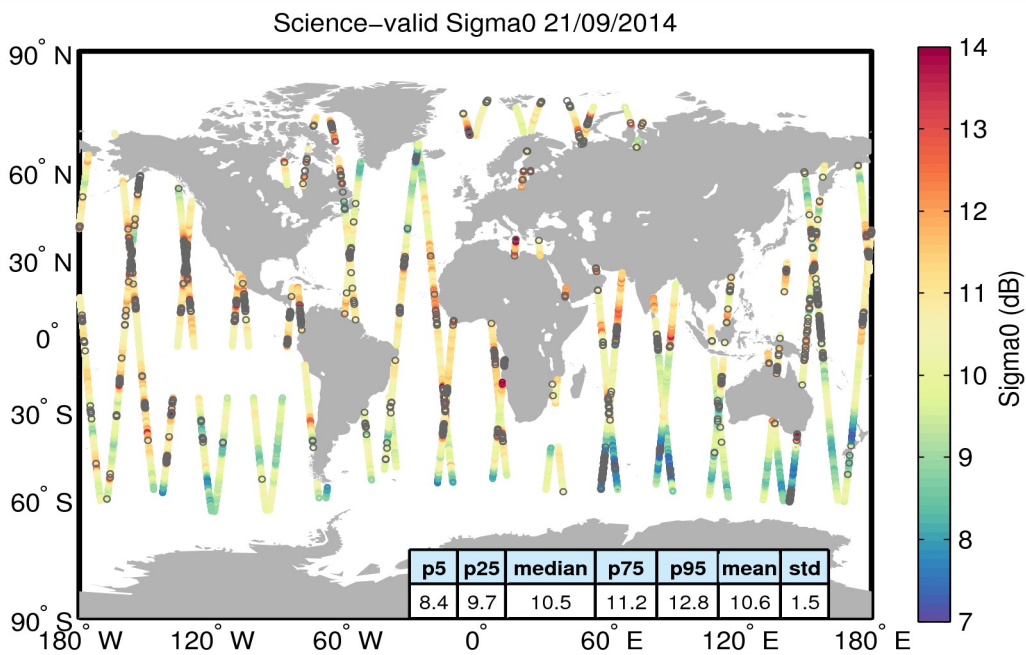
Figure 27. Geographical distribution of science-valid sigma0 data over oceans and lakes for 21/09/2014. The statistical values shown in the table refer to the sigma0 in dB and are calculated over all measurements shown in the figure. Gray circles denote records that have been rejected based on the editing criteria described in Table 4.
