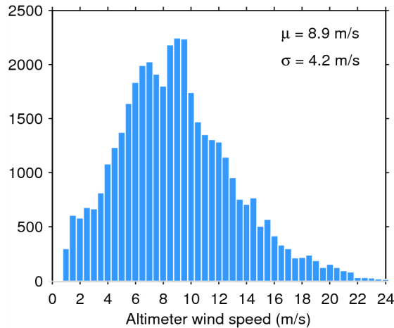
Figure 33. Histogram of flag-valid wind over oceans and lakes for 21/09/2014. The mean ( \mu ) and standard deviation ( \sigma ) are also shown. Note that values larger than 24 m/s are excluded from the histogram for the sake of readability but not from the computation of \mu and \sigma .
