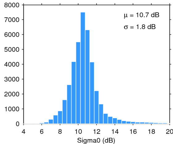
Figure 25. Histogram of flag-valid sigma0 over oceans and lakes for 21/09/2014. The mean ( \mu ) and standard deviation ( \sigma ) are also shown. Note that values outside [4 20] dB are excluded from the histogram for the sake of readability but not from the computation of \mu and \sigma .
