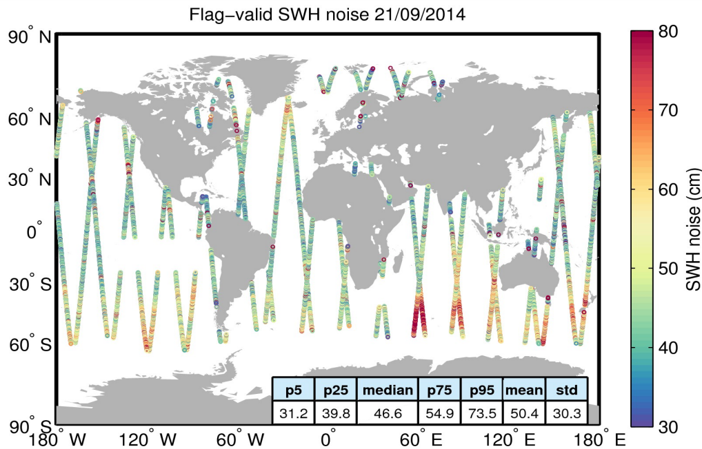
Figure 18. Geographical distribution of flag-valid 20-Hz SWH measurement noise over oceans and lakes for 21/09/2014. The statistical values shown in the figure refer to the SWH noise and are calculated over all measurements shown in the figure.
