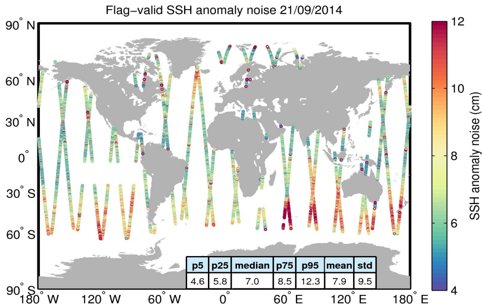
Figure 8. Geographical distribution of flag-valid 20-Hz SSH anomaly measurement noise over oceans and lakes for 21/09/2014. The statistical values shown in the table refer to the SSH anomaly noise and are calculated over all measurements shown in the figure.
