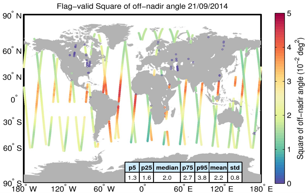
Figure 37. Geographical distribution of flag-valid mispointing data over oceans and lakes for 21/09/2014. The statistical values shown in the table refer to the mispointing in 10^{-2} \text{ deg}^2 and are calculated over all measurements shown in the figure.
