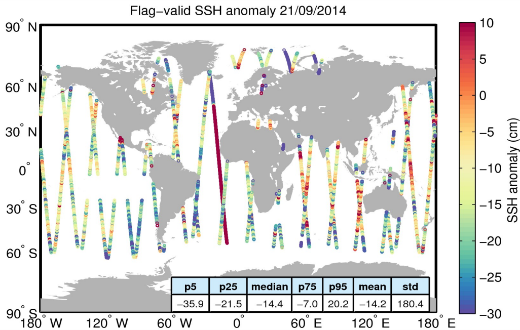
Figure 5. Geographical distribution of flag-valid 1-Hz SSH anomaly data over oceans and lakes for 21/09/2014. The statistical values shown in the table refer to the SSH anomaly in cm and are calculated over all measurements shown in the figure.
