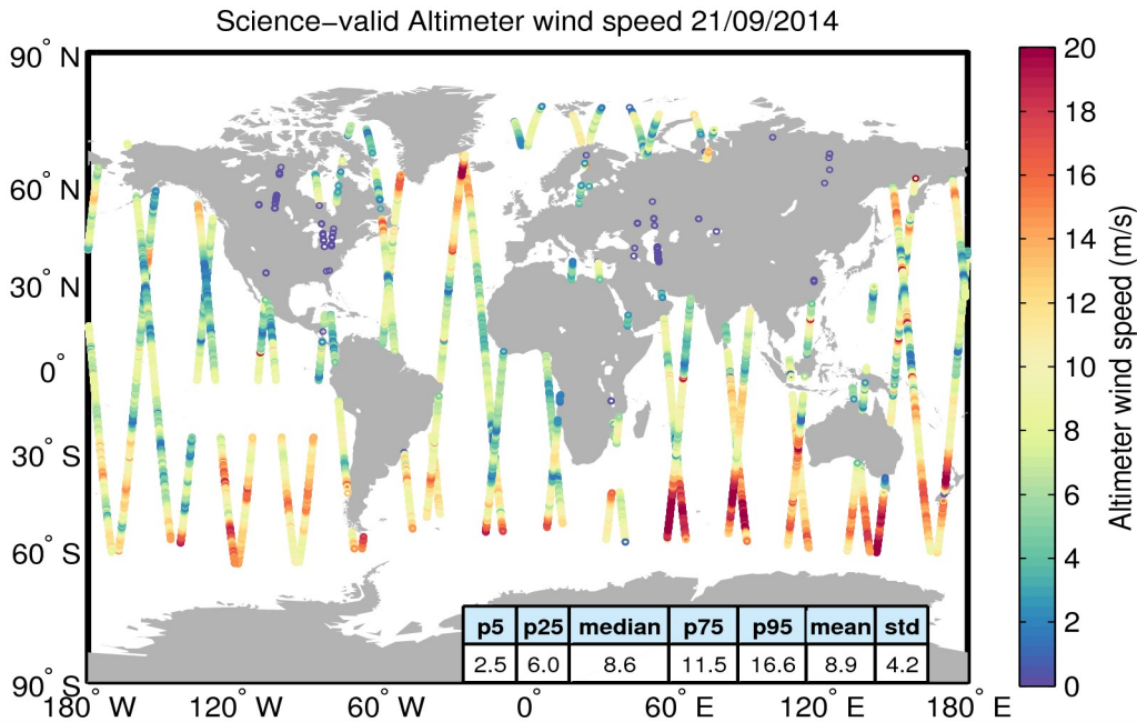
Figure 34. Geographical distribution of science-valid wind data over oceans and lakes for 21/09/2014. The statistical values shown in the table refer to the wind in m/s and are calculated over all measurements shown in the figure. Gray circles denote records that have been rejected based on the editing criteria described in Table 5.
