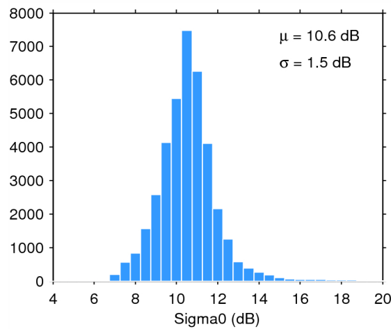
Figure 28. Histogram of science-valid sigma0 over oceans and lakes for 21/09/2014. The mean ( \mu ) and standard deviation ( \sigma ) are also shown. Note that values outside [4 20] dB are excluded from the histogram for the sake of readability but not from the computation of \mu and \sigma .
