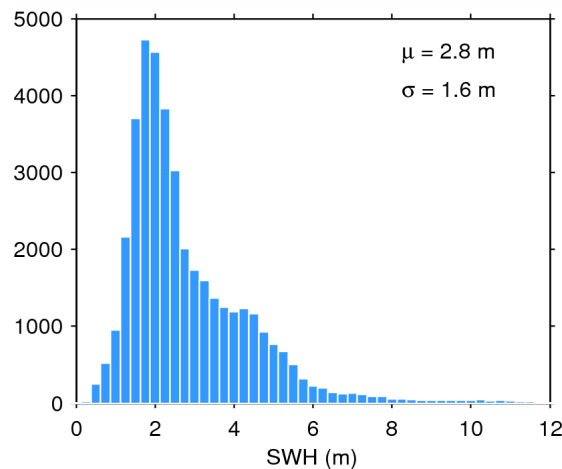
Figure 17. Histogram of flag-valid SWH over oceans and lakes for 21/09/2014. The mean ( \mu ) and standard deviation ( \sigma ) are also shown. Note that values larger than 12 m are excluded from the histogram for the sake of readability but not from the computation of \mu and \sigma .
