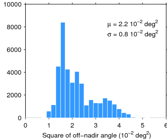
Figure 39. Histogram of flag-valid mispointing over oceans and lakes for 21/09/2014. The mean ( \mu ) and standard deviation ( \sigma ) are also shown. Note that values than 6 \cdot 10^{-2} \text{ deg}^2 are excluded from the histogram for the sake of readability but not from the computation of \mu and \sigma .
