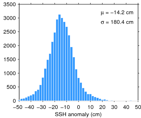
Figure 7. Histogram of flag-valid SSH anomaly over oceans and lakes for 21/09/2014. The mean ( \mu ) and standard deviation ( \sigma ) are also shown. Note that values outside [-50\ 50] cm are excluded from the histogram for the sake of readability but not from the computation of \mu and \sigma .
