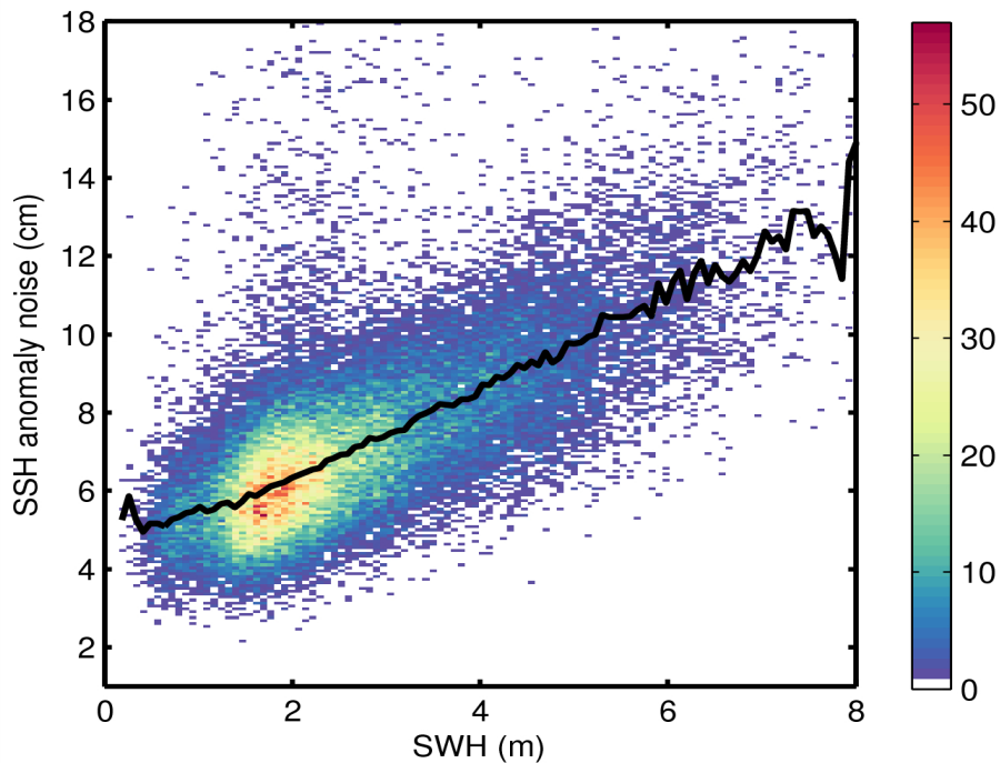
Figure 9. 2D histogram showing flag-valid SSH anomaly noise as a function of SWH for 20/09/2014. The black line denotes the median SSH anomaly as a function of SWH.
