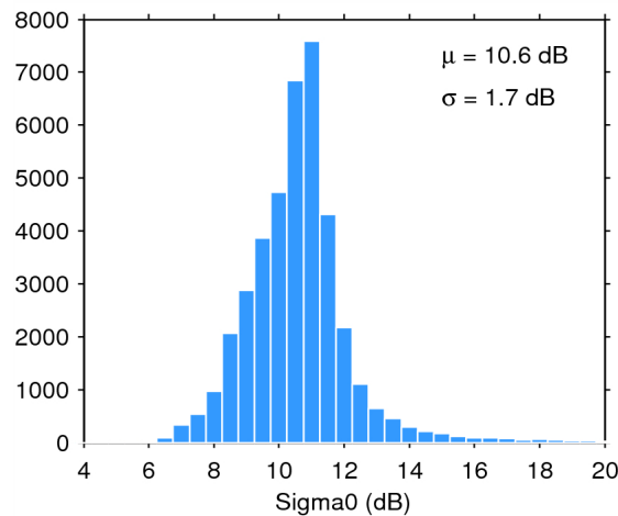
Figure 25. Histogram of flag-valid sigma0 over oceans and lakes for 20/09/2014. The mean ( \mu ) and standard deviation ( \sigma ) are also shown. Note that values outside [4 20] dB are excluded from the histogram for the sake of readability but not from the computation of \mu and \sigma .
