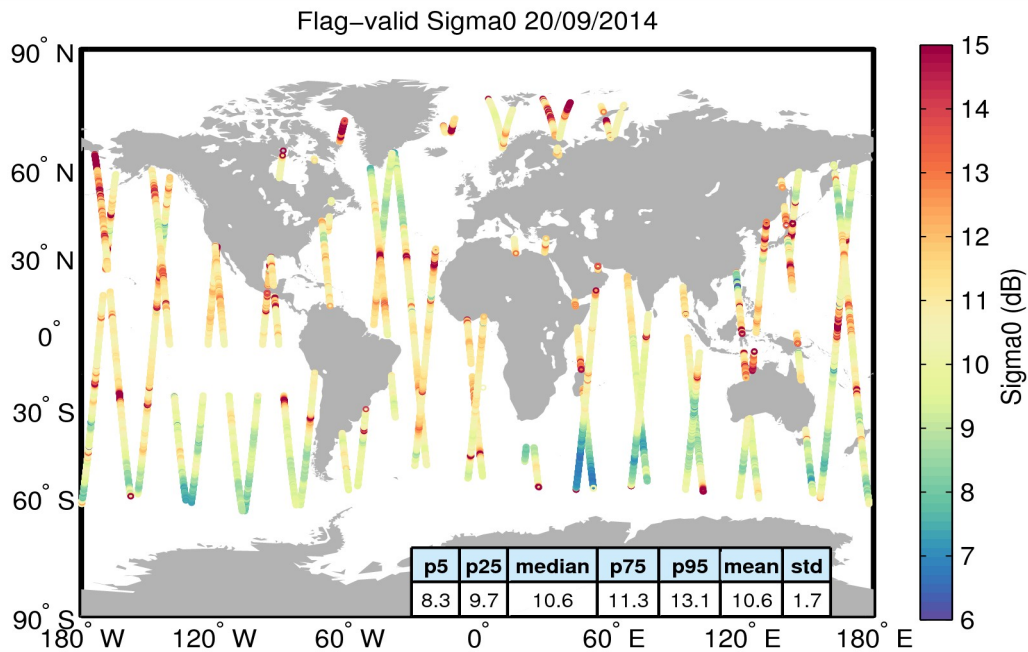
Figure 23. Geographical distribution of flag-valid sigma0 data over oceans and lakes for 20/09/2014. The statistical values shown in the table refer to the sigma0 in dB and are calculated over all measurements shown in the figure.
