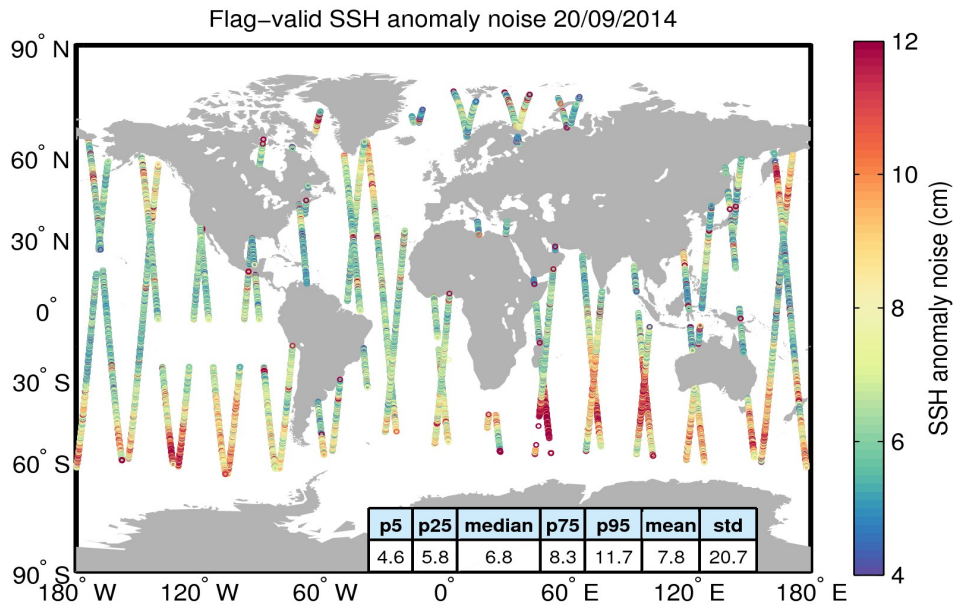
Figure 8. Geographical distribution of flag-valid 20-Hz SSH anomaly measurement noise over oceans and lakes for 20/09/2014. The statistical values shown in the table refer to the SSH anomaly noise and are calculated over all measurements shown in the figure.
