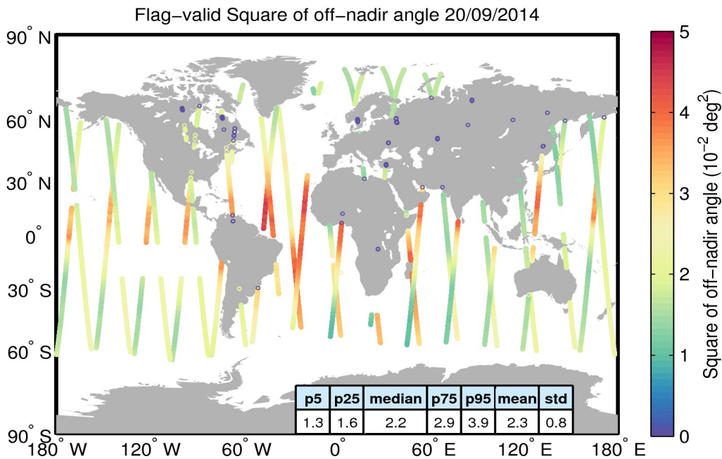
Figure 37. Geographical distribution of flag-valid mispointing data over oceans and lakes for 20/09/2014. The statistical values shown in the table refer to the mispointing in 10^{-2} \text{ deg}^2 and are calculated over all measurements shown in the figure.
