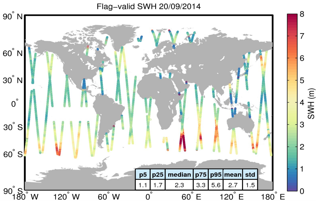
Figure 15. Geographical distribution of flag-valid SWH data over oceans and lakes for 20/09/2014. The statistical values shown in the table refer to the SWH in m and are calculated over all measurements shown in the figure.
