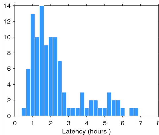
Figure 2. Histogram of the data latency for 20/09/2014. The y-axis denotes the number of files that are made available with a delay of x-hours with respect to the mean time of the records stored in the file.
