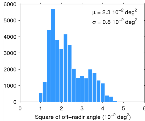
Figure 39. Histogram of flag-valid mispointing over oceans and lakes for 20/09/2014. The mean ( \mu ) and standard deviation ( \sigma ) are also shown. Note that values than 6 \cdot 10^{-2} \text{ deg}^2 are excluded from the histogram for the sake of readability but not from the computation of \mu and \sigma .
