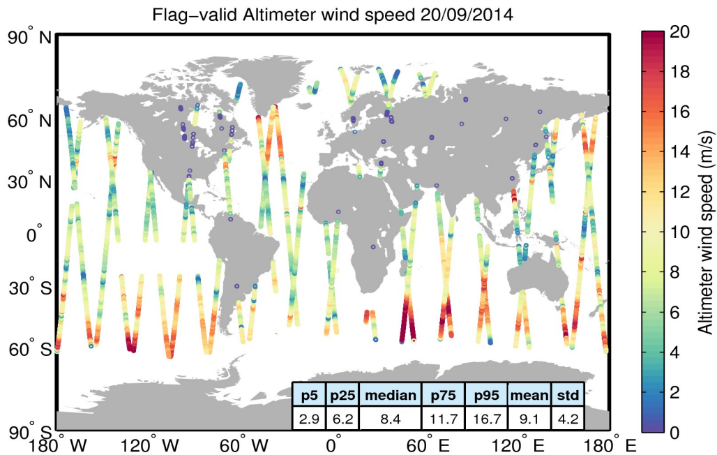
Figure 31. Geographical distribution of flag-valid wind data over oceans and lakes for 20/09/2014. The statistical values shown in the table refer to the wind in m/s and are calculated over all measurements shown in the figure.
