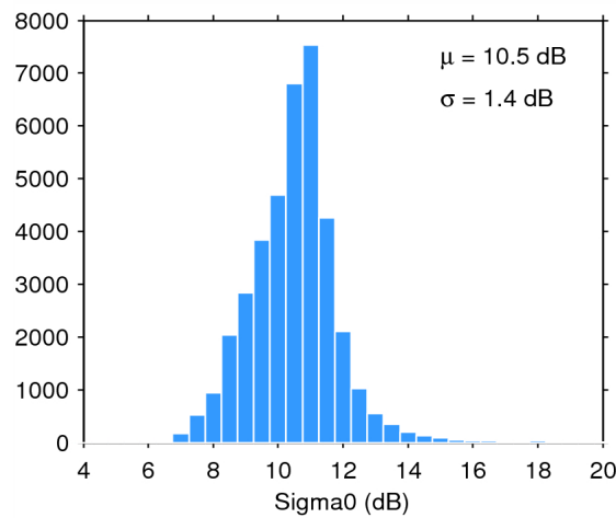
Figure 28. Histogram of science-valid sigma0 over oceans and lakes for 20/09/2014. The mean ( \mu ) and standard deviation ( \sigma ) are also shown. Note that values outside [4 20] dB are excluded from the histogram for the sake of readability but not from the computation of \mu and \sigma .
