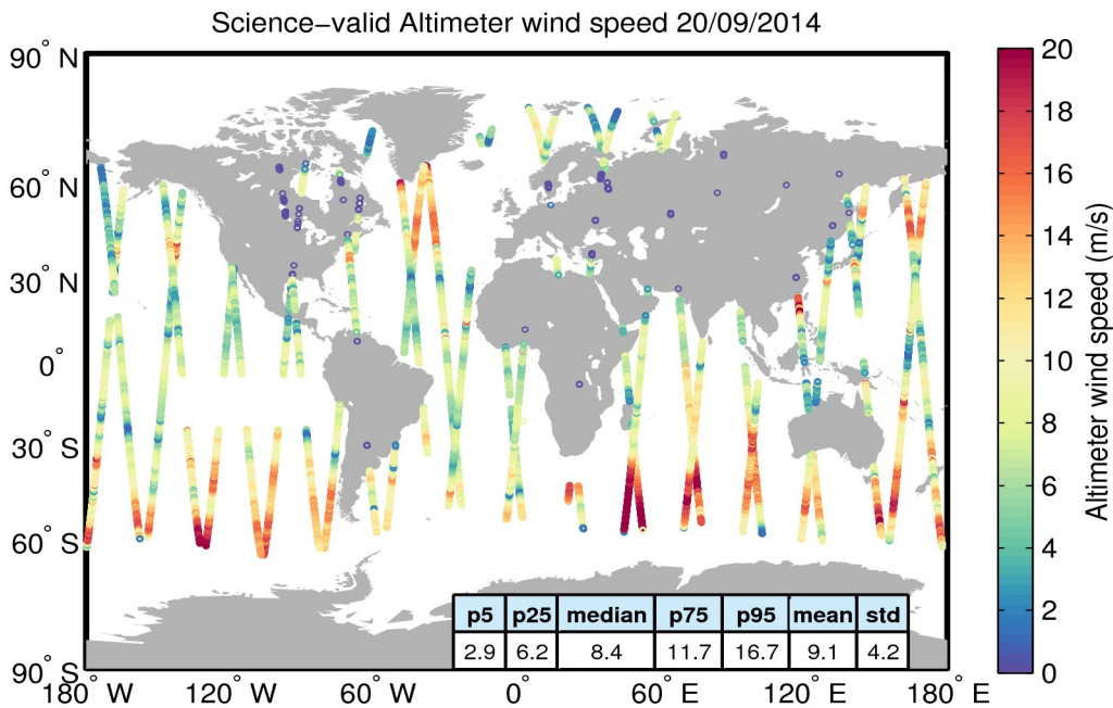
Figure 34. Geographical distribution of science-valid wind data over oceans and lakes for 20/09/2014. The statistical values shown in the table refer to the wind in m/s and are calculated over all measurements shown in the figure. Gray circles denote records that have been rejected based on the editing criteria described in Table 5.
