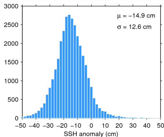
Figure 11. Histogram of science-valid SSH anomaly over oceans and lakes for 20/09/2014. The mean ( \mu ) and standard deviation ( \sigma ) are also shown. Note that values outside [-50 50] cm are excluded from the histogram for the sake of readability but not from the computation of \mu and \sigma .
