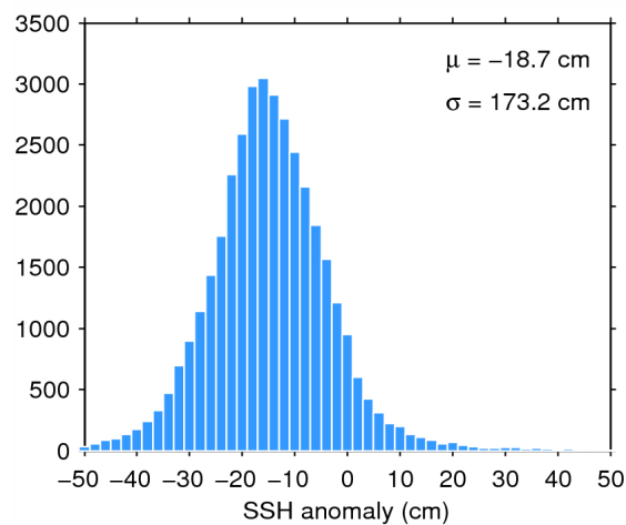
Figure 7. Histogram of flag-valid SSH anomaly over oceans and lakes for 20/09/2014. The mean ( \mu ) and standard deviation ( \sigma ) are also shown. Note that values outside [-50 \ 50] cm are excluded from the histogram for the sake of readability but not from the computation of \mu and \sigma .
