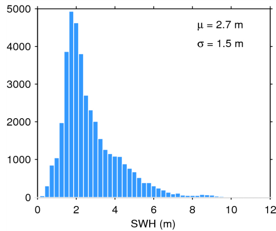
Figure 17. Histogram of flag-valid SWH over oceans and lakes for 20/09/2014. The mean ( \mu ) and standard deviation ( \sigma ) are also shown. Note that values larger than 12 m are excluded from the histogram for the sake of readability but not from the computation of \mu and \sigma .
