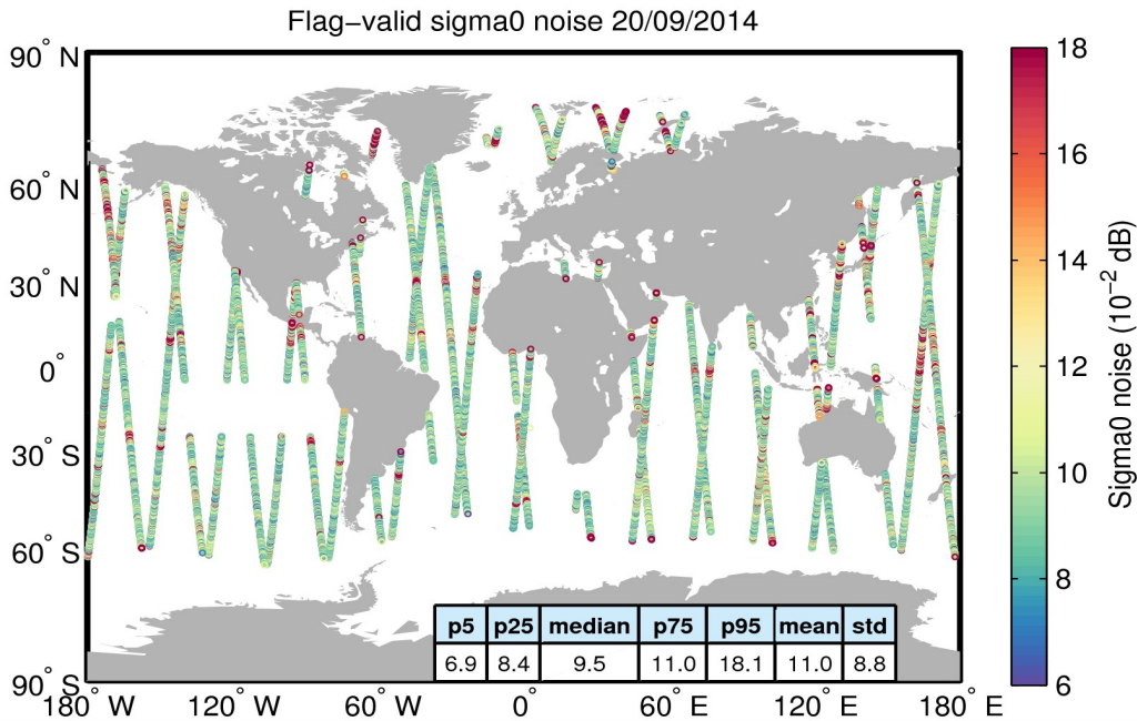
Figure 26. Geographical distribution of flag-valid 20-Hz sigma0 measurement noise over oceans and lakes for 20/09/2014. The statistical values shown in the table refer to the sigma0 noise and are calculated over all measurements shown in the figure.
