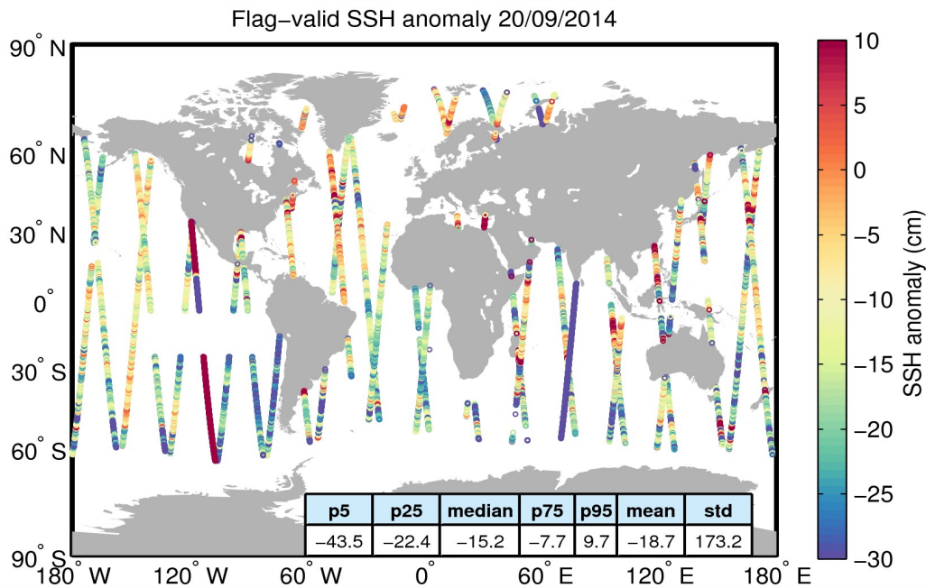
Figure 5. Geographical distribution of flag-valid 1-Hz SSH anomaly data over oceans and lakes for 20/09/2014. The statistical values shown in the table refer to the SSH anomaly in cm and are calculated over all measurements shown in the figure.
