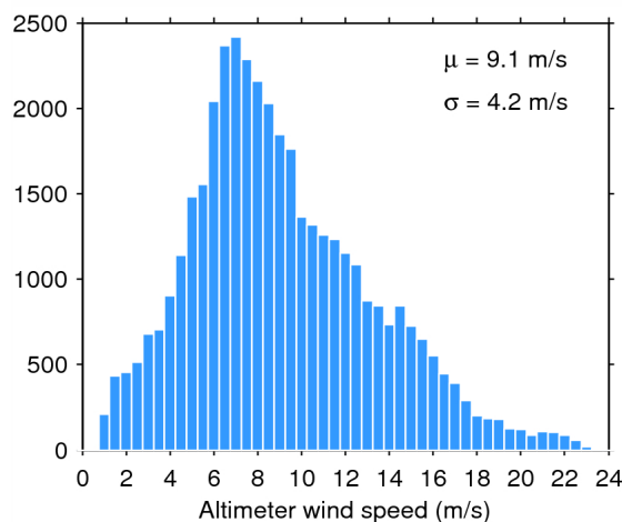
Figure 35. Histogram of science-valid wind over oceans and lakes for 20/09/2014. The mean ( \mu ) and standard deviation ( \sigma ) are also shown. Note that values larger than 24 m/s are excluded from the histogram for the sake of readability but not from the computation of \mu and \sigma .
