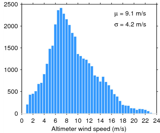
Figure 33. Histogram of flag-valid wind over oceans and lakes for 20/09/2014. The mean ( \mu ) and standard deviation ( \sigma ) are also shown. Note that values larger than 24 m/s are excluded from the histogram for the sake of readability but not from the computation of \mu and \sigma .
