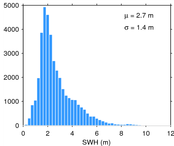
Figure 20. Histogram of science-valid SWH over oceans and lakes for 20/09/2014. The mean ( \mu ) and standard deviation ( \sigma ) are also shown. Note that values larger than 12 m are excluded from the histogram for the sake of readability but not from the computation of \mu and \sigma .
