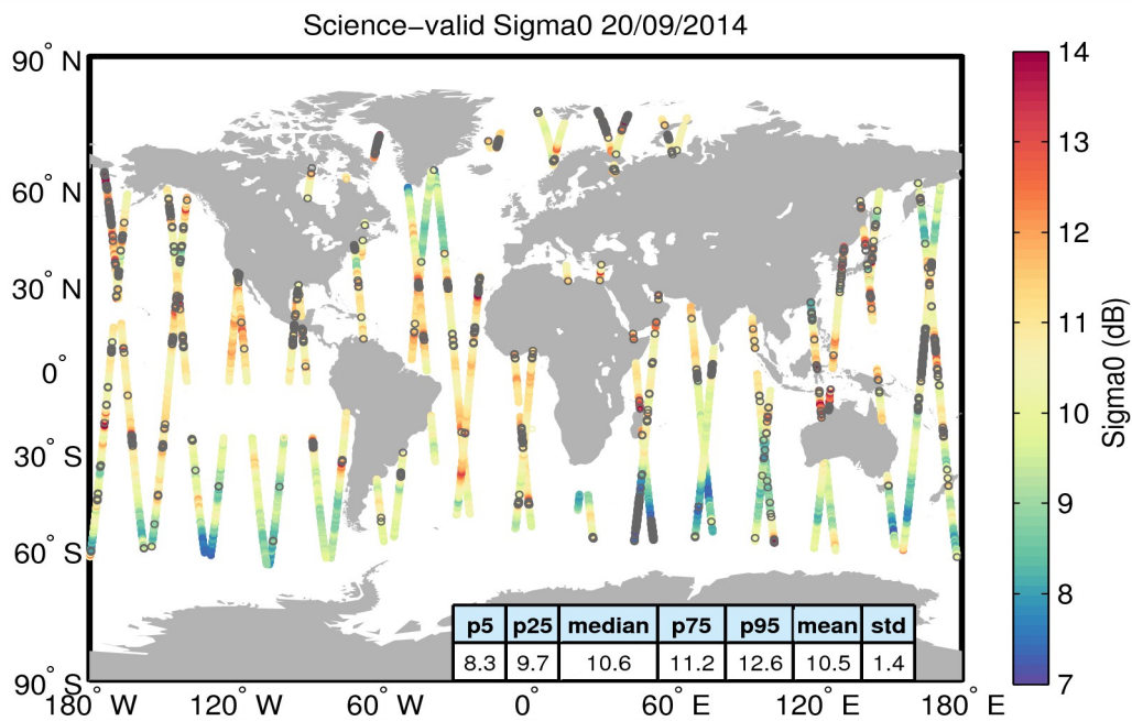
Figure 27. Geographical distribution of science-valid sigma0 data over oceans and lakes for 20/09/2014. The statistical values shown in the table refer to the sigma0 in dB and are calculated over all measurements shown in the figure. Gray circles denote records that have been rejected based on the editing criteria described in Table 4.
