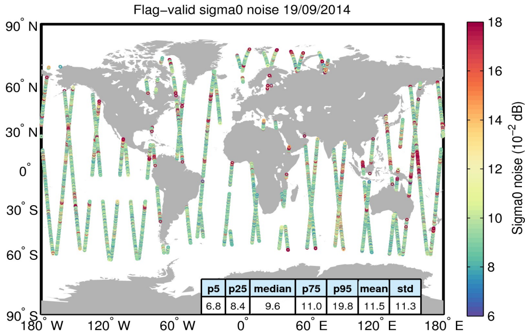
Figure 26. Geographical distribution of flag-valid 20-Hz sigma0 measurement noise over oceans and lakes for 19/09/2014. The statistical values shown in the table refer to the sigma0 noise and are calculated over all measurements shown in the figure.
