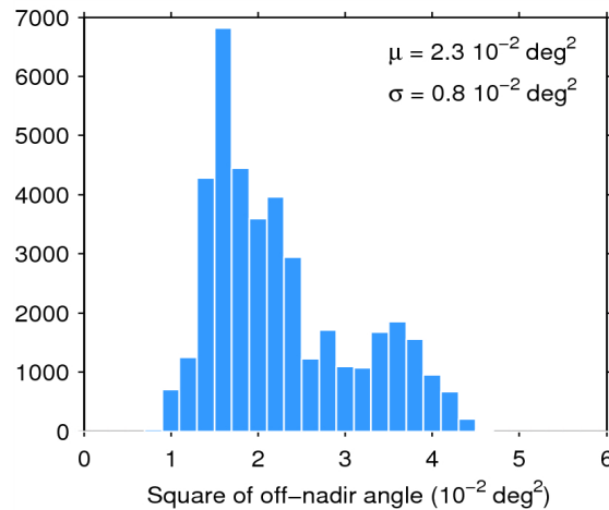
Figure 39. Histogram of flag-valid mispointing over oceans and lakes for 19/09/2014. The mean ( \mu ) and standard deviation ( \sigma ) are also shown. Note that values than 6 \cdot 10^{-2} \text{ deg}^2 are excluded from the histogram for the sake of readability but not from the computation of \mu and \sigma .
