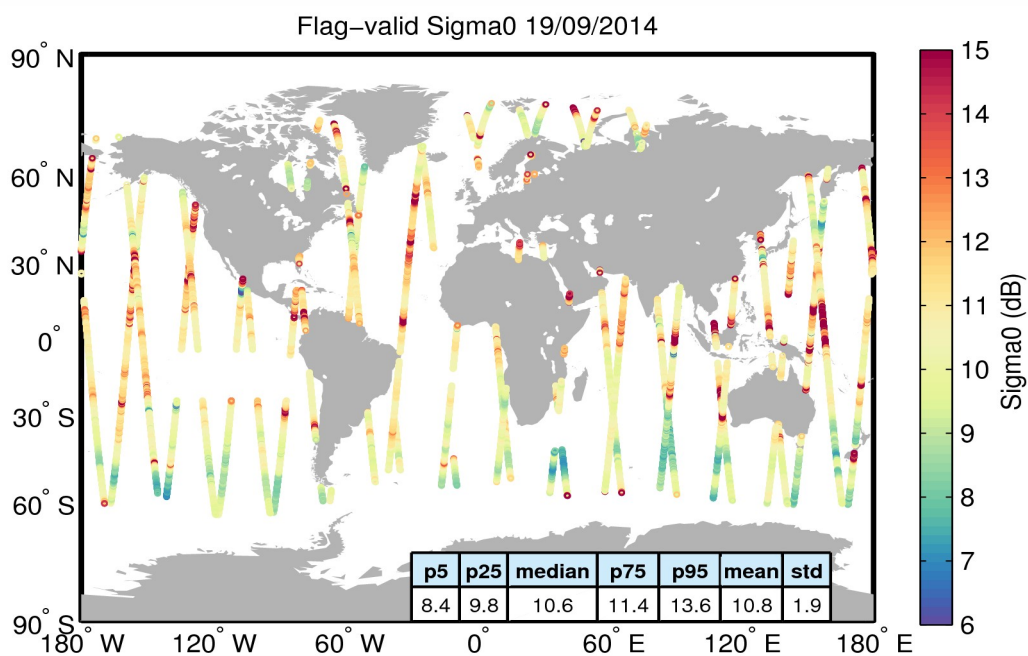
Figure 23. Geographical distribution of flag-valid sigma0 data over oceans and lakes for 19/09/2014. The statistical values shown in the table refer to the sigma0 in dB and are calculated over all measurements shown in the figure.
