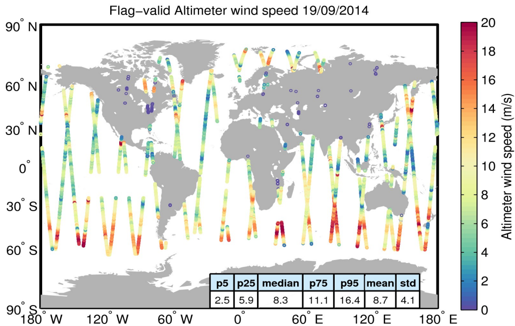
Figure 31. Geographical distribution of flag-valid wind data over oceans and lakes for 19/09/2014. The statistical values shown in the table refer to the wind in m/s and are calculated over all measurements shown in the figure.
