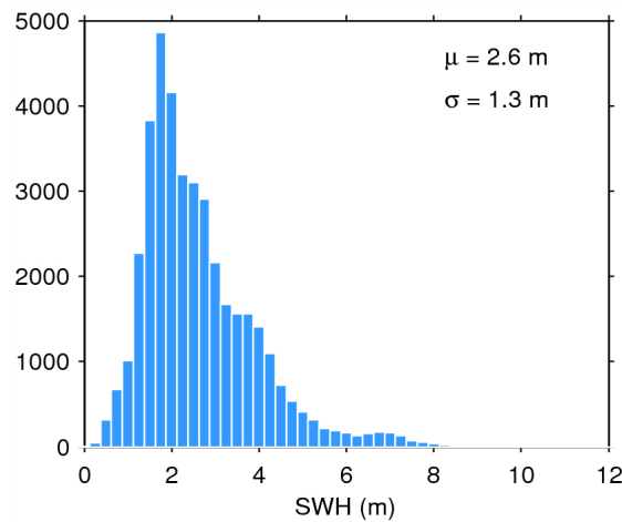
Figure 17. Histogram of flag-valid SWH over oceans and lakes for 19/09/2014. The mean ( \mu ) and standard deviation ( \sigma ) are also shown. Note that values larger than 12 m are excluded from the histogram for the sake of readability but not from the computation of \mu and \sigma .
