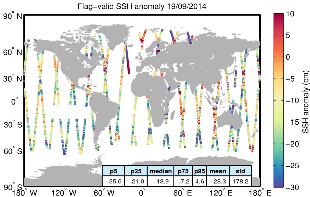
Figure 5. Geographical distribution of flag-valid 1-Hz SSH anomaly data over oceans and lakes for 19/09/2014. The statistical values shown in the table refer to the SSH anomaly in cm and are calculated over all measurements shown in the figure.
