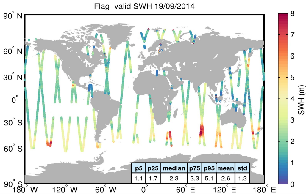
Figure 15. Geographical distribution of flag-valid SWH data over oceans and lakes for 19/09/2014. The statistical values shown in the table refer to the SWH in m and are calculated over all measurements shown in the figure.
