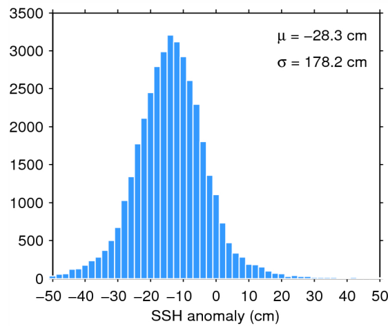
Figure 7. Histogram of flag-valid SSH anomaly over oceans and lakes for 19/09/2014. The mean ( \mu ) and standard deviation ( \sigma ) are also shown. Note that values outside [-50\ 50] cm are excluded from the histogram for the sake of readability but not from the computation of \mu and \sigma .
