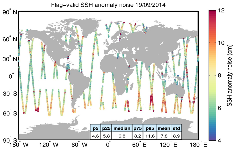
Figure 8. Geographical distribution of flag-valid 20-Hz SSH anomaly measurement noise over oceans and lakes for 19/09/2014. The statistical values shown in the table refer to the SSH anomaly noise and are calculated over all measurements shown in the figure.
