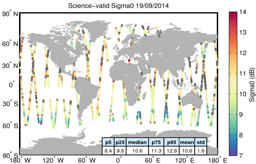
Figure 27. Geographical distribution of science-valid sigma0 data over oceans and lakes for 19/09/2014. The statistical values shown in the table refer to the sigma0 in dB and are calculated over all measurements shown in the figure. Gray circles denote records that have been rejected based on the editing criteria described in Table 4.
