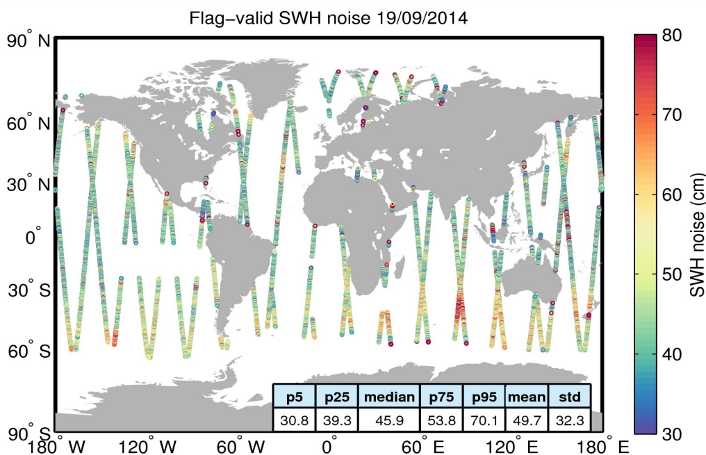
Figure 18. Geographical distribution of flag-valid 20-Hz SWH measurement noise over oceans and lakes for 19/09/2014. The statistical values shown in the figure refer to the SWH noise and are calculated over all measurements shown in the figure.
