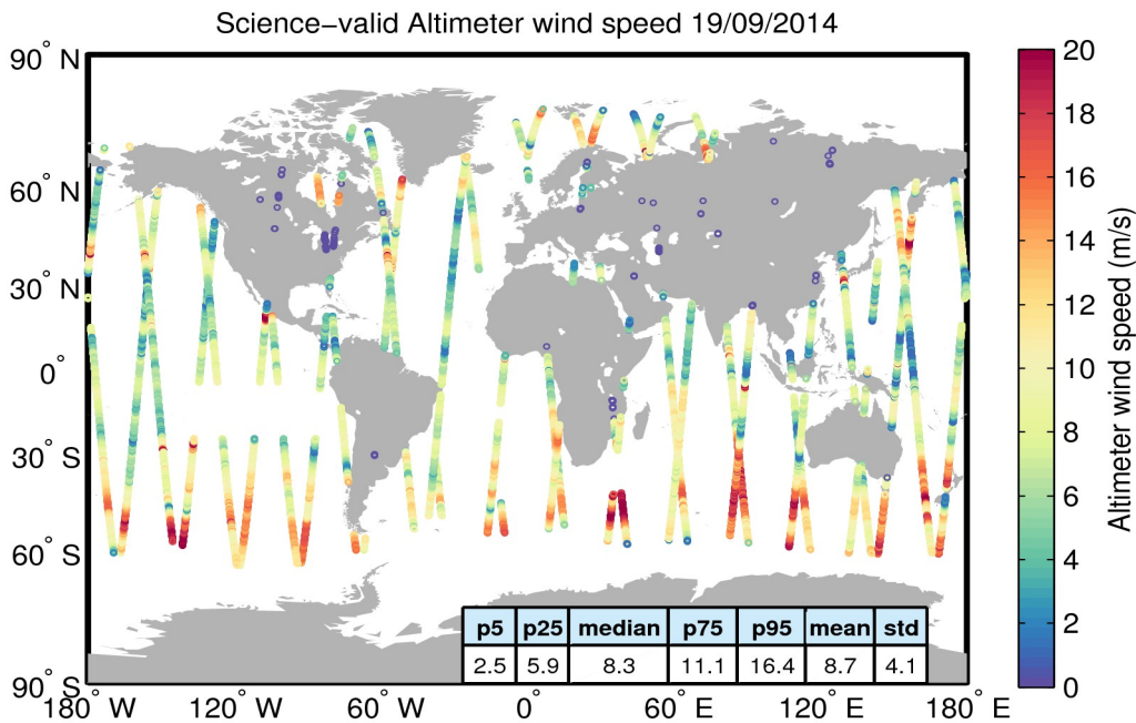
Figure 34. Geographical distribution of science-valid wind data over oceans and lakes for 19/09/2014. The statistical values shown in the table refer to the wind in m/s and are calculated over all measurements shown in the figure. Gray circles denote records that have been rejected based on the editing criteria described in Table 5.
