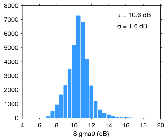
Figure 28. Histogram of science-valid sigma0 over oceans and lakes for 19/09/2014. The mean ( \mu ) and standard deviation ( \sigma ) are also shown. Note that values outside [4 20] dB are excluded from the histogram for the sake of readability but not from the computation of \mu and \sigma .
