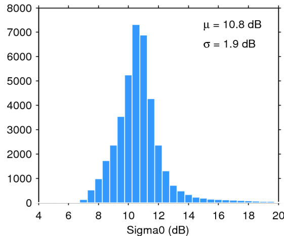
Figure 25. Histogram of flag-valid sigma0 over oceans and lakes for 19/09/2014. The mean ( \mu ) and standard deviation ( \sigma ) are also shown. Note that values outside [4 20] dB are excluded from the histogram for the sake of readability but not from the computation of \mu and \sigma .
