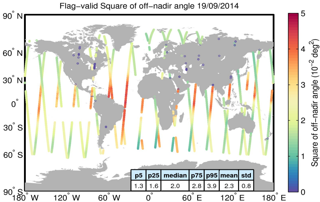
Figure 37. Geographical distribution of flag-valid mispointing data over oceans and lakes for 19/09/2014. The statistical values shown in the table refer to the mispointing in 10^{-2} \text{ deg}^2 and are calculated over all measurements shown in the figure.
