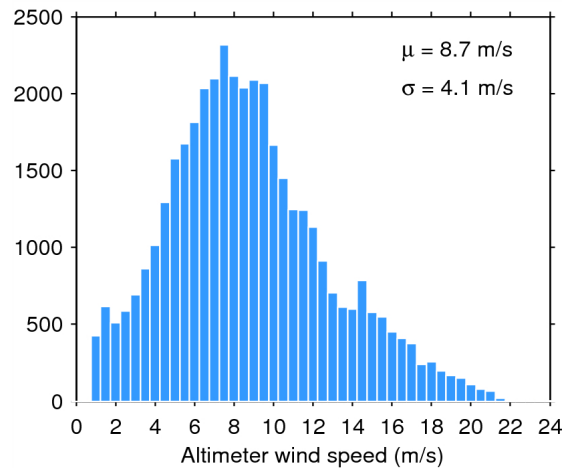
Figure 33. Histogram of flag-valid wind over oceans and lakes for 19/09/2014. The mean ( \mu ) and standard deviation ( \sigma ) are also shown. Note that values larger than 24 m/s are excluded from the histogram for the sake of readability but not from the computation of \mu and \sigma .
