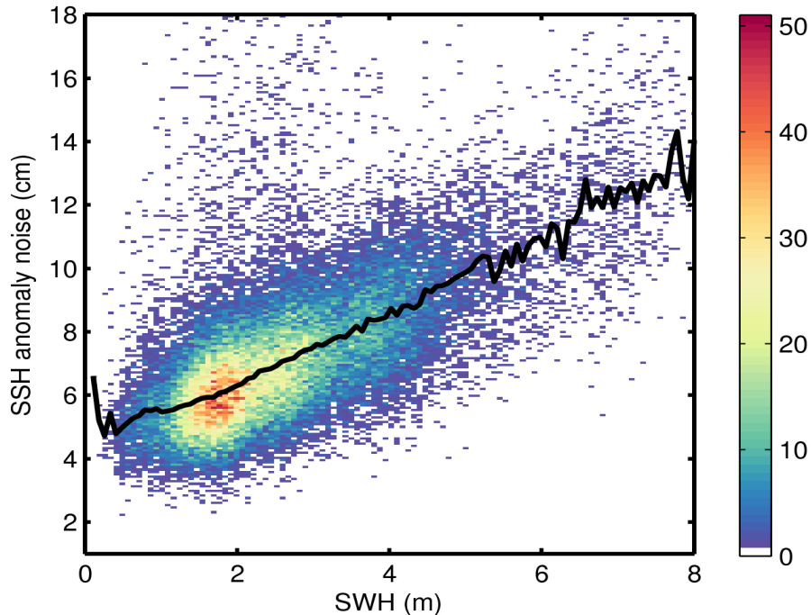
Figure 9. 2D histogram showing flag-valid SSH anomaly noise as a function of SWH for 19/09/2014. The black line denotes the median SSH anomaly as a function of SWH.
