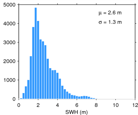
Figure 20. Histogram of science-valid SWH over oceans and lakes for 19/09/2014. The mean ( \mu ) and standard deviation ( \sigma ) are also shown. Note that values larger than 12 m are excluded from the histogram for the sake of readability but not from the computation of \mu and \sigma .
