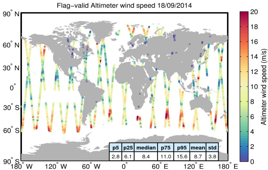
Figure 31. Geographical distribution of flag-valid wind data over oceans and lakes for 18/09/2014. The statistical values shown in the table refer to the wind in m/s and are calculated over all measurements shown in the figure.
