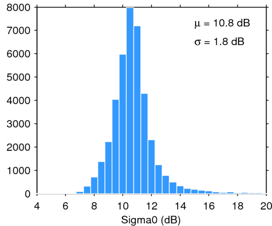
Figure 25. Histogram of flag-valid sigma0 over oceans and lakes for 18/09/2014. The mean ( \mu ) and standard deviation ( \sigma ) are also shown. Note that values outside [4 20] dB are excluded from the histogram for the sake of readability but not from the computation of \mu and \sigma .
