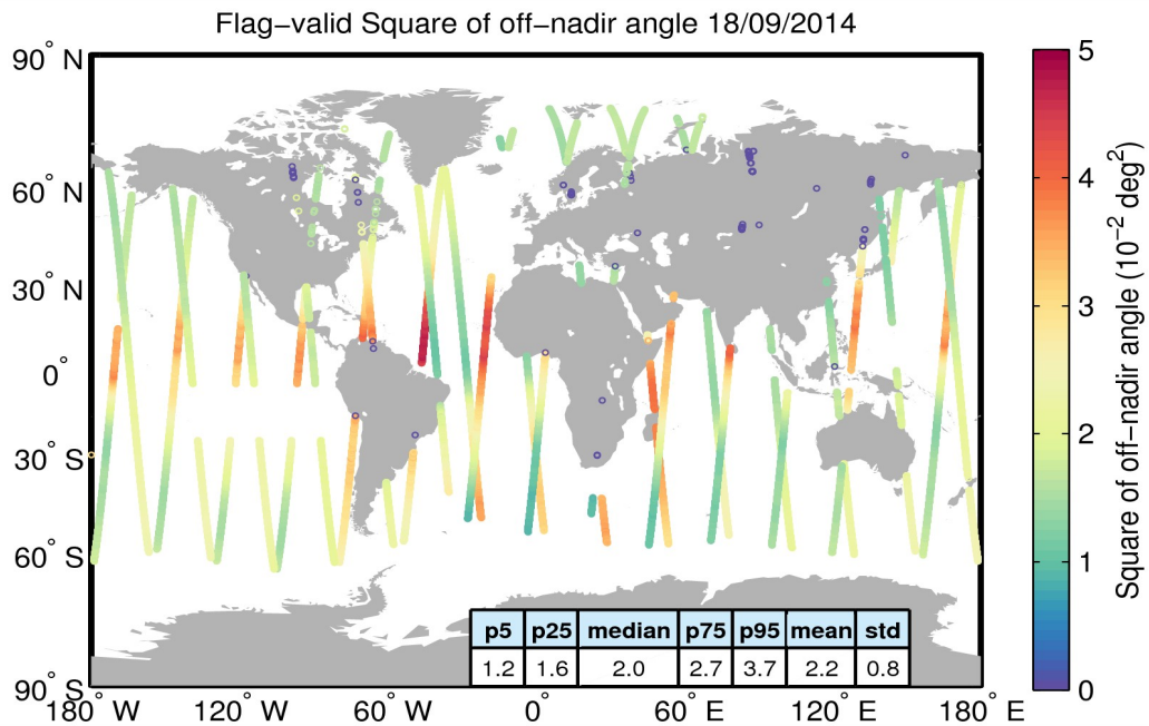
Figure 37. Geographical distribution of flag-valid mispointing data over oceans and lakes for 18/09/2014. The statistical values shown in the table refer to the mispointing in 10^{-2} \text{ deg}^2 and are calculated over all measurements shown in the figure.
