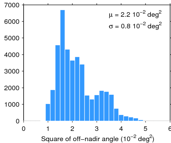
Figure 39. Histogram of flag-valid mispointing over oceans and lakes for 18/09/2014. The mean ( \mu ) and standard deviation ( \sigma ) are also shown. Note that values than 6 \cdot 10^{-2} \text{ deg}^2 are excluded from the histogram for the sake of readability but not from the computation of \mu and \sigma .
