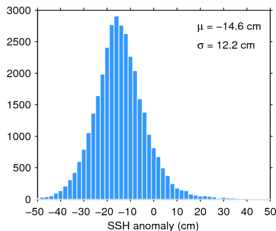
Figure 11. Histogram of science-valid SSH anomaly over oceans and lakes for 18/09/2014. The mean ( \mu ) and standard deviation ( \sigma ) are also shown. Note that values outside [-50 50] cm are excluded from the histogram for the sake of readability but not from the computation of \mu and \sigma .
