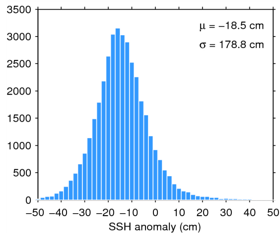
Figure 7. Histogram of flag-valid SSH anomaly over oceans and lakes for 18/09/2014. The mean ( \mu ) and standard deviation ( \sigma ) are also shown. Note that values outside [-50 50] cm are excluded from the histogram for the sake of readability but not from the computation of \mu and \sigma .
