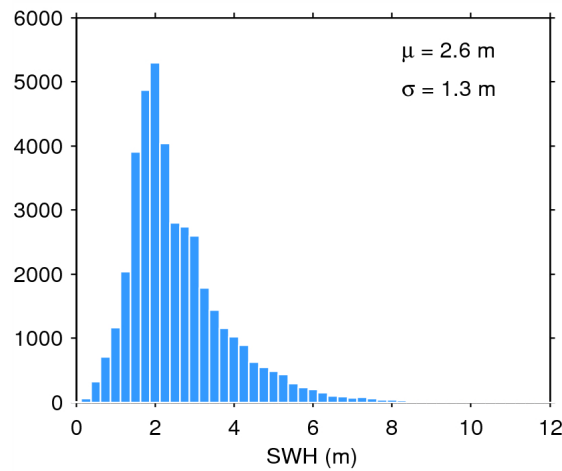
Figure 17. Histogram of flag-valid SWH over oceans and lakes for 18/09/2014. The mean ( \mu ) and standard deviation ( \sigma ) are also shown. Note that values larger than 12 m are excluded from the histogram for the sake of readability but not from the computation of \mu and \sigma .
