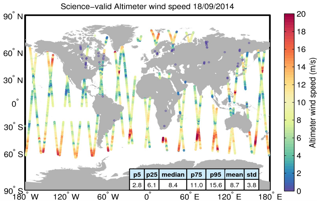
Figure 34. Geographical distribution of science-valid wind data over oceans and lakes for 18/09/2014. The statistical values shown in the table refer to the wind in m/s and are calculated over all measurements shown in the figure. Gray circles denote records that have been rejected based on the editing criteria described in Table 5.
