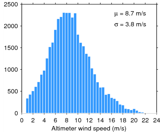
Figure 33. Histogram of flag-valid wind over oceans and lakes for 18/09/2014. The mean ( \mu ) and standard deviation ( \sigma ) are also shown. Note that values larger than 24 m/s are excluded from the histogram for the sake of readability but not from the computation of \mu and \sigma .
