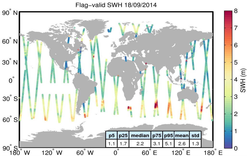
Figure 15. Geographical distribution of flag-valid SWH data over oceans and lakes for 18/09/2014. The statistical values shown in the table refer to the SWH in m and are calculated over all measurements shown in the figure.
