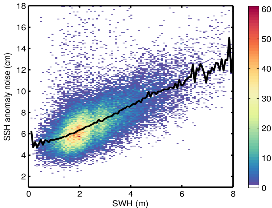
Figure 9. 2D histogram showing flag-valid SSH anomaly noise as a function of SWH for 18/09/2014. The black line denotes the median SSH anomaly as a function of SWH.
