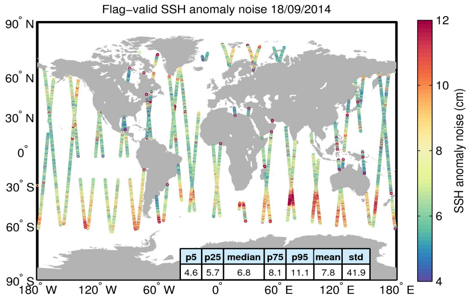
Figure 8. Geographical distribution of flag-valid 20-Hz SSH anomaly measurement noise over oceans and lakes for 18/09/2014. The statistical values shown in the table refer to the SSH anomaly noise and are calculated over all measurements shown in the figure.
