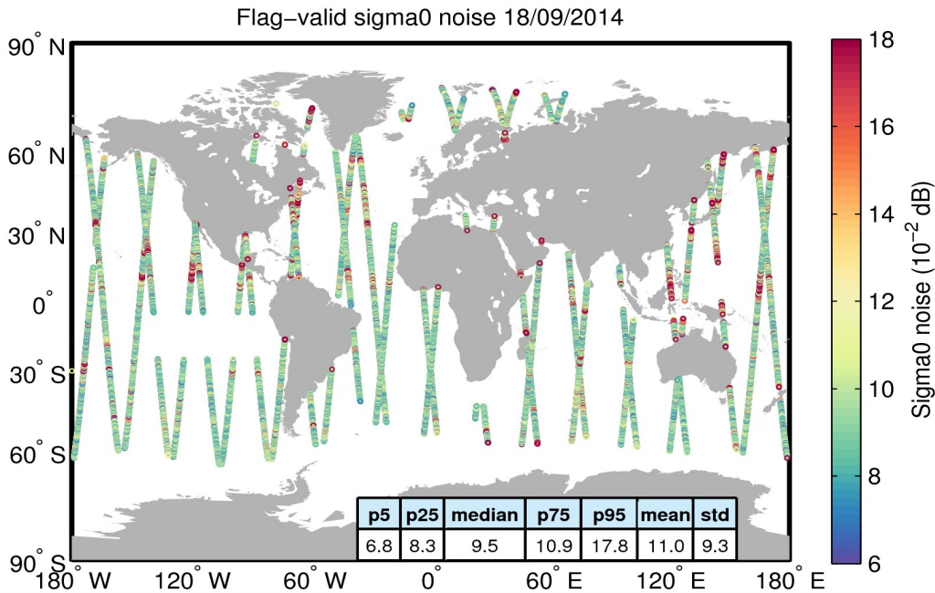
Figure 26. Geographical distribution of flag-valid 20-Hz sigma0 measurement noise over oceans and lakes for 18/09/2014. The statistical values shown in the table refer to the sigma0 noise and are calculated over all measurements shown in the figure.
