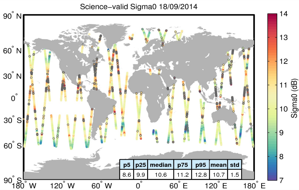
Figure 27. Geographical distribution of science-valid sigma0 data over oceans and lakes for 18/09/2014. The statistical values shown in the table refer to the sigma0 in dB and are calculated over all measurements shown in the figure. Gray circles denote records that have been rejected based on the editing criteria described in Table 4.
