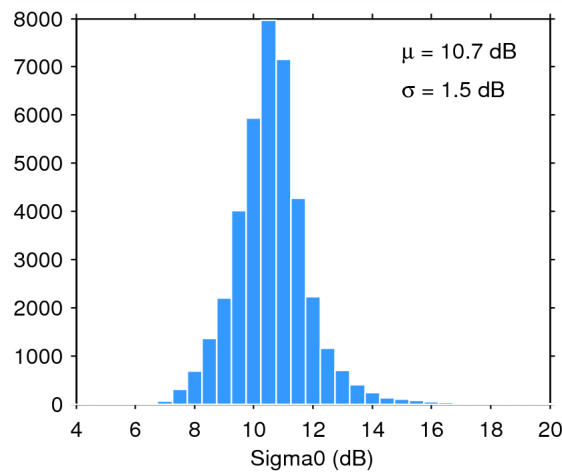
Figure 28. Histogram of science-valid sigma0 over oceans and lakes for 18/09/2014. The mean ( \mu ) and standard deviation ( \sigma ) are also shown. Note that values outside [4 20] dB are excluded from the histogram for the sake of readability but not from the computation of \mu and \sigma .
