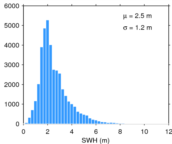
Figure 20. Histogram of science-valid SWH over oceans and lakes for 18/09/2014. The mean ( \mu ) and standard deviation ( \sigma ) are also shown. Note that values larger than 12 m are excluded from the histogram for the sake of readability but not from the computation of \mu and \sigma .
