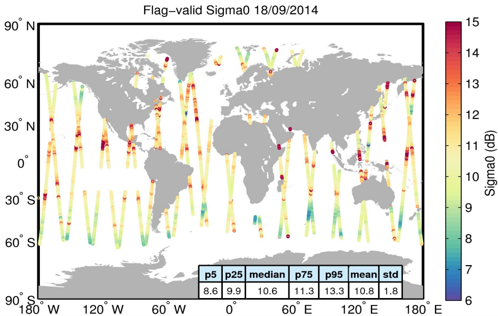
Figure 23. Geographical distribution of flag-valid sigma0 data over oceans and lakes for 18/09/2014. The statistical values shown in the table refer to the sigma0 in dB and are calculated over all measurements shown in the figure.
