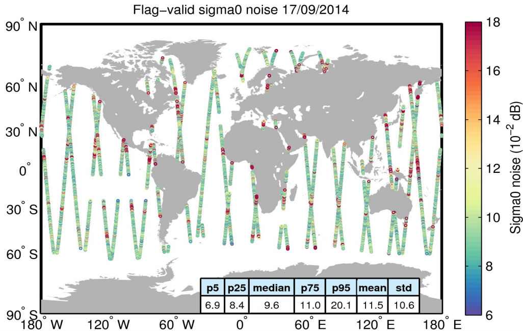
Figure 26. Geographical distribution of flag-valid 20-Hz sigma0 measurement noise over oceans and lakes for 17/09/2014. The statistical values shown in the table refer to the sigma0 noise and are calculated over all measurements shown in the figure.
