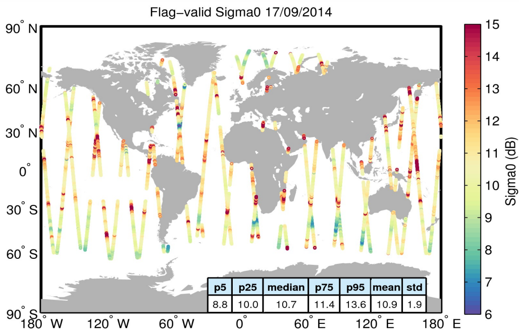
Figure 23. Geographical distribution of flag-valid sigma0 data over oceans and lakes for 17/09/2014. The statistical values shown in the table refer to the sigma0 in dB and are calculated over all measurements shown in the figure.
