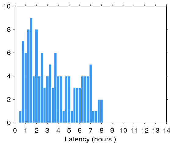
Figure 2. Histogram of the data latency for 17/09/2014. The y-axis denotes the number of files that are made available with a delay of x-hours with respect to the mean time of the records stored in the file.
