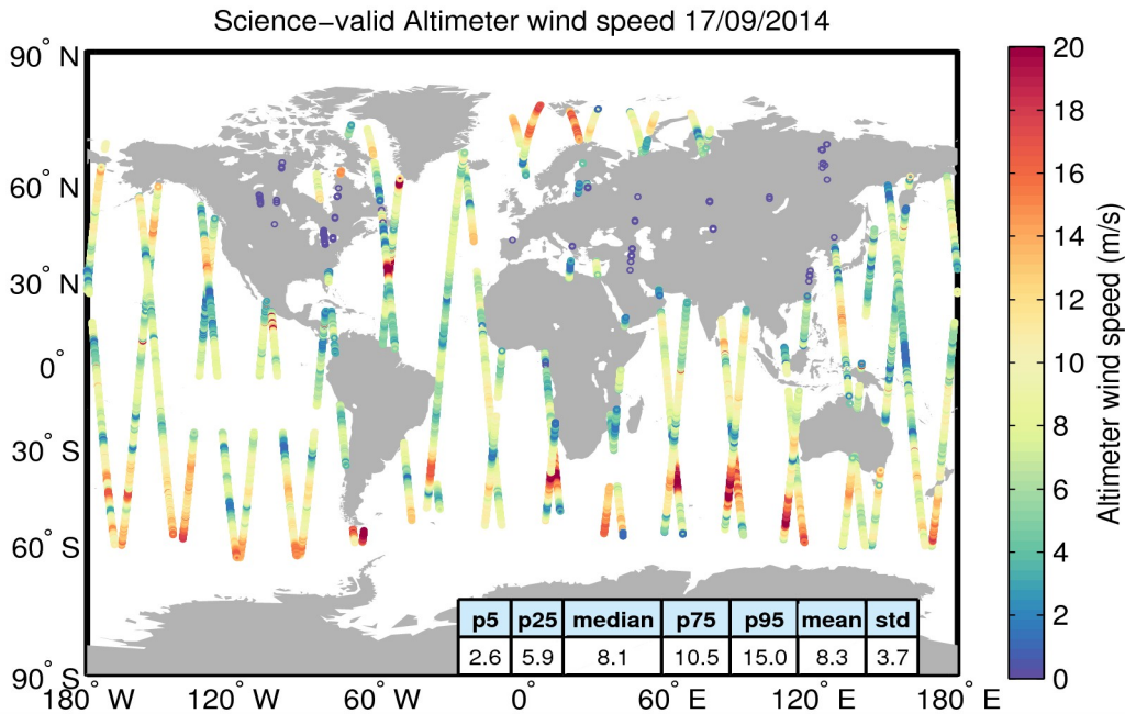
Figure 34. Geographical distribution of science-valid wind data over oceans and lakes for 17/09/2014. The statistical values shown in the table refer to the wind in m/s and are calculated over all measurements shown in the figure. Gray circles denote records that have been rejected based on the editing criteria described in Table 5.
