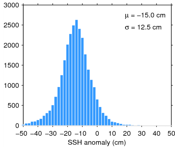
Figure 11. Histogram of science-valid SSH anomaly over oceans and lakes for 17/09/2014. The mean ( \mu ) and standard deviation ( \sigma ) are also shown. Note that values outside [-50 50] cm are excluded from the histogram for the sake of readability but not from the computation of \mu and \sigma .
