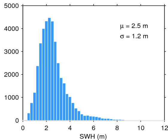
Figure 20. Histogram of science-valid SWH over oceans and lakes for 17/09/2014. The mean ( \mu ) and standard deviation ( \sigma ) are also shown. Note that values larger than 12 m are excluded from the histogram for the sake of readability but not from the computation of \mu and \sigma .
