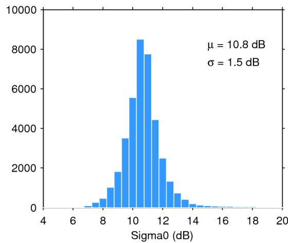
Figure 28. Histogram of science-valid sigma0 over oceans and lakes for 17/09/2014. The mean ( \mu ) and standard deviation ( \sigma ) are also shown. Note that values outside [4 20] dB are excluded from the histogram for the sake of readability but not from the computation of \mu and \sigma .
