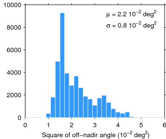
Figure 39. Histogram of flag-valid mispointing over oceans and lakes for 17/09/2014. The mean ( \mu ) and standard deviation ( \sigma ) are also shown. Note that values than 6 \cdot 10^{-2} \text{ deg}^2 are excluded from the histogram for the sake of readability but not from the computation of \mu and \sigma .
