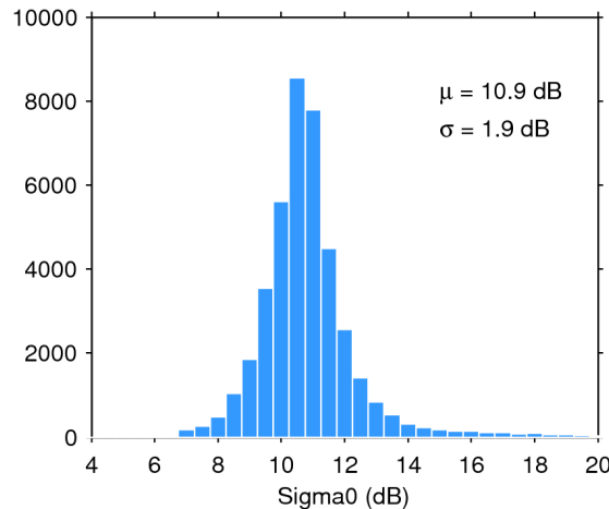
Figure 25. Histogram of flag-valid sigma0 over oceans and lakes for 17/09/2014. The mean ( \mu ) and standard deviation ( \sigma ) are also shown. Note that values outside [4 20] dB are excluded from the histogram for the sake of readability but not from the computation of \mu and \sigma .
