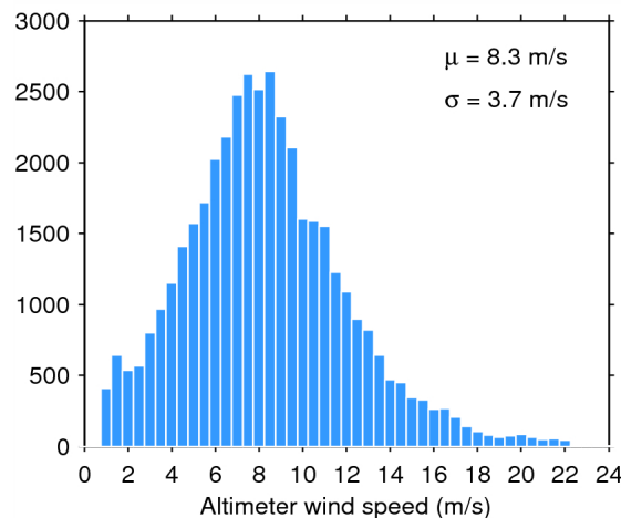
Figure 35. Histogram of science-valid wind over oceans and lakes for 17/09/2014. The mean ( \mu ) and standard deviation ( \sigma ) are also shown. Note that values larger than 24 m/s are excluded from the histogram for the sake of readability but not from the computation of \mu and \sigma .
