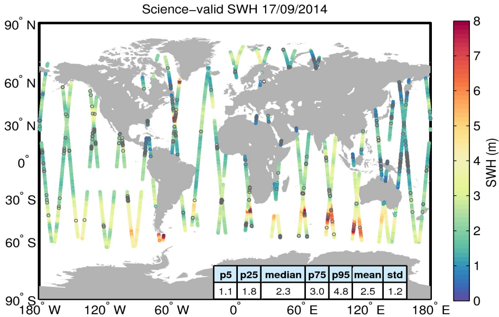
Figure 19. Geographical distribution of science-valid SWH data over oceans and lakes for 17/09/2014. The statistical values shown in the table refer to the SWH in m and are calculated over all measurements shown in the figure. Gray circles denote records that have been rejected based on the editing criteria described in Table 3.
