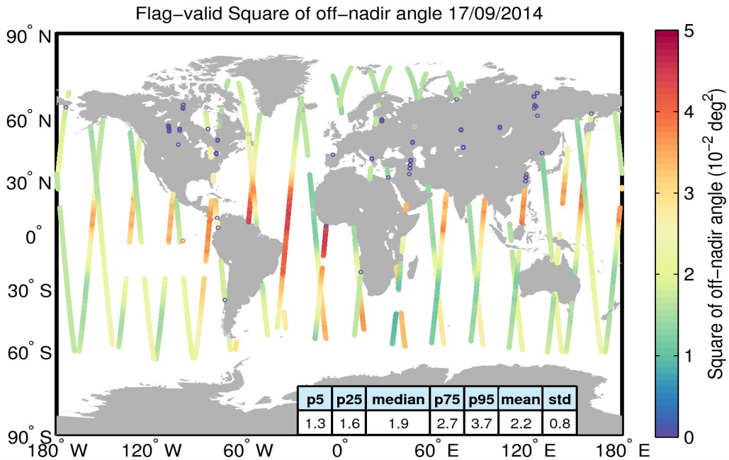
Figure 37. Geographical distribution of flag-valid mispointing data over oceans and lakes for 17/09/2014. The statistical values shown in the table refer to the mispointing in 10^{-2} \text{ deg}^2 and are calculated over all measurements shown in the figure.
