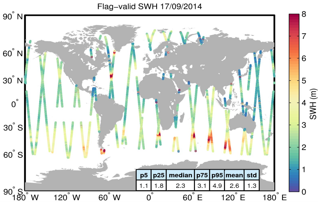
Figure 15. Geographical distribution of flag-valid SWH data over oceans and lakes for 17/09/2014. The statistical values shown in the table refer to the SWH in m and are calculated over all measurements shown in the figure.
