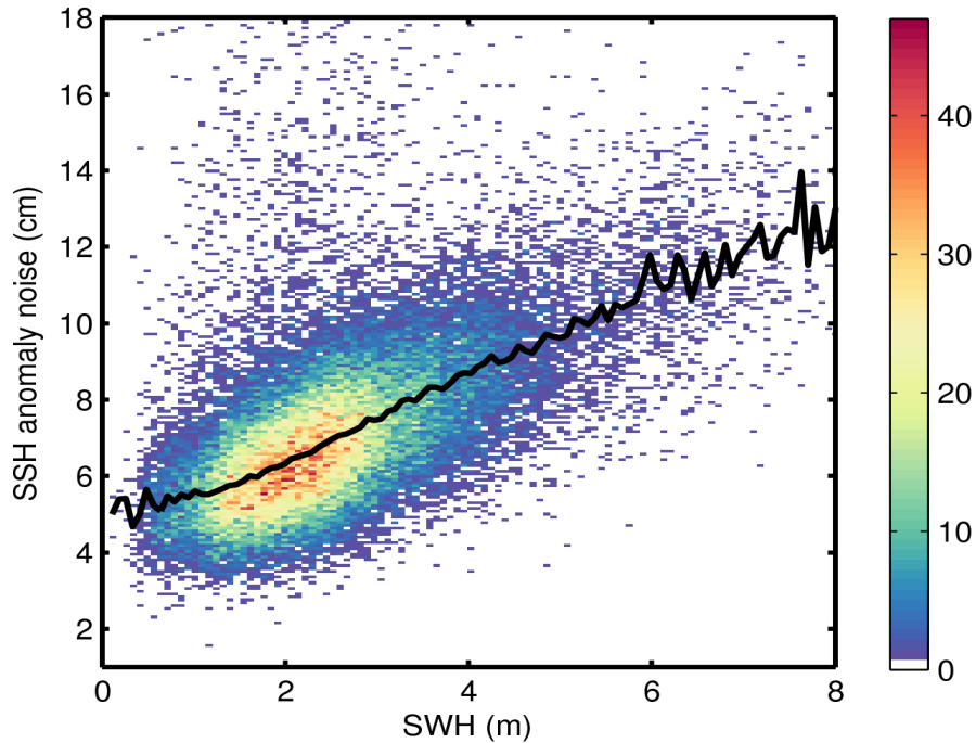
Figure 9. 2D histogram showing flag-valid SSH anomaly noise as a function of SWH for 17/09/2014. The black line denotes the median SSH anomaly as a function of SWH.
