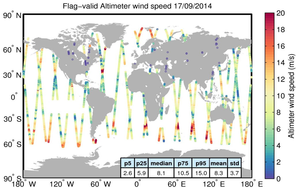
Figure 31. Geographical distribution of flag-valid wind data over oceans and lakes for 17/09/2014. The statistical values shown in the table refer to the wind in m/s and are calculated over all measurements shown in the figure.
