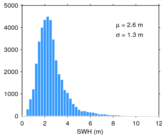
Figure 17. Histogram of flag-valid SWH over oceans and lakes for 17/09/2014. The mean ( \mu ) and standard deviation ( \sigma ) are also shown. Note that values larger than 12 m are excluded from the histogram for the sake of readability but not from the computation of \mu and \sigma .
