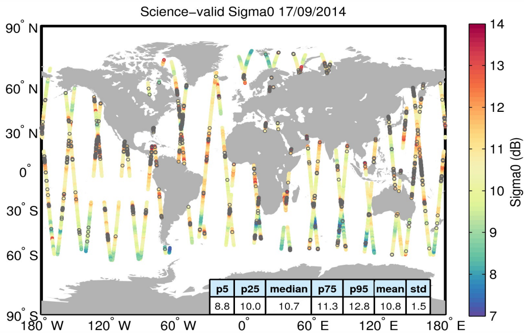
Figure 27. Geographical distribution of science-valid sigma0 data over oceans and lakes for 17/09/2014. The statistical values shown in the table refer to the sigma0 in dB and are calculated over all measurements shown in the figure. Gray circles denote records that have been rejected based on the editing criteria described in Table 4.
