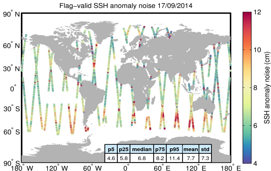
Figure 8. Geographical distribution of flag-valid 20-Hz SSH anomaly measurement noise over oceans and lakes for 17/09/2014. The statistical values shown in the table refer to the SSH anomaly noise and are calculated over all measurements shown in the figure.
