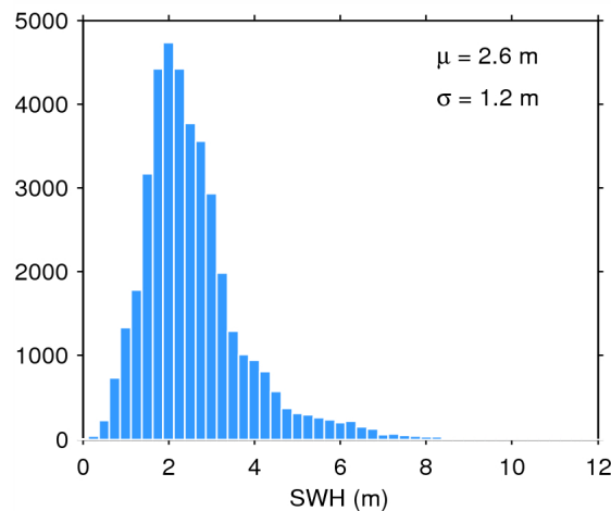
Figure 20. Histogram of science-valid SWH over oceans and lakes for 16/09/2014. The mean ( \mu ) and standard deviation ( \sigma ) are also shown. Note that values larger than 12 m are excluded from the histogram for the sake of readability but not from the computation of \mu and \sigma .
