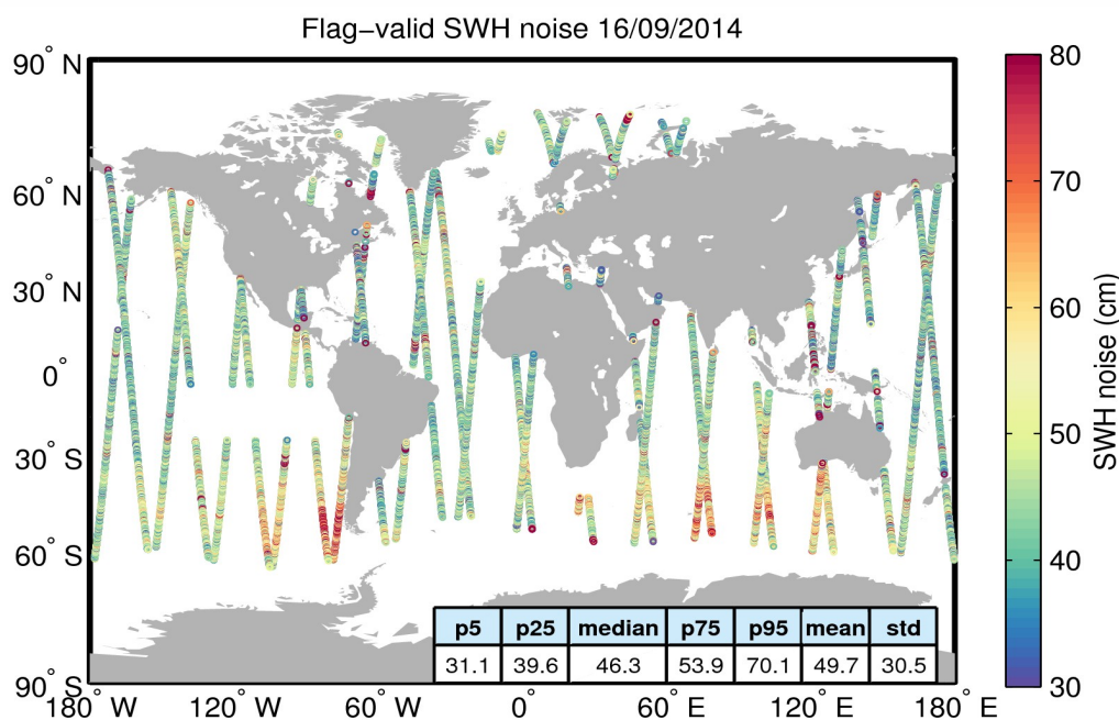
Figure 18. Geographical distribution of flag-valid 20-Hz SWH measurement noise over oceans and lakes for 16/09/2014. The statistical values shown in the figure refer to the SWH noise and are calculated over all measurements shown in the figure.
