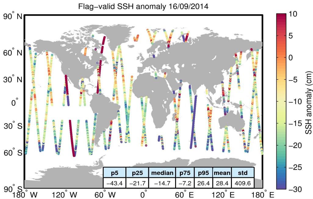
Figure 5. Geographical distribution of flag-valid 1-Hz SSH anomaly data over oceans and lakes for 16/09/2014. The statistical values shown in the table refer to the SSH anomaly in cm and are calculated over all measurements shown in the figure.
