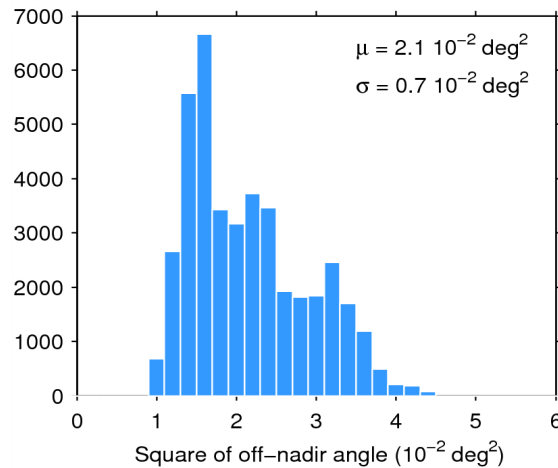
Figure 39. Histogram of flag-valid mispointing over oceans and lakes for 16/09/2014. The mean ( \mu ) and standard deviation ( \sigma ) are also shown. Note that values than 6 \cdot 10^{-2} \text{ deg}^2 are excluded from the histogram for the sake of readability but not from the computation of \mu and \sigma .
