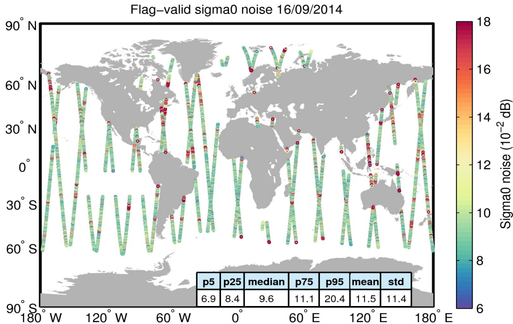
Figure 26. Geographical distribution of flag-valid 20-Hz sigma0 measurement noise over oceans and lakes for 16/09/2014. The statistical values shown in the table refer to the sigma0 noise and are calculated over all measurements shown in the figure.
