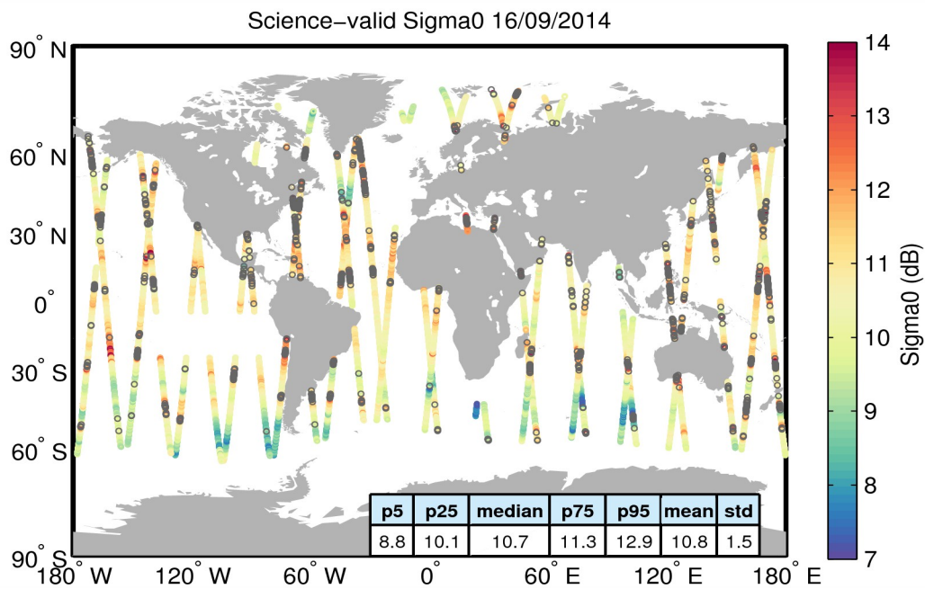
Figure 27. Geographical distribution of science-valid sigma0 data over oceans and lakes for 16/09/2014. The statistical values shown in the table refer to the sigma0 in dB and are calculated over all measurements shown in the figure. Gray circles denote records that have been rejected based on the editing criteria described in Table 4.
