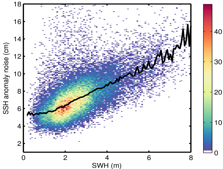
Figure 9. 2D histogram showing flag-valid SSH anomaly noise as a function of SWH for 16/09/2014. The black line denotes the median SSH anomaly as a function of SWH.
