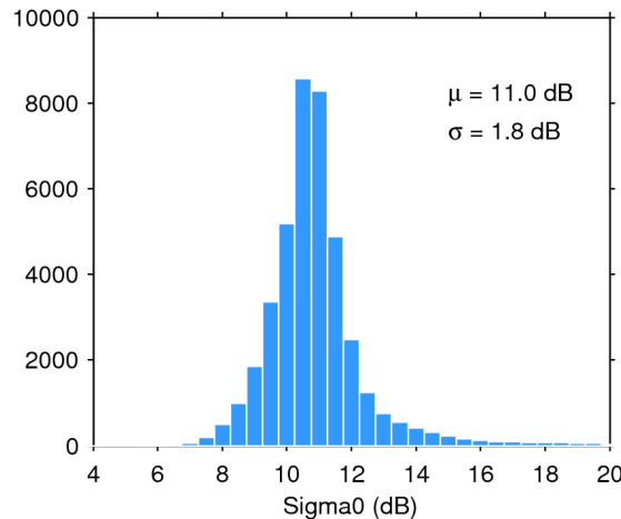
Figure 25. Histogram of flag-valid sigma0 over oceans and lakes for 16/09/2014. The mean ( \mu ) and standard deviation ( \sigma ) are also shown. Note that values outside [4 20] dB are excluded from the histogram for the sake of readability but not from the computation of \mu and \sigma .
