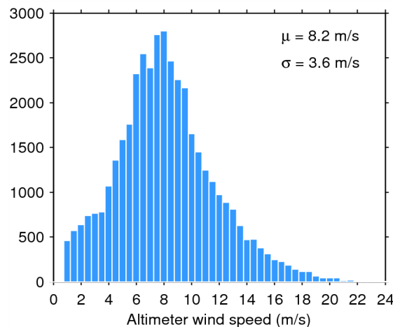
Figure 35. Histogram of science-valid wind over oceans and lakes for 16/09/2014. The mean ( \mu ) and standard deviation ( \sigma ) are also shown. Note that values larger than 24 m/s are excluded from the histogram for the sake of readability but not from the computation of \mu and \sigma .
