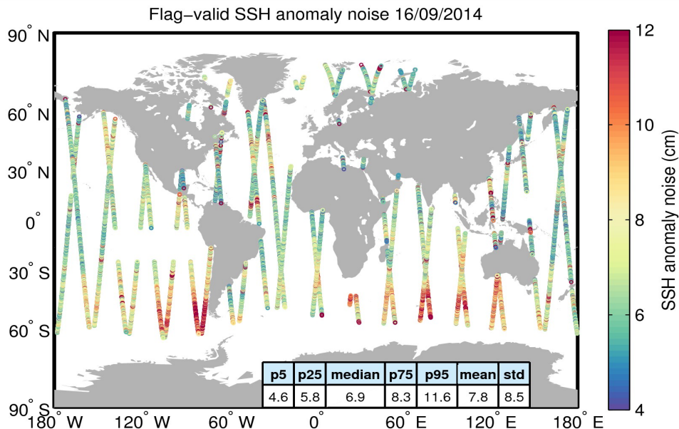
Figure 8. Geographical distribution of flag-valid 20-Hz SSH anomaly measurement noise over oceans and lakes for 16/09/2014. The statistical values shown in the table refer to the SSH anomaly noise and are calculated over all measurements shown in the figure.
