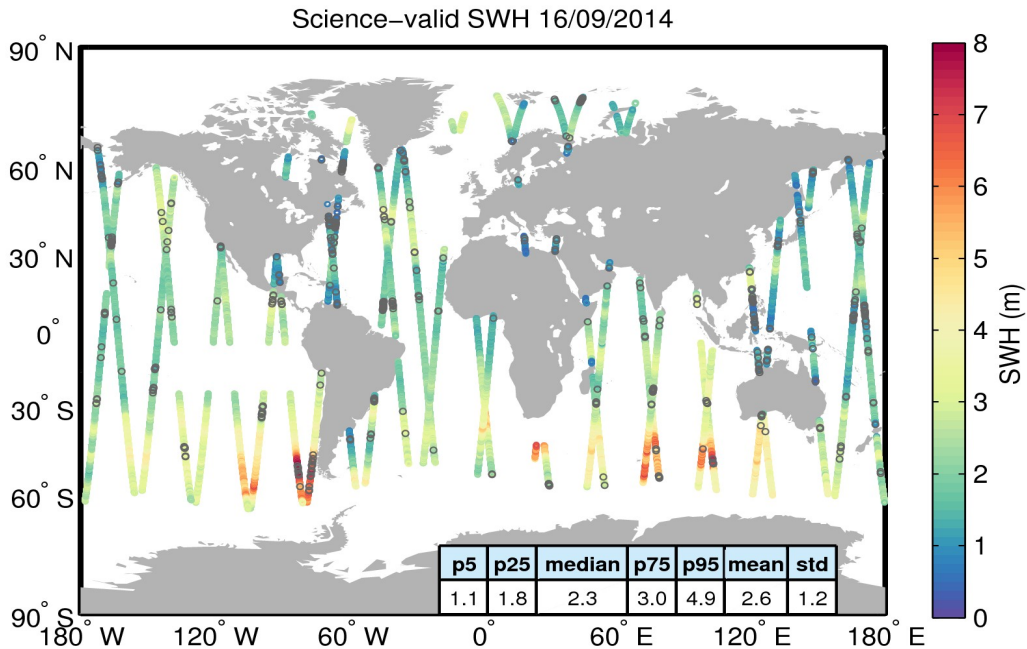
Figure 19. Geographical distribution of science-valid SWH data over oceans and lakes for 16/09/2014. The statistical values shown in the table refer to the SWH in m and are calculated over all measurements shown in the figure. Gray circles denote records that have been rejected based on the editing criteria described in Table 3.
