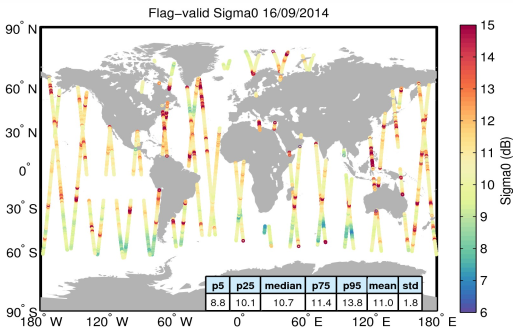
Figure 23. Geographical distribution of flag-valid sigma0 data over oceans and lakes for 16/09/2014. The statistical values shown in the table refer to the sigma0 in dB and are calculated over all measurements shown in the figure.
