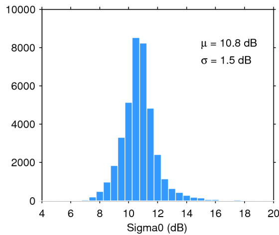
Figure 28. Histogram of science-valid sigma0 over oceans and lakes for 16/09/2014. The mean ( \mu ) and standard deviation ( \sigma ) are also shown. Note that values outside [4 20] dB are excluded from the histogram for the sake of readability but not from the computation of \mu and \sigma .
