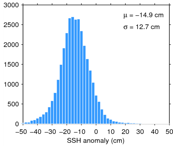
Figure 11. Histogram of science-valid SSH anomaly over oceans and lakes for 16/09/2014. The mean ( \mu ) and standard deviation ( \sigma ) are also shown. Note that values outside [-50 50] cm are excluded from the histogram for the sake of readability but not from the computation of \mu and \sigma .
