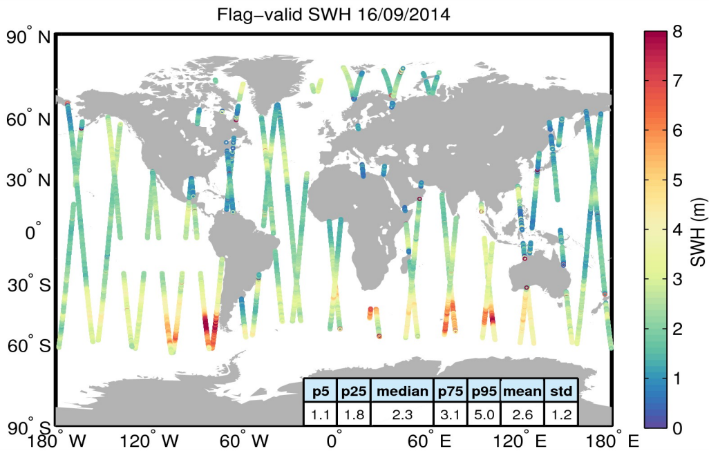
Figure 15. Geographical distribution of flag-valid SWH data over oceans and lakes for 16/09/2014. The statistical values shown in the table refer to the SWH in m and are calculated over all measurements shown in the figure.
