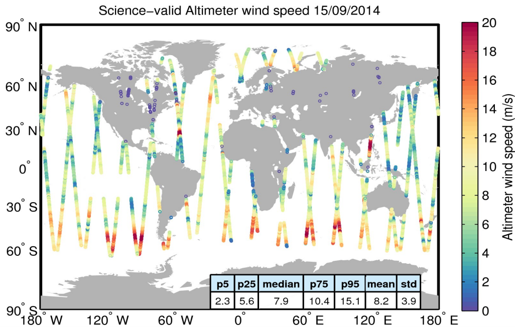
Figure 34. Geographical distribution of science-valid wind data over oceans and lakes for 15/09/2014. The statistical values shown in the table refer to the wind in m/s and are calculated over all measurements shown in the figure. Gray circles denote records that have been rejected based on the editing criteria described in Table 5.
