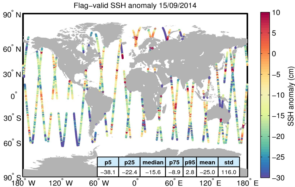
Figure 5. Geographical distribution of flag-valid 1-Hz SSH anomaly data over oceans and lakes for 15/09/2014. The statistical values shown in the table refer to the SSH anomaly in cm and are calculated over all measurements shown in the figure.
