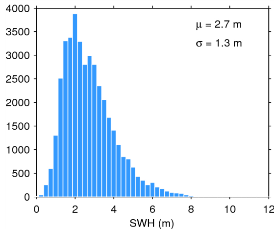
Figure 20. Histogram of science-valid SWH over oceans and lakes for 15/09/2014. The mean ( \mu ) and standard deviation ( \sigma ) are also shown. Note that values larger than 12 m are excluded from the histogram for the sake of readability but not from the computation of \mu and \sigma .
