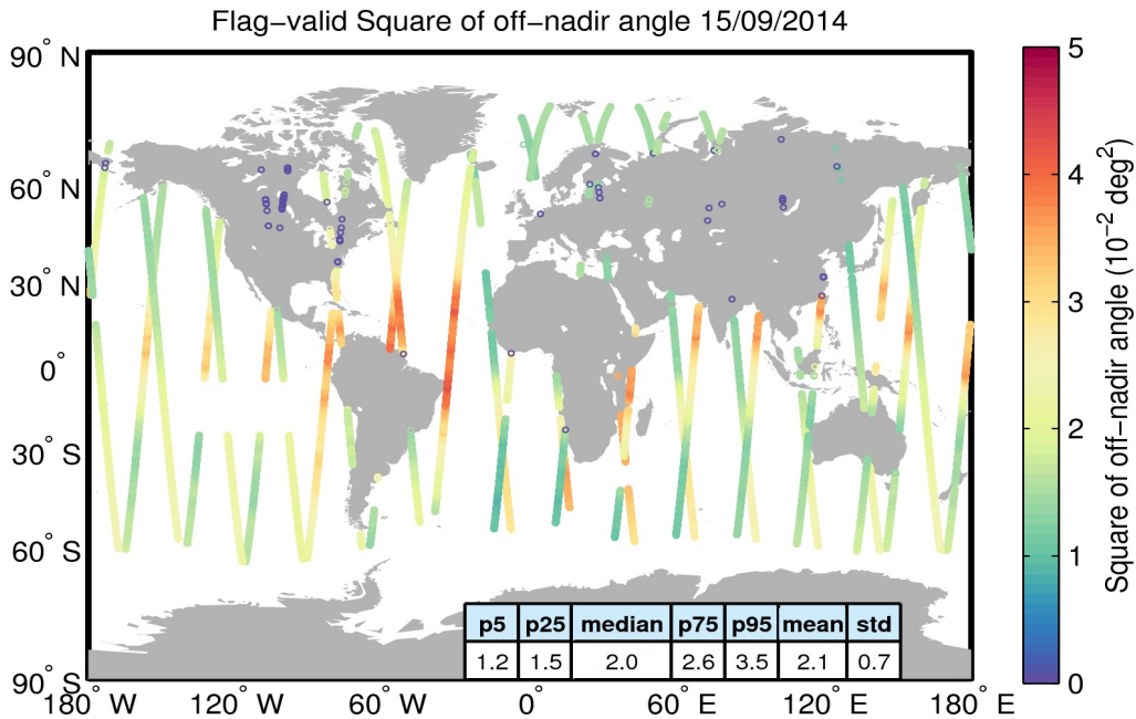
Figure 37. Geographical distribution of flag-valid mispointing data over oceans and lakes for 15/09/2014. The statistical values shown in the table refer to the mispointing in 10^{-2} \text{ deg}^2 and are calculated over all measurements shown in the figure.
