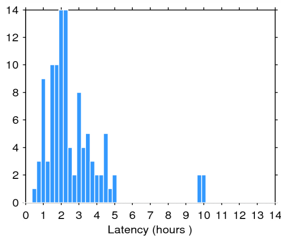
Figure 2. Histogram of the data latency for 15/09/2014. The y-axis denotes the number of files that are made available with a delay of x-hours with respect to the mean time of the records stored in the file.
