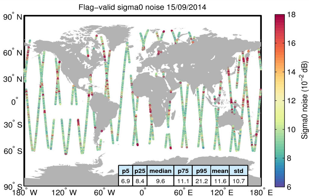
Figure 26. Geographical distribution of flag-valid 20-Hz sigma0 measurement noise over oceans and lakes for 15/09/2014. The statistical values shown in the table refer to the sigma0 noise and are calculated over all measurements shown in the figure.
