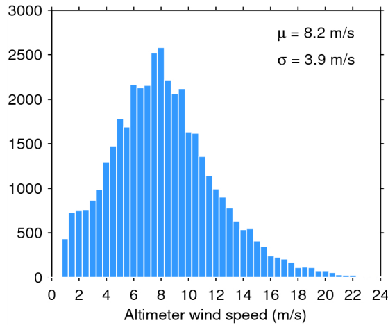
Figure 33. Histogram of flag-valid wind over oceans and lakes for 15/09/2014. The mean ( \mu ) and standard deviation ( \sigma ) are also shown. Note that values larger than 24 m/s are excluded from the histogram for the sake of readability but not from the computation of \mu and \sigma .
