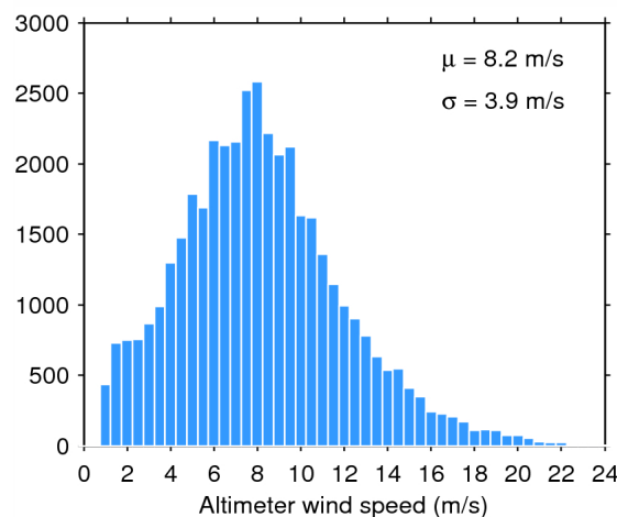
Figure 35. Histogram of science-valid wind over oceans and lakes for 15/09/2014. The mean ( \mu ) and standard deviation ( \sigma ) are also shown. Note that values larger than 24 m/s are excluded from the histogram for the sake of readability but not from the computation of \mu and \sigma .
