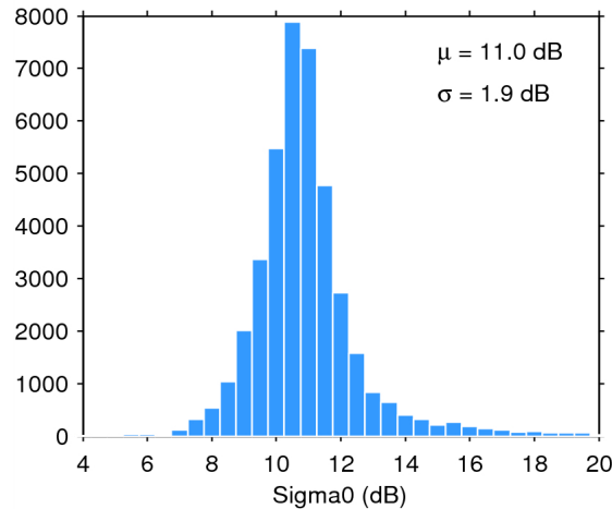
Figure 25. Histogram of flag-valid sigma0 over oceans and lakes for 15/09/2014. The mean ( \mu ) and standard deviation ( \sigma ) are also shown. Note that values outside [4 20] dB are excluded from the histogram for the sake of readability but not from the computation of \mu and \sigma .
