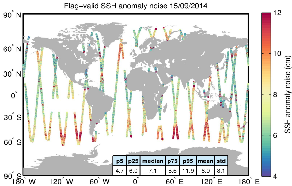
Figure 8. Geographical distribution of flag-valid 20-Hz SSH anomaly measurement noise over oceans and lakes for 15/09/2014. The statistical values shown in the table refer to the SSH anomaly noise and are calculated over all measurements shown in the figure.
