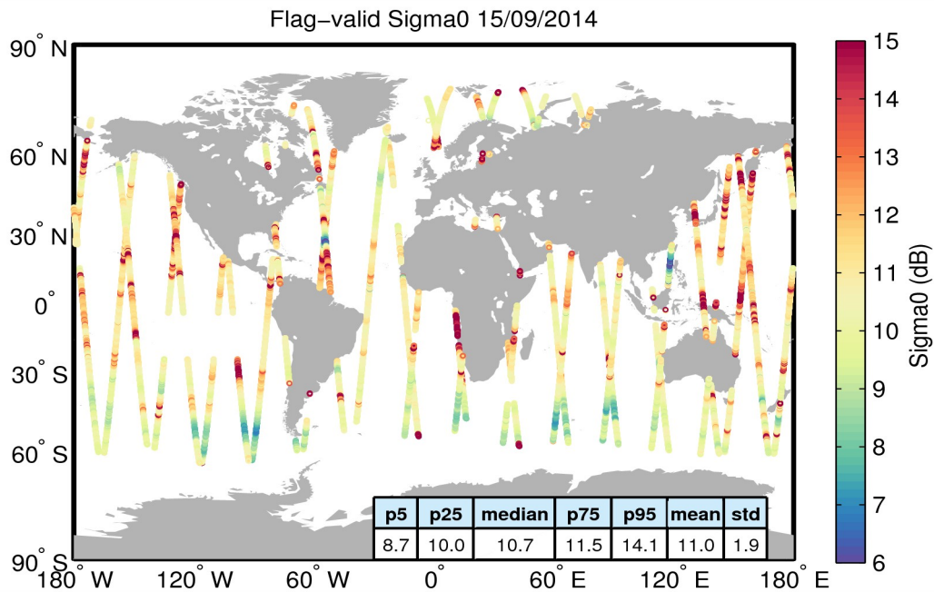
Figure 23. Geographical distribution of flag-valid sigma0 data over oceans and lakes for 15/09/2014. The statistical values shown in the table refer to the sigma0 in dB and are calculated over all measurements shown in the figure.
