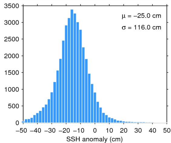
Figure 7. Histogram of flag-valid SSH anomaly over oceans and lakes for 15/09/2014. The mean ( \mu ) and standard deviation ( \sigma ) are also shown. Note that values outside [-50 50] cm are excluded from the histogram for the sake of readability but not from the computation of \mu and \sigma .
