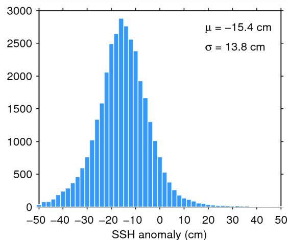
Figure 11. Histogram of science-valid SSH anomaly over oceans and lakes for 15/09/2014. The mean ( \mu ) and standard deviation ( \sigma ) are also shown. Note that values outside [-50 50] cm are excluded from the histogram for the sake of readability but not from the computation of \mu and \sigma .
