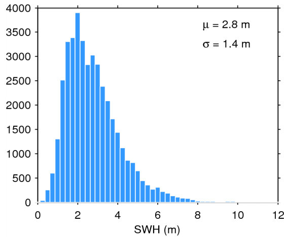
Figure 17. Histogram of flag-valid SWH over oceans and lakes for 15/09/2014. The mean ( \mu ) and standard deviation ( \sigma ) are also shown. Note that values larger than 12 m are excluded from the histogram for the sake of readability but not from the computation of \mu and \sigma .
