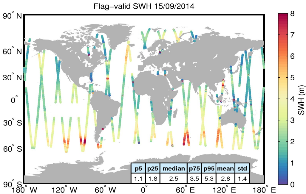
Figure 15. Geographical distribution of flag-valid SWH data over oceans and lakes for 15/09/2014. The statistical values shown in the table refer to the SWH in m and are calculated over all measurements shown in the figure.
