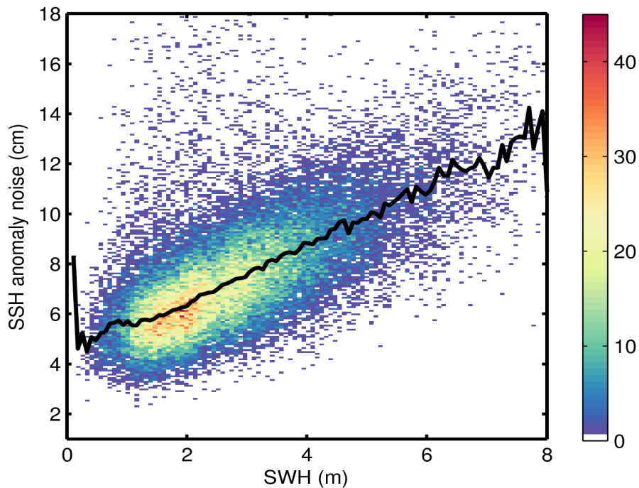
Figure 9. 2D histogram showing flag-valid SSH anomaly noise as a function of SWH for 15/09/2014. The black line denotes the median SSH anomaly as a function of SWH.
