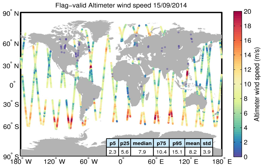
Figure 31. Geographical distribution of flag-valid wind data over oceans and lakes for 15/09/2014. The statistical values shown in the table refer to the wind in m/s and are calculated over all measurements shown in the figure.
