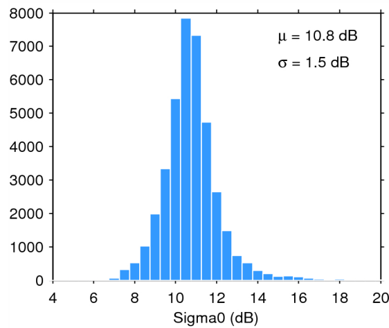
Figure 28. Histogram of science-valid sigma0 over oceans and lakes for 15/09/2014. The mean ( \mu ) and standard deviation ( \sigma ) are also shown. Note that values outside [4 20] dB are excluded from the histogram for the sake of readability but not from the computation of \mu and \sigma .
