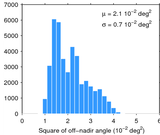
Figure 39. Histogram of flag-valid mispointing over oceans and lakes for 15/09/2014. The mean ( \mu ) and standard deviation ( \sigma ) are also shown. Note that values than 6 \cdot 10^{-2} \text{ deg}^2 are excluded from the histogram for the sake of readability but not from the computation of \mu and \sigma .
