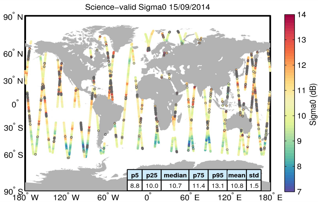
Figure 27. Geographical distribution of science-valid sigma0 data over oceans and lakes for 15/09/2014. The statistical values shown in the table refer to the sigma0 in dB and are calculated over all measurements shown in the figure. Gray circles denote records that have been rejected based on the editing criteria described in Table 4.
