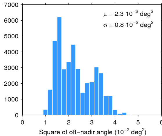
Figure 39. Histogram of flag-valid mispointing over oceans and lakes for 14/09/2014. The mean ( \mu ) and standard deviation ( \sigma ) are also shown. Note that values than 6 \cdot 10^{-2} \text{ deg}^2 are excluded from the histogram for the sake of readability but not from the computation of \mu and \sigma .
