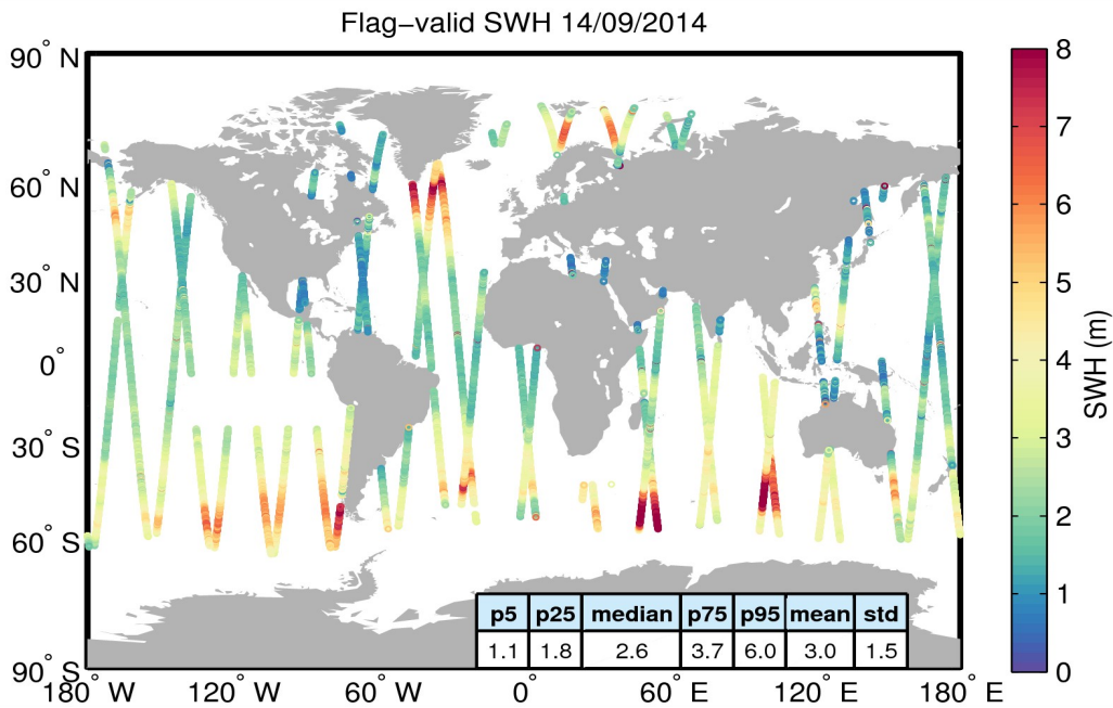
Figure 15. Geographical distribution of flag-valid SWH data over oceans and lakes for 14/09/2014. The statistical values shown in the table refer to the SWH in m and are calculated over all measurements shown in the figure.
