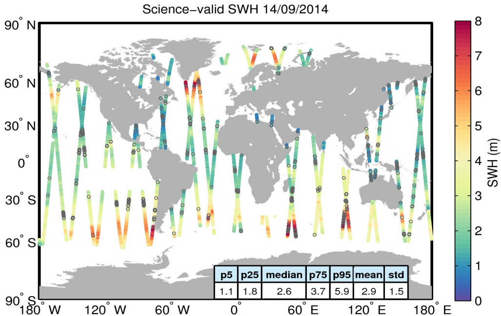
Figure 19. Geographical distribution of science-valid SWH data over oceans and lakes for 14/09/2014. The statistical values shown in the table refer to the SWH in m and are calculated over all measurements shown in the figure. Gray circles denote records that have been rejected based on the editing criteria described in Table 3.
