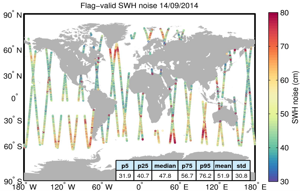
Figure 18. Geographical distribution of flag-valid 20-Hz SWH measurement noise over oceans and lakes for 14/09/2014. The statistical values shown in the figure refer to the SWH noise and are calculated over all measurements shown in the figure.
