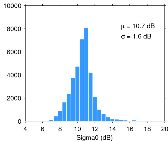
Figure 28. Histogram of science-valid sigma0 over oceans and lakes for 14/09/2014. The mean ( \mu ) and standard deviation ( \sigma ) are also shown. Note that values outside [4 20] dB are excluded from the histogram for the sake of readability but not from the computation of \mu and \sigma .
