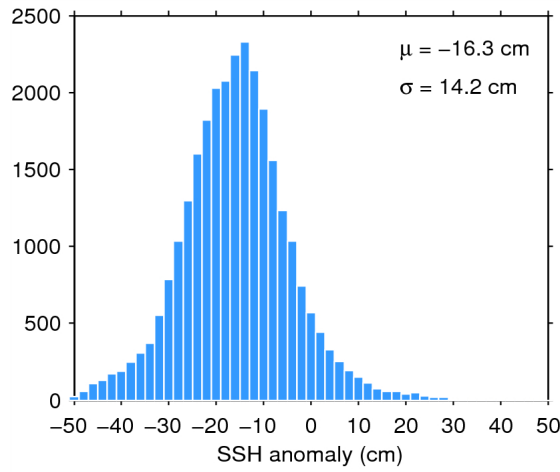
Figure 11. Histogram of science-valid SSH anomaly over oceans and lakes for 14/09/2014. The mean ( \mu ) and standard deviation ( \sigma ) are also shown. Note that values outside [-50 50] cm are excluded from the histogram for the sake of readability but not from the computation of \mu and \sigma .
