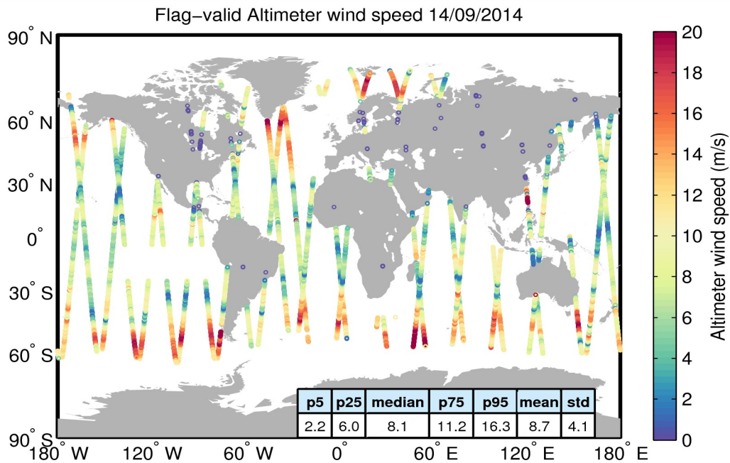
Figure 31. Geographical distribution of flag-valid wind data over oceans and lakes for 14/09/2014. The statistical values shown in the table refer to the wind in m/s and are calculated over all measurements shown in the figure.
