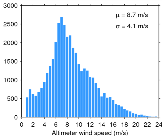
Figure 35. Histogram of science-valid wind over oceans and lakes for 14/09/2014. The mean ( \mu ) and standard deviation ( \sigma ) are also shown. Note that values larger than 24 m/s are excluded from the histogram for the sake of readability but not from the computation of \mu and \sigma .
