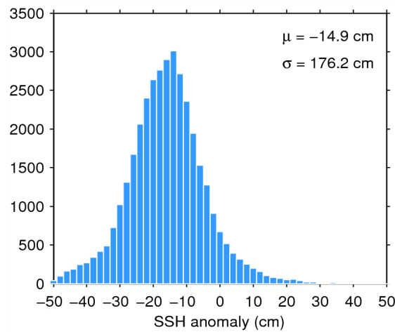
Figure 7. Histogram of flag-valid SSH anomaly over oceans and lakes for 14/09/2014. The mean ( \mu ) and standard deviation ( \sigma ) are also shown. Note that values outside [-50\ 50] cm are excluded from the histogram for the sake of readability but not from the computation of \mu and \sigma .
