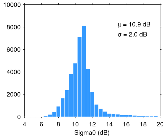
Figure 25. Histogram of flag-valid sigma0 over oceans and lakes for 14/09/2014. The mean ( \mu ) and standard deviation ( \sigma ) are also shown. Note that values outside [4 20] dB are excluded from the histogram for the sake of readability but not from the computation of \mu and \sigma .
