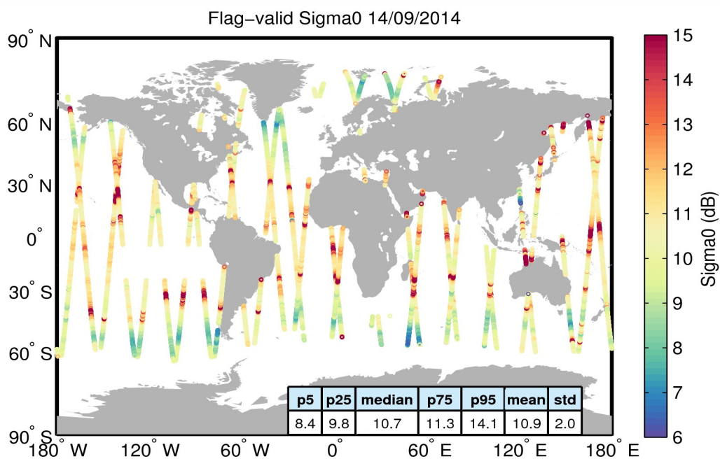
Figure 23. Geographical distribution of flag-valid sigma0 data over oceans and lakes for 14/09/2014. The statistical values shown in the table refer to the sigma0 in dB and are calculated over all measurements shown in the figure.
