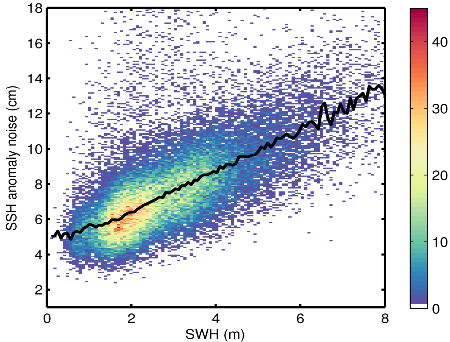
Figure 9. 2D histogram showing flag-valid SSH anomaly noise as a function of SWH for 14/09/2014. The black line denotes the median SSH anomaly as a function of SWH.
