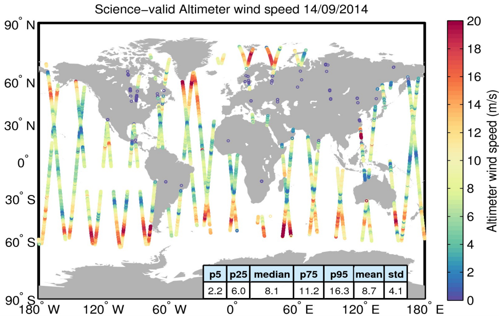
Figure 34. Geographical distribution of science-valid wind data over oceans and lakes for 14/09/2014. The statistical values shown in the table refer to the wind in m/s and are calculated over all measurements shown in the figure. Gray circles denote records that have been rejected based on the editing criteria described in Table 5.
