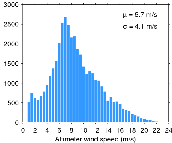
Figure 33. Histogram of flag-valid wind over oceans and lakes for 14/09/2014. The mean ( \mu ) and standard deviation ( \sigma ) are also shown. Note that values larger than 24 m/s are excluded from the histogram for the sake of readability but not from the computation of \mu and \sigma .
