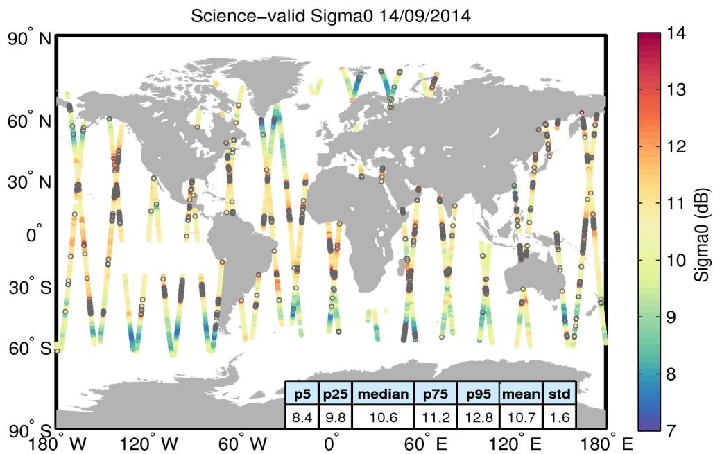
Figure 27. Geographical distribution of science-valid sigma0 data over oceans and lakes for 14/09/2014. The statistical values shown in the table refer to the sigma0 in dB and are calculated over all measurements shown in the figure. Gray circles denote records that have been rejected based on the editing criteria described in Table 4.
