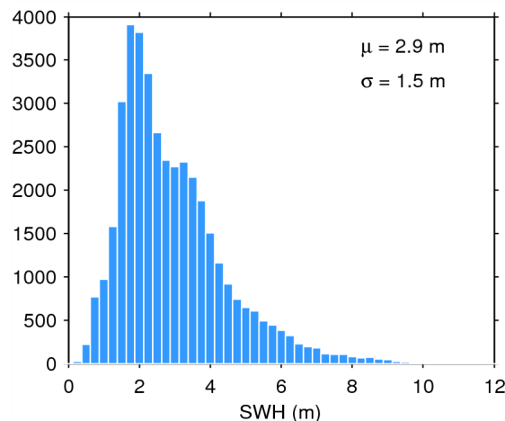
Figure 20. Histogram of science-valid SWH over oceans and lakes for 14/09/2014. The mean ( \mu ) and standard deviation ( \sigma ) are also shown. Note that values larger than 12 m are excluded from the histogram for the sake of readability but not from the computation of \mu and \sigma .
