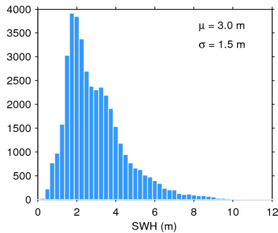
Figure 17. Histogram of flag-valid SWH over oceans and lakes for 14/09/2014. The mean ( \mu ) and standard deviation ( \sigma ) are also shown. Note that values larger than 12 m are excluded from the histogram for the sake of readability but not from the computation of \mu and \sigma .
