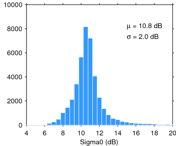
Figure 25. Histogram of flag-valid sigma0 over oceans and lakes for 13/09/2014. The mean ( \mu ) and standard deviation ( \sigma ) are also shown. Note that values outside [4 20] dB are excluded from the histogram for the sake of readability but not from the computation of \mu and \sigma .
