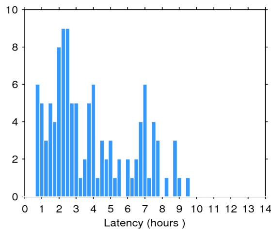
Figure 2. Histogram of the data latency for 13/09/2014. The y-axis denotes the number of files that are made available with a delay of x-hours with respect to the mean time of the records stored in the file.
