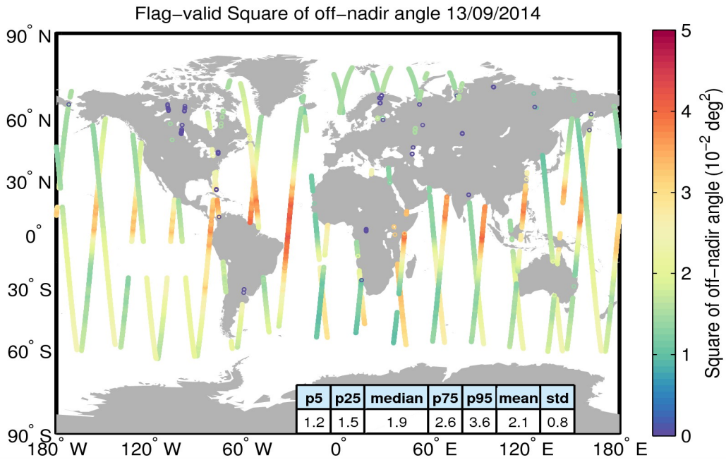
Figure 37. Geographical distribution of flag-valid mispointing data over oceans and lakes for 13/09/2014. The statistical values shown in the table refer to the mispointing in 10^{-2} \text{ deg}^2 and are calculated over all measurements shown in the figure.
