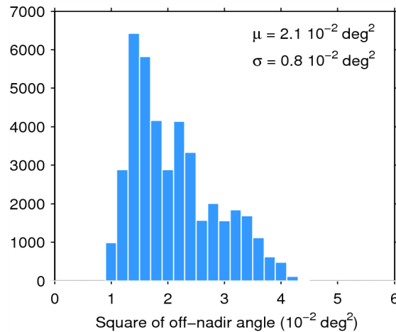
Figure 39. Histogram of flag-valid mispointing over oceans and lakes for 13/09/2014. The mean ( \mu ) and standard deviation ( \sigma ) are also shown. Note that values than 6 \cdot 10^{-2} \text{ deg}^2 are excluded from the histogram for the sake of readability but not from the computation of \mu and \sigma .
