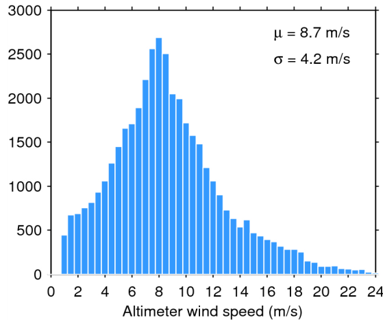
Figure 33. Histogram of flag-valid wind over oceans and lakes for 13/09/2014. The mean ( \mu ) and standard deviation ( \sigma ) are also shown. Note that values larger than 24 m/s are excluded from the histogram for the sake of readability but not from the computation of \mu and \sigma .
