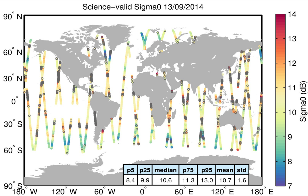
Figure 27. Geographical distribution of science-valid sigma0 data over oceans and lakes for 13/09/2014. The statistical values shown in the table refer to the sigma0 in dB and are calculated over all measurements shown in the figure. Gray circles denote records that have been rejected based on the editing criteria described in Table 4.
