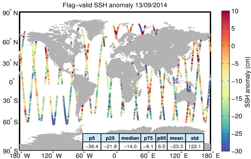
Figure 5. Geographical distribution of flag-valid 1-Hz SSH anomaly data over oceans and lakes for 13/09/2014. The statistical values shown in the table refer to the SSH anomaly in cm and are calculated over all measurements shown in the figure.
