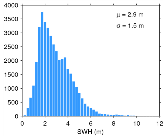
Figure 17. Histogram of flag-valid SWH over oceans and lakes for 13/09/2014. The mean ( \mu ) and standard deviation ( \sigma ) are also shown. Note that values larger than 12 m are excluded from the histogram for the sake of readability but not from the computation of \mu and \sigma .
