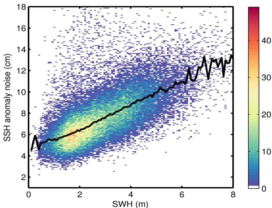
Figure 9. 2D histogram showing flag-valid SSH anomaly noise as a function of SWH for 13/09/2014. The black line denotes the median SSH anomaly as a function of SWH.
