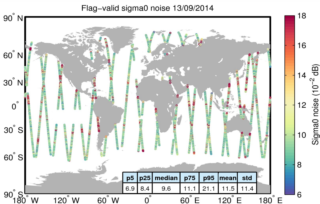
Figure 26. Geographical distribution of flag-valid 20-Hz sigma0 measurement noise over oceans and lakes for 13/09/2014. The statistical values shown in the table refer to the sigma0 noise and are calculated over all measurements shown in the figure.
