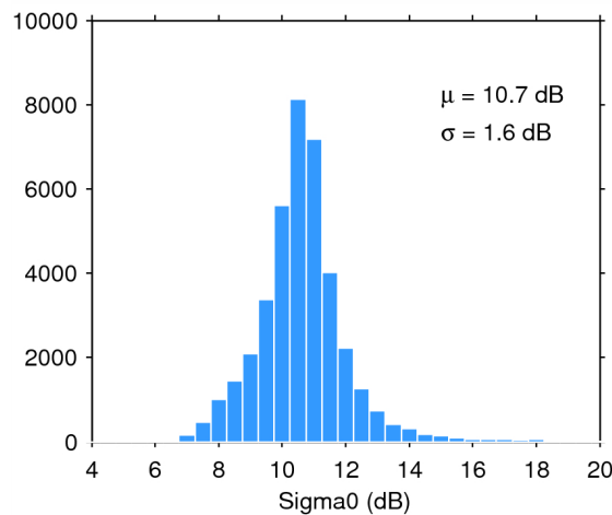
Figure 28. Histogram of science-valid sigma0 over oceans and lakes for 13/09/2014. The mean ( \mu ) and standard deviation ( \sigma ) are also shown. Note that values outside [4 20] dB are excluded from the histogram for the sake of readability but not from the computation of \mu and \sigma .
