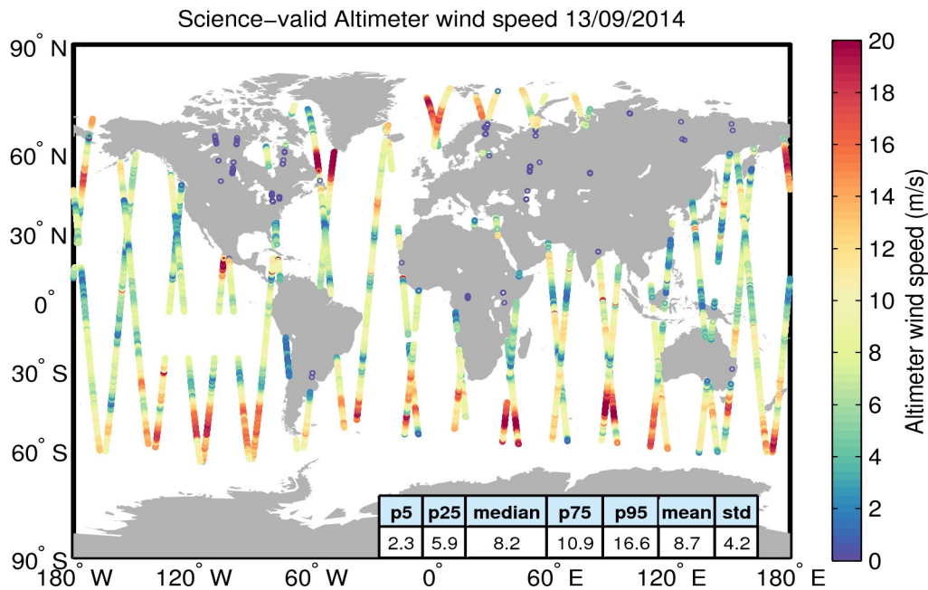
Figure 34. Geographical distribution of science-valid wind data over oceans and lakes for 13/09/2014. The statistical values shown in the table refer to the wind in m/s and are calculated over all measurements shown in the figure. Gray circles denote records that have been rejected based on the editing criteria described in Table 5.
