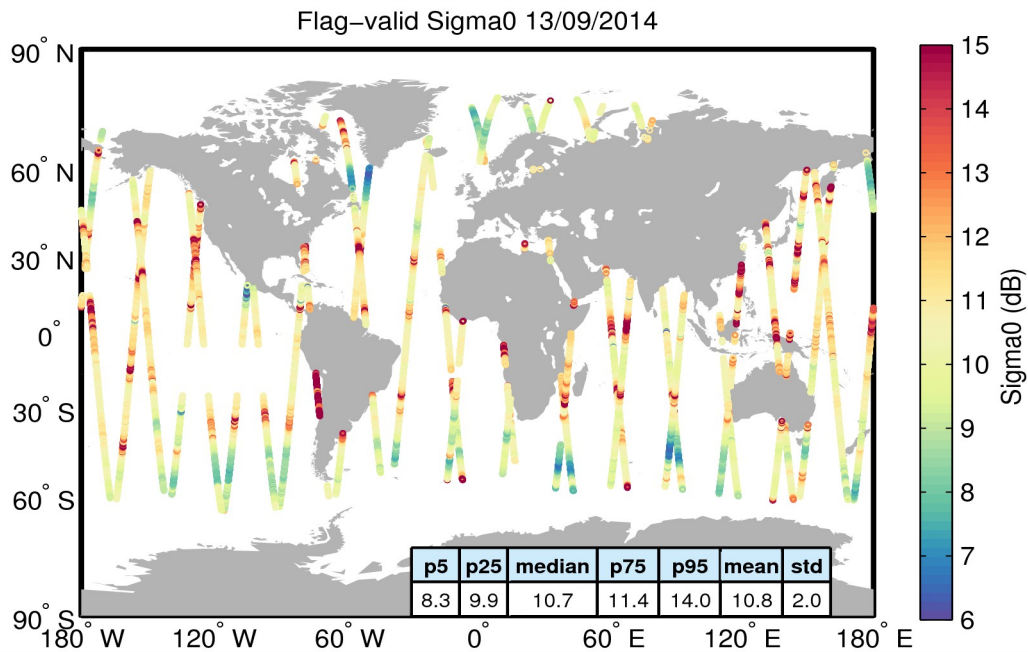
Figure 23. Geographical distribution of flag-valid sigma0 data over oceans and lakes for 13/09/2014. The statistical values shown in the table refer to the sigma0 in dB and are calculated over all measurements shown in the figure.
