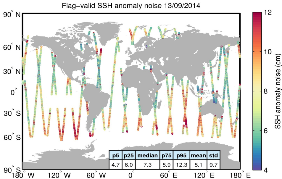
Figure 8. Geographical distribution of flag-valid 20-Hz SSH anomaly measurement noise over oceans and lakes for 13/09/2014. The statistical values shown in the table refer to the SSH anomaly noise and are calculated over all measurements shown in the figure.
