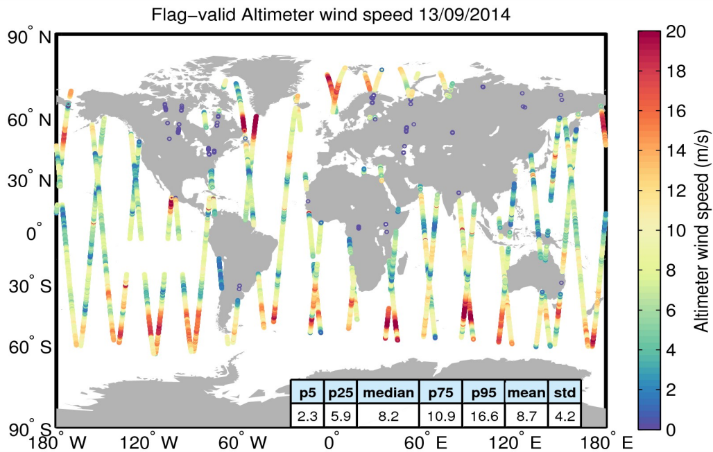
Figure 31. Geographical distribution of flag-valid wind data over oceans and lakes for 13/09/2014. The statistical values shown in the table refer to the wind in m/s and are calculated over all measurements shown in the figure.
