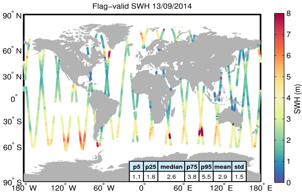
Figure 15. Geographical distribution of flag-valid SWH data over oceans and lakes for 13/09/2014. The statistical values shown in the table refer to the SWH in m and are calculated over all measurements shown in the figure.
