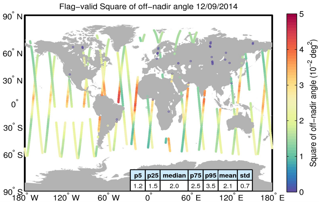
Figure 37. Geographical distribution of flag-valid mispointing data over oceans and lakes for 12/09/2014. The statistical values shown in the table refer to the mispointing in 10^{-2} \text{ deg}^2 and are calculated over all measurements shown in the figure.
