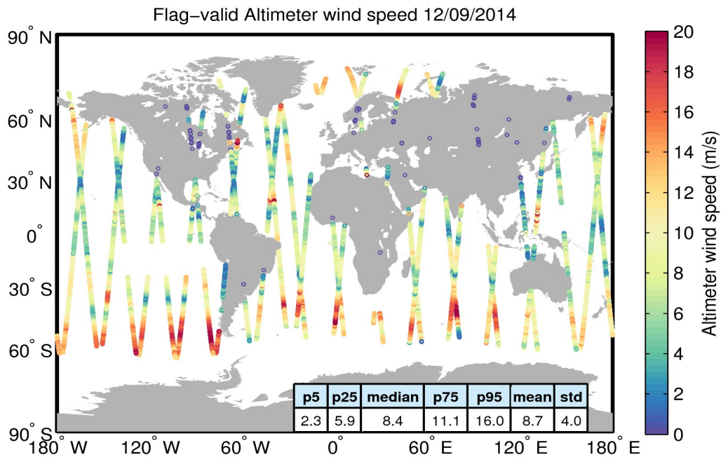
Figure 31. Geographical distribution of flag-valid wind data over oceans and lakes for 12/09/2014. The statistical values shown in the table refer to the wind in m/s and are calculated over all measurements shown in the figure.
