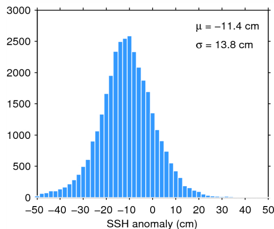
Figure 11. Histogram of science-valid SSH anomaly over oceans and lakes for 12/09/2014. The mean ( \mu ) and standard deviation ( \sigma ) are also shown. Note that values outside [-50 50] cm are excluded from the histogram for the sake of readability but not from the computation of \mu and \sigma .
