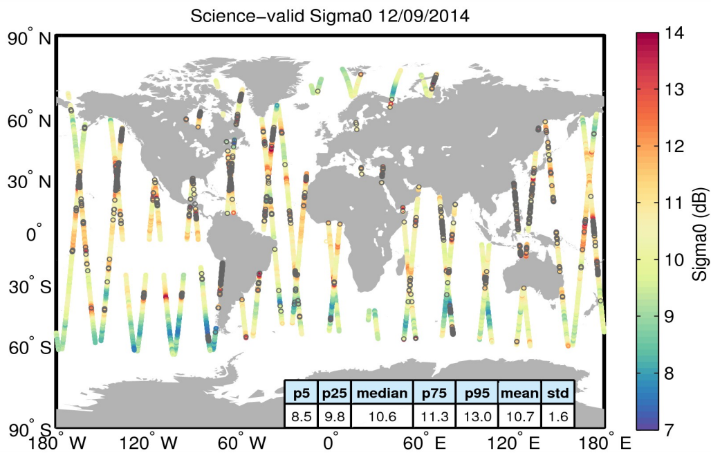
Figure 27. Geographical distribution of science-valid sigma0 data over oceans and lakes for 12/09/2014. The statistical values shown in the table refer to the sigma0 in dB and are calculated over all measurements shown in the figure. Gray circles denote records that have been rejected based on the editing criteria described in Table 4.
