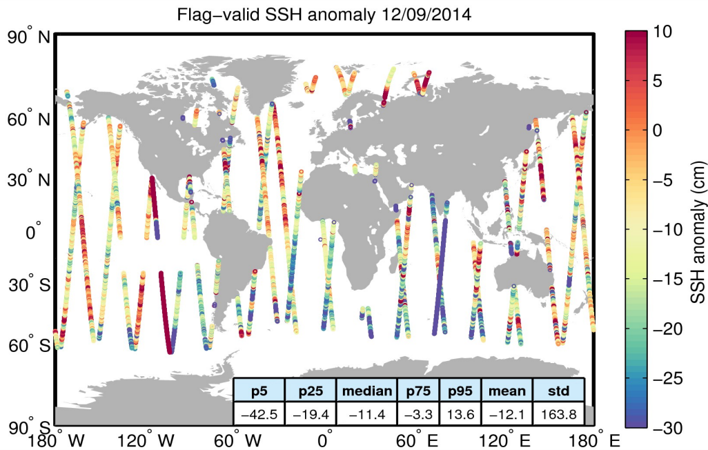
Figure 5. Geographical distribution of flag-valid 1-Hz SSH anomaly data over oceans and lakes for 12/09/2014. The statistical values shown in the table refer to the SSH anomaly in cm and are calculated over all measurements shown in the figure.
