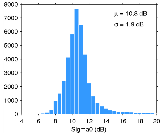
Figure 25. Histogram of flag-valid sigma0 over oceans and lakes for 12/09/2014. The mean ( \mu ) and standard deviation ( \sigma ) are also shown. Note that values outside [4 20] dB are excluded from the histogram for the sake of readability but not from the computation of \mu and \sigma .
