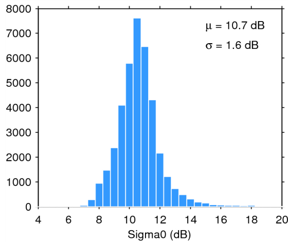
Figure 28. Histogram of science-valid sigma0 over oceans and lakes for 12/09/2014. The mean ( \mu ) and standard deviation ( \sigma ) are also shown. Note that values outside [4 20] dB are excluded from the histogram for the sake of readability but not from the computation of \mu and \sigma .
