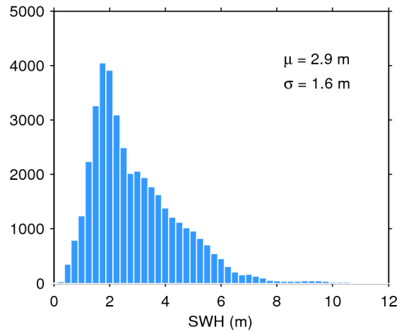
Figure 17. Histogram of flag-valid SWH over oceans and lakes for 12/09/2014. The mean ( \mu ) and standard deviation ( \sigma ) are also shown. Note that values larger than 12 m are excluded from the histogram for the sake of readability but not from the computation of \mu and \sigma .
