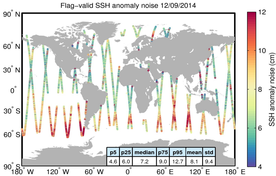
Figure 8. Geographical distribution of flag-valid 20-Hz SSH anomaly measurement noise over oceans and lakes for 12/09/2014. The statistical values shown in the table refer to the SSH anomaly noise and are calculated over all measurements shown in the figure.
