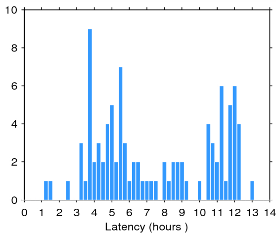
Figure 2. Histogram of the data latency for 12/09/2014. The y-axis denotes the number of files that are made available with a delay of x-hours with respect to the mean time of the records stored in the file.
