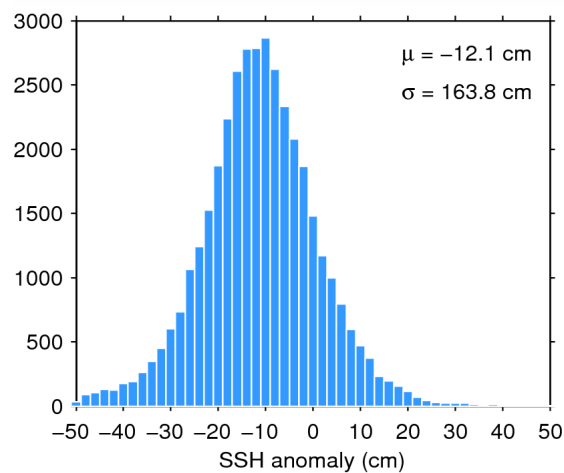
Figure 7. Histogram of flag-valid SSH anomaly over oceans and lakes for 12/09/2014. The mean ( \mu ) and standard deviation ( \sigma ) are also shown. Note that values outside [-50 \ 50] cm are excluded from the histogram for the sake of readability but not from the computation of \mu and \sigma .
