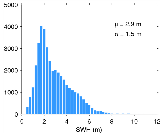
Figure 20. Histogram of science-valid SWH over oceans and lakes for 12/09/2014. The mean ( \mu ) and standard deviation ( \sigma ) are also shown. Note that values larger than 12 m are excluded from the histogram for the sake of readability but not from the computation of \mu and \sigma .
