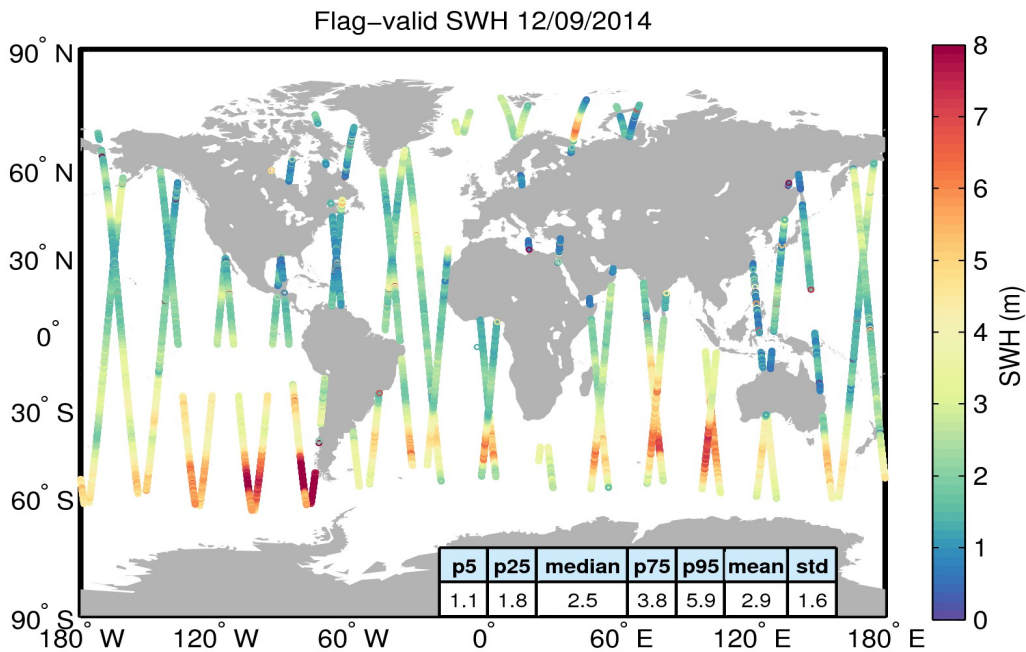
Figure 15. Geographical distribution of flag-valid SWH data over oceans and lakes for 12/09/2014. The statistical values shown in the table refer to the SWH in m and are calculated over all measurements shown in the figure.
