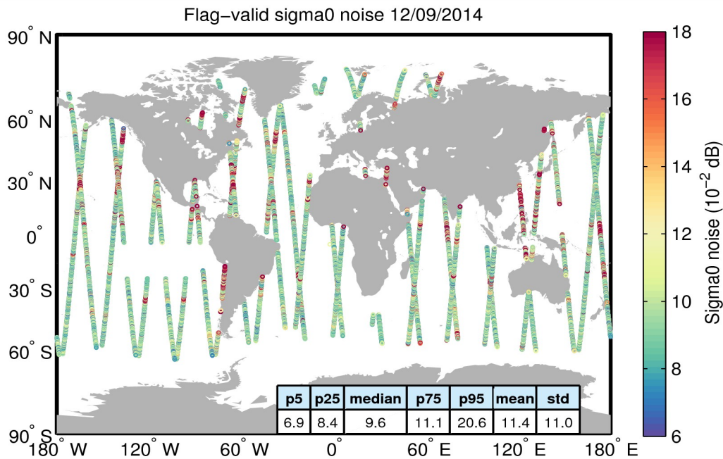
Figure 26. Geographical distribution of flag-valid 20-Hz sigma0 measurement noise over oceans and lakes for 12/09/2014. The statistical values shown in the table refer to the sigma0 noise and are calculated over all measurements shown in the figure.
