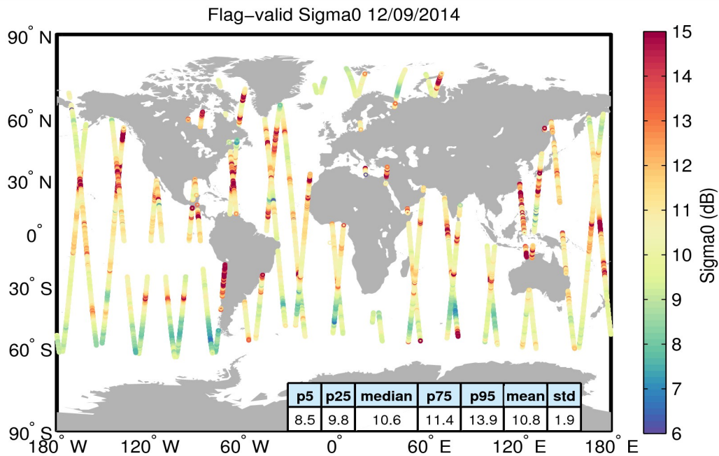
Figure 23. Geographical distribution of flag-valid sigma0 data over oceans and lakes for 12/09/2014. The statistical values shown in the table refer to the sigma0 in dB and are calculated over all measurements shown in the figure.
