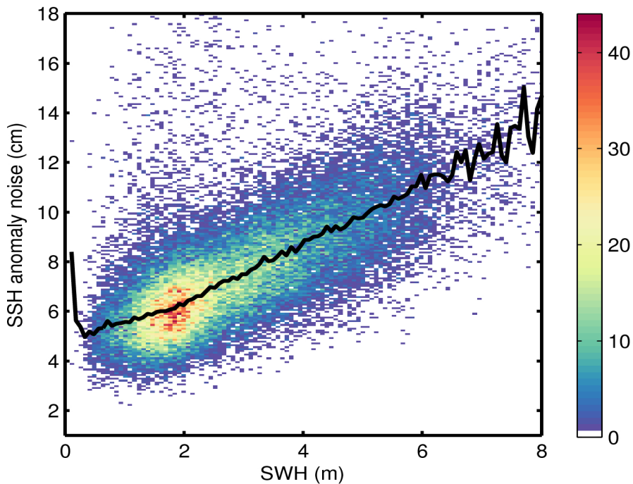
Figure 9. 2D histogram showing flag-valid SSH anomaly noise as a function of SWH for 12/09/2014. The black line denotes the median SSH anomaly as a function of SWH.
