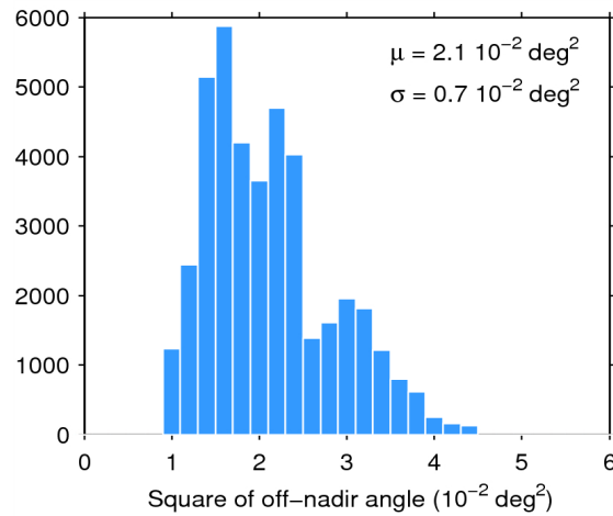
Figure 39. Histogram of flag-valid mispointing over oceans and lakes for 12/09/2014. The mean ( \mu ) and standard deviation ( \sigma ) are also shown. Note that values than 6 \cdot 10^{-2} \text{ deg}^2 are excluded from the histogram for the sake of readability but not from the computation of \mu and \sigma .
