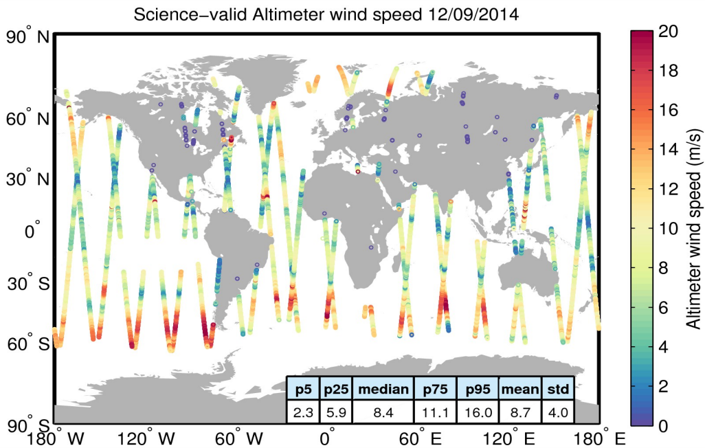
Figure 34. Geographical distribution of science-valid wind data over oceans and lakes for 12/09/2014. The statistical values shown in the table refer to the wind in m/s and are calculated over all measurements shown in the figure. Gray circles denote records that have been rejected based on the editing criteria described in Table 5.
