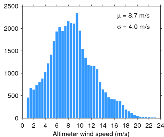
Figure 35. Histogram of science-valid wind over oceans and lakes for 12/09/2014. The mean ( \mu ) and standard deviation ( \sigma ) are also shown. Note that values larger than 24 m/s are excluded from the histogram for the sake of readability but not from the computation of \mu and \sigma .
