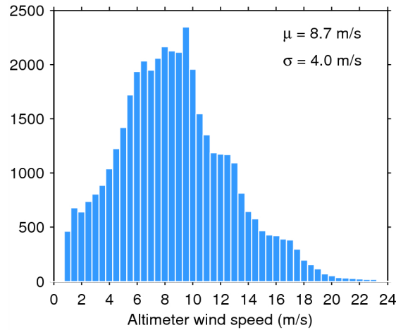
Figure 33. Histogram of flag-valid wind over oceans and lakes for 12/09/2014. The mean ( \mu ) and standard deviation ( \sigma ) are also shown. Note that values larger than 24 m/s are excluded from the histogram for the sake of readability but not from the computation of \mu and \sigma .
