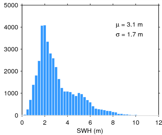
Figure 17. Histogram of flag-valid SWH over oceans and lakes for 11/09/2014. The mean ( \mu ) and standard deviation ( \sigma ) are also shown. Note that values larger than 12 m are excluded from the histogram for the sake of readability but not from the computation of \mu and \sigma .
