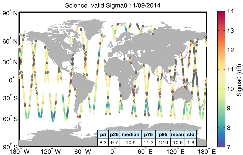
Figure 27. Geographical distribution of science-valid sigma0 data over oceans and lakes for 11/09/2014. The statistical values shown in the table refer to the sigma0 in dB and are calculated over all measurements shown in the figure. Gray circles denote records that have been rejected based on the editing criteria described in Table 4.
