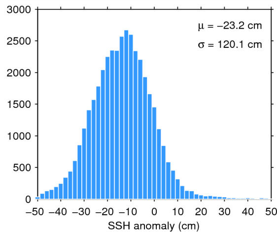
Figure 7. Histogram of flag-valid SSH anomaly over oceans and lakes for 11/09/2014. The mean ( \mu ) and standard deviation ( \sigma ) are also shown. Note that values outside [-50\ 50] cm are excluded from the histogram for the sake of readability but not from the computation of \mu and \sigma .
