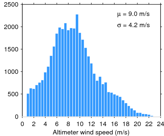
Figure 33. Histogram of flag-valid wind over oceans and lakes for 11/09/2014. The mean ( \mu ) and standard deviation ( \sigma ) are also shown. Note that values larger than 24 m/s are excluded from the histogram for the sake of readability but not from the computation of \mu and \sigma .
