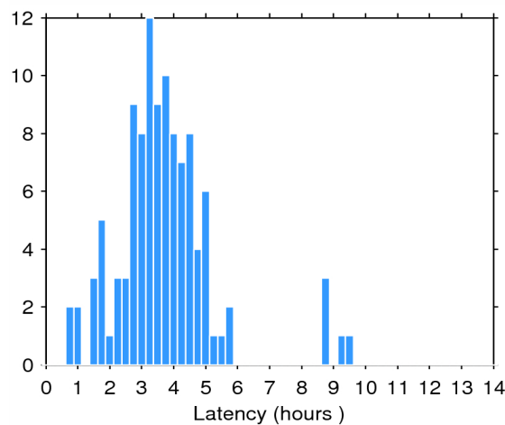
Figure 2. Histogram of the data latency for 11/09/2014. The y-axis denotes the number of files that are made available with a delay of x-hours with respect to the mean time of the records stored in the file.
