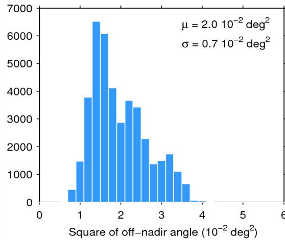
Figure 39. Histogram of flag-valid mispointing over oceans and lakes for 11/09/2014. The mean ( \mu ) and standard deviation ( \sigma ) are also shown. Note that values than 6 \cdot 10^{-2} \text{ deg}^2 are excluded from the histogram for the sake of readability but not from the computation of \mu and \sigma .
