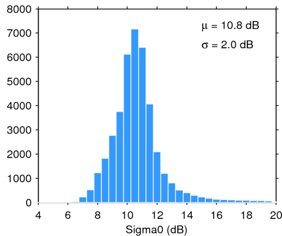
Figure 25. Histogram of flag-valid sigma0 over oceans and lakes for 11/09/2014. The mean ( \mu ) and standard deviation ( \sigma ) are also shown. Note that values outside [4 20] dB are excluded from the histogram for the sake of readability but not from the computation of \mu and \sigma .
