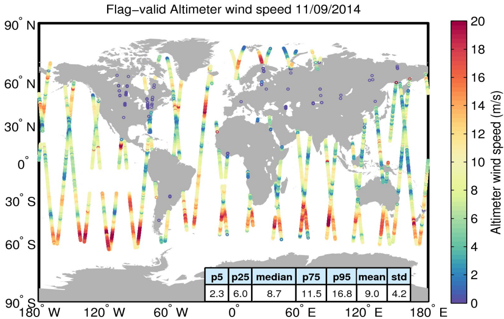
Figure 31. Geographical distribution of flag-valid wind data over oceans and lakes for 11/09/2014. The statistical values shown in the table refer to the wind in m/s and are calculated over all measurements shown in the figure.
