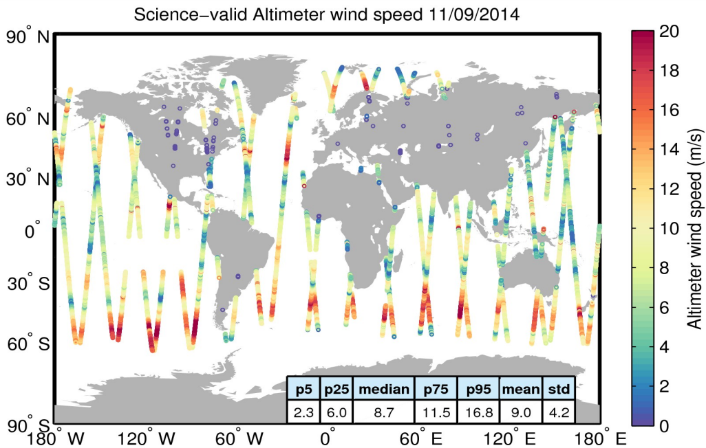
Figure 34. Geographical distribution of science-valid wind data over oceans and lakes for 11/09/2014. The statistical values shown in the table refer to the wind in m/s and are calculated over all measurements shown in the figure. Gray circles denote records that have been rejected based on the editing criteria described in Table 5.
