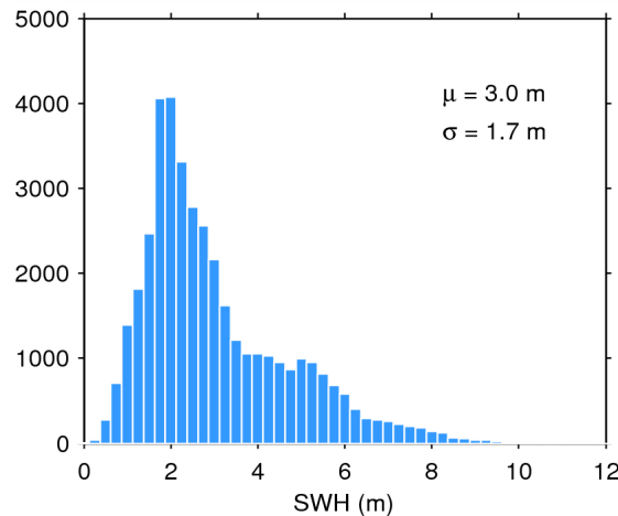
Figure 20. Histogram of science-valid SWH over oceans and lakes for 11/09/2014. The mean ( \mu ) and standard deviation ( \sigma ) are also shown. Note that values larger than 12 m are excluded from the histogram for the sake of readability but not from the computation of \mu and \sigma .
