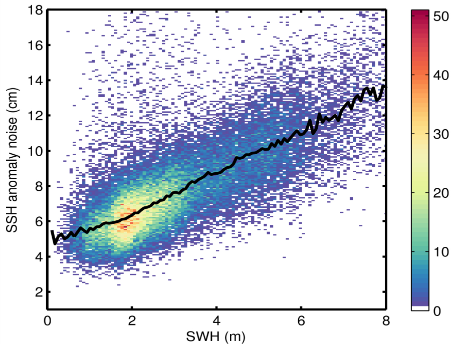
Figure 9. 2D histogram showing flag-valid SSH anomaly noise as a function of SWH for 11/09/2014. The black line denotes the median SSH anomaly as a function of SWH.
