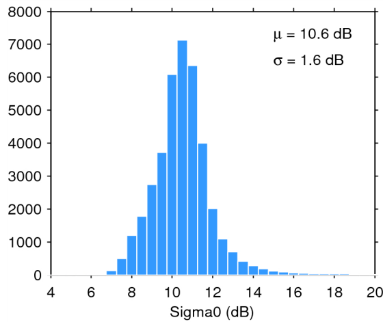
Figure 28. Histogram of science-valid sigma0 over oceans and lakes for 11/09/2014. The mean ( \mu ) and standard deviation ( \sigma ) are also shown. Note that values outside [4 20] dB are excluded from the histogram for the sake of readability but not from the computation of \mu and \sigma .
