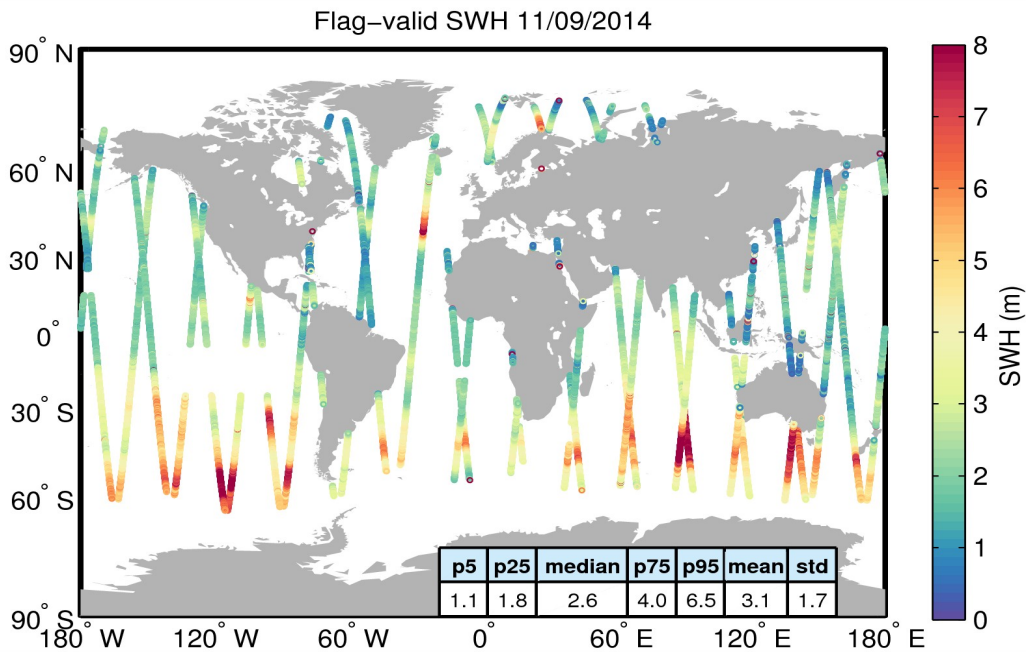
Figure 15. Geographical distribution of flag-valid SWH data over oceans and lakes for 11/09/2014. The statistical values shown in the table refer to the SWH in m and are calculated over all measurements shown in the figure.
