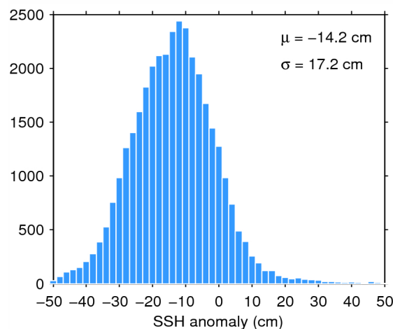
Figure 11. Histogram of science-valid SSH anomaly over oceans and lakes for 11/09/2014. The mean ( \mu ) and standard deviation ( \sigma ) are also shown. Note that values outside [-50 50] cm are excluded from the histogram for the sake of readability but not from the computation of \mu and \sigma .
