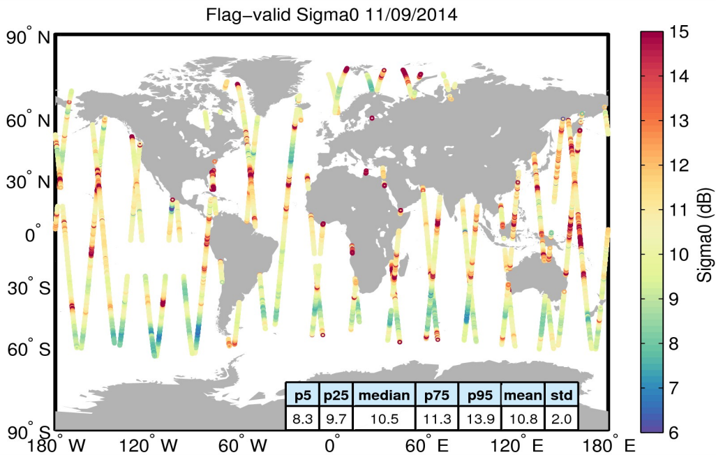
Figure 23. Geographical distribution of flag-valid sigma0 data over oceans and lakes for 11/09/2014. The statistical values shown in the table refer to the sigma0 in dB and are calculated over all measurements shown in the figure.
