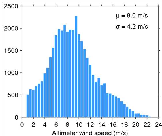
Figure 35. Histogram of science-valid wind over oceans and lakes for 11/09/2014. The mean ( \mu ) and standard deviation ( \sigma ) are also shown. Note that values larger than 24 m/s are excluded from the histogram for the sake of readability but not from the computation of \mu and \sigma .
