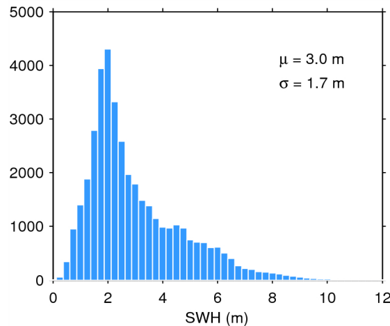
Figure 20. Histogram of science-valid SWH over oceans and lakes for 10/09/2014. The mean ( \mu ) and standard deviation ( \sigma ) are also shown. Note that values larger than 12 m are excluded from the histogram for the sake of readability but not from the computation of \mu and \sigma .
