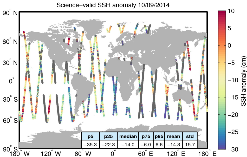
Figure 10. Geographical distribution of science-valid SSH anomaly data over oceans and lakes for 10/09/2014. The statistical values shown in the table refer to the SSH anomaly in cm and are calculated over all measurements shown in the figure. Gray circles denote records that have been rejected based on the editing criteria described in Table 2.
