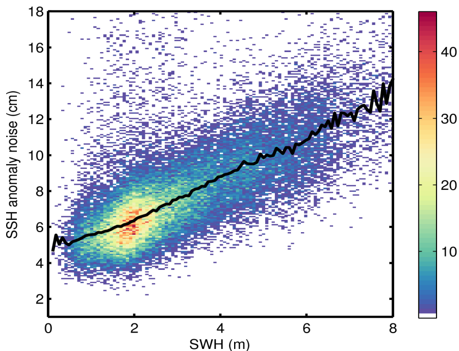
Figure 9. 2D histogram showing flag-valid SSH anomaly noise as a function of SWH for 10/09/2014. The black line denotes the median SSH anomaly as a function of SWH.
