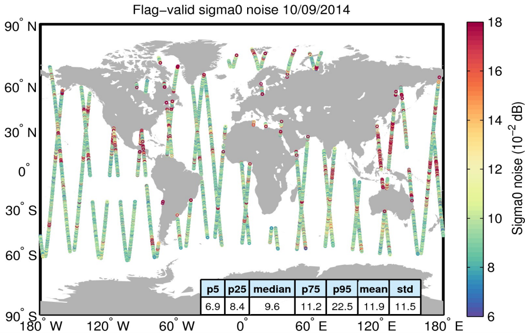
Figure 26. Geographical distribution of flag-valid 20-Hz sigma0 measurement noise over oceans and lakes for 10/09/2014. The statistical values shown in the table refer to the sigma0 noise and are calculated over all measurements shown in the figure.
