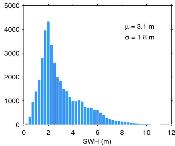
Figure 17. Histogram of flag-valid SWH over oceans and lakes for 10/09/2014. The mean ( \mu ) and standard deviation ( \sigma ) are also shown. Note that values larger than 12 m are excluded from the histogram for the sake of readability but not from the computation of \mu and \sigma .
