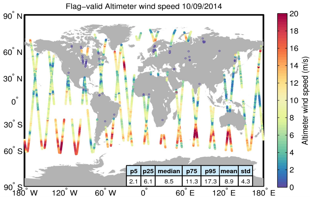
Figure 31. Geographical distribution of flag-valid wind data over oceans and lakes for 10/09/2014. The statistical values shown in the table refer to the wind in m/s and are calculated over all measurements shown in the figure.
