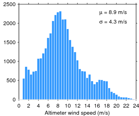
Figure 33. Histogram of flag-valid wind over oceans and lakes for 10/09/2014. The mean ( \mu ) and standard deviation ( \sigma ) are also shown. Note that values larger than 24 m/s are excluded from the histogram for the sake of readability but not from the computation of \mu and \sigma .
