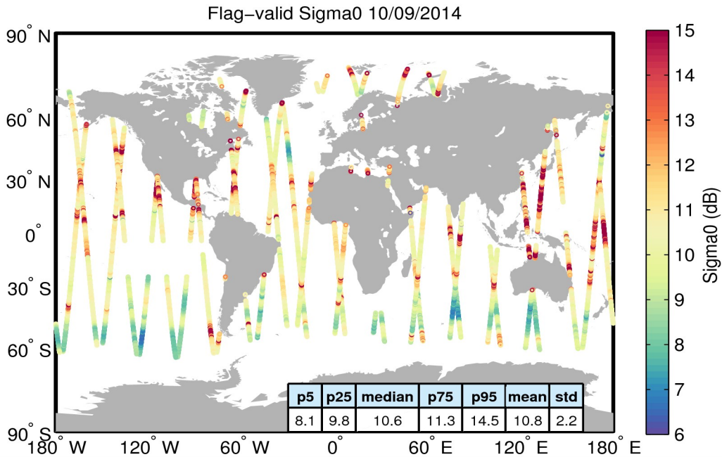
Figure 23. Geographical distribution of flag-valid sigma0 data over oceans and lakes for 10/09/2014. The statistical values shown in the table refer to the sigma0 in dB and are calculated over all measurements shown in the figure.
