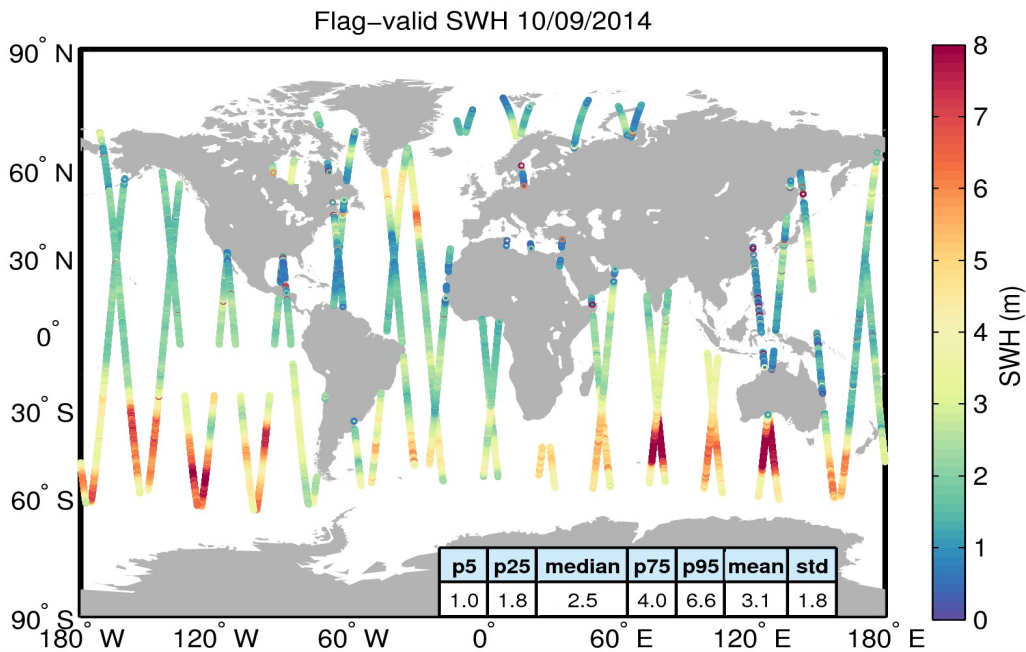
Figure 15. Geographical distribution of flag-valid SWH data over oceans and lakes for 10/09/2014. The statistical values shown in the table refer to the SWH in m and are calculated over all measurements shown in the figure.
