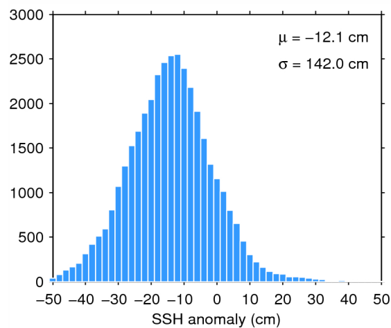
Figure 7. Histogram of flag-valid SSH anomaly over oceans and lakes for 10/09/2014. The mean ( \mu ) and standard deviation ( \sigma ) are also shown. Note that values outside [-50 50] cm are excluded from the histogram for the sake of readability but not from the computation of \mu and \sigma .
