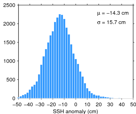
Figure 11. Histogram of science-valid SSH anomaly over oceans and lakes for 10/09/2014. The mean ( \mu ) and standard deviation ( \sigma ) are also shown. Note that values outside [-50 50] cm are excluded from the histogram for the sake of readability but not from the computation of \mu and \sigma .
