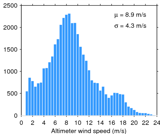
Figure 35. Histogram of science-valid wind over oceans and lakes for 10/09/2014. The mean ( \mu ) and standard deviation ( \sigma ) are also shown. Note that values larger than 24 m/s are excluded from the histogram for the sake of readability but not from the computation of \mu and \sigma .
