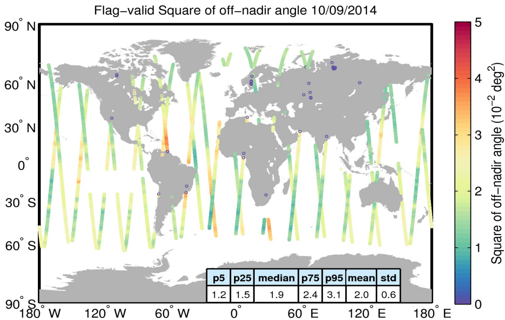
Figure 37. Geographical distribution of flag-valid mispointing data over oceans and lakes for 10/09/2014. The statistical values shown in the table refer to the mispointing in 10^{-2} \text{ deg}^2 and are calculated over all measurements shown in the figure.
