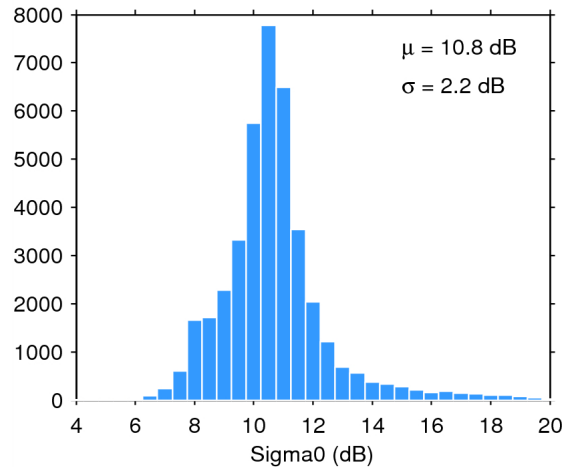
Figure 25. Histogram of flag-valid sigma0 over oceans and lakes for 10/09/2014. The mean ( \mu ) and standard deviation ( \sigma ) are also shown. Note that values outside [4 20] dB are excluded from the histogram for the sake of readability but not from the computation of \mu and \sigma .
