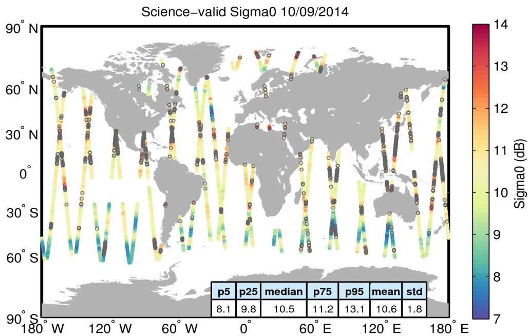
Figure 27. Geographical distribution of science-valid sigma0 data over oceans and lakes for 10/09/2014. The statistical values shown in the table refer to the sigma0 in dB and are calculated over all measurements shown in the figure. Gray circles denote records that have been rejected based on the editing criteria described in Table 4.
