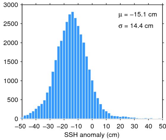
Figure 11. Histogram of science-valid SSH anomaly over oceans and lakes for 09/09/2014. The mean ( \mu ) and standard deviation ( \sigma ) are also shown. Note that values outside [-50 50] cm are excluded from the histogram for the sake of readability but not from the computation of \mu and \sigma .
