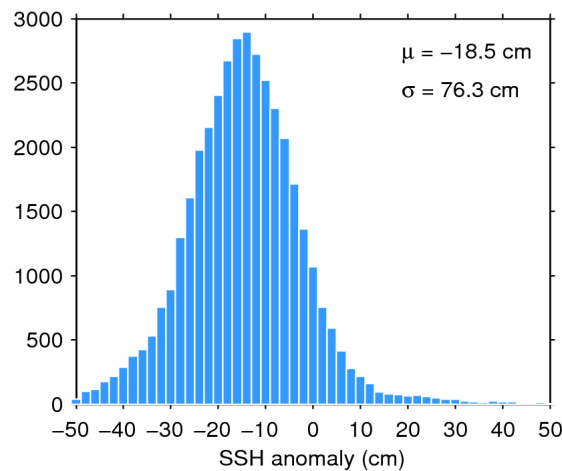
Figure 7. Histogram of flag-valid SSH anomaly over oceans and lakes for 09/09/2014. The mean ( \mu ) and standard deviation ( \sigma ) are also shown. Note that values outside [-50\ 50] cm are excluded from the histogram for the sake of readability but not from the computation of \mu and \sigma .
