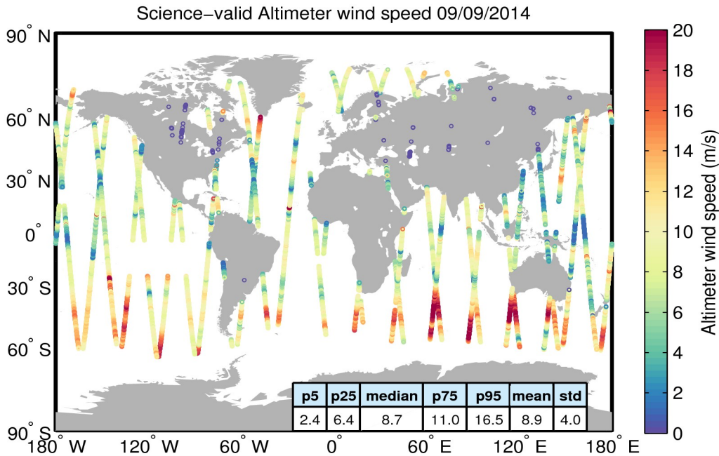
Figure 34. Geographical distribution of science-valid wind data over oceans and lakes for 09/09/2014. The statistical values shown in the table refer to the wind in m/s and are calculated over all measurements shown in the figure. Gray circles denote records that have been rejected based on the editing criteria described in Table 5.
