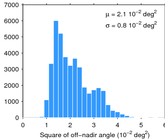
Figure 39. Histogram of flag-valid mispointing over oceans and lakes for 09/09/2014. The mean ( \mu ) and standard deviation ( \sigma ) are also shown. Note that values than 6 \cdot 10^{-2} \text{ deg}^2 are excluded from the histogram for the sake of readability but not from the computation of \mu and \sigma .
