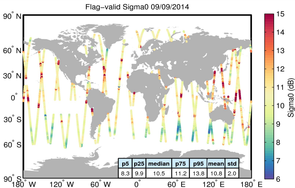
Figure 23. Geographical distribution of flag-valid sigma0 data over oceans and lakes for 09/09/2014. The statistical values shown in the table refer to the sigma0 in dB and are calculated over all measurements shown in the figure.
