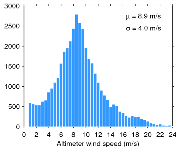
Figure 35. Histogram of science-valid wind over oceans and lakes for 09/09/2014. The mean ( \mu ) and standard deviation ( \sigma ) are also shown. Note that values larger than 24 m/s are excluded from the histogram for the sake of readability but not from the computation of \mu and \sigma .
