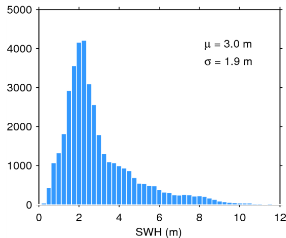
Figure 17. Histogram of flag-valid SWH over oceans and lakes for 09/09/2014. The mean ( \mu ) and standard deviation ( \sigma ) are also shown. Note that values larger than 12 m are excluded from the histogram for the sake of readability but not from the computation of \mu and \sigma .
