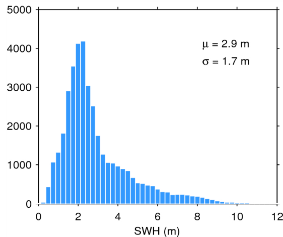
Figure 20. Histogram of science-valid SWH over oceans and lakes for 09/09/2014. The mean ( \mu ) and standard deviation ( \sigma ) are also shown. Note that values larger than 12 m are excluded from the histogram for the sake of readability but not from the computation of \mu and \sigma .
