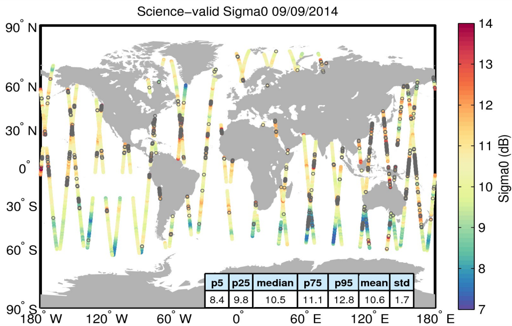
Figure 27. Geographical distribution of science-valid sigma0 data over oceans and lakes for 09/09/2014. The statistical values shown in the table refer to the sigma0 in dB and are calculated over all measurements shown in the figure. Gray circles denote records that have been rejected based on the editing criteria described in Table 4.
