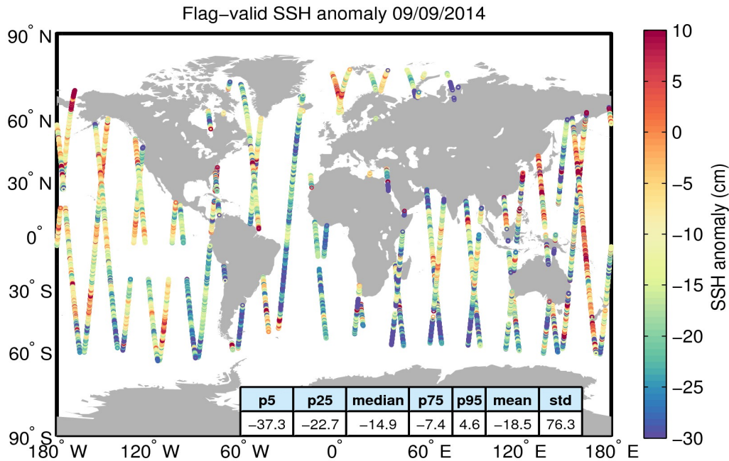
Figure 5. Geographical distribution of flag-valid 1-Hz SSH anomaly data over oceans and lakes for 09/09/2014. The statistical values shown in the table refer to the SSH anomaly in cm and are calculated over all measurements shown in the figure.
