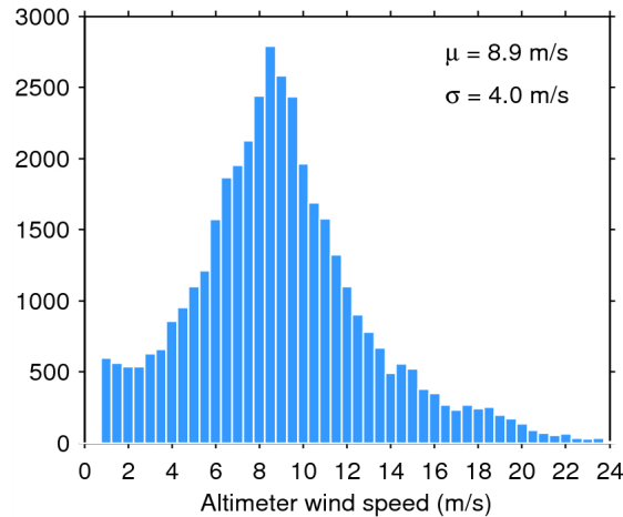
Figure 33. Histogram of flag-valid wind over oceans and lakes for 09/09/2014. The mean ( \mu ) and standard deviation ( \sigma ) are also shown. Note that values larger than 24 m/s are excluded from the histogram for the sake of readability but not from the computation of \mu and \sigma .
