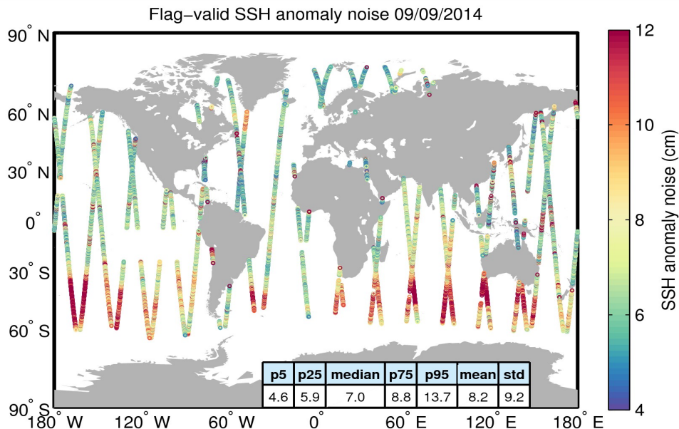
Figure 8. Geographical distribution of flag-valid 20-Hz SSH anomaly measurement noise over oceans and lakes for 09/09/2014. The statistical values shown in the table refer to the SSH anomaly noise and are calculated over all measurements shown in the figure.
