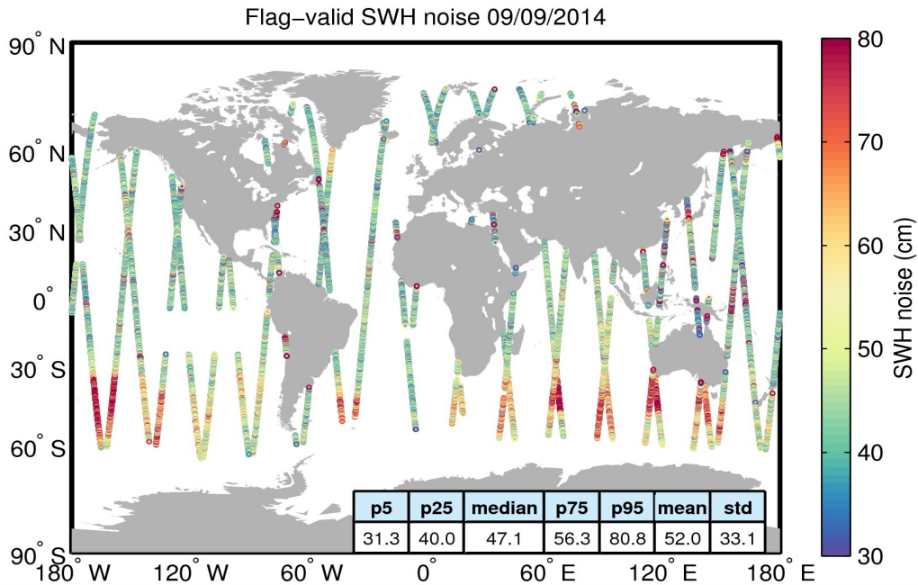
Figure 18. Geographical distribution of flag-valid 20-Hz SWH measurement noise over oceans and lakes for 09/09/2014. The statistical values shown in the figure refer to the SWH noise and are calculated over all measurements shown in the figure.
