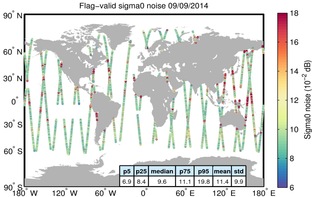
Figure 26. Geographical distribution of flag-valid 20-Hz sigma0 measurement noise over oceans and lakes for 09/09/2014. The statistical values shown in the table refer to the sigma0 noise and are calculated over all measurements shown in the figure.
