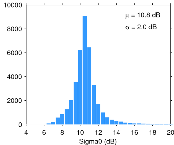
Figure 25. Histogram of flag-valid sigma0 over oceans and lakes for 09/09/2014. The mean ( \mu ) and standard deviation ( \sigma ) are also shown. Note that values outside [4 20] dB are excluded from the histogram for the sake of readability but not from the computation of \mu and \sigma .
