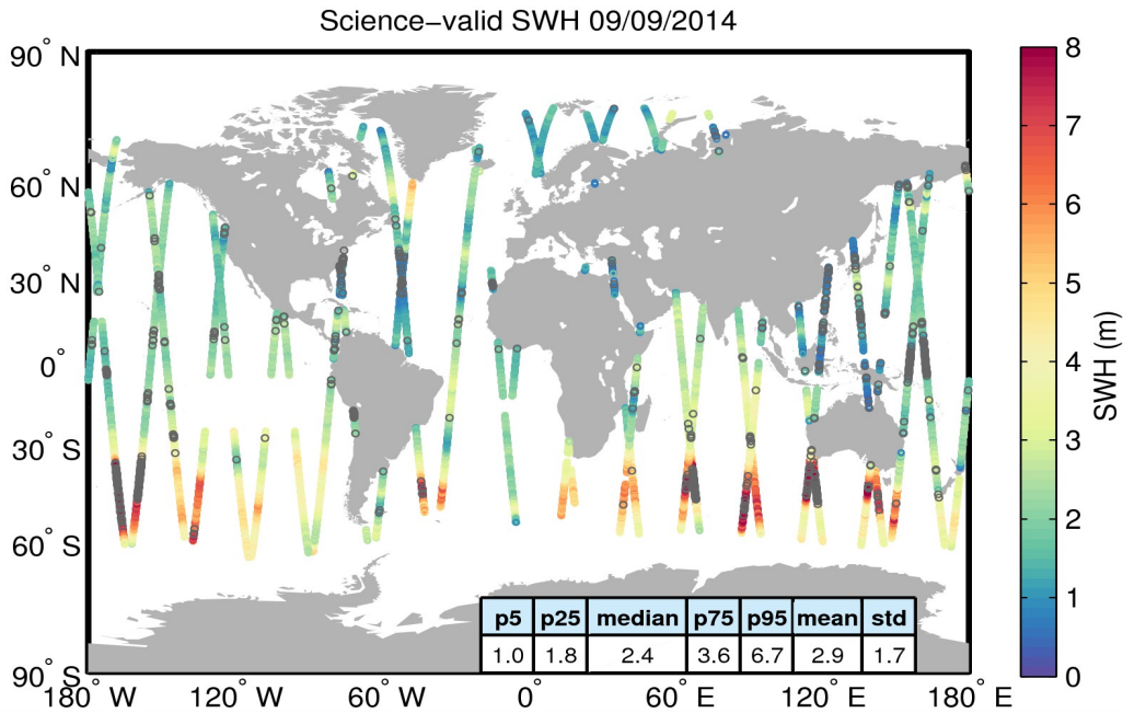
Figure 19. Geographical distribution of science-valid SWH data over oceans and lakes for 09/09/2014. The statistical values shown in the table refer to the SWH in m and are calculated over all measurements shown in the figure. Gray circles denote records that have been rejected based on the editing criteria described in Table 3.
