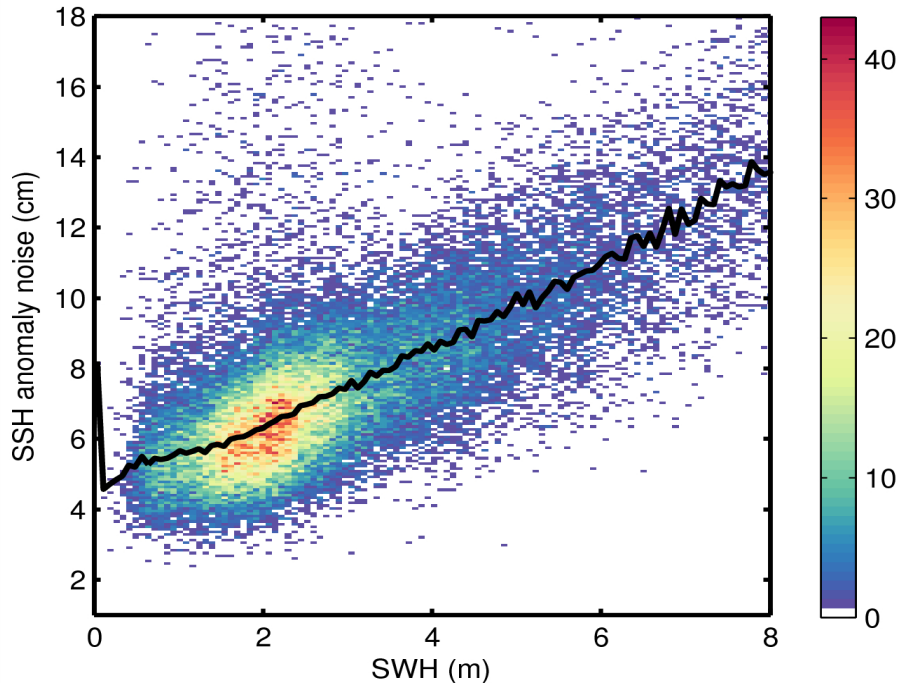
Figure 9. 2D histogram showing flag-valid SSH anomaly noise as a function of SWH for 09/09/2014. The black line denotes the median SSH anomaly as a function of SWH.
