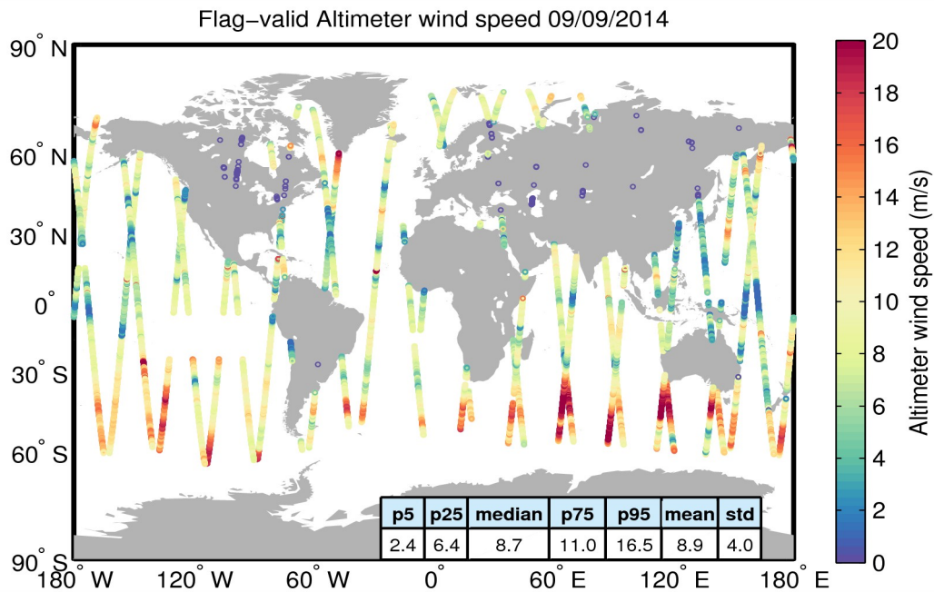
Figure 31. Geographical distribution of flag-valid wind data over oceans and lakes for 09/09/2014. The statistical values shown in the table refer to the wind in m/s and are calculated over all measurements shown in the figure.
