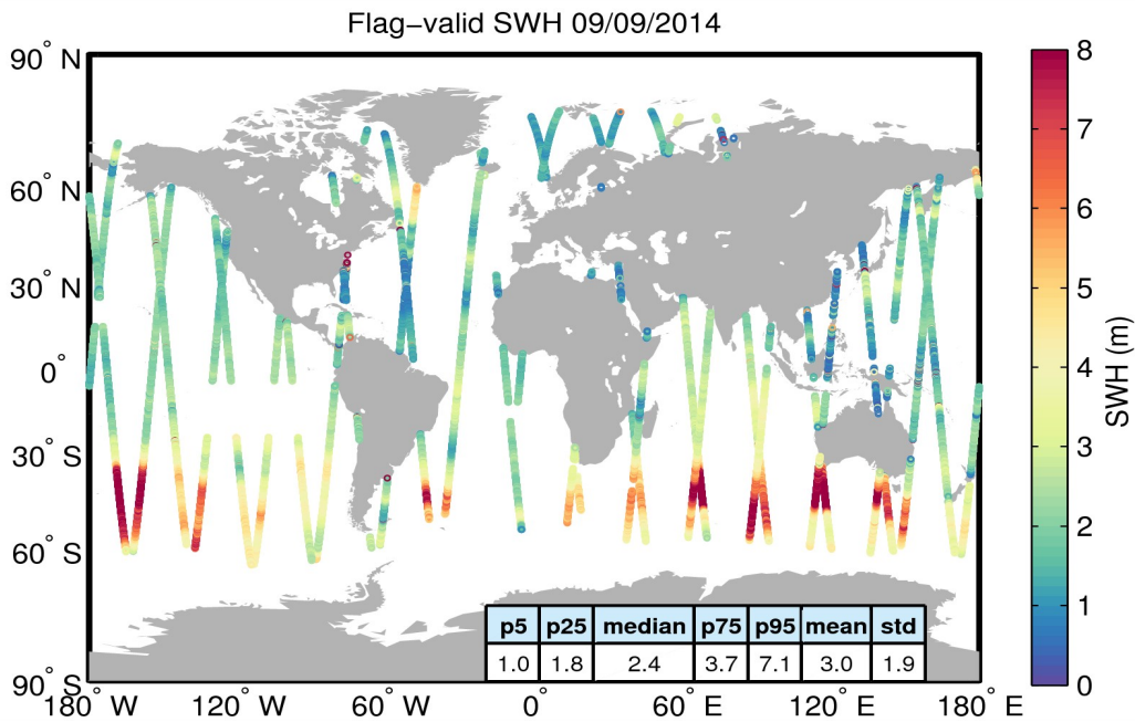
Figure 15. Geographical distribution of flag-valid SWH data over oceans and lakes for 09/09/2014. The statistical values shown in the table refer to the SWH in m and are calculated over all measurements shown in the figure.
