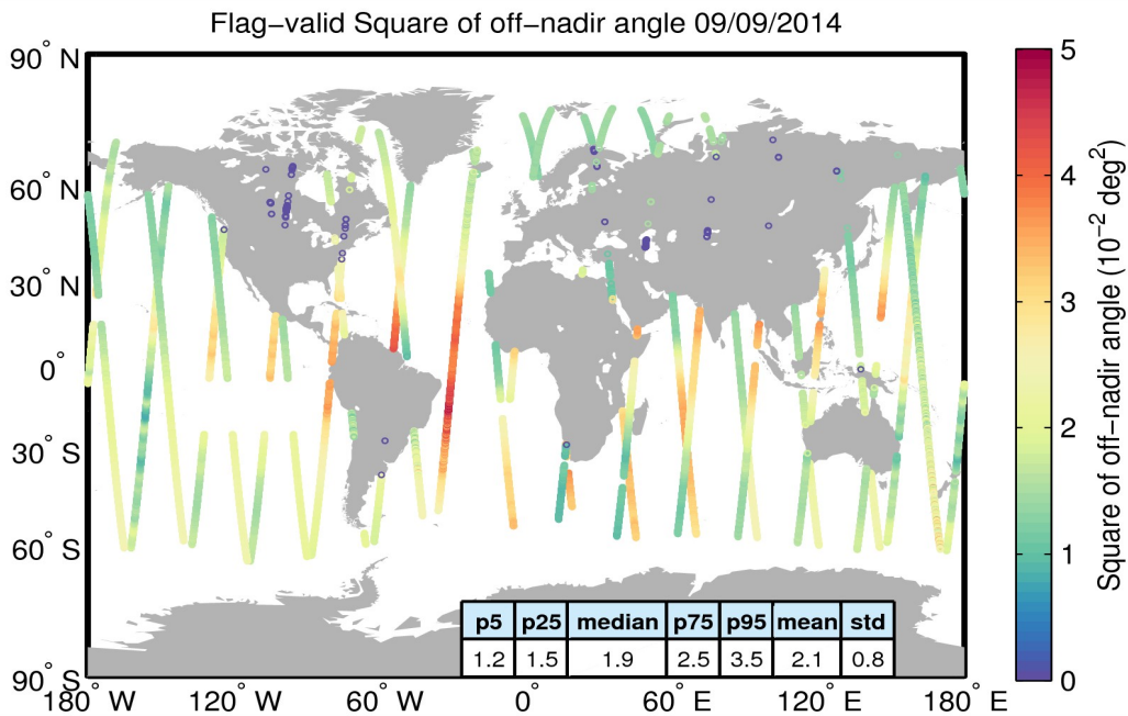
Figure 37. Geographical distribution of flag-valid mispointing data over oceans and lakes for 09/09/2014. The statistical values shown in the table refer to the mispointing in 10^{-2} \text{ deg}^2 and are calculated over all measurements shown in the figure.
