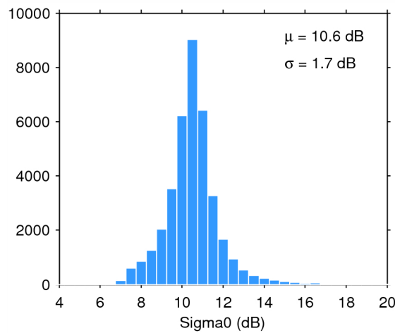
Figure 28. Histogram of science-valid sigma0 over oceans and lakes for 09/09/2014. The mean ( \mu ) and standard deviation ( \sigma ) are also shown. Note that values outside [4 20] dB are excluded from the histogram for the sake of readability but not from the computation of \mu and \sigma .
