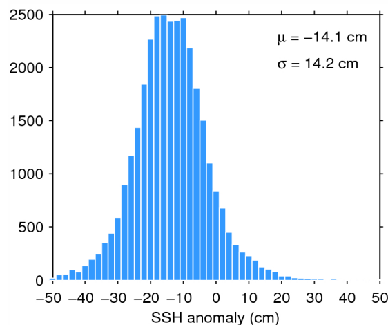
Figure 11. Histogram of science-valid SSH anomaly over oceans and lakes for 08/09/2014. The mean ( \mu ) and standard deviation ( \sigma ) are also shown. Note that values outside [-50 50] cm are excluded from the histogram for the sake of readability but not from the computation of \mu and \sigma .
