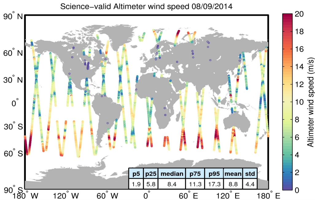
Figure 34. Geographical distribution of science-valid wind data over oceans and lakes for 08/09/2014. The statistical values shown in the table refer to the wind in m/s and are calculated over all measurements shown in the figure. Gray circles denote records that have been rejected based on the editing criteria described in Table 5.
