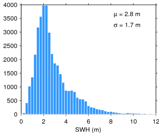
Figure 20. Histogram of science-valid SWH over oceans and lakes for 08/09/2014. The mean ( \mu ) and standard deviation ( \sigma ) are also shown. Note that values larger than 12 m are excluded from the histogram for the sake of readability but not from the computation of \mu and \sigma .
