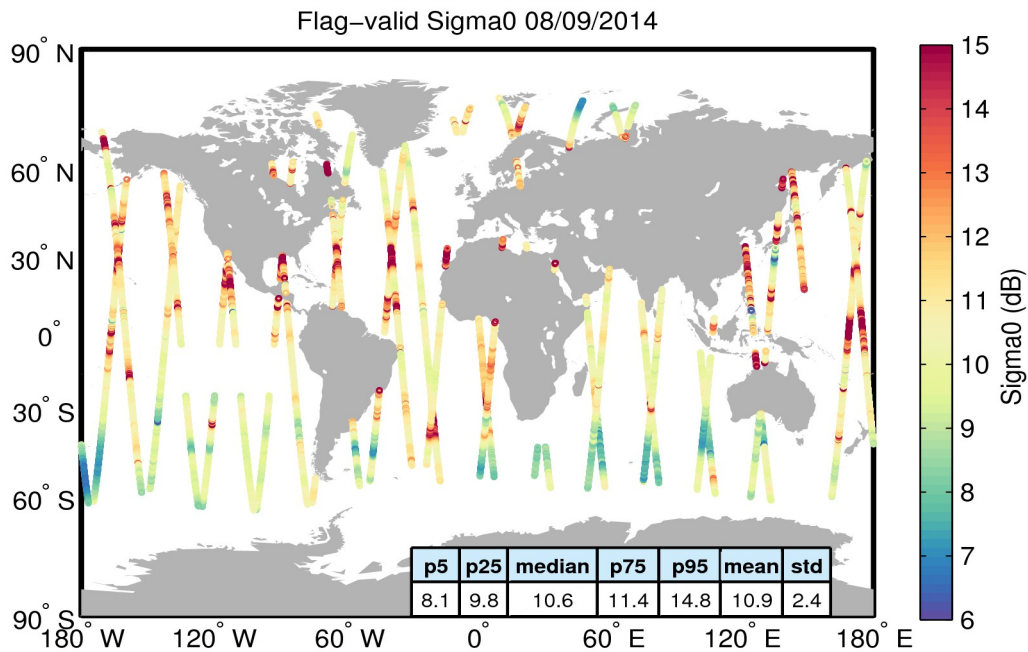
Figure 23. Geographical distribution of flag-valid sigma0 data over oceans and lakes for 08/09/2014. The statistical values shown in the table refer to the sigma0 in dB and are calculated over all measurements shown in the figure.
