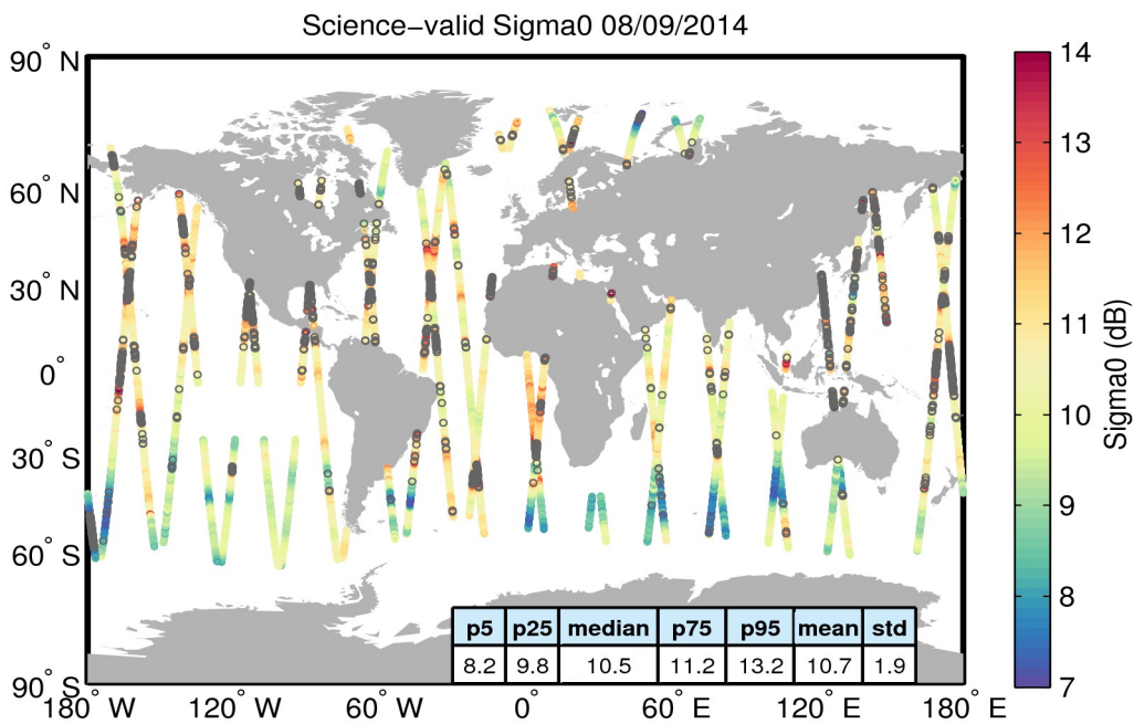
Figure 27. Geographical distribution of science-valid sigma0 data over oceans and lakes for 08/09/2014. The statistical values shown in the table refer to the sigma0 in dB and are calculated over all measurements shown in the figure. Gray circles denote records that have been rejected based on the editing criteria described in Table 4.
