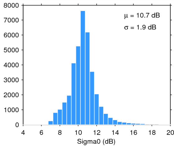
Figure 28. Histogram of science-valid sigma0 over oceans and lakes for 08/09/2014. The mean ( \mu ) and standard deviation ( \sigma ) are also shown. Note that values outside [4 20] dB are excluded from the histogram for the sake of readability but not from the computation of \mu and \sigma .
