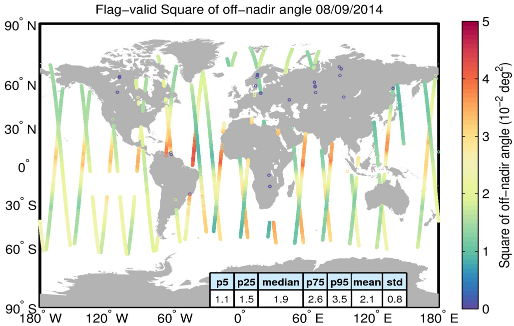
Figure 37. Geographical distribution of flag-valid mispointing data over oceans and lakes for 08/09/2014. The statistical values shown in the table refer to the mispointing in 10^{-2} \text{ deg}^2 and are calculated over all measurements shown in the figure.
