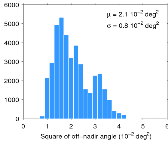
Figure 39. Histogram of flag-valid mispointing over oceans and lakes for 08/09/2014. The mean ( \mu ) and standard deviation ( \sigma ) are also shown. Note that values than 6 \cdot 10^{-2} \text{ deg}^2 are excluded from the histogram for the sake of readability but not from the computation of \mu and \sigma .
