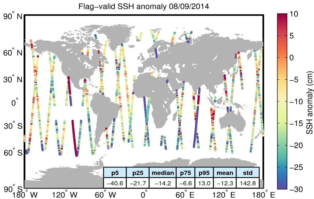
Figure 5. Geographical distribution of flag-valid 1-Hz SSH anomaly data over oceans and lakes for 08/09/2014. The statistical values shown in the table refer to the SSH anomaly in cm and are calculated over all measurements shown in the figure.
