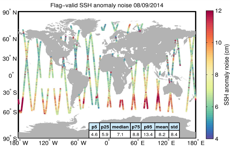
Figure 8. Geographical distribution of flag-valid 20-Hz SSH anomaly measurement noise over oceans and lakes for 08/09/2014. The statistical values shown in the table refer to the SSH anomaly noise and are calculated over all measurements shown in the figure.
