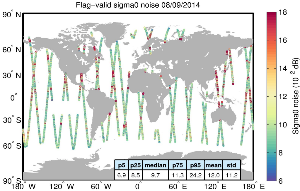
Figure 26. Geographical distribution of flag-valid 20-Hz sigma0 measurement noise over oceans and lakes for 08/09/2014. The statistical values shown in the table refer to the sigma0 noise and are calculated over all measurements shown in the figure.
