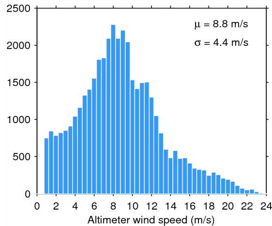
Figure 33. Histogram of flag-valid wind over oceans and lakes for 08/09/2014. The mean ( \mu ) and standard deviation ( \sigma ) are also shown. Note that values larger than 24 m/s are excluded from the histogram for the sake of readability but not from the computation of \mu and \sigma .
