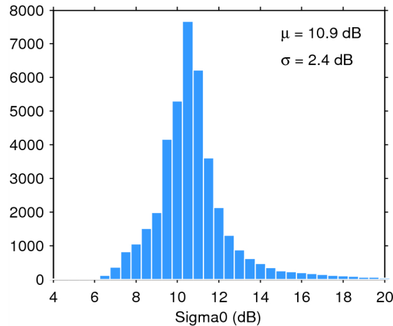
Figure 25. Histogram of flag-valid sigma0 over oceans and lakes for 08/09/2014. The mean ( \mu ) and standard deviation ( \sigma ) are also shown. Note that values outside [4 20] dB are excluded from the histogram for the sake of readability but not from the computation of \mu and \sigma .
