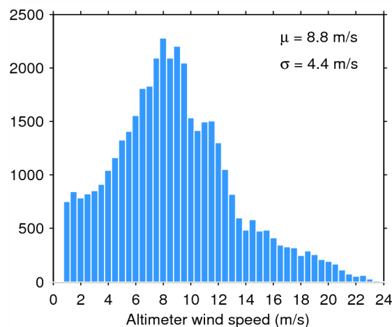
Figure 35. Histogram of science-valid wind over oceans and lakes for 08/09/2014. The mean ( \mu ) and standard deviation ( \sigma ) are also shown. Note that values larger than 24 m/s are excluded from the histogram for the sake of readability but not from the computation of \mu and \sigma .
