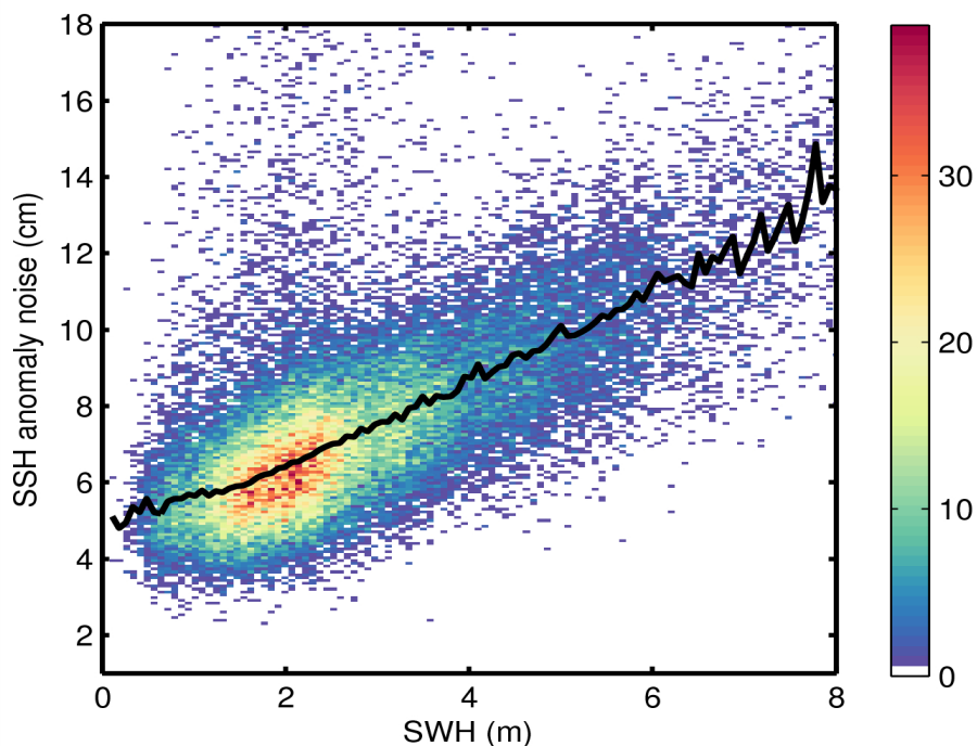
Figure 9. 2D histogram showing flag-valid SSH anomaly noise as a function of SWH for 08/09/2014. The black line denotes the median SSH anomaly as a function of SWH.
