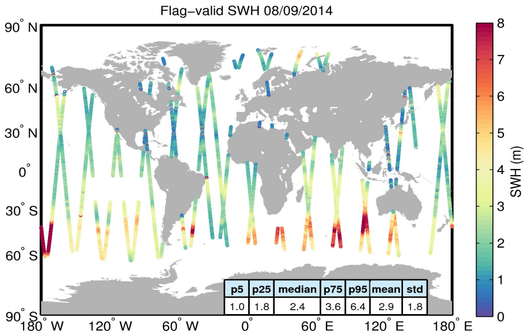
Figure 15. Geographical distribution of flag-valid SWH data over oceans and lakes for 08/09/2014. The statistical values shown in the table refer to the SWH in m and are calculated over all measurements shown in the figure.
