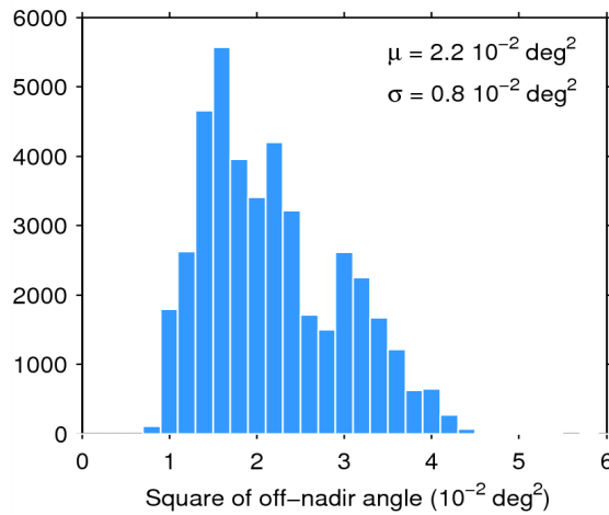
Figure 39. Histogram of flag-valid mispointing over oceans and lakes for 06/09/2014. The mean ( \mu ) and standard deviation ( \sigma ) are also shown. Note that values than 6 \cdot 10^{-2} \text{ deg}^2 are excluded from the histogram for the sake of readability but not from the computation of \mu and \sigma .
