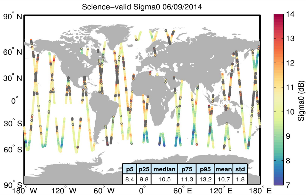
Figure 27. Geographical distribution of science-valid sigma0 data over oceans and lakes for 06/09/2014. The statistical values shown in the table refer to the sigma0 in dB and are calculated over all measurements shown in the figure. Gray circles denote records that have been rejected based on the editing criteria described in Table 4.
