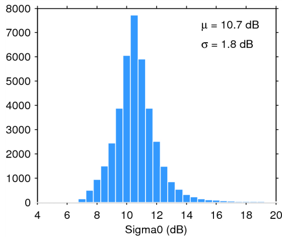
Figure 28. Histogram of science-valid sigma0 over oceans and lakes for 06/09/2014. The mean ( \mu ) and standard deviation ( \sigma ) are also shown. Note that values outside [4 20] dB are excluded from the histogram for the sake of readability but not from the computation of \mu and \sigma .
