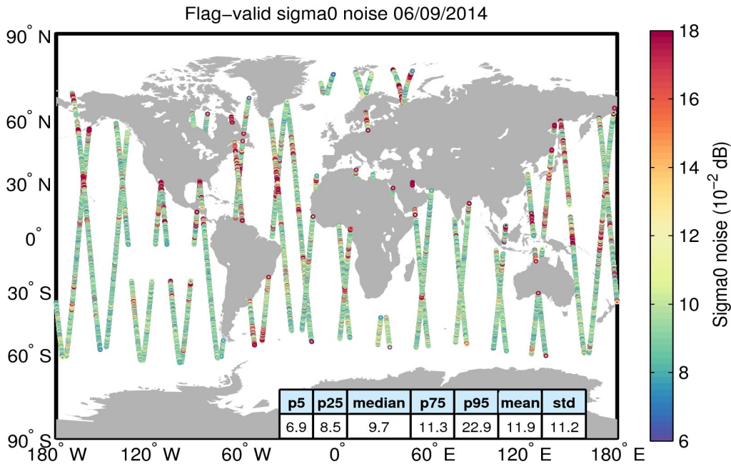
Figure 26. Geographical distribution of flag-valid 20-Hz sigma0 measurement noise over oceans and lakes for 06/09/2014. The statistical values shown in the table refer to the sigma0 noise and are calculated over all measurements shown in the figure.
