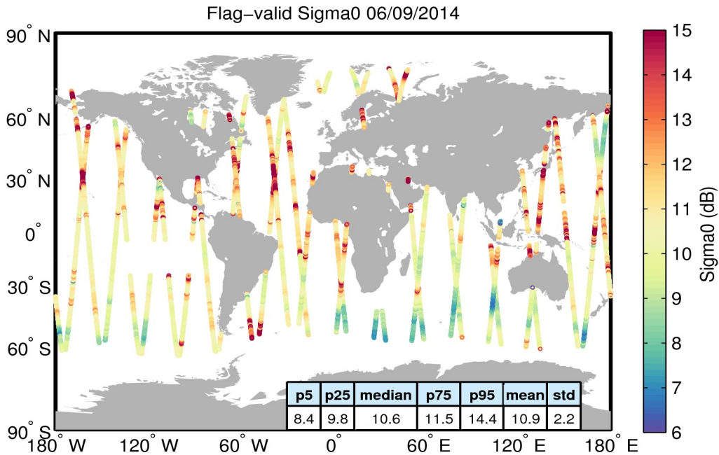
Figure 23. Geographical distribution of flag-valid sigma0 data over oceans and lakes for 06/09/2014. The statistical values shown in the table refer to the sigma0 in dB and are calculated over all measurements shown in the figure.
