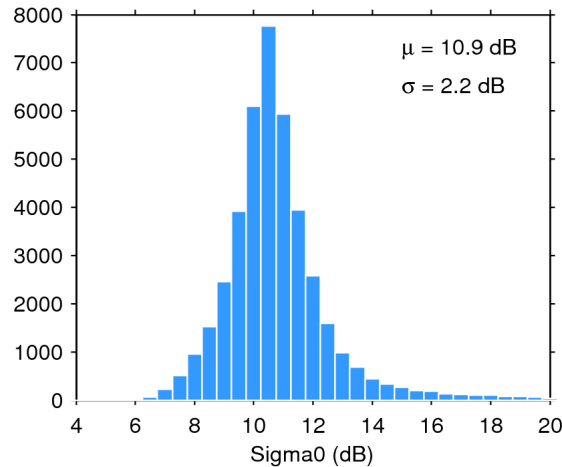
Figure 25. Histogram of flag-valid sigma0 over oceans and lakes for 06/09/2014. The mean ( \mu ) and standard deviation ( \sigma ) are also shown. Note that values outside [4 20] dB are excluded from the histogram for the sake of readability but not from the computation of \mu and \sigma .
