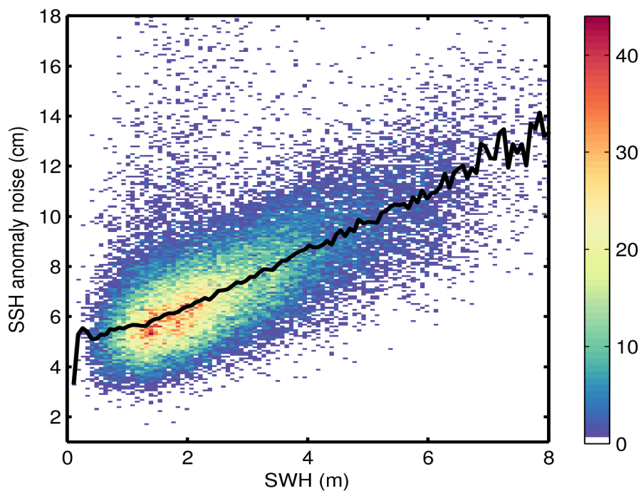
Figure 9. 2D histogram showing flag-valid SSH anomaly noise as a function of SWH for 06/09/2014. The black line denotes the median SSH anomaly as a function of SWH.
