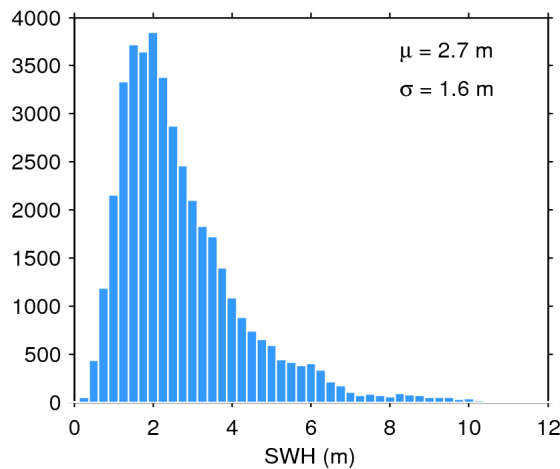
Figure 17. Histogram of flag-valid SWH over oceans and lakes for 06/09/2014. The mean ( \mu ) and standard deviation ( \sigma ) are also shown. Note that values larger than 12 m are excluded from the histogram for the sake of readability but not from the computation of \mu and \sigma .
