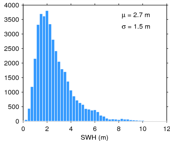
Figure 20. Histogram of science-valid SWH over oceans and lakes for 06/09/2014. The mean ( \mu ) and standard deviation ( \sigma ) are also shown. Note that values larger than 12 m are excluded from the histogram for the sake of readability but not from the computation of \mu and \sigma .
