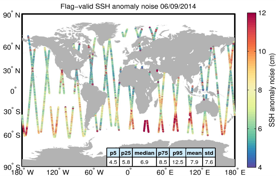
Figure 8. Geographical distribution of flag-valid 20-Hz SSH anomaly measurement noise over oceans and lakes for 06/09/2014. The statistical values shown in the table refer to the SSH anomaly noise and are calculated over all measurements shown in the figure.
