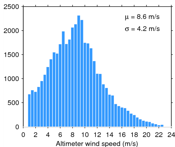
Figure 35. Histogram of science-valid wind over oceans and lakes for 06/09/2014. The mean ( \mu ) and standard deviation ( \sigma ) are also shown. Note that values larger than 24 m/s are excluded from the histogram for the sake of readability but not from the computation of \mu and \sigma .
