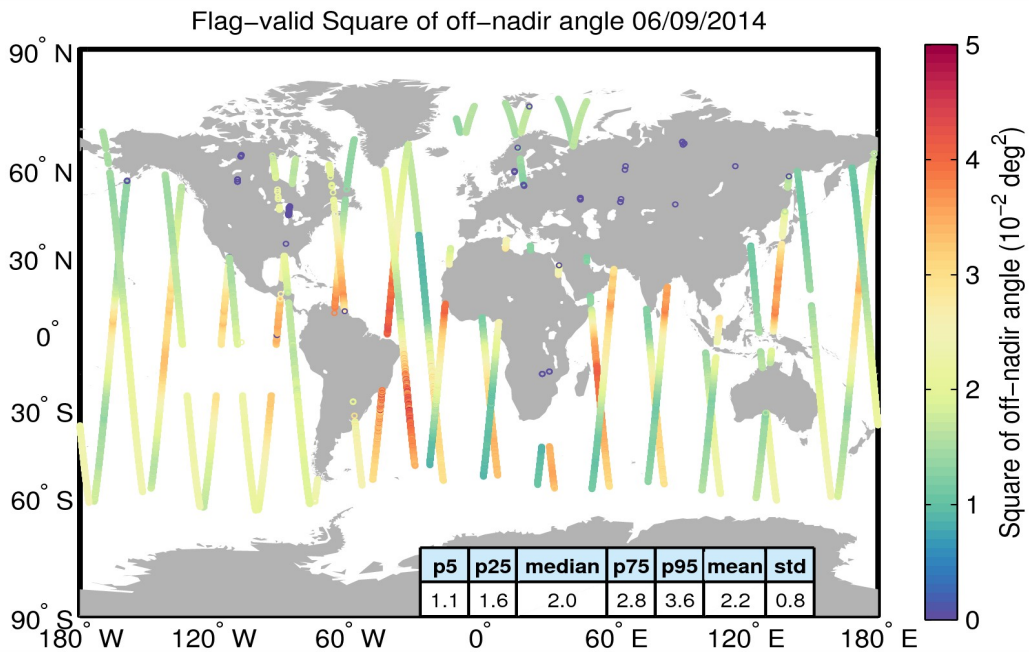
Figure 37. Geographical distribution of flag-valid mispointing data over oceans and lakes for 06/09/2014. The statistical values shown in the table refer to the mispointing in 10^{-2} \text{ deg}^2 and are calculated over all measurements shown in the figure.
