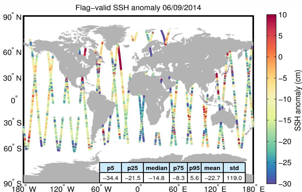
Figure 5. Geographical distribution of flag-valid 1-Hz SSH anomaly data over oceans and lakes for 06/09/2014. The statistical values shown in the table refer to the SSH anomaly in cm and are calculated over all measurements shown in the figure.
