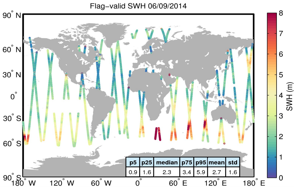
Figure 15. Geographical distribution of flag-valid SWH data over oceans and lakes for 06/09/2014. The statistical values shown in the table refer to the SWH in m and are calculated over all measurements shown in the figure.
