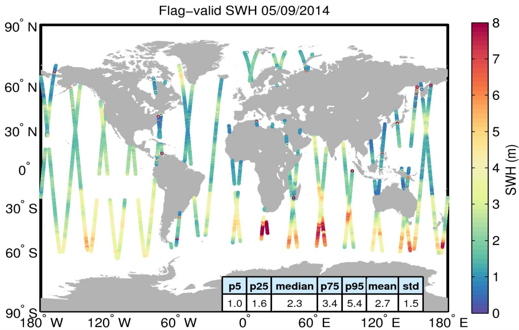
Figure 15. Geographical distribution of flag-valid SWH data over oceans and lakes for 05/09/2014. The statistical values shown in the table refer to the SWH in m and are calculated over all measurements shown in the figure.
