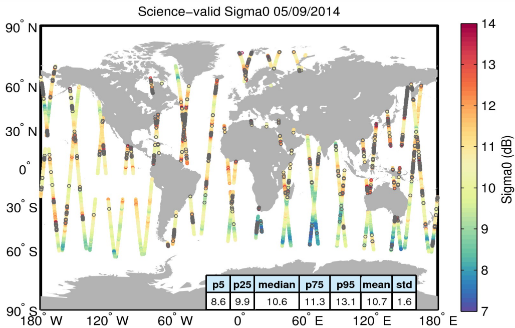
Figure 27. Geographical distribution of science-valid sigma0 data over oceans and lakes for 05/09/2014. The statistical values shown in the table refer to the sigma0 in dB and are calculated over all measurements shown in the figure. Gray circles denote records that have been rejected based on the editing criteria described in Table 4.
