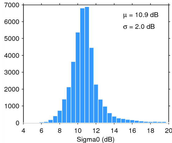
Figure 25. Histogram of flag-valid sigma0 over oceans and lakes for 05/09/2014. The mean ( \mu ) and standard deviation ( \sigma ) are also shown. Note that values outside [4 20] dB are excluded from the histogram for the sake of readability but not from the computation of \mu and \sigma .
