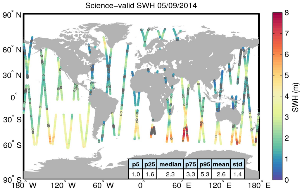
Figure 19. Geographical distribution of science-valid SWH data over oceans and lakes for 05/09/2014. The statistical values shown in the table refer to the SWH in m and are calculated over all measurements shown in the figure. Gray circles denote records that have been rejected based on the editing criteria described in Table 3.
