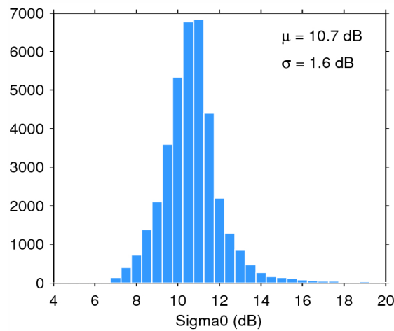
Figure 28. Histogram of science-valid sigma0 over oceans and lakes for 05/09/2014. The mean ( \mu ) and standard deviation ( \sigma ) are also shown. Note that values outside [4 20] dB are excluded from the histogram for the sake of readability but not from the computation of \mu and \sigma .
