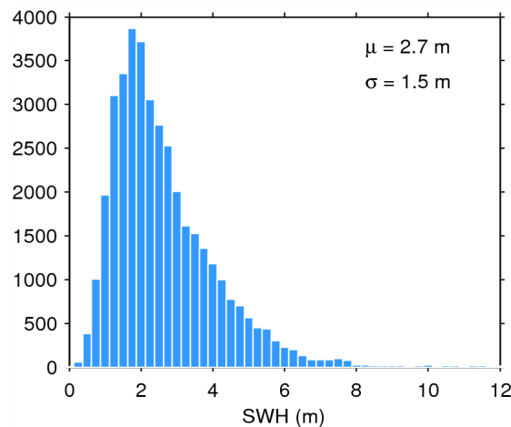
Figure 17. Histogram of flag-valid SWH over oceans and lakes for 05/09/2014. The mean ( \mu ) and standard deviation ( \sigma ) are also shown. Note that values larger than 12 m are excluded from the histogram for the sake of readability but not from the computation of \mu and \sigma .
