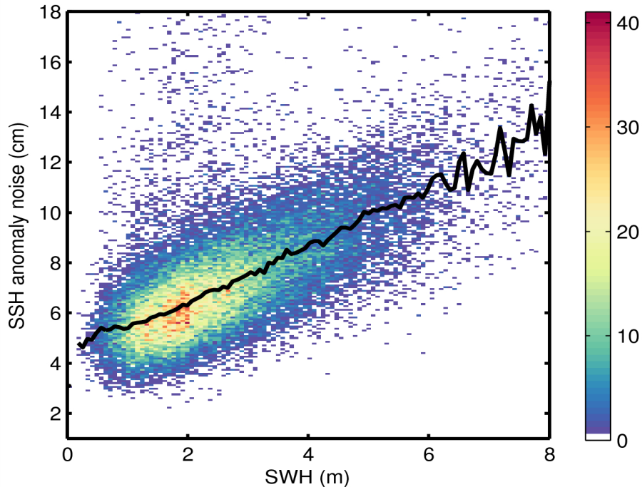
Figure 9. 2D histogram showing flag-valid SSH anomaly noise as a function of SWH for 05/09/2014. The black line denotes the median SSH anomaly as a function of SWH.
