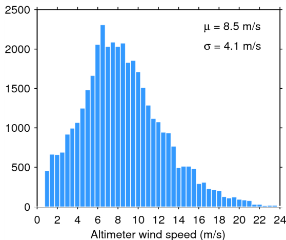
Figure 33. Histogram of flag-valid wind over oceans and lakes for 05/09/2014. The mean ( \mu ) and standard deviation ( \sigma ) are also shown. Note that values larger than 24 m/s are excluded from the histogram for the sake of readability but not from the computation of \mu and \sigma .
