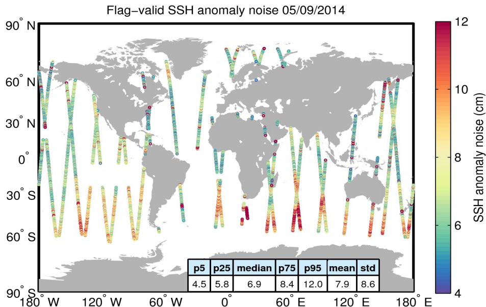
Figure 8. Geographical distribution of flag-valid 20-Hz SSH anomaly measurement noise over oceans and lakes for 05/09/2014. The statistical values shown in the table refer to the SSH anomaly noise and are calculated over all measurements shown in the figure.
