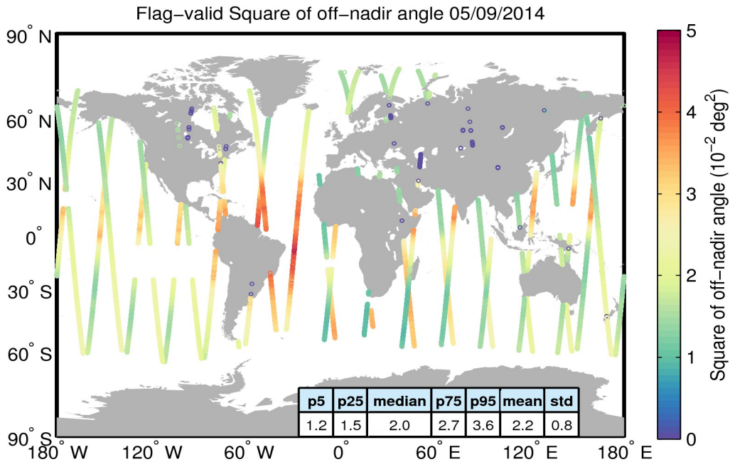
Figure 37. Geographical distribution of flag-valid mispointing data over oceans and lakes for 05/09/2014. The statistical values shown in the table refer to the mispointing in 10^{-2} \text{ deg}^2 and are calculated over all measurements shown in the figure.
