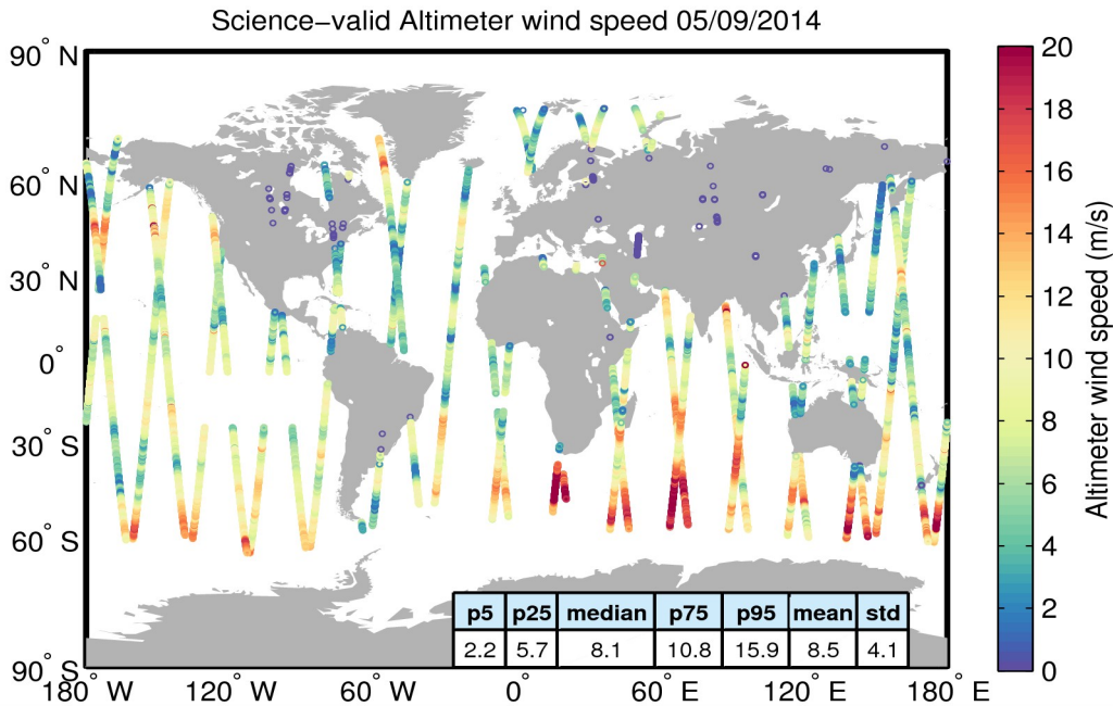
Figure 34. Geographical distribution of science-valid wind data over oceans and lakes for 05/09/2014. The statistical values shown in the table refer to the wind in m/s and are calculated over all measurements shown in the figure. Gray circles denote records that have been rejected based on the editing criteria described in Table 5.
