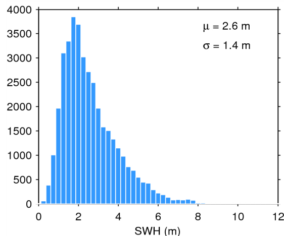
Figure 20. Histogram of science-valid SWH over oceans and lakes for 05/09/2014. The mean ( \mu ) and standard deviation ( \sigma ) are also shown. Note that values larger than 12 m are excluded from the histogram for the sake of readability but not from the computation of \mu and \sigma .
