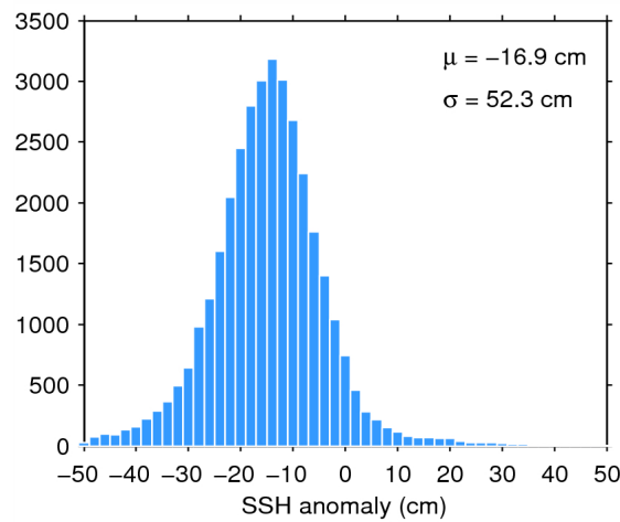
Figure 7. Histogram of flag-valid SSH anomaly over oceans and lakes for 05/09/2014. The mean ( \mu ) and standard deviation ( \sigma ) are also shown. Note that values outside [-50\ 50] cm are excluded from the histogram for the sake of readability but not from the computation of \mu and \sigma .
