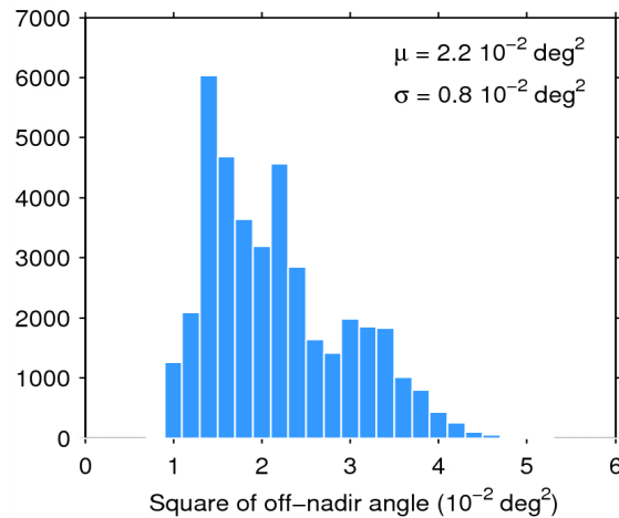
Figure 39. Histogram of flag-valid mispointing over oceans and lakes for 05/09/2014. The mean ( \mu ) and standard deviation ( \sigma ) are also shown. Note that values than 6 \cdot 10^{-2} \text{ deg}^2 are excluded from the histogram for the sake of readability but not from the computation of \mu and \sigma .
