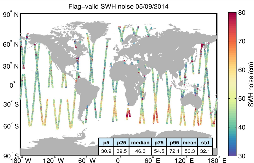
Figure 18. Geographical distribution of flag-valid 20-Hz SWH measurement noise over oceans and lakes for 05/09/2014. The statistical values shown in the figure refer to the SWH noise and are calculated over all measurements shown in the figure.
