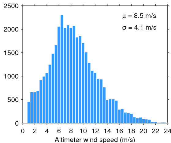
Figure 35. Histogram of science-valid wind over oceans and lakes for 05/09/2014. The mean ( \mu ) and standard deviation ( \sigma ) are also shown. Note that values larger than 24 m/s are excluded from the histogram for the sake of readability but not from the computation of \mu and \sigma .
