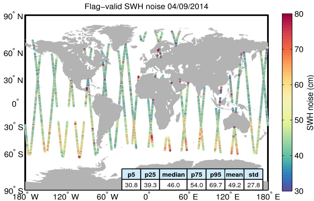
Figure 18. Geographical distribution of flag-valid 20-Hz SWH measurement noise over oceans and lakes for 04/09/2014. The statistical values shown in the figure refer to the SWH noise and are calculated over all measurements shown in the figure.
