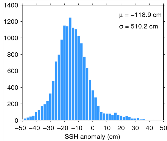
Figure 7. Histogram of flag-valid SSH anomaly over oceans and lakes for 04/09/2014. The mean ( \mu ) and standard deviation ( \sigma ) are also shown. Note that values outside [-50\ 50] cm are excluded from the histogram for the sake of readability but not from the computation of \mu and \sigma .
