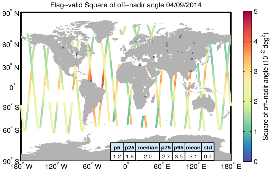
Figure 37. Geographical distribution of flag-valid mispointing data over oceans and lakes for 04/09/2014. The statistical values shown in the table refer to the mispointing in 10^{-2} \text{ deg}^2 and are calculated over all measurements shown in the figure.
