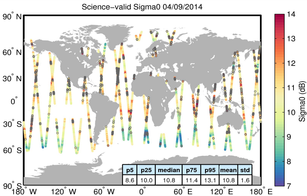
Figure 27. Geographical distribution of science-valid sigma0 data over oceans and lakes for 04/09/2014. The statistical values shown in the table refer to the sigma0 in dB and are calculated over all measurements shown in the figure. Gray circles denote records that have been rejected based on the editing criteria described in Table 4.
