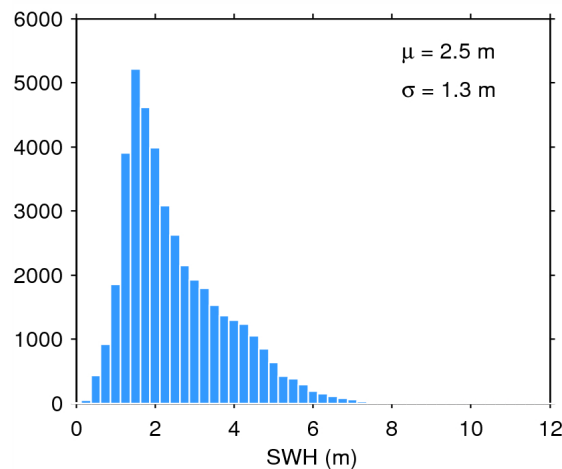
Figure 17. Histogram of flag-valid SWH over oceans and lakes for 04/09/2014. The mean ( \mu ) and standard deviation ( \sigma ) are also shown. Note that values larger than 12 m are excluded from the histogram for the sake of readability but not from the computation of \mu and \sigma .
