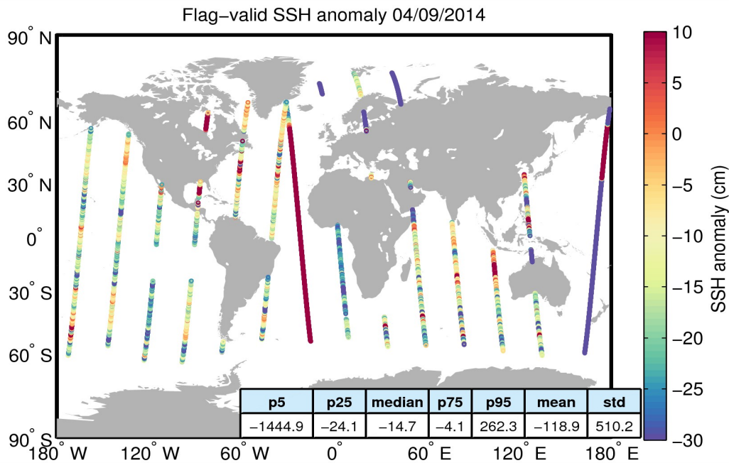
Figure 5. Geographical distribution of flag-valid 1-Hz SSH anomaly data over oceans and lakes for 04/09/2014. The statistical values shown in the table refer to the SSH anomaly in cm and are calculated over all measurements shown in the figure.
