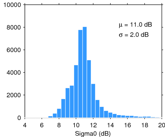
Figure 25. Histogram of flag-valid sigma0 over oceans and lakes for 04/09/2014. The mean ( \mu ) and standard deviation ( \sigma ) are also shown. Note that values outside [4 20] dB are excluded from the histogram for the sake of readability but not from the computation of \mu and \sigma .
