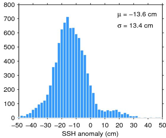
Figure 11. Histogram of science-valid SSH anomaly over oceans and lakes for 04/09/2014. The mean ( \mu ) and standard deviation ( \sigma ) are also shown. Note that values outside [-50 50] cm are excluded from the histogram for the sake of readability but not from the computation of \mu and \sigma .
