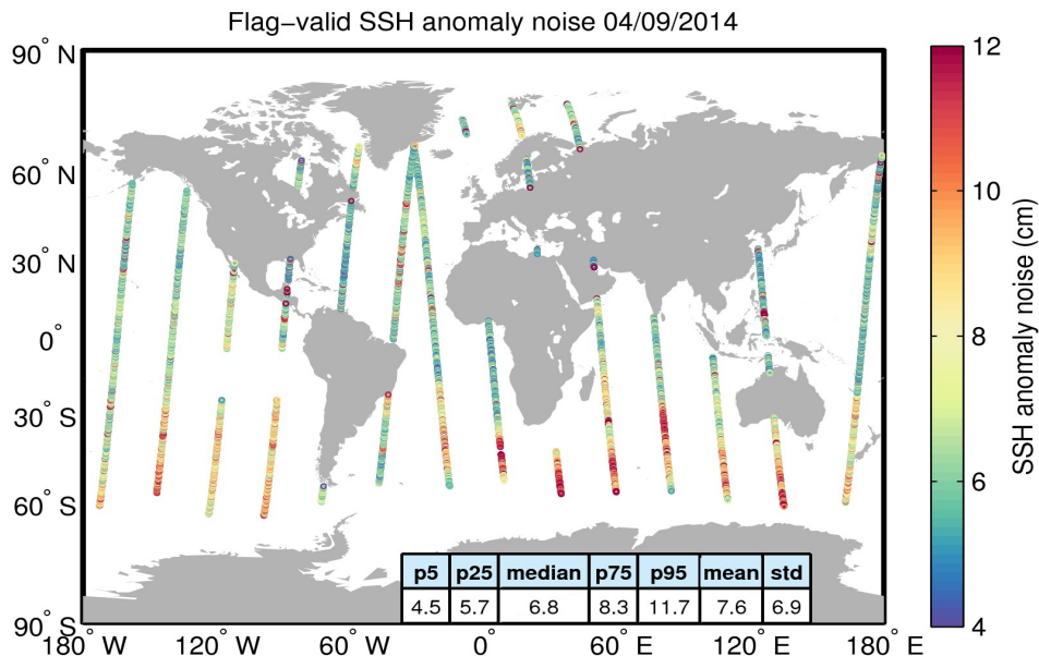
Figure 8. Geographical distribution of flag-valid 20-Hz SSH anomaly measurement noise over oceans and lakes for 04/09/2014. The statistical values shown in the table refer to the SSH anomaly noise and are calculated over all measurements shown in the figure.
