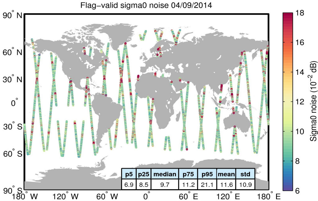
Figure 26. Geographical distribution of flag-valid 20-Hz sigma0 measurement noise over oceans and lakes for 04/09/2014. The statistical values shown in the table refer to the sigma0 noise and are calculated over all measurements shown in the figure.
