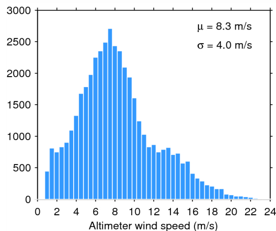
Figure 35. Histogram of science-valid wind over oceans and lakes for 04/09/2014. The mean ( \mu ) and standard deviation ( \sigma ) are also shown. Note that values larger than 24 m/s are excluded from the histogram for the sake of readability but not from the computation of \mu and \sigma .
