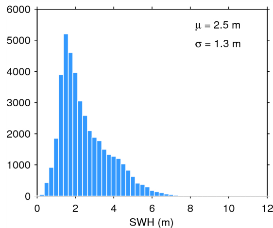
Figure 20. Histogram of science-valid SWH over oceans and lakes for 04/09/2014. The mean ( \mu ) and standard deviation ( \sigma ) are also shown. Note that values larger than 12 m are excluded from the histogram for the sake of readability but not from the computation of \mu and \sigma .
