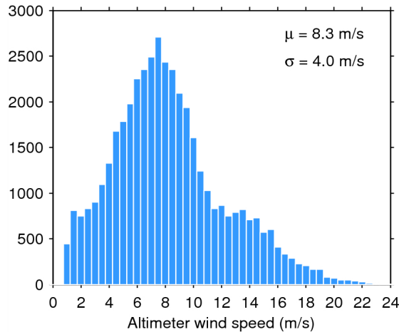
Figure 33. Histogram of flag-valid wind over oceans and lakes for 04/09/2014. The mean ( \mu ) and standard deviation ( \sigma ) are also shown. Note that values larger than 24 m/s are excluded from the histogram for the sake of readability but not from the computation of \mu and \sigma .
