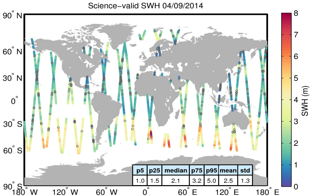
Figure 19. Geographical distribution of science-valid SWH data over oceans and lakes for 04/09/2014. The statistical values shown in the table refer to the SWH in m and are calculated over all measurements shown in the figure. Gray circles denote records that have been rejected based on the editing criteria described in Table 3.
