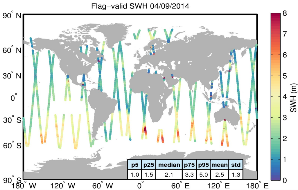
Figure 15. Geographical distribution of flag-valid SWH data over oceans and lakes for 04/09/2014. The statistical values shown in the table refer to the SWH in m and are calculated over all measurements shown in the figure.
