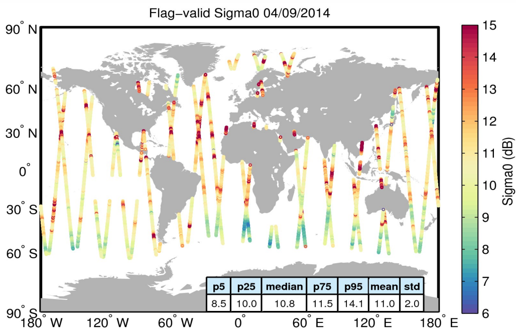
Figure 23. Geographical distribution of flag-valid sigma0 data over oceans and lakes for 04/09/2014. The statistical values shown in the table refer to the sigma0 in dB and are calculated over all measurements shown in the figure.
