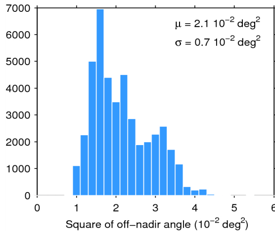
Figure 39. Histogram of flag-valid mispointing over oceans and lakes for 04/09/2014. The mean ( \mu ) and standard deviation ( \sigma ) are also shown. Note that values than 6 \cdot 10^{-2} \text{ deg}^2 are excluded from the histogram for the sake of readability but not from the computation of \mu and \sigma .
