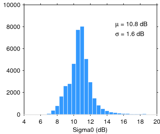
Figure 28. Histogram of science-valid sigma0 over oceans and lakes for 04/09/2014. The mean ( \mu ) and standard deviation ( \sigma ) are also shown. Note that values outside [4 20] dB are excluded from the histogram for the sake of readability but not from the computation of \mu and \sigma .
