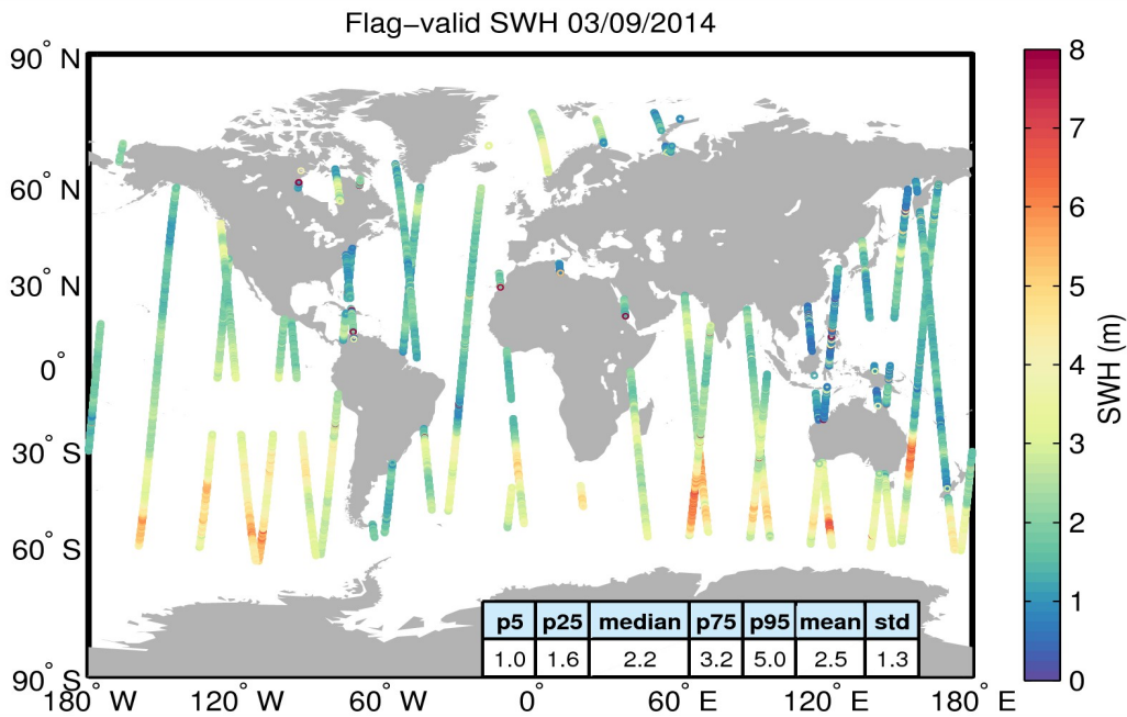
Figure 15. Geographical distribution of flag-valid SWH data over oceans and lakes for 03/09/2014. The statistical values shown in the table refer to the SWH in m and are calculated over all measurements shown in the figure.
