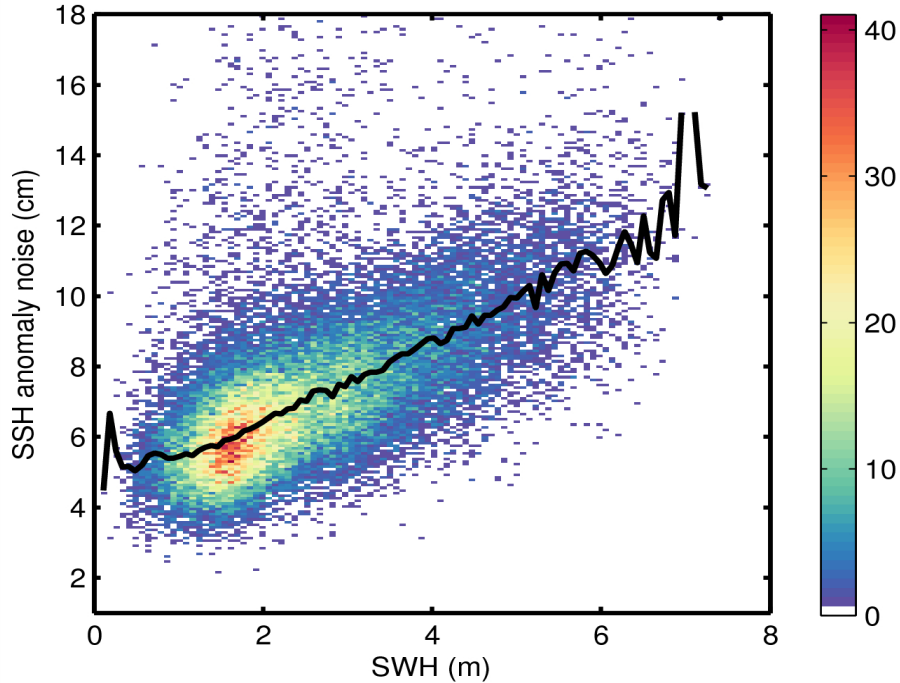
Figure 9. 2D histogram showing flag-valid SSH anomaly noise as a function of SWH for 03/09/2014. The black line denotes the median SSH anomaly as a function of SWH.
