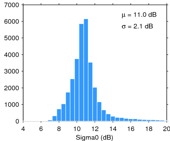
Figure 25. Histogram of flag-valid sigma0 over oceans and lakes for 03/09/2014. The mean ( \mu ) and standard deviation ( \sigma ) are also shown. Note that values outside [4 20] dB are excluded from the histogram for the sake of readability but not from the computation of \mu and \sigma .
