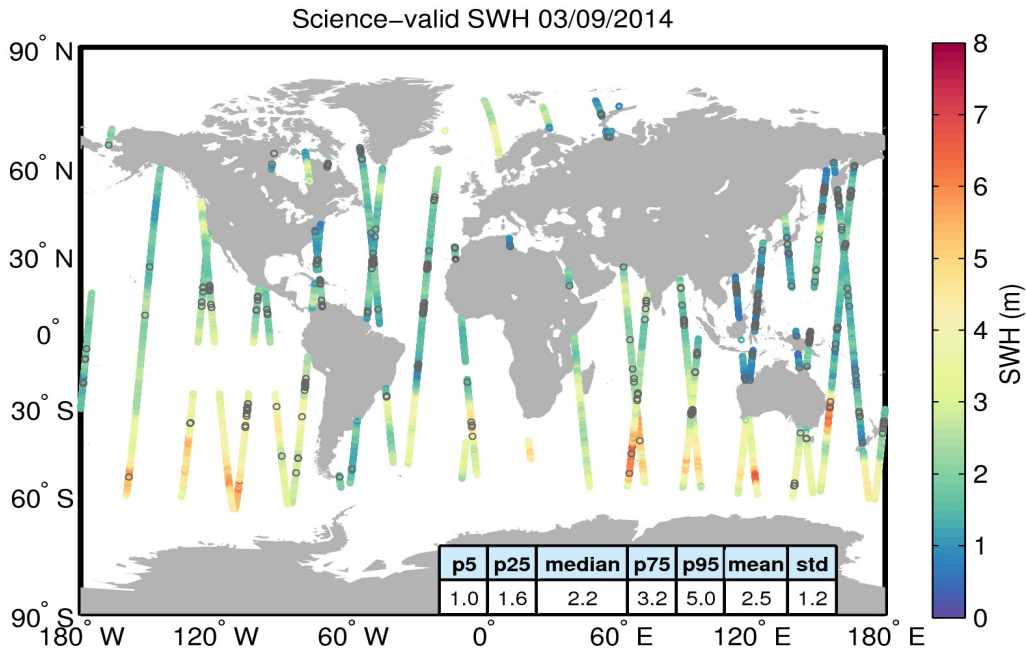
Figure 19. Geographical distribution of science-valid SWH data over oceans and lakes for 03/09/2014. The statistical values shown in the table refer to the SWH in m and are calculated over all measurements shown in the figure. Gray circles denote records that have been rejected based on the editing criteria described in Table 3.
