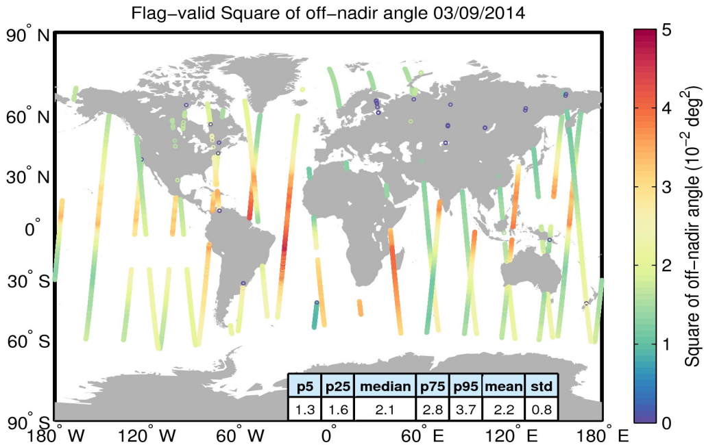
Figure 37. Geographical distribution of flag-valid mispointing data over oceans and lakes for 03/09/2014. The statistical values shown in the table refer to the mispointing in 10^{-2} \text{ deg}^2 and are calculated over all measurements shown in the figure.
