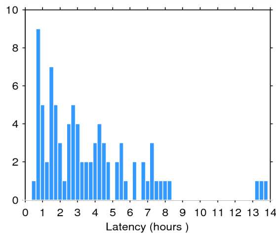
Figure 2. Histogram of the data latency for 03/09/2014. The y-axis denotes the number of files that are made available with a delay of x-hours with respect to the mean time of the records stored in the file.
