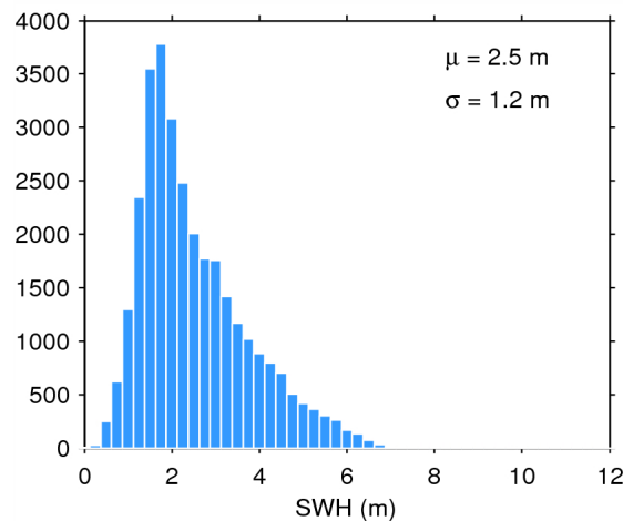
Figure 20. Histogram of science-valid SWH over oceans and lakes for 03/09/2014. The mean ( \mu ) and standard deviation ( \sigma ) are also shown. Note that values larger than 12 m are excluded from the histogram for the sake of readability but not from the computation of \mu and \sigma .
