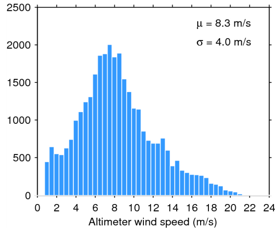
Figure 33. Histogram of flag-valid wind over oceans and lakes for 03/09/2014. The mean ( \mu ) and standard deviation ( \sigma ) are also shown. Note that values larger than 24 m/s are excluded from the histogram for the sake of readability but not from the computation of \mu and \sigma .
