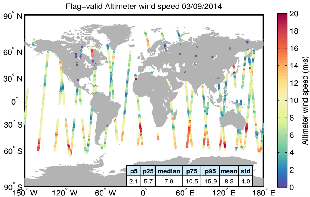
Figure 31. Geographical distribution of flag-valid wind data over oceans and lakes for 03/09/2014. The statistical values shown in the table refer to the wind in m/s and are calculated over all measurements shown in the figure.
