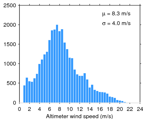
Figure 35. Histogram of science-valid wind over oceans and lakes for 03/09/2014. The mean ( \mu ) and standard deviation ( \sigma ) are also shown. Note that values larger than 24 m/s are excluded from the histogram for the sake of readability but not from the computation of \mu and \sigma .
