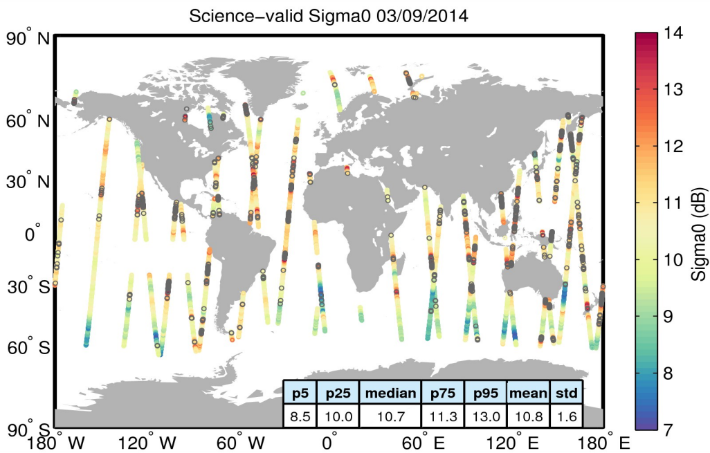
Figure 27. Geographical distribution of science-valid sigma0 data over oceans and lakes for 03/09/2014. The statistical values shown in the table refer to the sigma0 in dB and are calculated over all measurements shown in the figure. Gray circles denote records that have been rejected based on the editing criteria described in Table 4.
