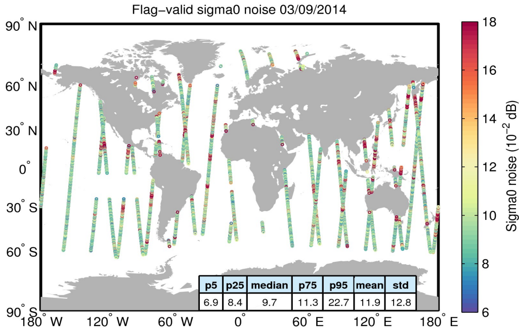
Figure 26. Geographical distribution of flag-valid 20-Hz sigma0 measurement noise over oceans and lakes for 03/09/2014. The statistical values shown in the table refer to the sigma0 noise and are calculated over all measurements shown in the figure.
