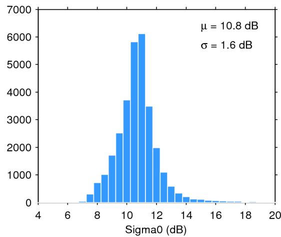
Figure 28. Histogram of science-valid sigma0 over oceans and lakes for 03/09/2014. The mean ( \mu ) and standard deviation ( \sigma ) are also shown. Note that values outside [4 20] dB are excluded from the histogram for the sake of readability but not from the computation of \mu and \sigma .
