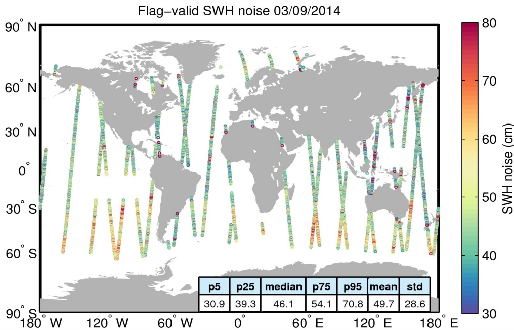
Figure 18. Geographical distribution of flag-valid 20-Hz SWH measurement noise over oceans and lakes for 03/09/2014. The statistical values shown in the figure refer to the SWH noise and are calculated over all measurements shown in the figure.
