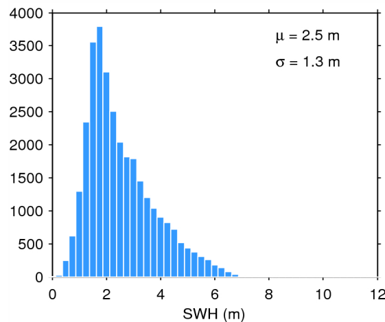
Figure 17. Histogram of flag-valid SWH over oceans and lakes for 03/09/2014. The mean ( \mu ) and standard deviation ( \sigma ) are also shown. Note that values larger than 12 m are excluded from the histogram for the sake of readability but not from the computation of \mu and \sigma .
