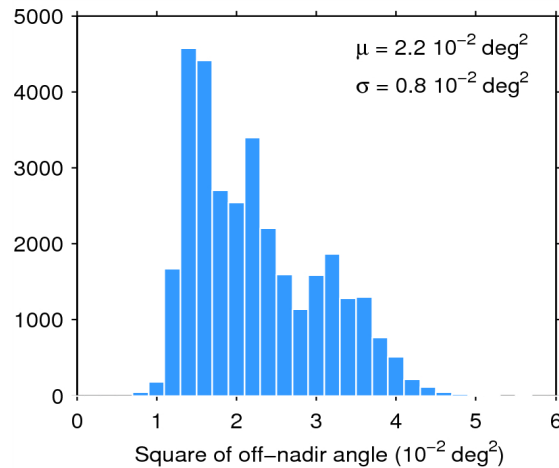
Figure 39. Histogram of flag-valid mispointing over oceans and lakes for 03/09/2014. The mean ( \mu ) and standard deviation ( \sigma ) are also shown. Note that values than 6 \cdot 10^{-2} \text{ deg}^2 are excluded from the histogram for the sake of readability but not from the computation of \mu and \sigma .
