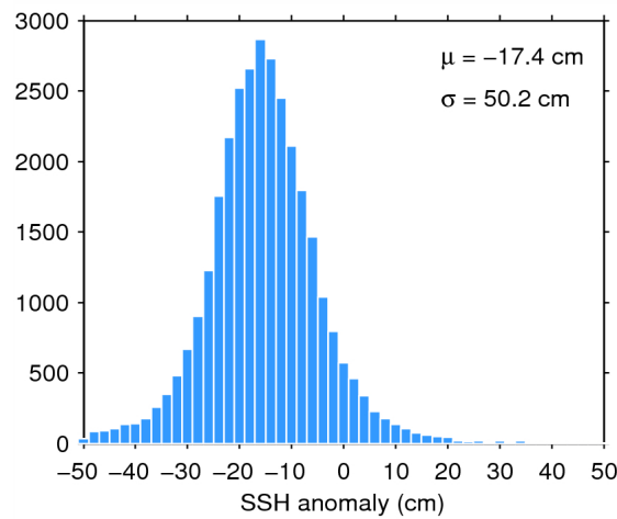
Figure 7. Histogram of flag-valid SSH anomaly over oceans and lakes for 03/09/2014. The mean ( \mu ) and standard deviation ( \sigma ) are also shown. Note that values outside [-50\ 50] cm are excluded from the histogram for the sake of readability but not from the computation of \mu and \sigma .
