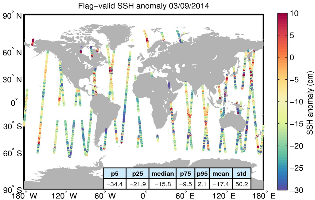
Figure 5. Geographical distribution of flag-valid 1-Hz SSH anomaly data over oceans and lakes for 03/09/2014. The statistical values shown in the table refer to the SSH anomaly in cm and are calculated over all measurements shown in the figure.
