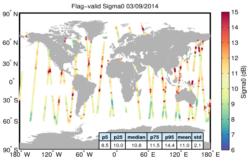
Figure 23. Geographical distribution of flag-valid sigma0 data over oceans and lakes for 03/09/2014. The statistical values shown in the table refer to the sigma0 in dB and are calculated over all measurements shown in the figure.
