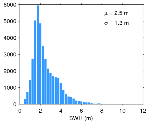
Figure 17. Histogram of flag-valid SWH over oceans and lakes for 02/09/2014. The mean ( \mu ) and standard deviation ( \sigma ) are also shown. Note that values larger than 12 m are excluded from the histogram for the sake of readability but not from the computation of \mu and \sigma .
