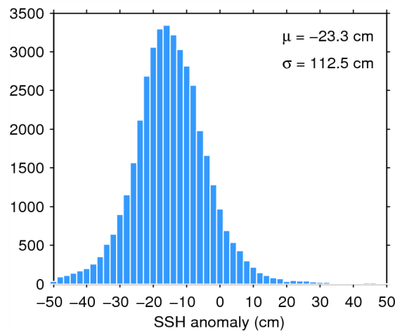
Figure 7. Histogram of flag-valid SSH anomaly over oceans and lakes for 02/09/2014. The mean ( \mu ) and standard deviation ( \sigma ) are also shown. Note that values outside [-50 50] cm are excluded from the histogram for the sake of readability but not from the computation of \mu and \sigma .
