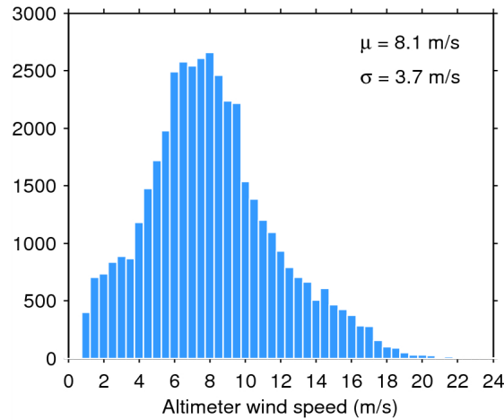
Figure 33. Histogram of flag-valid wind over oceans and lakes for 02/09/2014. The mean ( \mu ) and standard deviation ( \sigma ) are also shown. Note that values larger than 24 m/s are excluded from the histogram for the sake of readability but not from the computation of \mu and \sigma .
