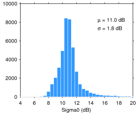
Figure 25. Histogram of flag-valid sigma0 over oceans and lakes for 02/09/2014. The mean ( \mu ) and standard deviation ( \sigma ) are also shown. Note that values outside [4 20] dB are excluded from the histogram for the sake of readability but not from the computation of \mu and \sigma .
