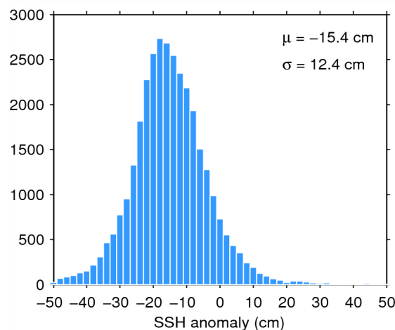
Figure 11. Histogram of science-valid SSH anomaly over oceans and lakes for 02/09/2014. The mean ( \mu ) and standard deviation ( \sigma ) are also shown. Note that values outside [-50 50] cm are excluded from the histogram for the sake of readability but not from the computation of \mu and \sigma .
