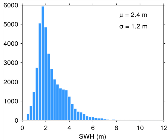
Figure 20. Histogram of science-valid SWH over oceans and lakes for 02/09/2014. The mean ( \mu ) and standard deviation ( \sigma ) are also shown. Note that values larger than 12 m are excluded from the histogram for the sake of readability but not from the computation of \mu and \sigma .
