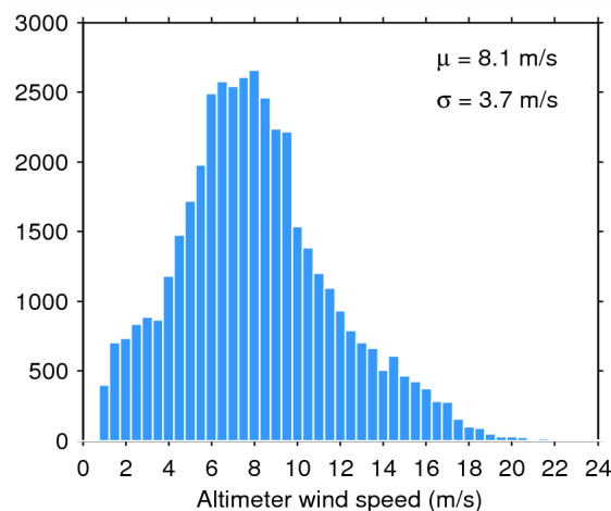
Figure 35. Histogram of science-valid wind over oceans and lakes for 02/09/2014. The mean ( \mu ) and standard deviation ( \sigma ) are also shown. Note that values larger than 24 m/s are excluded from the histogram for the sake of readability but not from the computation of \mu and \sigma .
