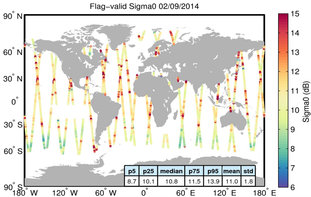
Figure 23. Geographical distribution of flag-valid sigma0 data over oceans and lakes for 02/09/2014. The statistical values shown in the table refer to the sigma0 in dB and are calculated over all measurements shown in the figure.
