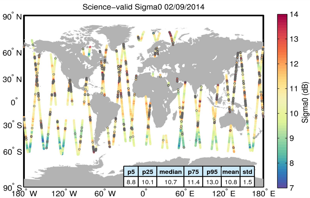
Figure 27. Geographical distribution of science-valid sigma0 data over oceans and lakes for 02/09/2014. The statistical values shown in the table refer to the sigma0 in dB and are calculated over all measurements shown in the figure. Gray circles denote records that have been rejected based on the editing criteria described in Table 4.
