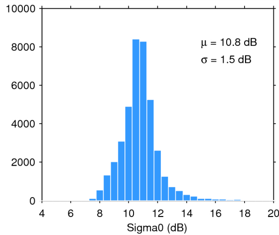
Figure 28. Histogram of science-valid sigma0 over oceans and lakes for 02/09/2014. The mean ( \mu ) and standard deviation ( \sigma ) are also shown. Note that values outside [4 20] dB are excluded from the histogram for the sake of readability but not from the computation of \mu and \sigma .
