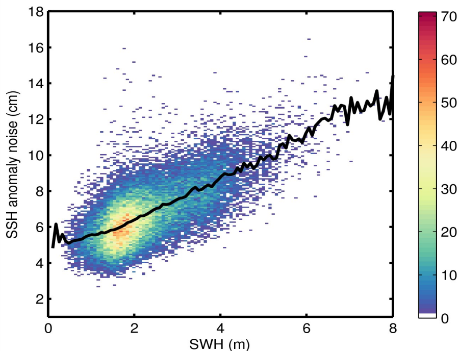
Figure 9. 2D histogram showing flag-valid SSH anomaly noise as a function of SWH for 02/09/2014. The black line denotes the median SSH anomaly as a function of SWH.
