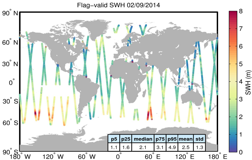
Figure 15. Geographical distribution of flag-valid SWH data over oceans and lakes for 02/09/2014. The statistical values shown in the figure refer to the SWH in m and are calculated over all measurements shown in the figure.
