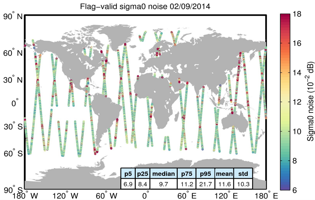
Figure 26. Geographical distribution of flag-valid 20-Hz sigma0 measurement noise over oceans and lakes for 02/09/2014. The statistical values shown in the table refer to the sigma0 noise and are calculated over all measurements shown in the figure.
