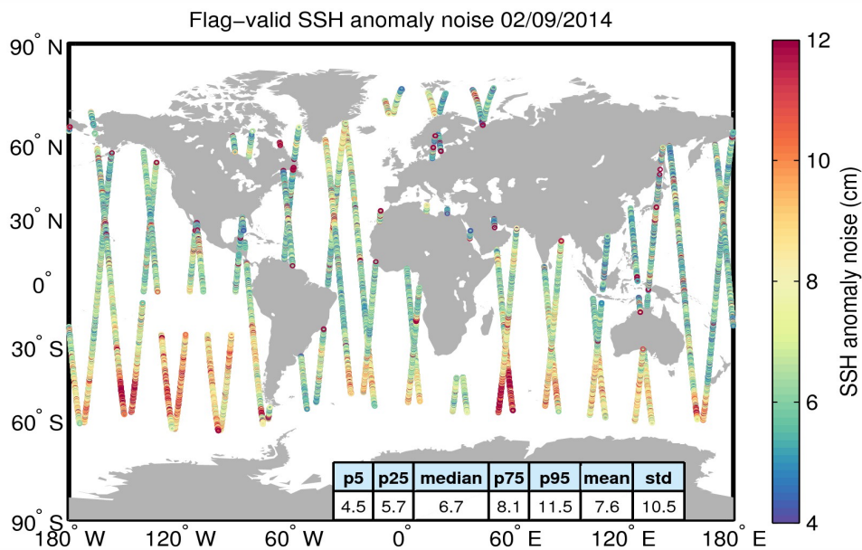
Figure 8. Geographical distribution of flag-valid 20-Hz SSH anomaly measurement noise over oceans and lakes for 02/09/2014. The statistical values shown in the table refer to the SSH anomaly noise and are calculated over all measurements shown in the figure.
