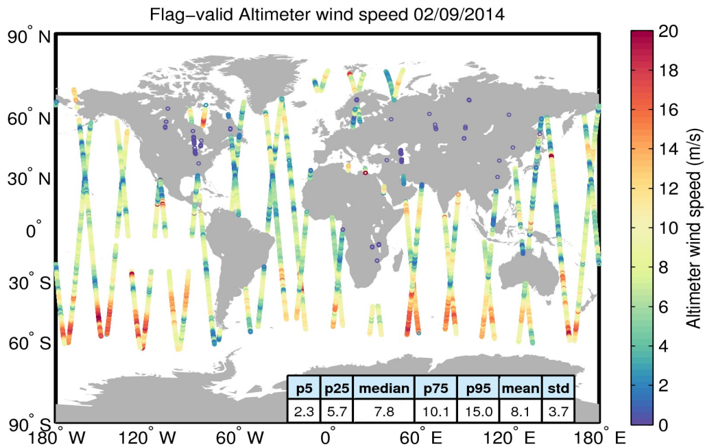
Figure 31. Geographical distribution of flag-valid wind data over oceans and lakes for 02/09/2014. The statistical values shown in the table refer to the wind in m/s and are calculated over all measurements shown in the figure.
