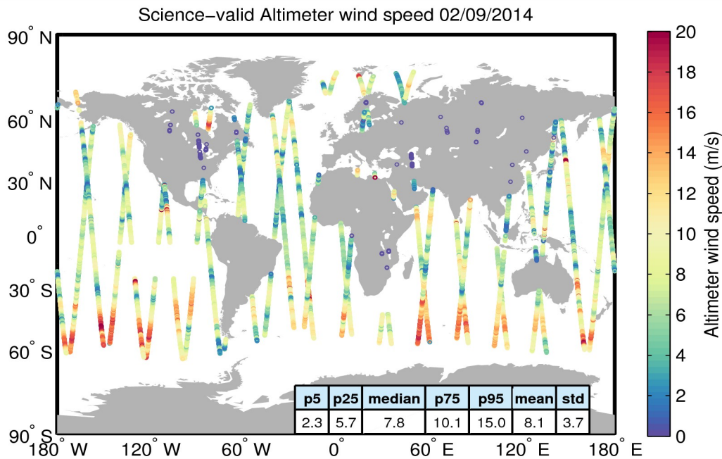
Figure 34. Geographical distribution of science-valid wind data over oceans and lakes for 02/09/2014. The statistical values shown in the table refer to the wind in m/s and are calculated over all measurements shown in the figure. Gray circles denote records that have been rejected based on the editing criteria described in Table 5.
