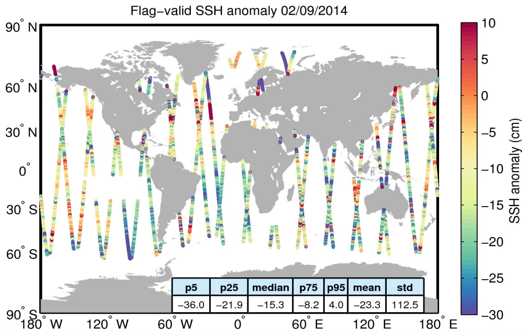
Figure 5. Geographical distribution of flag-valid 1-Hz SSH anomaly data over oceans and lakes for 02/09/2014. The statistical values shown in the table refer to the SSH anomaly in cm and are calculated over all measurements shown in the figure.
