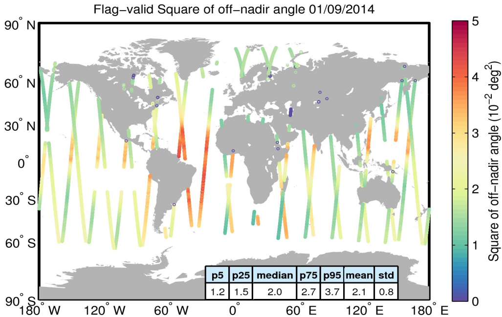
Figure 37. Geographical distribution of flag-valid mispointing data over oceans and lakes for 01/09/2014. The statistical values shown in the table refer to the mispointing in 10^{-2} \text{ deg}^2 and are calculated over all measurements shown in the figure.
