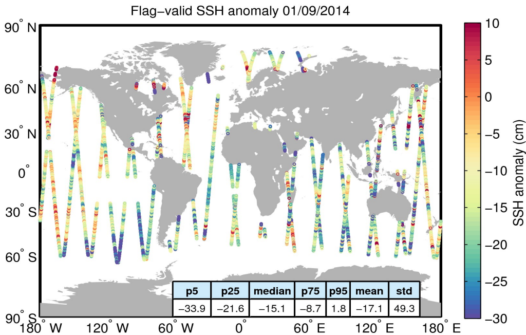
Figure 5. Geographical distribution of flag-valid 1-Hz SSH anomaly data over oceans and lakes for 01/09/2014. The statistical values shown in the table refer to the SSH anomaly in cm and are calculated over all measurements shown in the figure.
