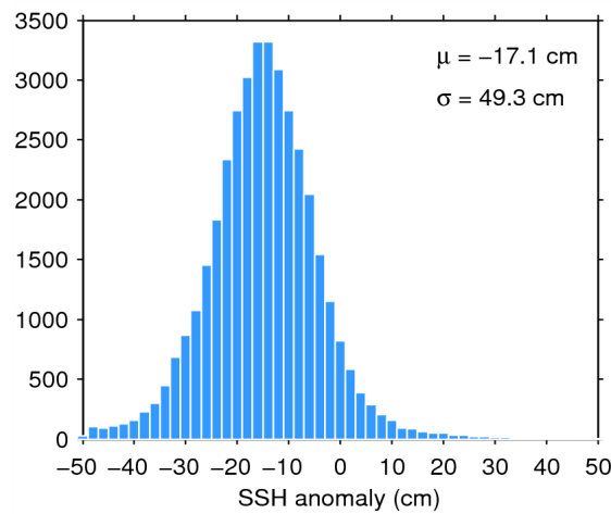
Figure 7. Histogram of flag-valid SSH anomaly over oceans and lakes for 01/09/2014. The mean ( \mu ) and standard deviation ( \sigma ) are also shown. Note that values outside [-50\ 50] cm are excluded from the histogram for the sake of readability but not from the computation of \mu and \sigma .
