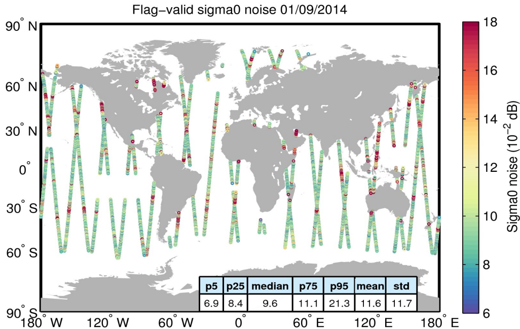
Figure 26. Geographical distribution of flag-valid 20-Hz sigma0 measurement noise over oceans and lakes for 01/09/2014. The statistical values shown in the table refer to the sigma0 noise and are calculated over all measurements shown in the figure.
