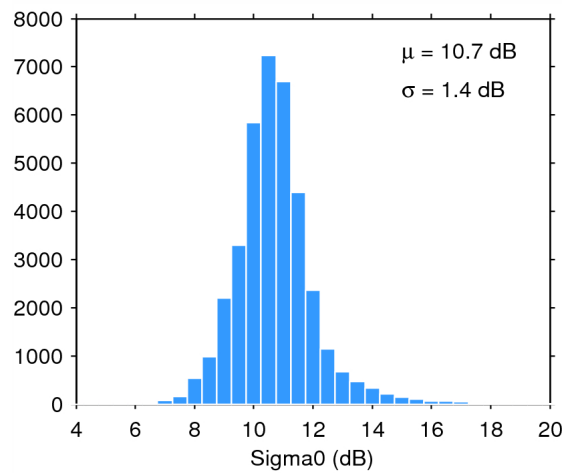
Figure 28. Histogram of science-valid sigma0 over oceans and lakes for 01/09/2014. The mean ( \mu ) and standard deviation ( \sigma ) are also shown. Note that values outside [4 20] dB are excluded from the histogram for the sake of readability but not from the computation of \mu and \sigma .
