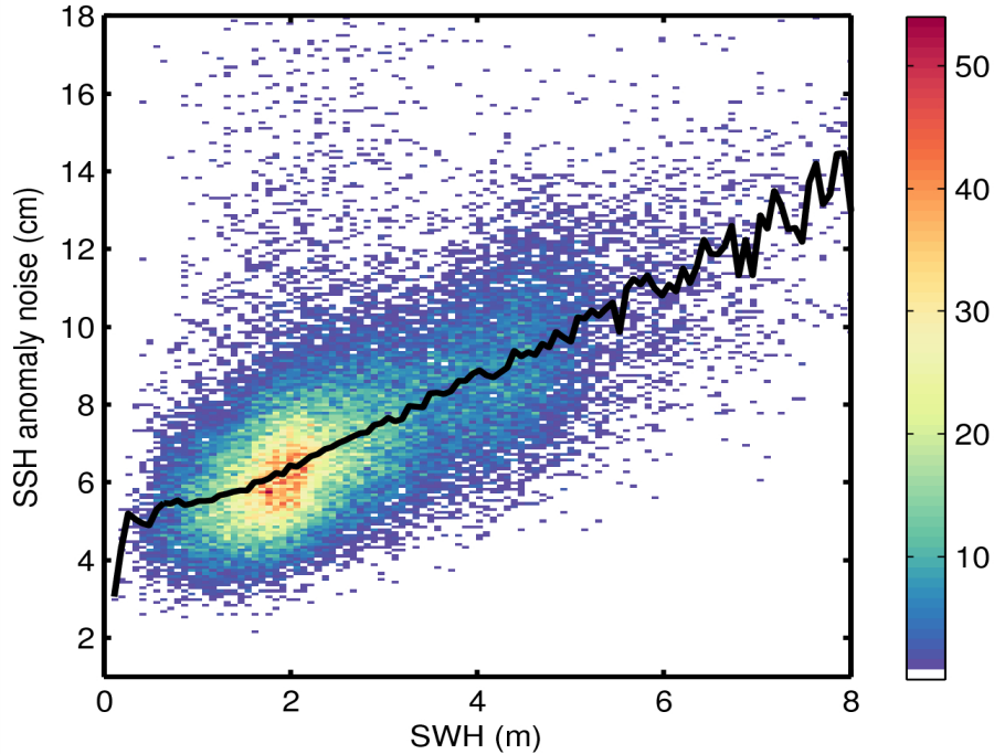
Figure 9. 2D histogram showing flag-valid SSH anomaly noise as a function of SWH for 01/09/2014. The black line denotes the median SSH anomaly as a function of SWH.
