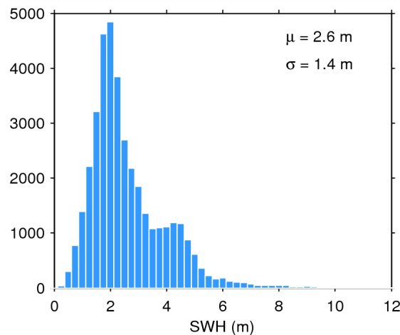
Figure 20. Histogram of science-valid SWH over oceans and lakes for 01/09/2014. The mean ( \mu ) and standard deviation ( \sigma ) are also shown. Note that values larger than 12 m are excluded from the histogram for the sake of readability but not from the computation of \mu and \sigma .
