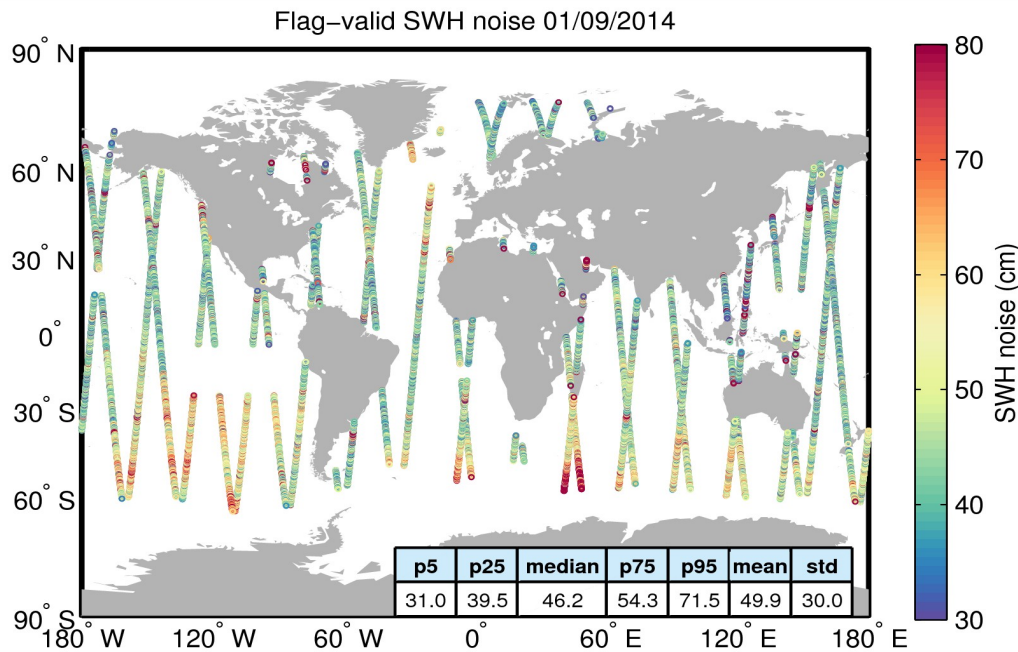
Figure 18. Geographical distribution of flag-valid 20-Hz SWH measurement noise over oceans and lakes for 01/09/2014. The statistical values shown in the figure refer to the SWH noise and are calculated over all measurements shown in the figure.
