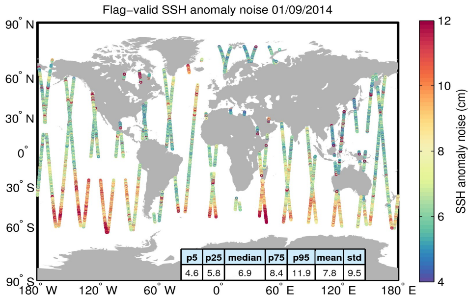
Figure 8. Geographical distribution of flag-valid 20-Hz SSH anomaly measurement noise over oceans and lakes for 01/09/2014. The statistical values shown in the table refer to the SSH anomaly noise and are calculated over all measurements shown in the figure.
