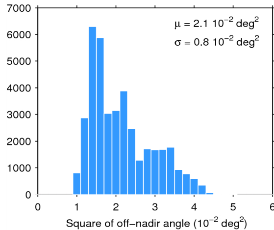
Figure 39. Histogram of flag-valid mispointing over oceans and lakes for 01/09/2014. The mean ( \mu ) and standard deviation ( \sigma ) are also shown. Note that values than 6 \cdot 10^{-2} \text{ deg}^2 are excluded from the histogram for the sake of readability but not from the computation of \mu and \sigma .
