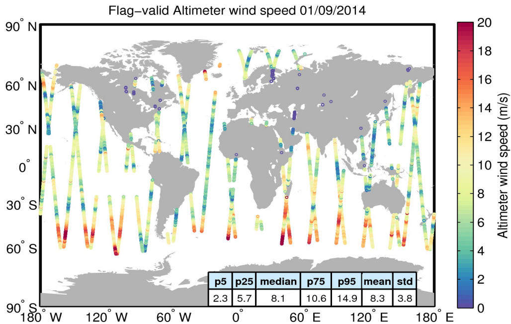
Figure 31. Geographical distribution of flag-valid wind data over oceans and lakes for 01/09/2014. The statistical values shown in the table refer to the wind in m/s and are calculated over all measurements shown in the figure.
