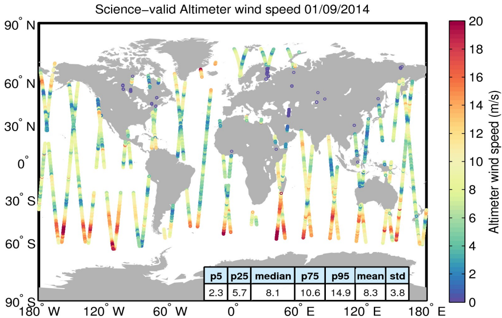
Figure 34. Geographical distribution of science-valid wind data over oceans and lakes for 01/09/2014. The statistical values shown in the table refer to the wind in m/s and are calculated over all measurements shown in the figure. Gray circles denote records that have been rejected based on the editing criteria described in Table 5.
