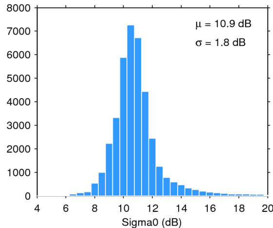
Figure 25. Histogram of flag-valid sigma0 over oceans and lakes for 01/09/2014. The mean ( \mu ) and standard deviation ( \sigma ) are also shown. Note that values outside [4 20] dB are excluded from the histogram for the sake of readability but not from the computation of \mu and \sigma .
