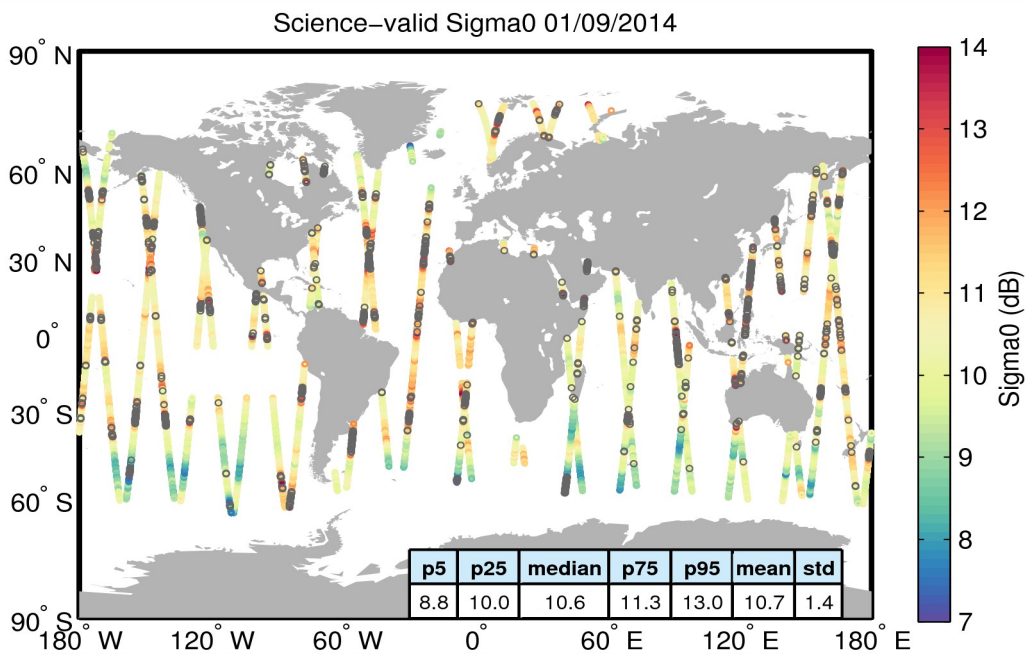
Figure 27. Geographical distribution of science-valid sigma0 data over oceans and lakes for 01/09/2014. The statistical values shown in the table refer to the sigma0 in dB and are calculated over all measurements shown in the figure. Gray circles denote records that have been rejected based on the editing criteria described in Table 4.
