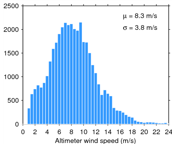
Figure 35. Histogram of science-valid wind over oceans and lakes for 01/09/2014. The mean ( \mu ) and standard deviation ( \sigma ) are also shown. Note that values larger than 24 m/s are excluded from the histogram for the sake of readability but not from the computation of \mu and \sigma .
