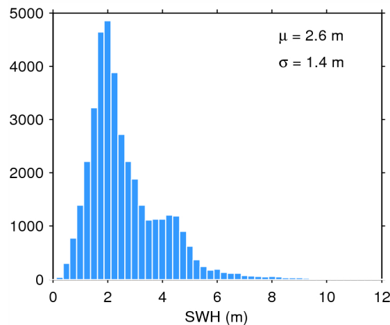
Figure 17. Histogram of flag-valid SWH over oceans and lakes for 01/09/2014. The mean ( \mu ) and standard deviation ( \sigma ) are also shown. Note that values larger than 12 m are excluded from the histogram for the sake of readability but not from the computation of \mu and \sigma .
