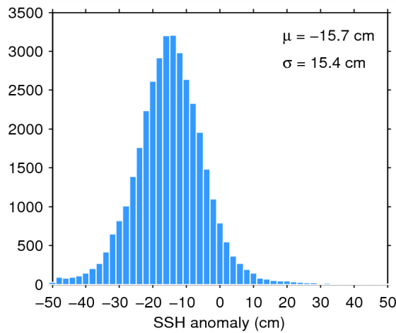
Figure 11. Histogram of science-valid SSH anomaly over oceans and lakes for 01/09/2014. The mean ( \mu ) and standard deviation ( \sigma ) are also shown. Note that values outside [-50 50] cm are excluded from the histogram for the sake of readability but not from the computation of \mu and \sigma .
