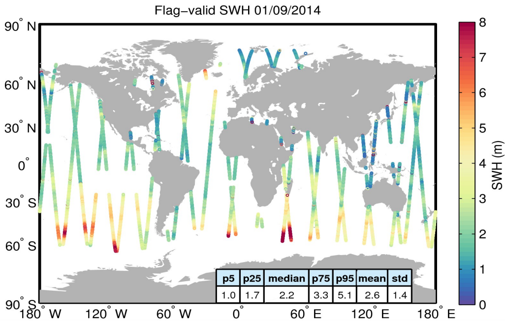
Figure 15. Geographical distribution of flag-valid SWH data over oceans and lakes for 01/09/2014. The statistical values shown in the table refer to the SWH in m and are calculated over all measurements shown in the figure.
