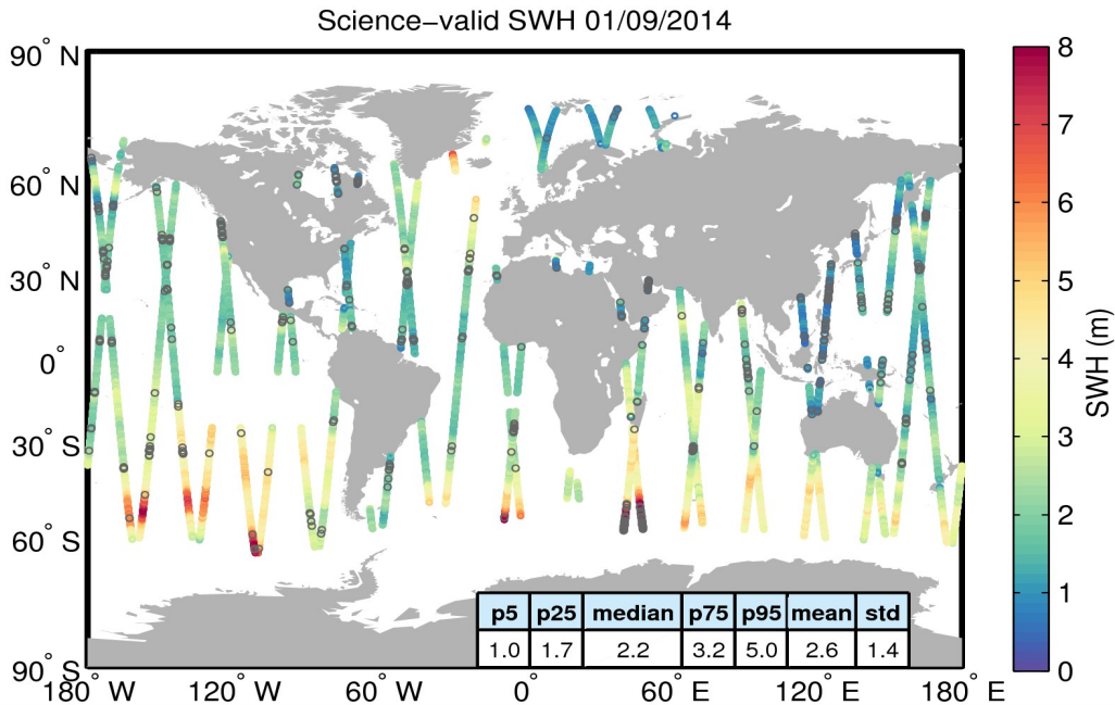
Figure 19. Geographical distribution of science-valid SWH data over oceans and lakes for 01/09/2014. The statistical values shown in the table refer to the SWH in m and are calculated over all measurements shown in the figure. Gray circles denote records that have been rejected based on the editing criteria described in Table 3.
