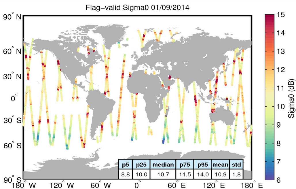
Figure 23. Geographical distribution of flag-valid sigma0 data over oceans and lakes for 01/09/2014. The statistical values shown in the table refer to the sigma0 in dB and are calculated over all measurements shown in the figure.
