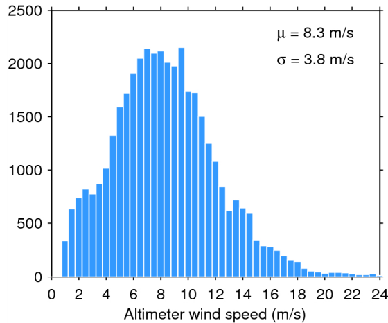
Figure 33. Histogram of flag-valid wind over oceans and lakes for 01/09/2014. The mean ( \mu ) and standard deviation ( \sigma ) are also shown. Note that values larger than 24 m/s are excluded from the histogram for the sake of readability but not from the computation of \mu and \sigma .
